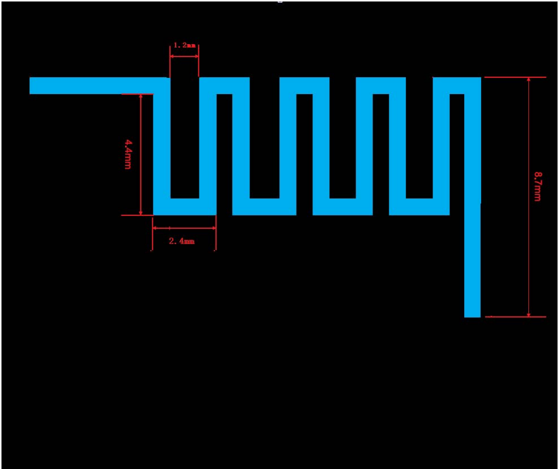
Antenna physical and physical dimensions
