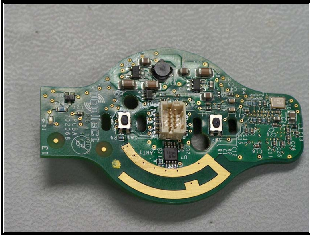
Photograph 11: Internal PCB - Top View
