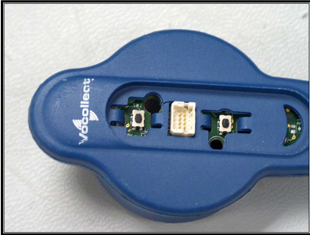
Photograph 9: SRX Wireless Headset without Keypad
