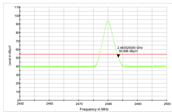
DH5-Channel 78: Average
