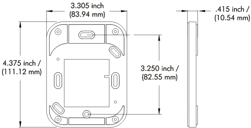
FIGURE 1. Model SWH-1100 Reader Backplate (includes tamper switch magnet)
