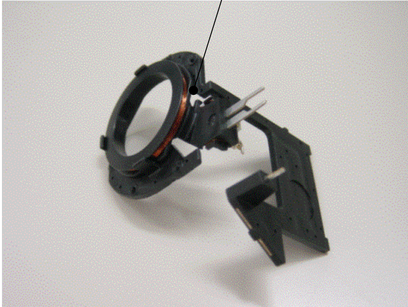
Immobilizer Antenna
