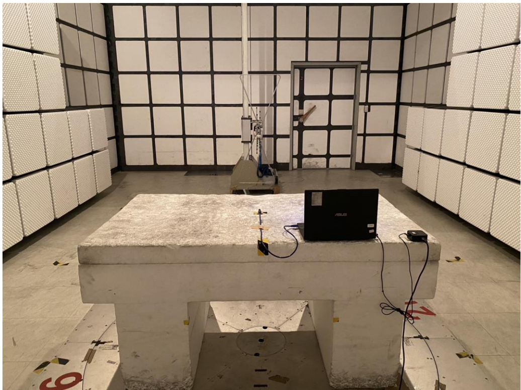
Rear View
