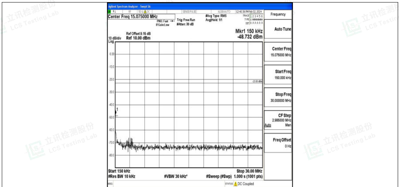
Band26_15MHz_16QAM_26865_1RB#0_0.15~30_0.15~30
