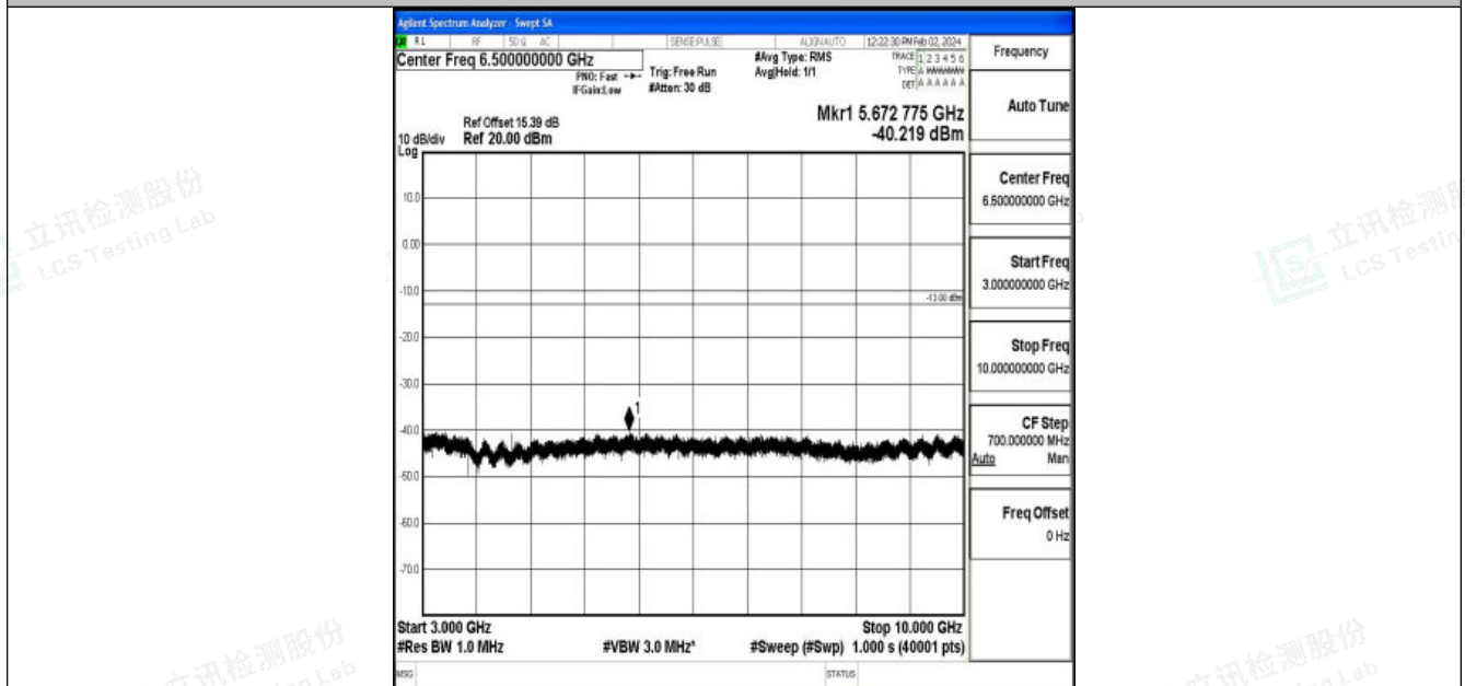
Band26_10MHz_16QAM_26915_1RB#0_3000~10000_3000~10000
