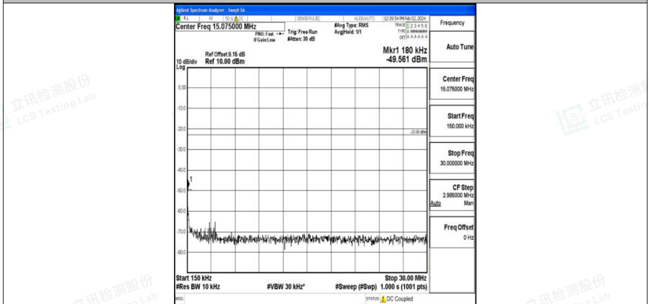
Band26_15MHz_QPSK_26865_1RB#0_0.15~30_0.15~30
