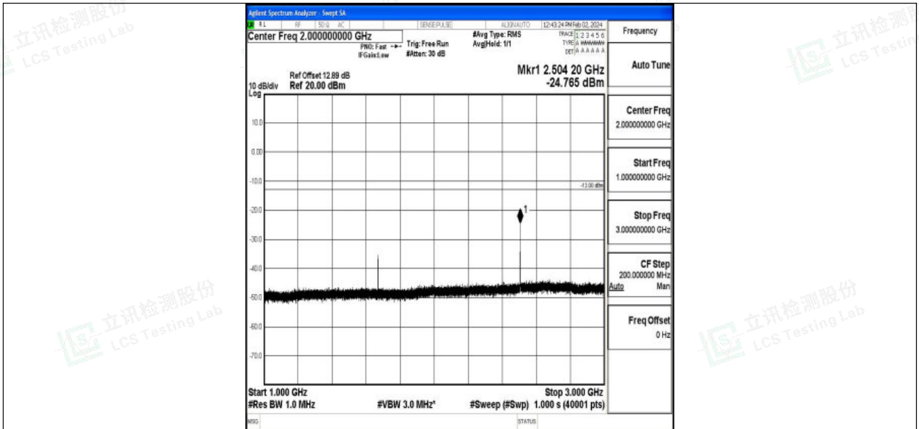
Band26_15MHz_16QAM_26965_1RB#0_1000~3000_1000~3000
