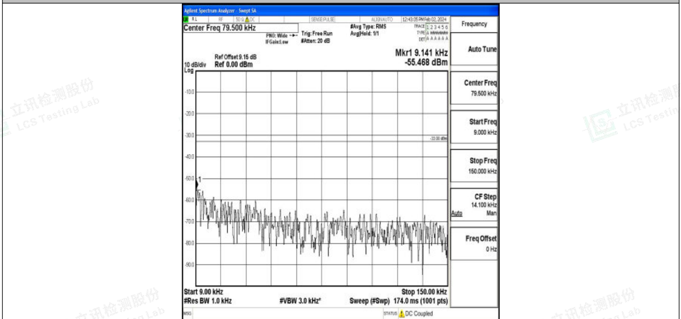
Band26_15MHz_16QAM_26965_1RB#0_0.009~0.15_0.009~0.15
