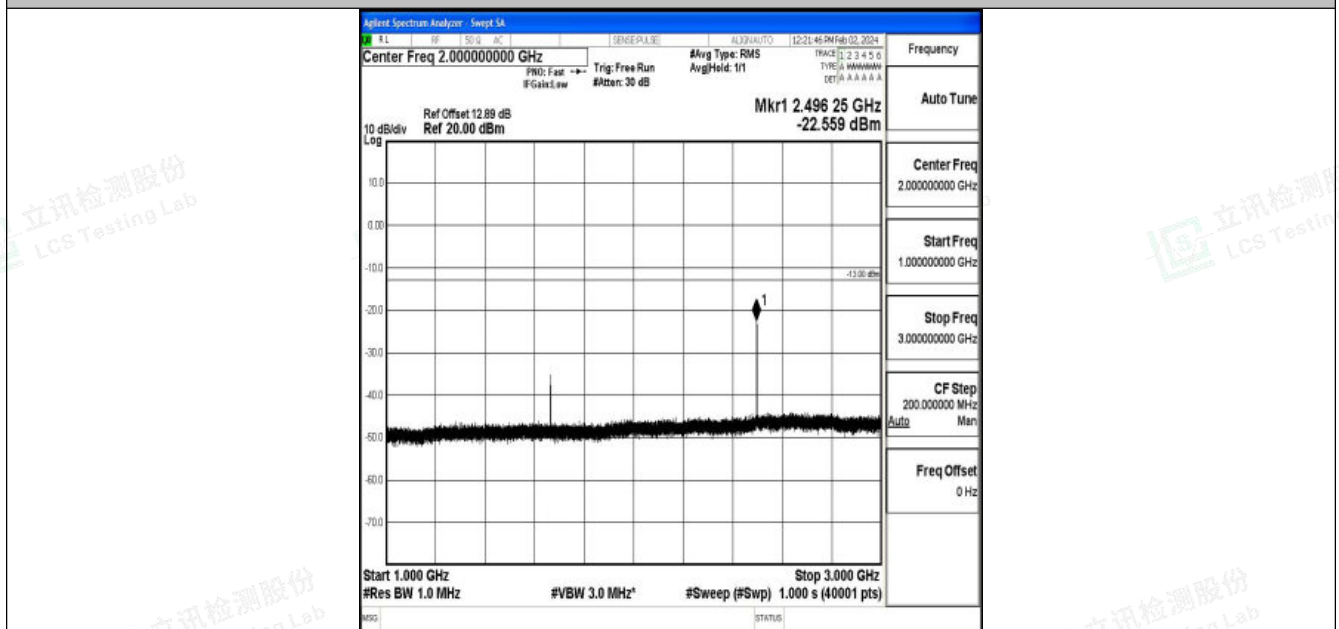
Band26_10MHz_QPSK_26915_1RB#0_1000~3000_1000~3000
