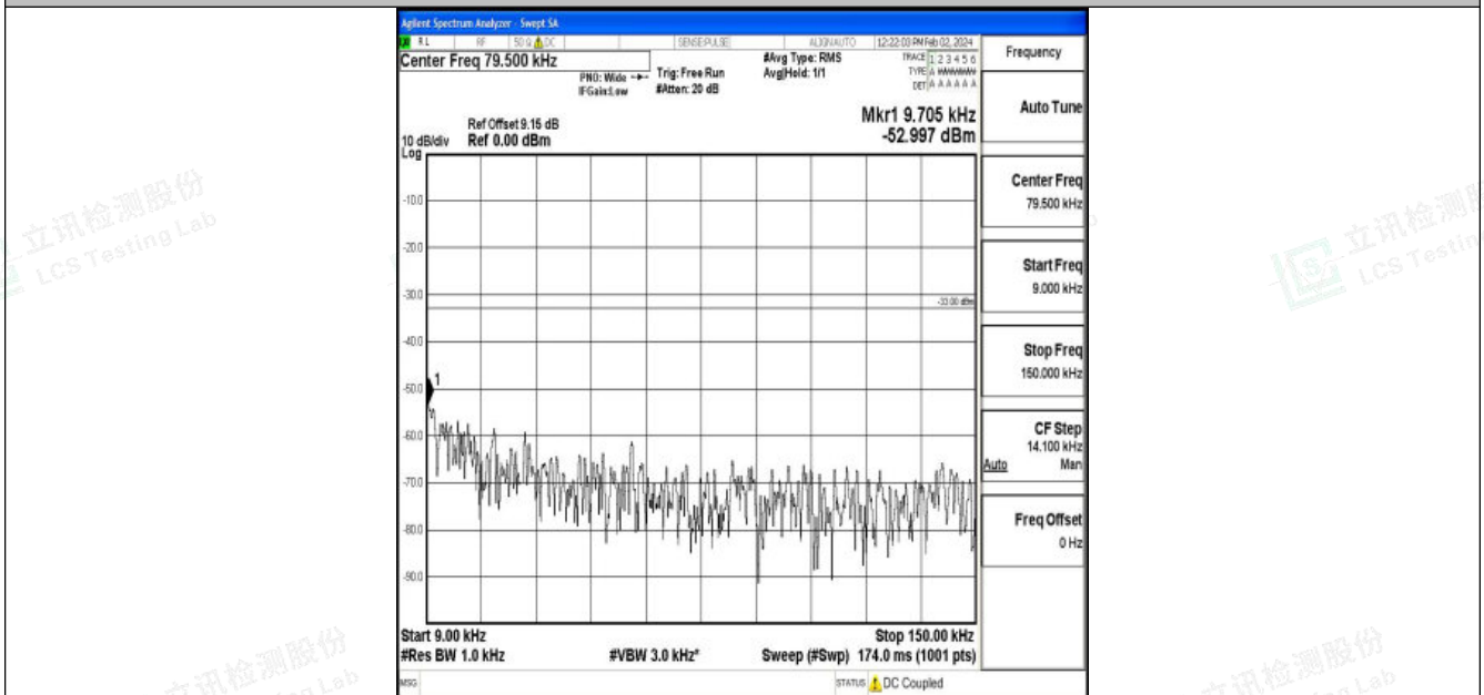
Band26_10MHz_16QAM_26915_1RB#0_0.009~0.15_0.009~0.15
