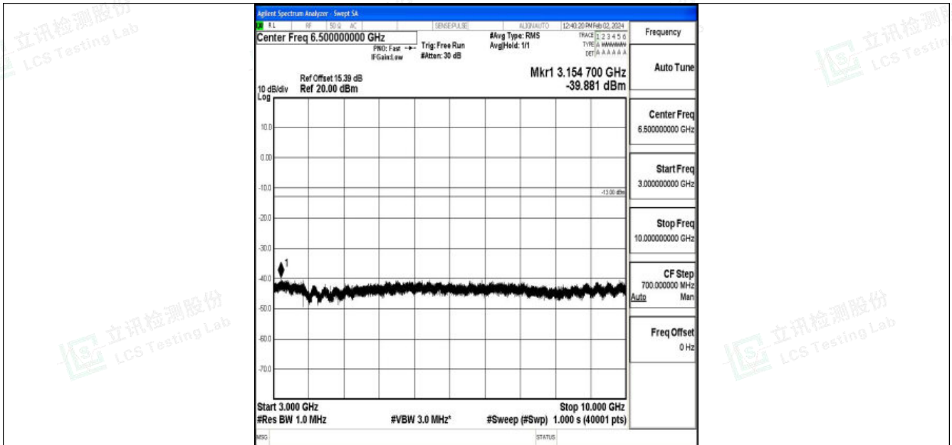
Band26_15MHz_QPSK_26865_1RB#0_3000~10000_3000~10000
