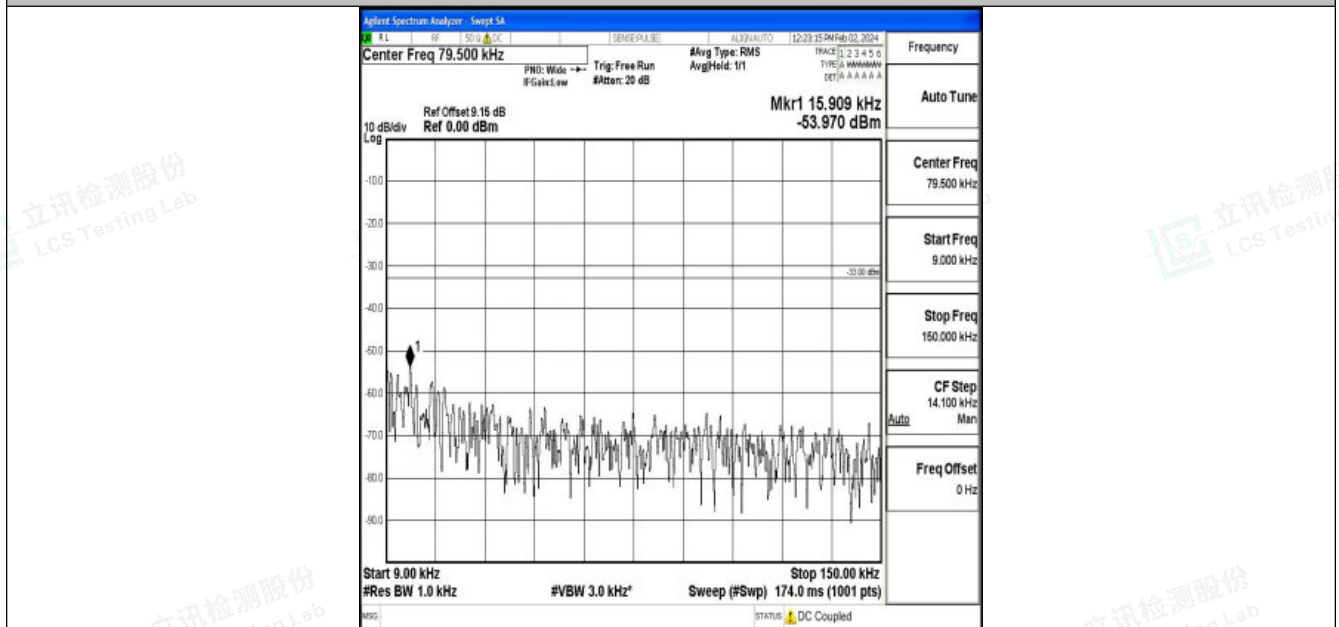
Band26_10MHz_16QAM_26990_1RB#0_0.009~0.15_0.009~0.15
