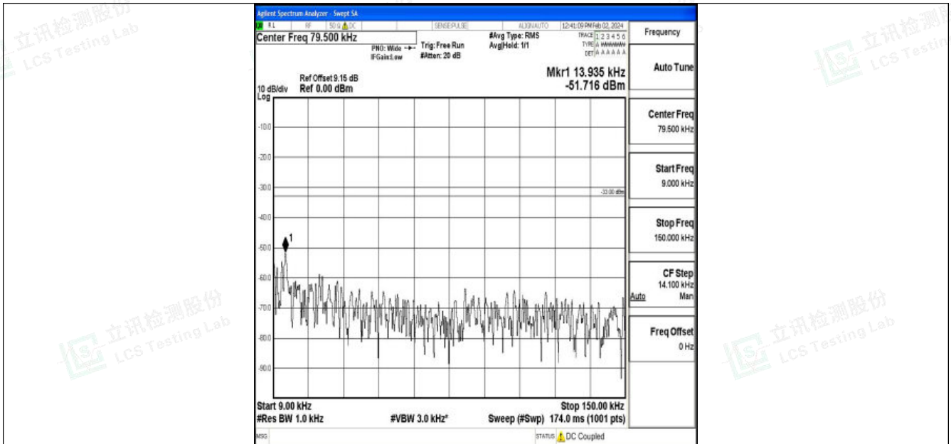
Band26_15MHz_QPSK_26915_1RB#0_0.009~0.15_0.009~0.15
