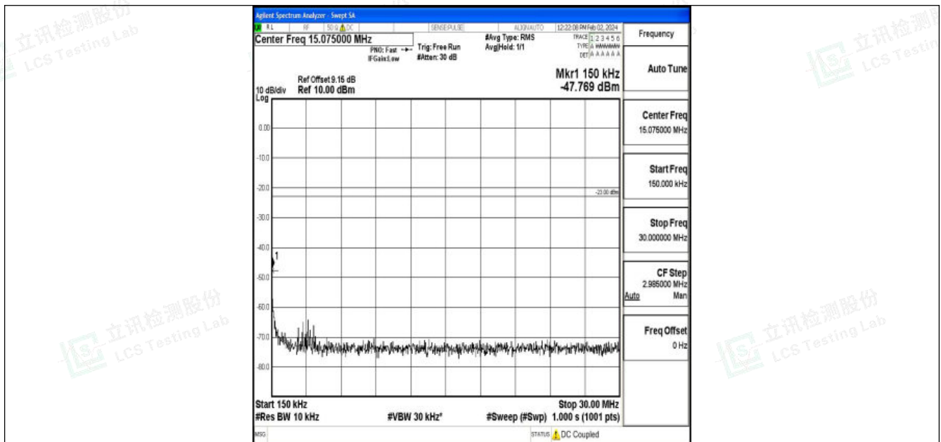
Band26_10MHz_16QAM_26915_1RB#0_0.15~30_0.15~30
