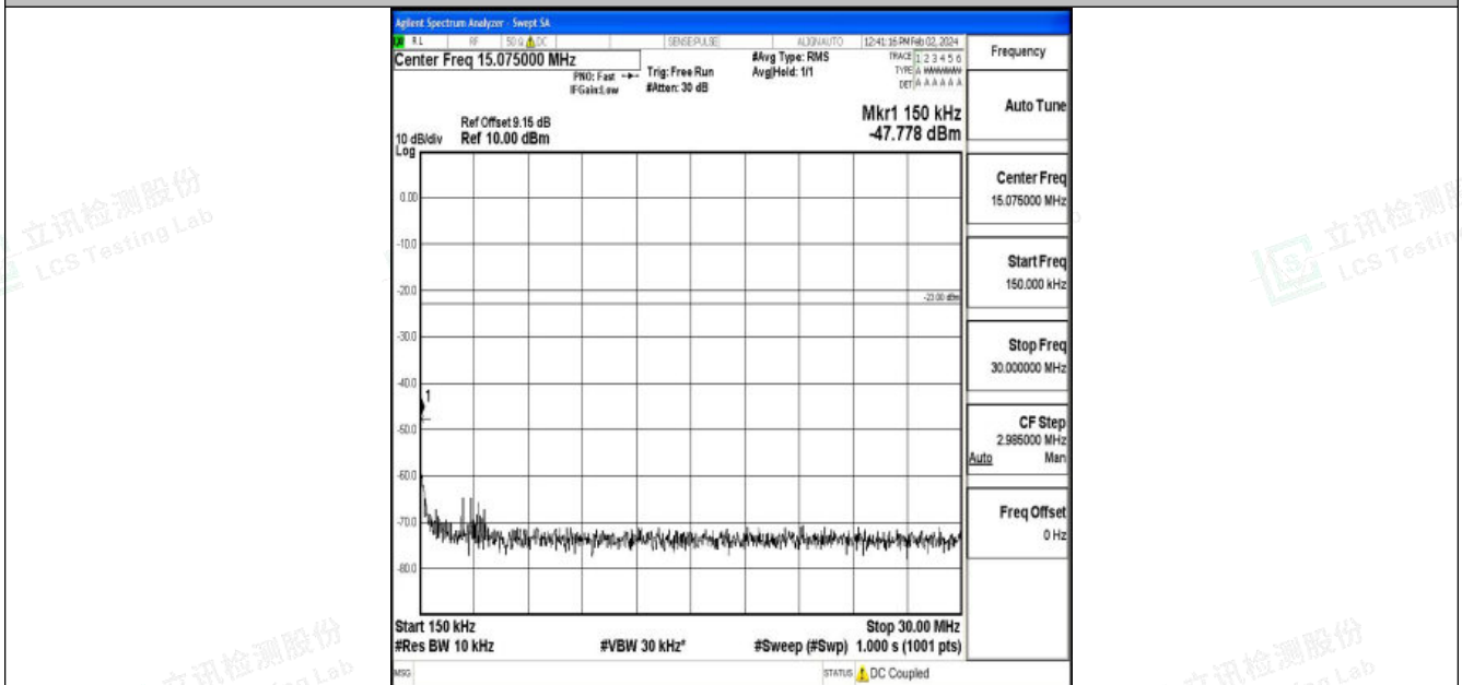
Band26_15MHz_QPSK_26915_1RB#0_0.15~30_0.15~30
