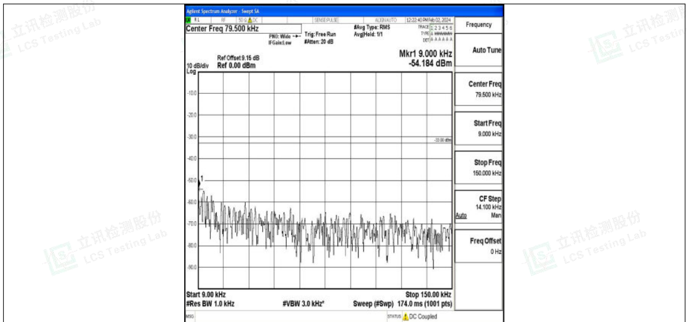
Band26_10MHz_QPSK_26990_1RB#0_0.009~0.15_0.009~0.15
