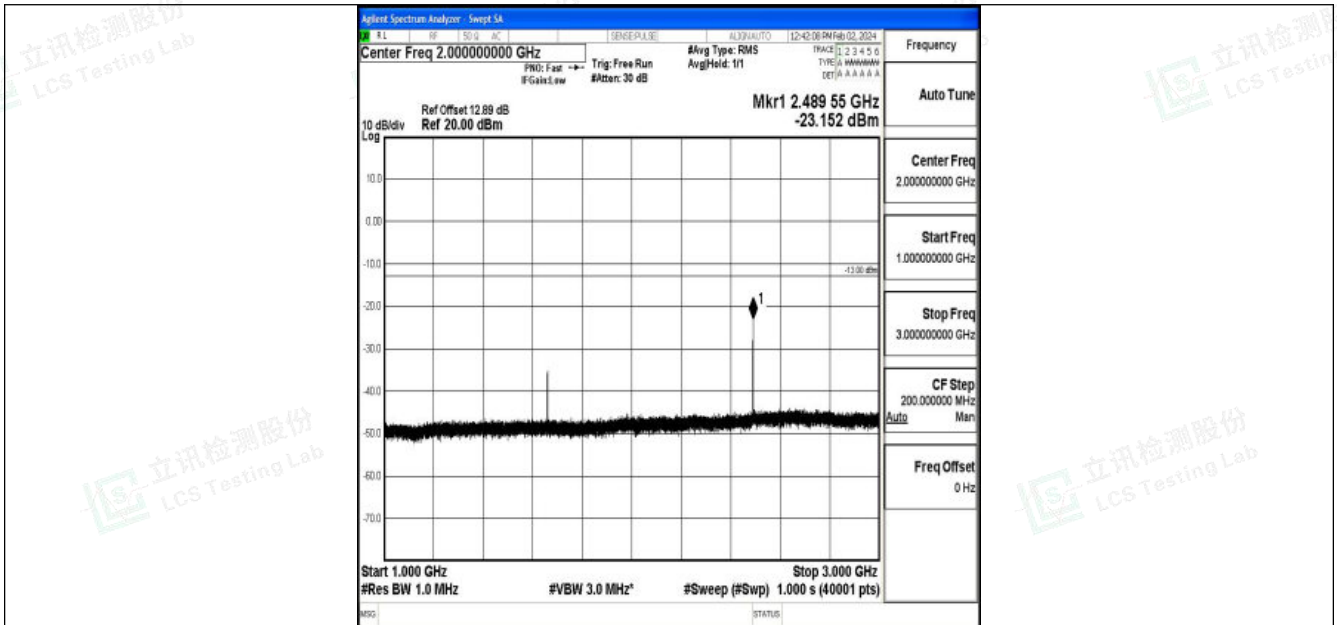
Band26_15MHz_16QAM_26915_1RB#0_1000~3000_1000~3000
