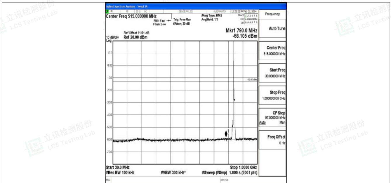
Band26_10MHz_QPSK_26990_1RB#0_30~1000_30~1000
