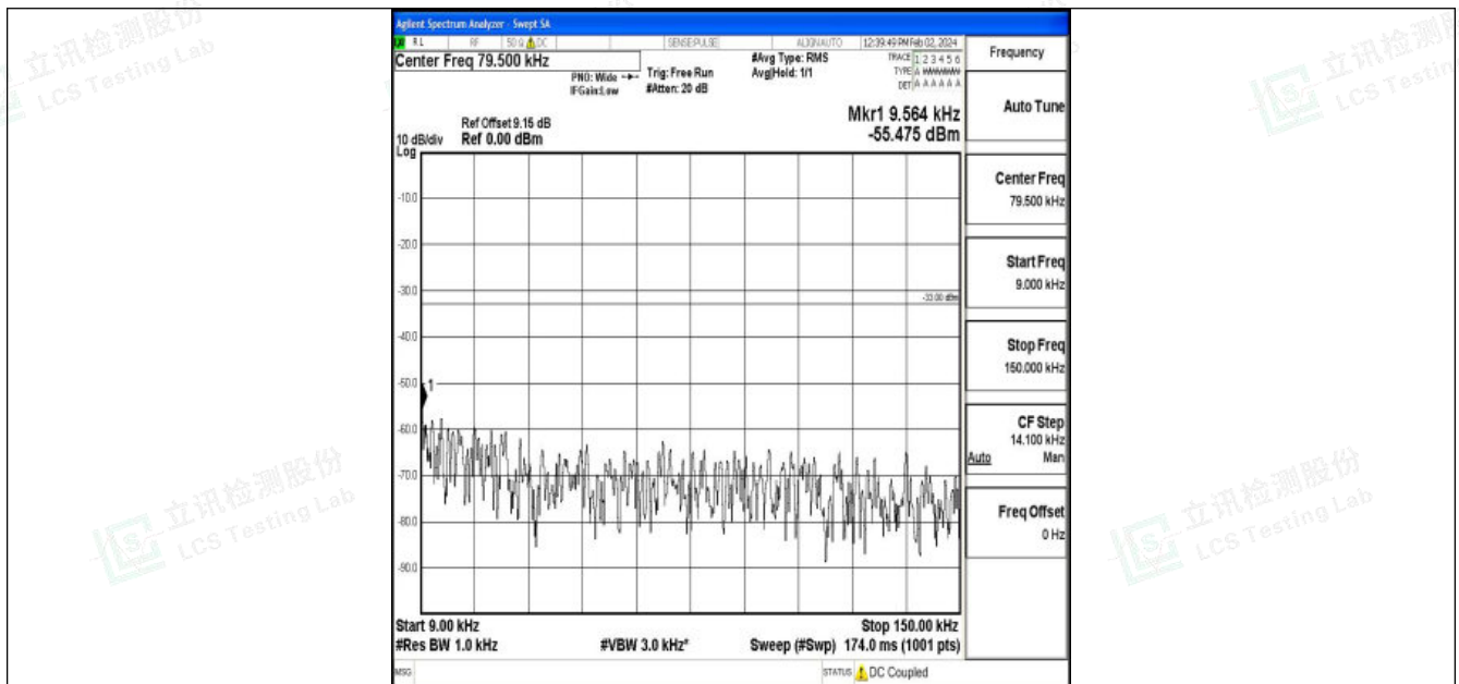
Band26_15MHz_QPSK_26865_1RB#0_0.009~0.15_0.009~0.15
