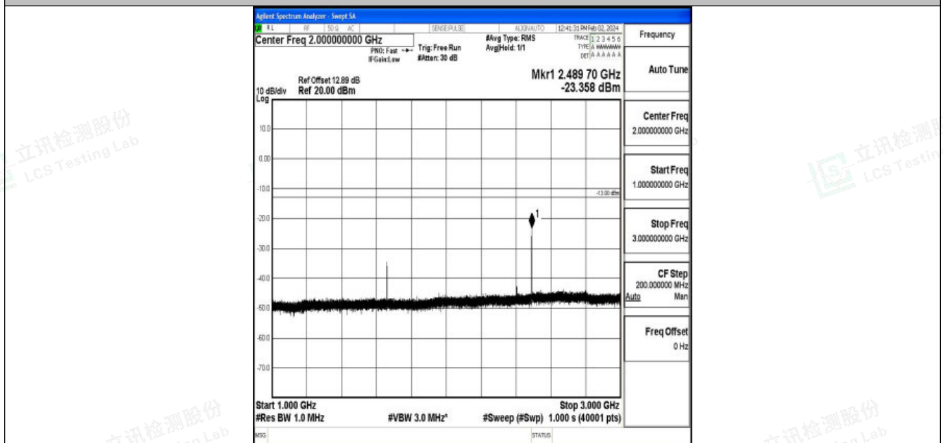
Band26_15MHz_QPSK_26915_1RB#0_1000~3000_1000~3000
