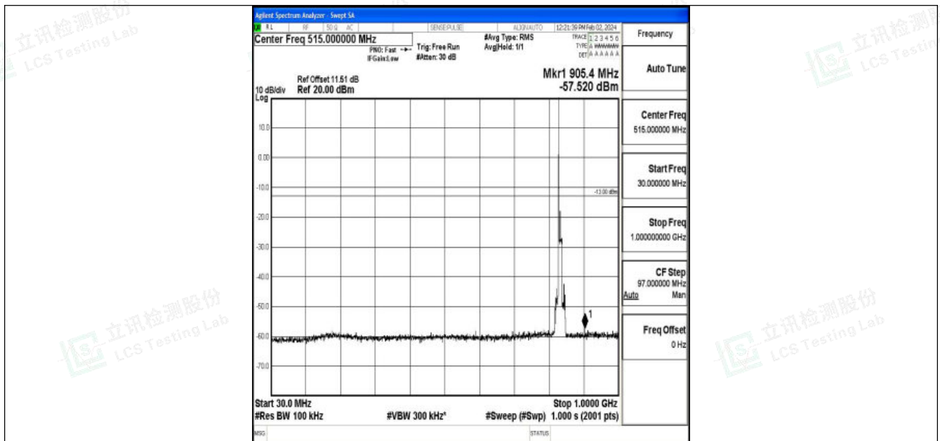
Band26_10MHz_QPSK_26915_1RB#0_30~1000_30~1000
