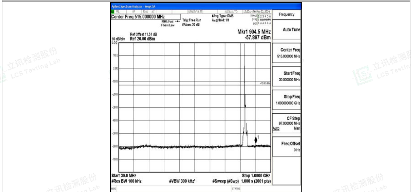
Band26_10MHz_16QAM_26915_1RB#0_30~1000_30~1000
