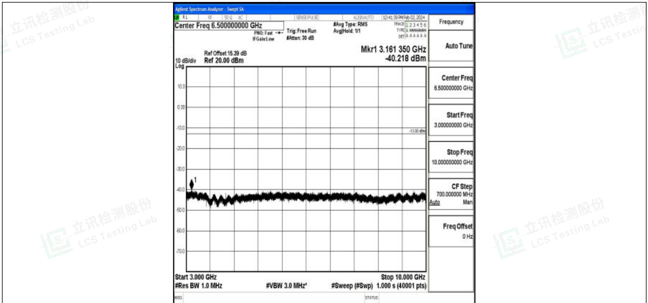
Band26_15MHz_QPSK_26915_1RB#0_3000~10000_3000~10000
