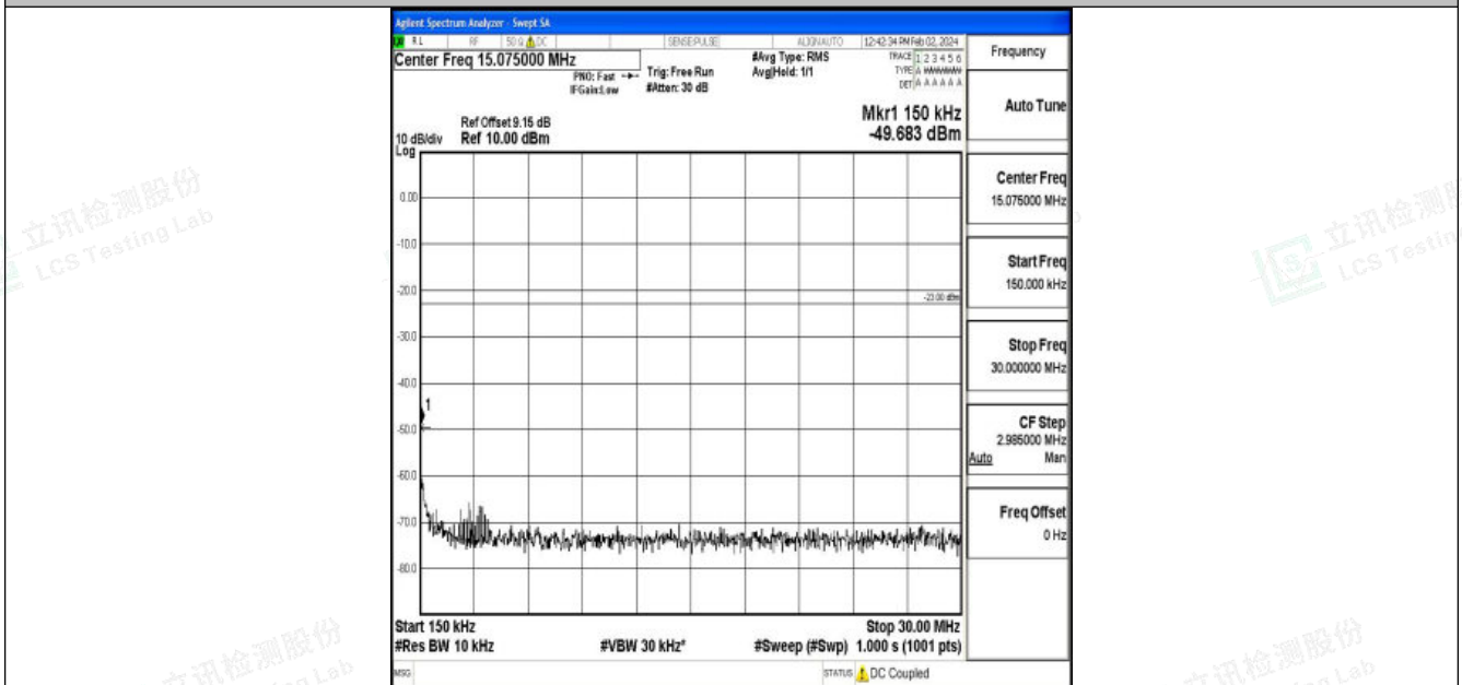
Band26_15MHz_QPSK_26965_1RB#0_0.15~30_0.15~30
