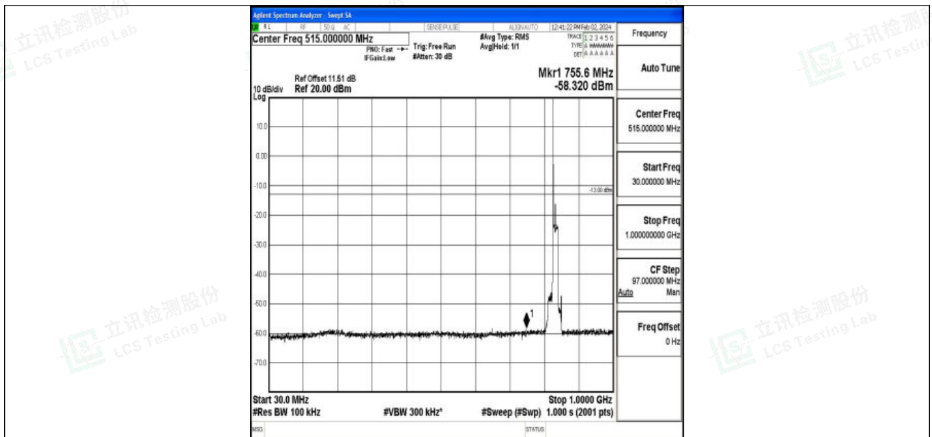
Band26_15MHz_QPSK_26915_1RB#0_30~1000_30~1000
