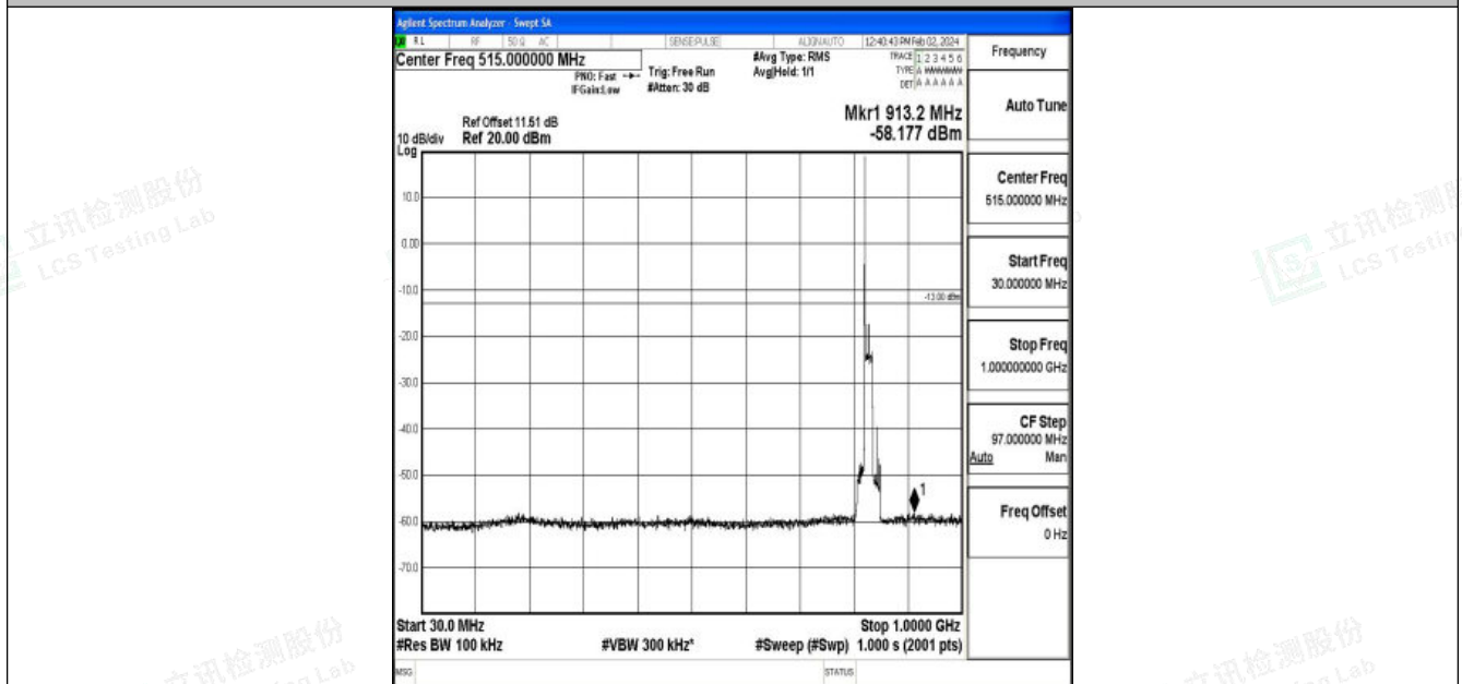
Band26_15MHz_16QAM_26865_1RB#0_30~1000_30~1000
