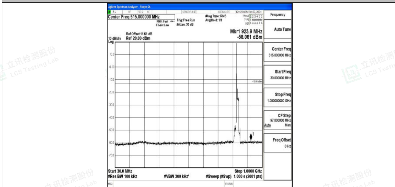
Band26_15MHz_16QAM_26915_1RB#0_30~1000_30~1000
