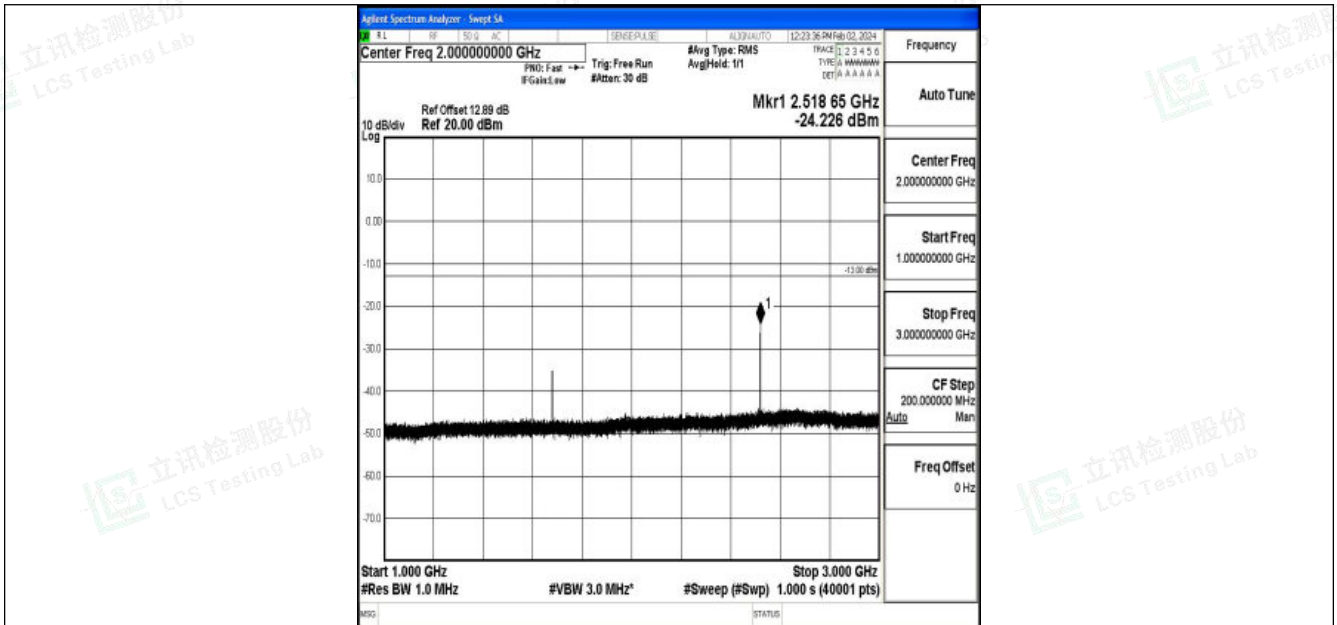
Band26_10MHz_16QAM_26990_1RB#0_1000~3000_1000~3000
