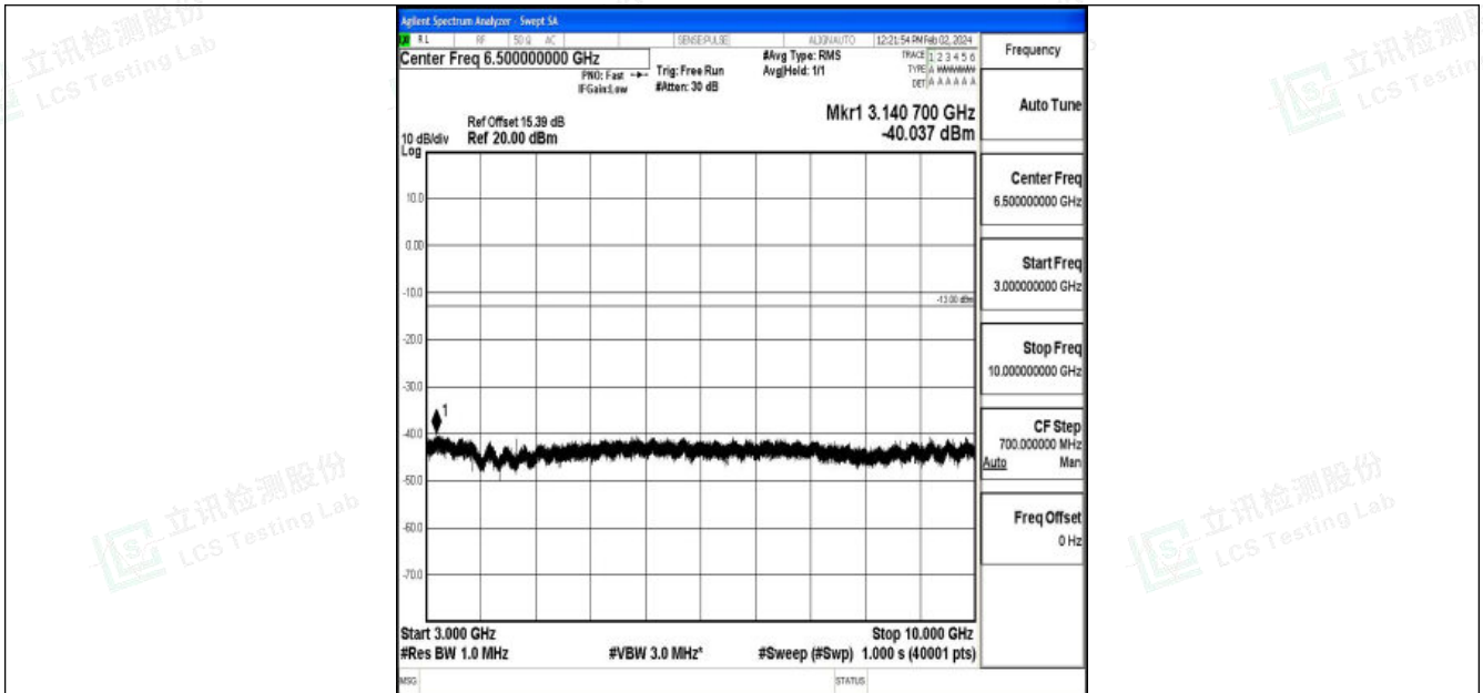
Band26_10MHz_QPSK_26915_1RB#0_3000~10000_3000~10000
