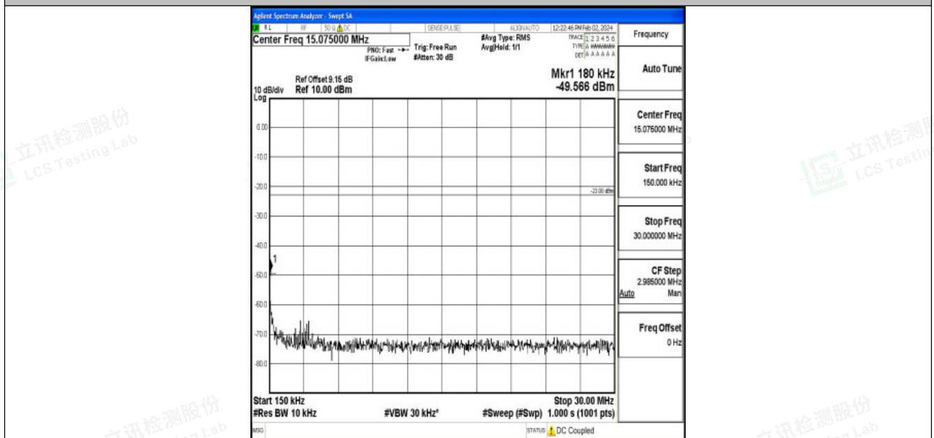
Band26_10MHz_QPSK_26990_1RB#0_0.15~30_0.15~30
