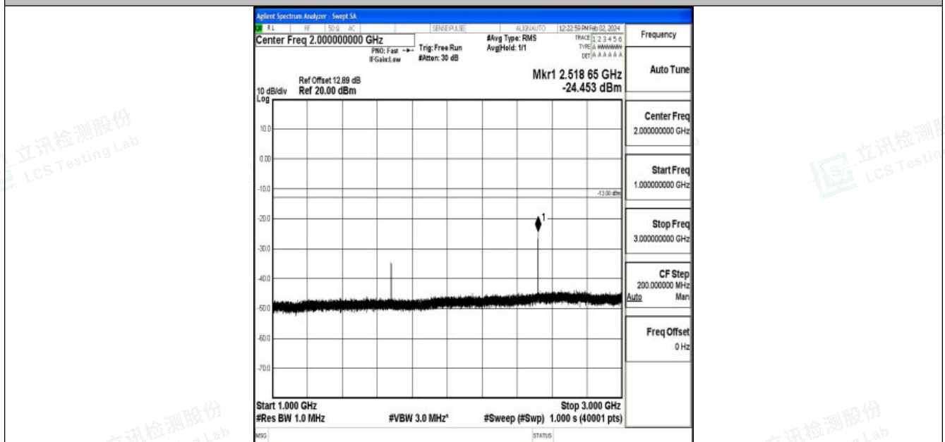
Band26_10MHz_QPSK_26990_1RB#0_1000~3000_1000~3000
