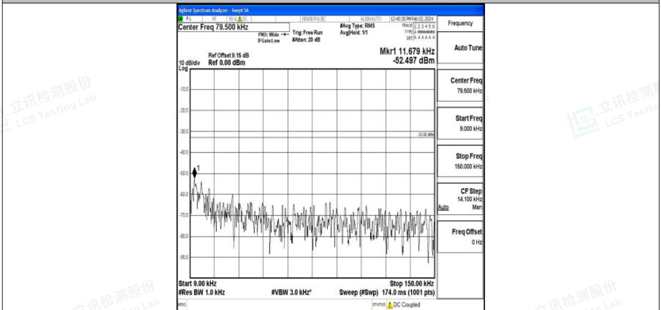
Band26_15MHz_16QAM_26865_1RB#0_0.009~0.15_0.009~0.15
