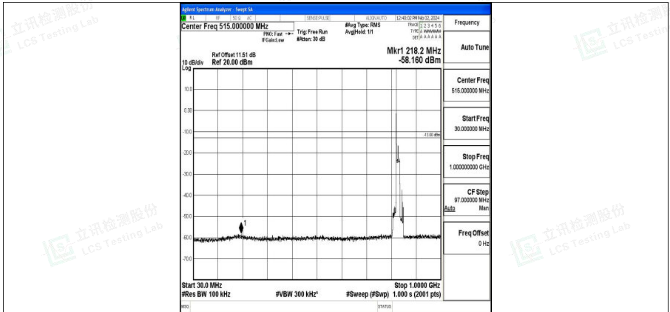
Band26_15MHz_QPSK_26865_1RB#0_30~1000_30~1000
