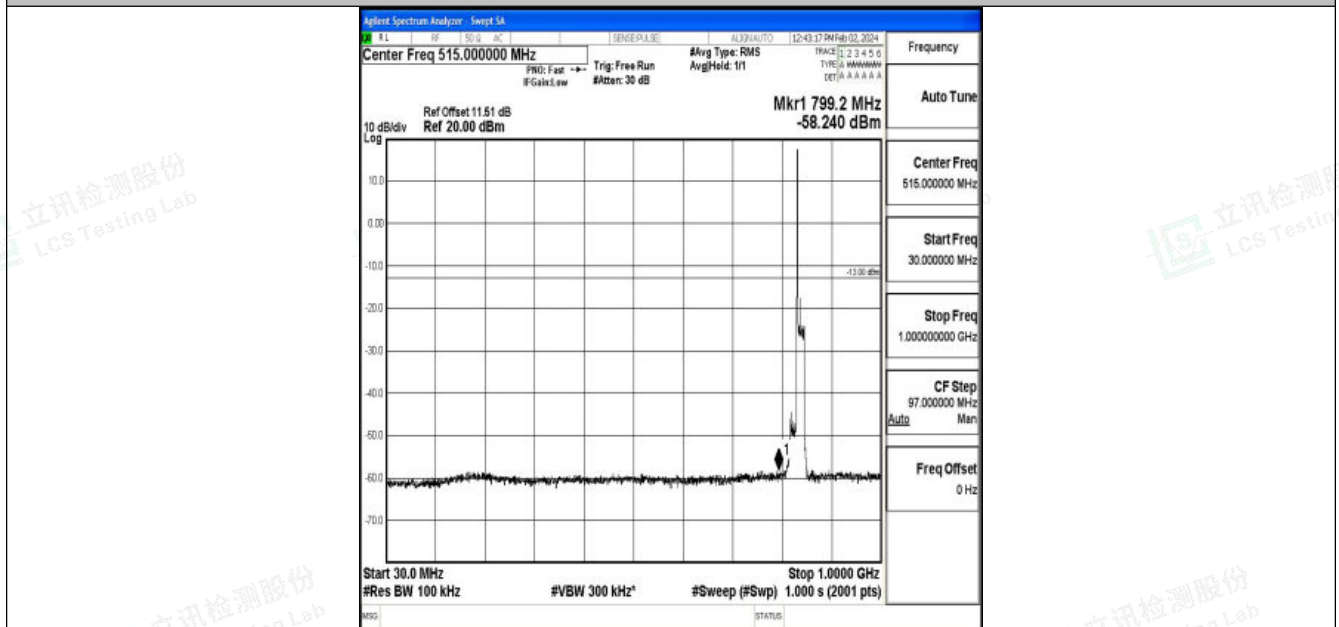
Band26_15MHz_16QAM_26965_1RB#0_30~1000_30~1000
