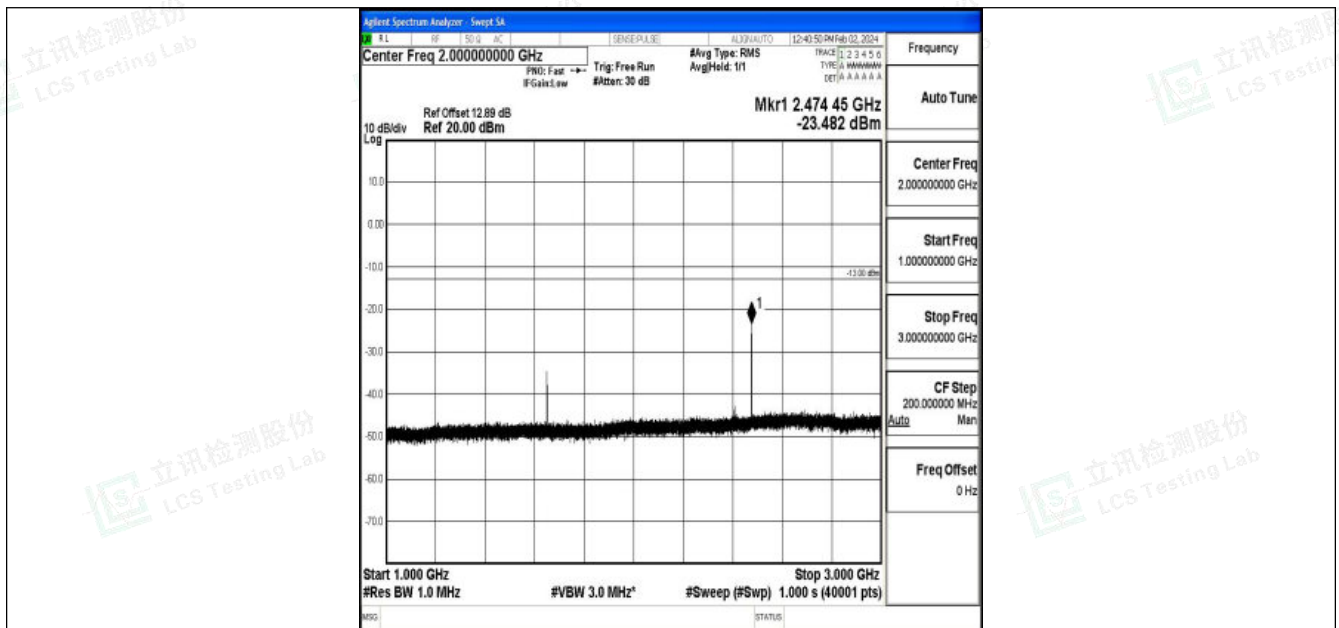
Band26_15MHz_16QAM_26865_1RB#0_1000~3000_1000~3000
