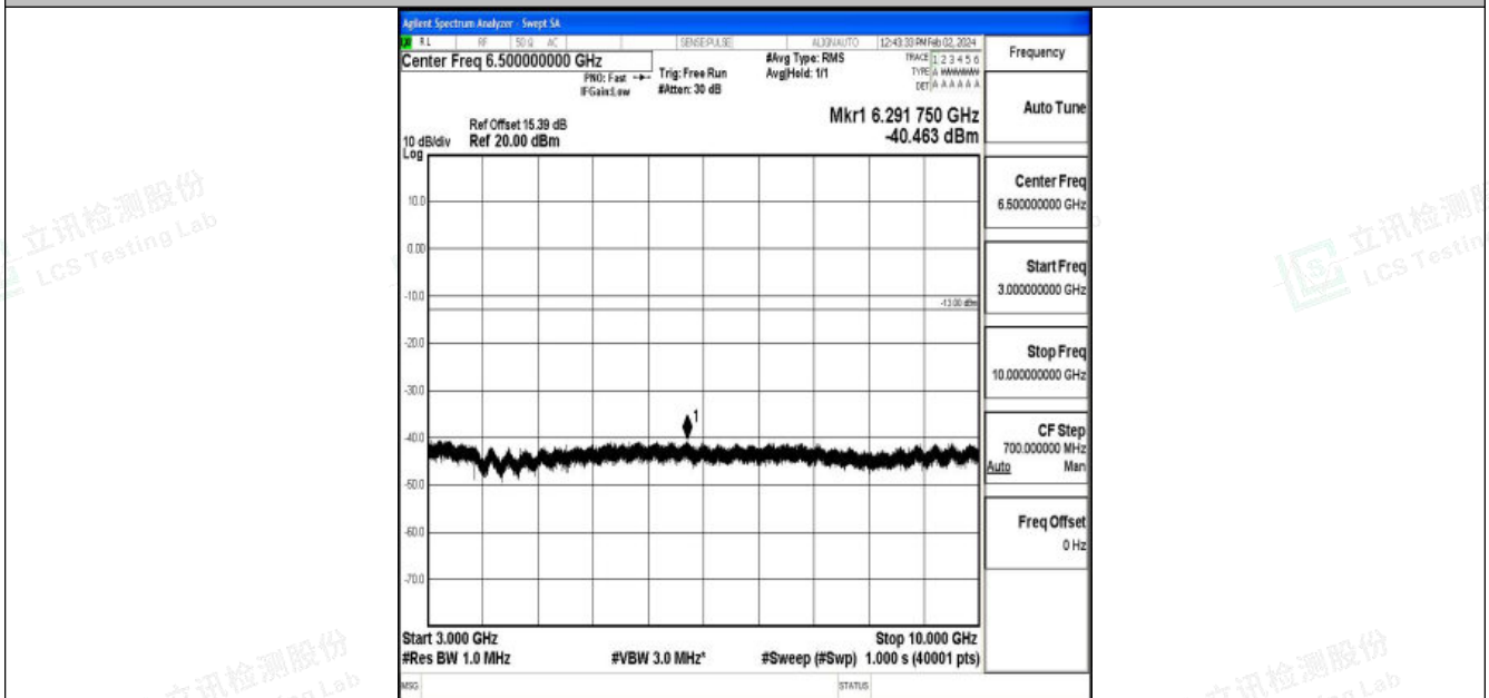
Band26_15MHz_16QAM_26965_1RB#0_3000~10000_3000~10000
