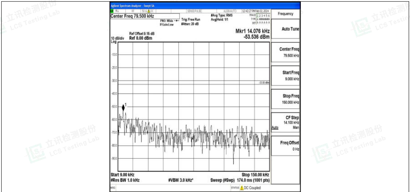
Band26_15MHz_QPSK_26965_1RB#0_0.009~0.15_0.009~0.15
