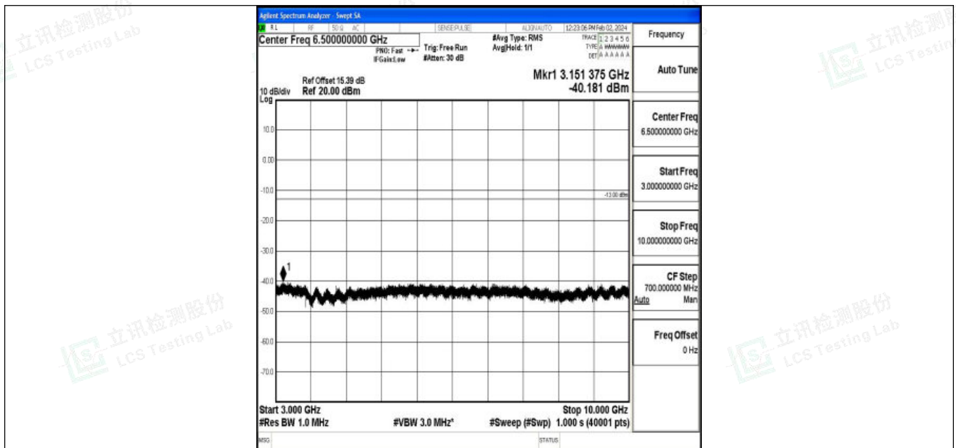
Band26_10MHz_QPSK_26990_1RB#0_3000~10000_3000~10000
