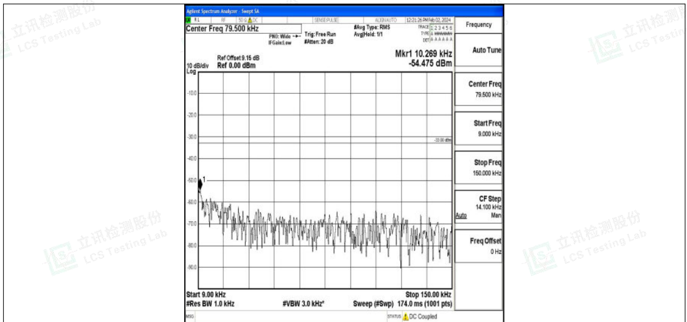
Band26_10MHz_QPSK_26915_1RB#0_0.009~0.15_0.009~0.15
