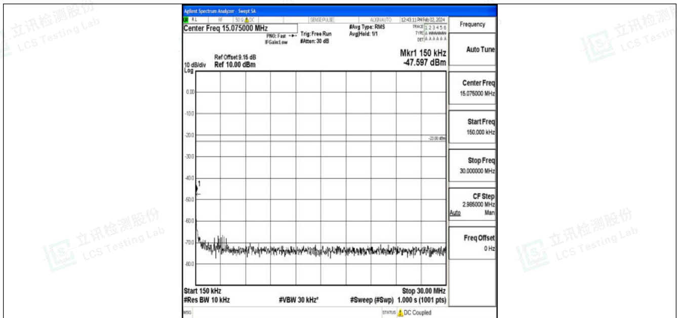
Band26_15MHz_16QAM_26965_1RB#0_0.15~30_0.15~30
