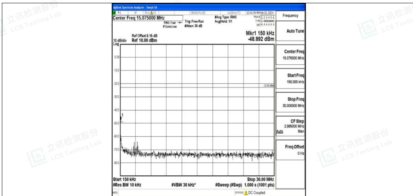
Band26_15MHz_16QAM_26915_1RB#0_0.15~30_0.15~30
