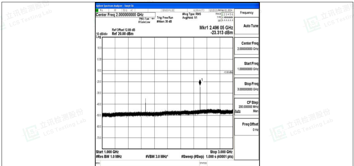
Band26_10MHz_16QAM_26915_1RB#0_1000~3000_1000~3000
