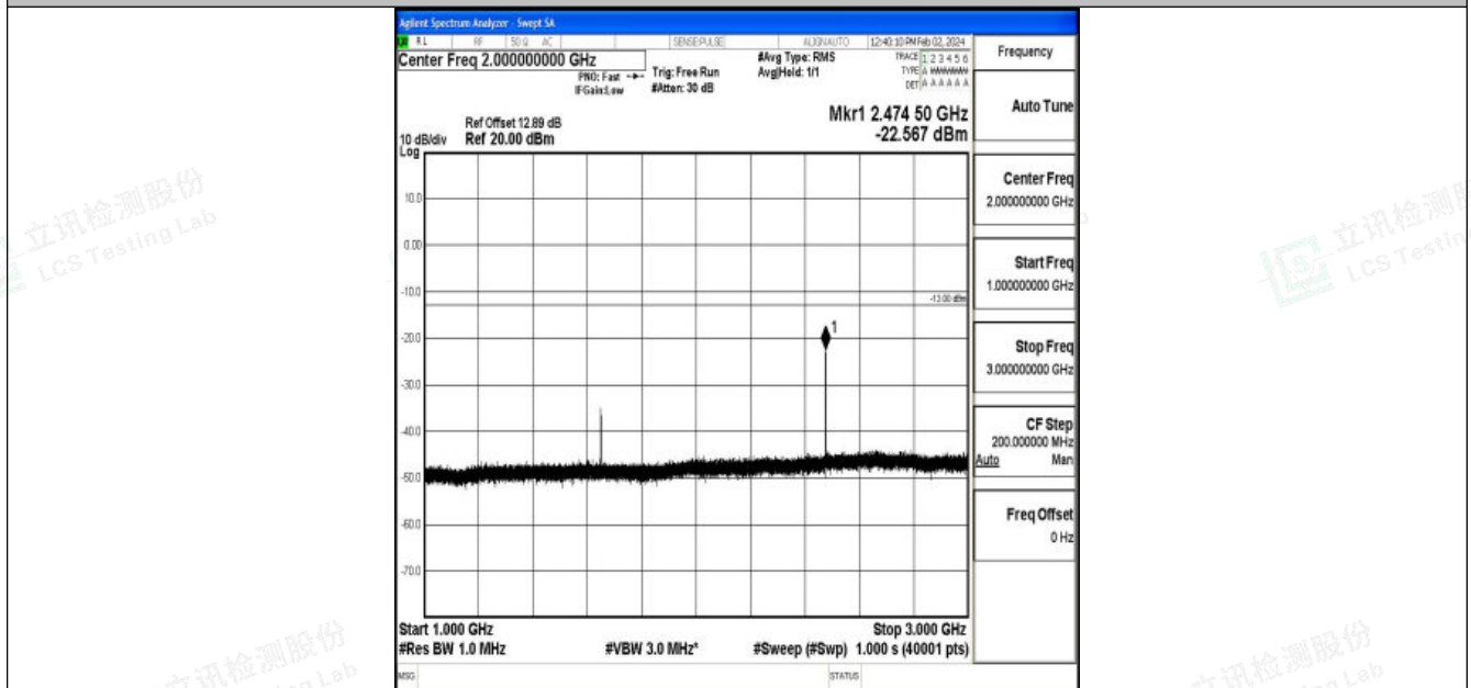
Band26_15MHz_QPSK_26865_1RB#0_1000~3000_1000~3000
