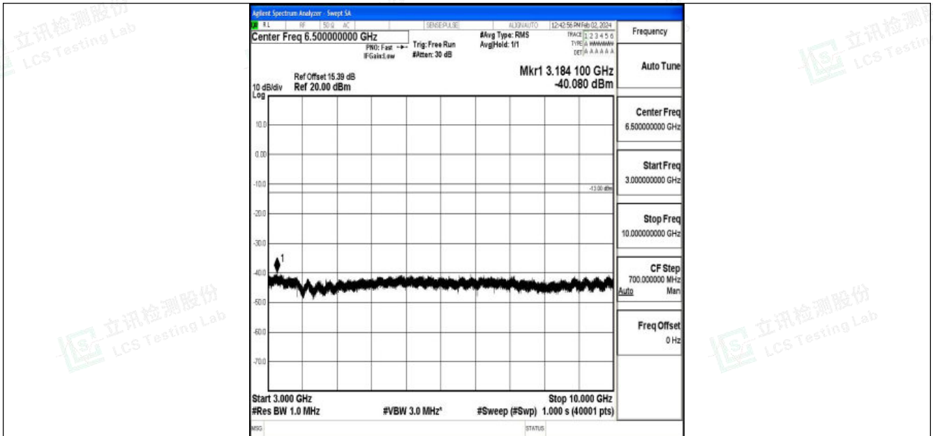
Band26_15MHz_QPSK_26965_1RB#0_3000~10000_3000~10000
