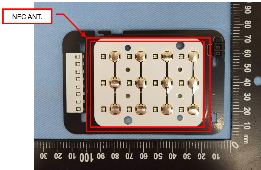
EUT Photo (22)
