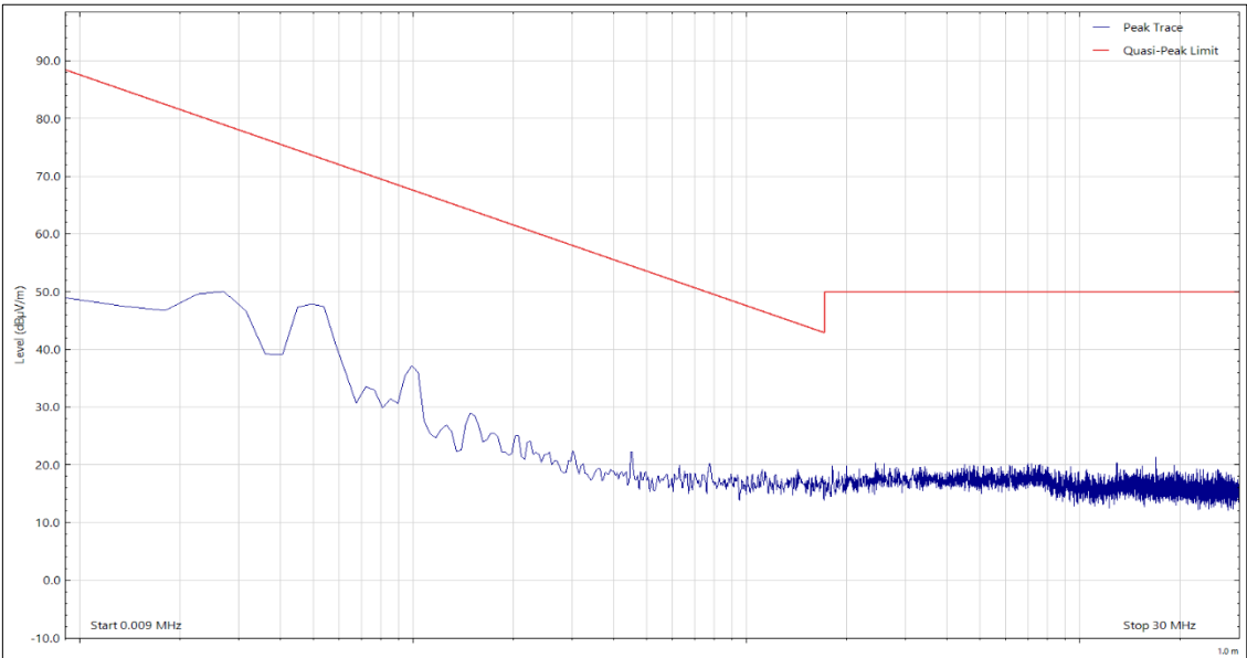
Figure 10 - Side On
