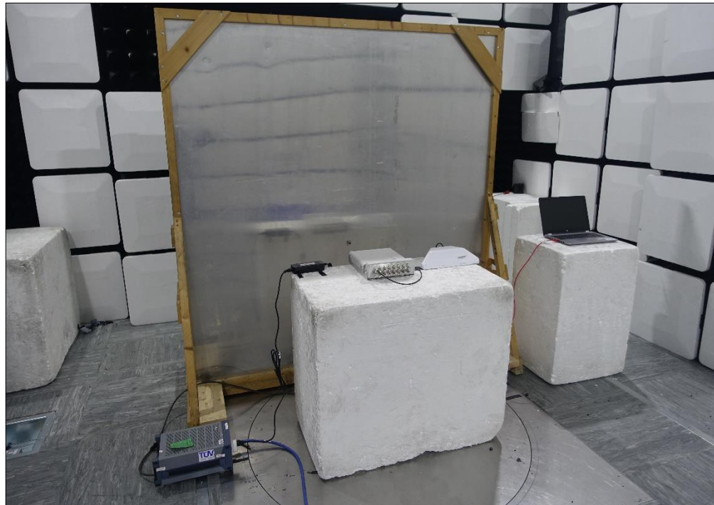
Figure 7 - Test Setup
