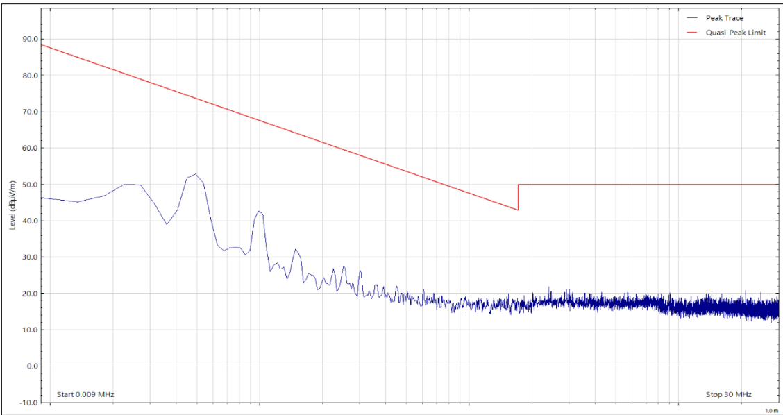
Figure 9 - Face On
