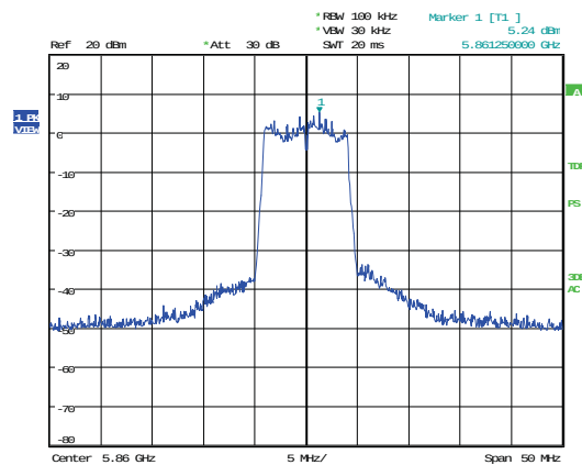
Figure 16: Conducted Spurious Emissions, Fundamental, Mode A (5860MHz) Configuration 1, RF output port 1
