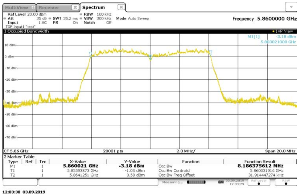
Figure 7: 99% Bandwidth, Mode A (5860MHz) Configuration 1, RF output port 2
