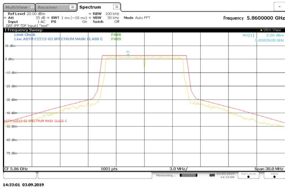
Figure 11: Transmit Spectrum Mask, Mode A (5860MHz) Configuration 2, RF output port 1
