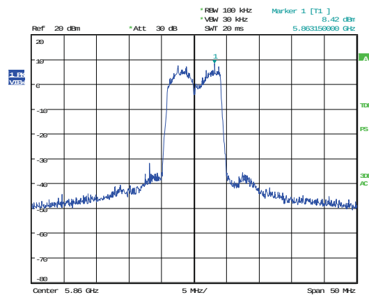
Figure 21: Conducted Spurious Emissions, Fundamental, Mode A (5860MHz) Configuration 1, RF output port 2
