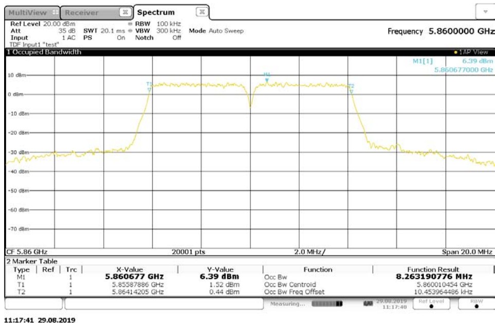
Figure 8: 99% Bandwidth, Mode A (5860MHz) Configuration 2, RF output port 1
