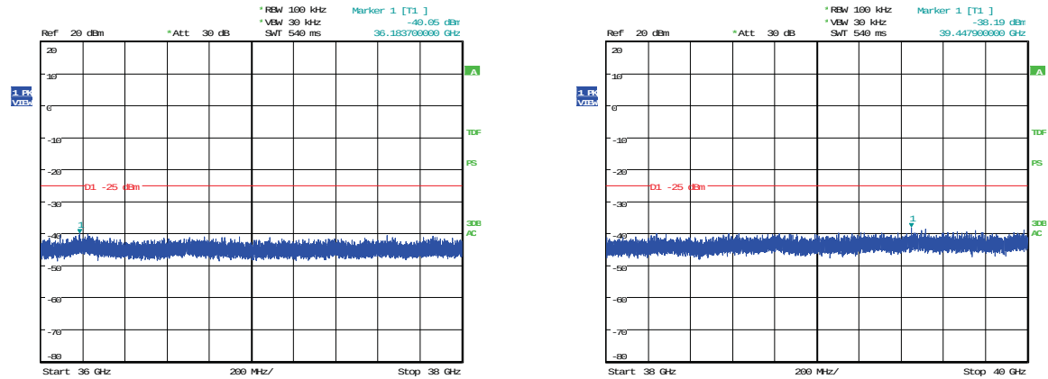
Figure 20: Conducted Spurious Emissions, 36 - 40GHz, Mode A (5860MHz) Configuration 1, RF output port 2
