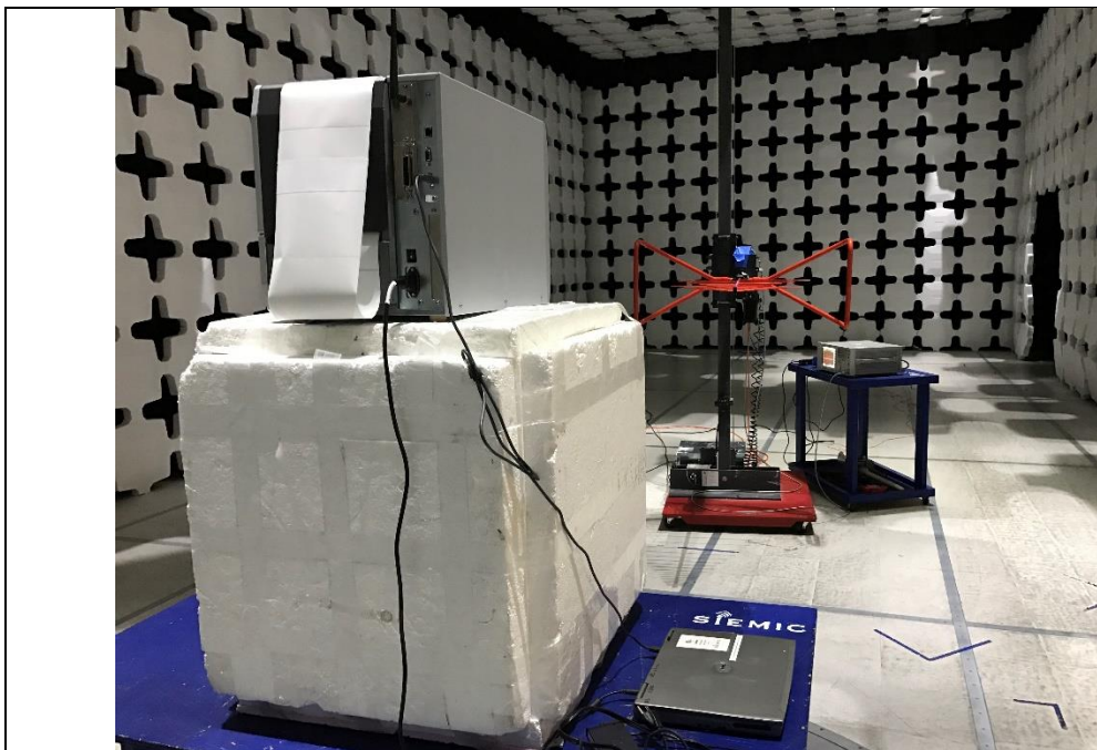
Radiated Emissions (<1GHz) – Front View
