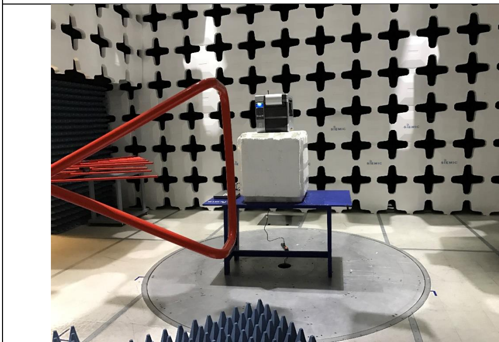
Radiated Emissions (<1GHz) – Rear View
