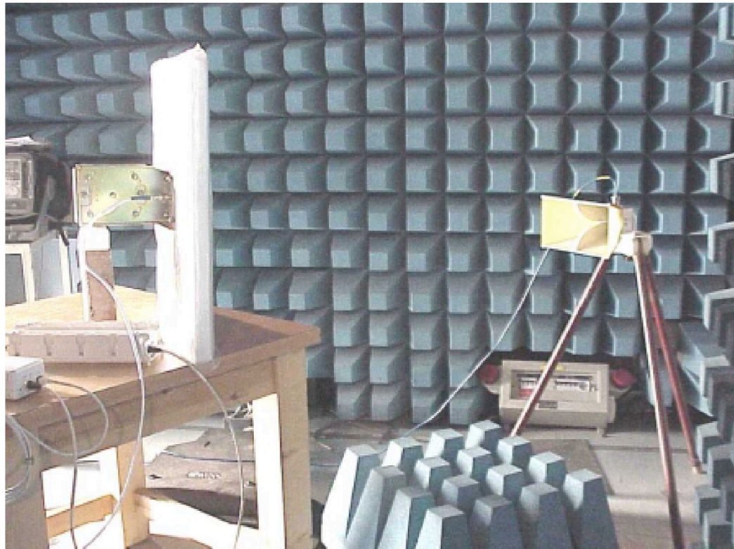
Photo #8. Radio unit with Unidirectional antenna UNI-28-4 P/N 858109 Spurious emission test
