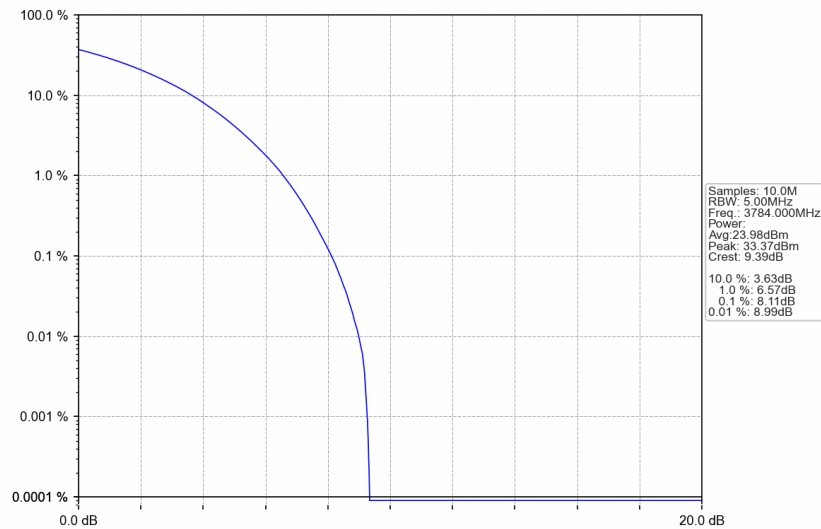
3780MHz-3980MHz_3784MHz_AWGN_SISO_Ant1_NTNV_AGC+3
