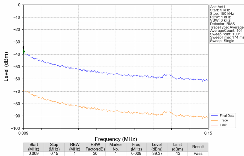
3780MHz-3980MHz_3977.5MHz_AWGN_SISO_Ant1_NTNV
