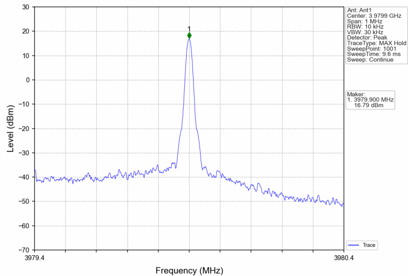
3780MHz-3980MHz_3979.9MHz_CW_SISO_Ant1_NTNV
