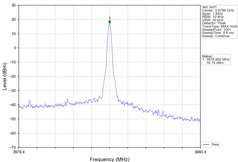
3780MHz-3980MHz_3979.9MHz_CW_SISO_Ant1_NTNV
