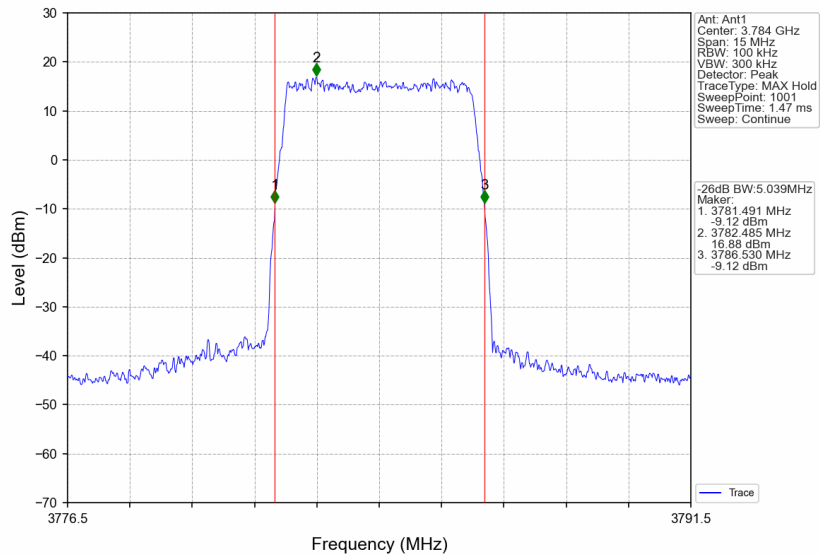
3780MHz-3980MHz_3784MHz_AWGN_SISO_Ant1_NTNV_AGC
