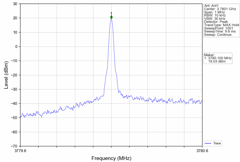
3780MHz-3980MHz_3780.1MHz_CW_SISO_Ant1_NTNV
