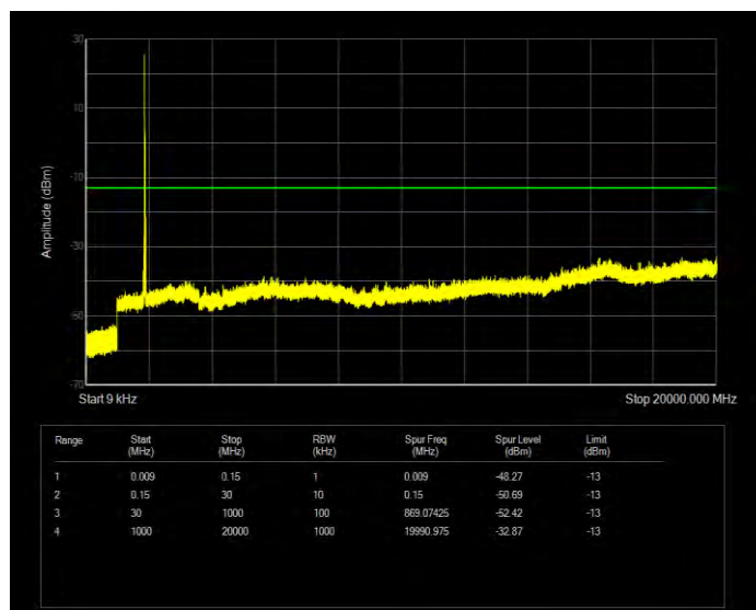
Band25 16QAM BW=20MHz Channel=26590 RB Size=1 Position=#0
