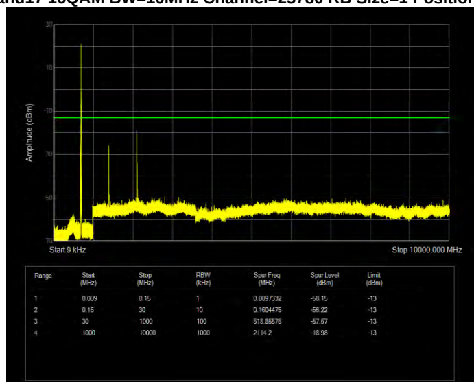
Band17 16QAM BW=10MHz Channel=23790 RB Size=1 Position=#0
