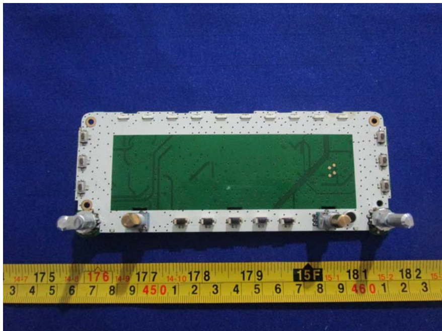
EUT – Control Panel Mainboard Top View
