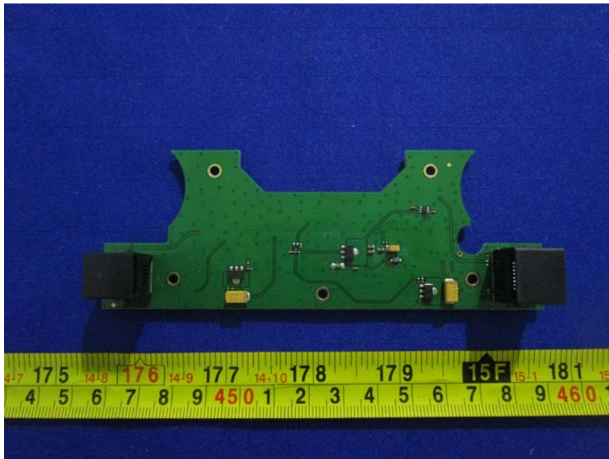
EUT –Control Panel Subboard Bottom View
