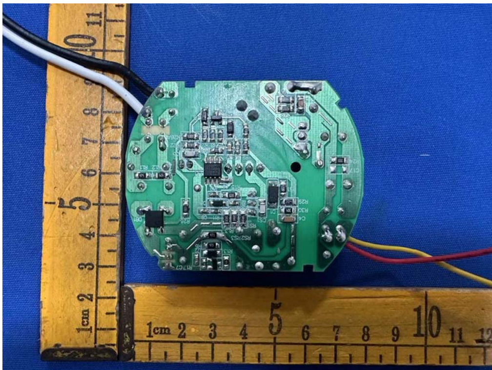
Fig.8(Model: FM-SB )
