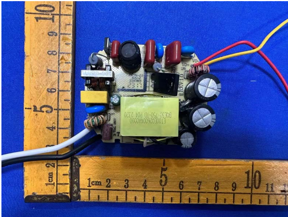
Fig.7(Model: FM-SB )
