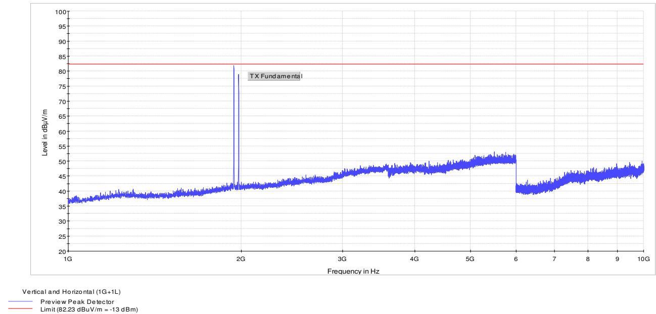
Figure 8.1-2: 1 to 10 GHz – 1G + 1L
