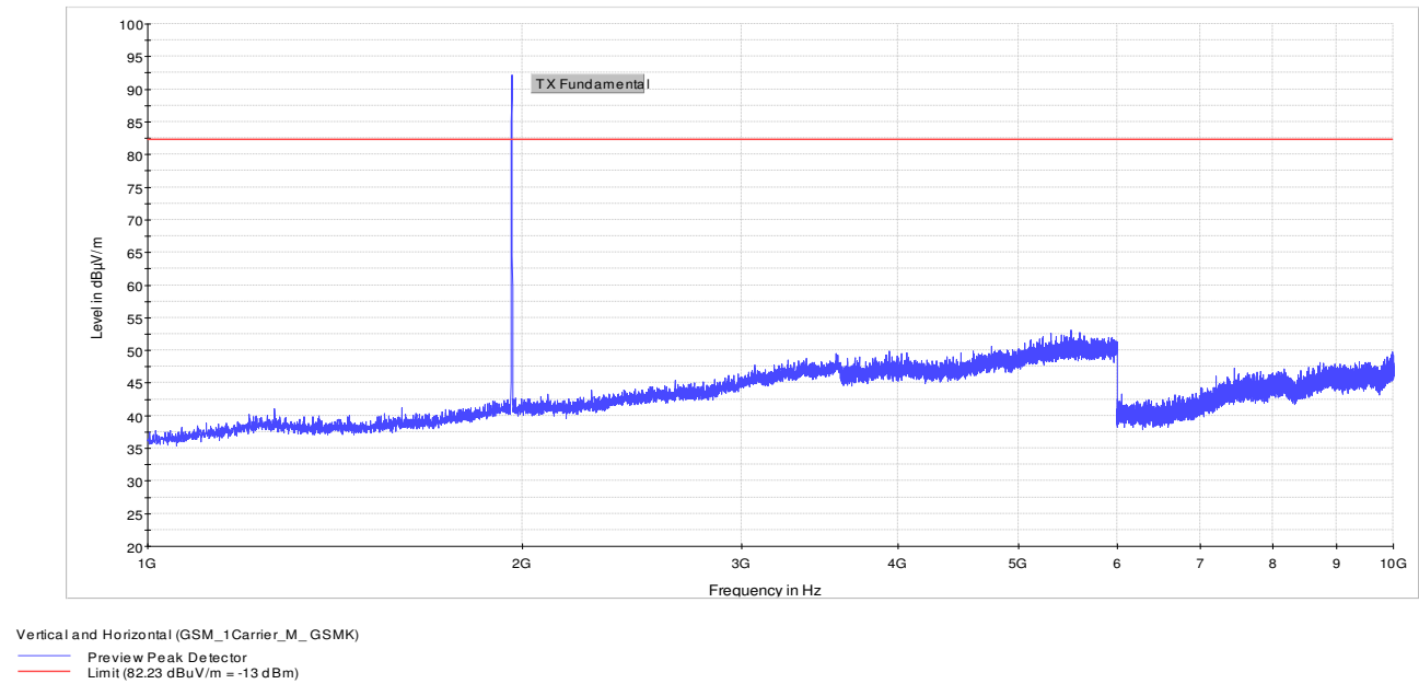
Figure 8.1-14: 1 to 10 GHz – GSM_1Carrier_M_GSMK
