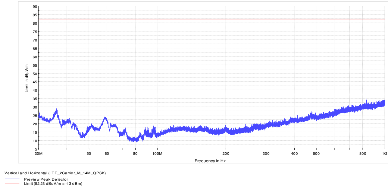
Figure 8.1-29: 30 to 1000 MHz – LTE_2Carrier_M_14M_QPSK
