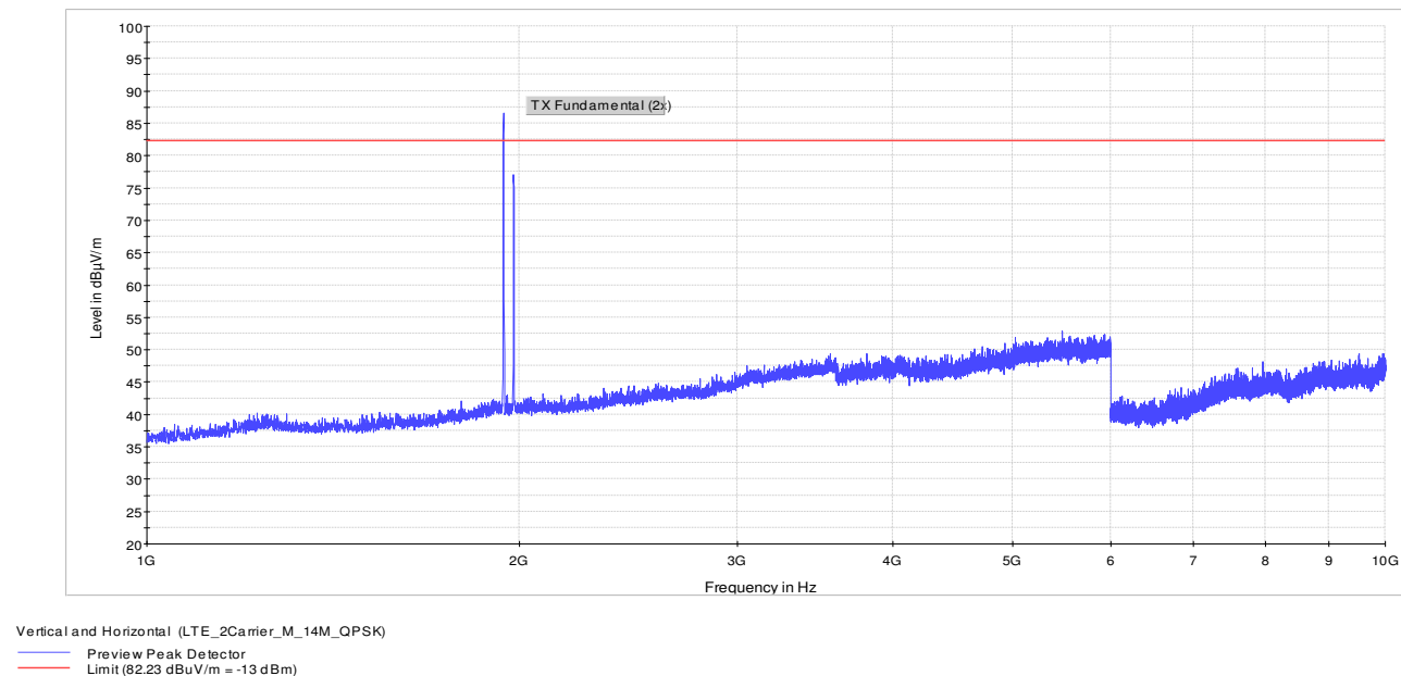
Figure 8.1-30: 1 to 10 GHz – LTE_2Carrier_M_14M_QPSK
