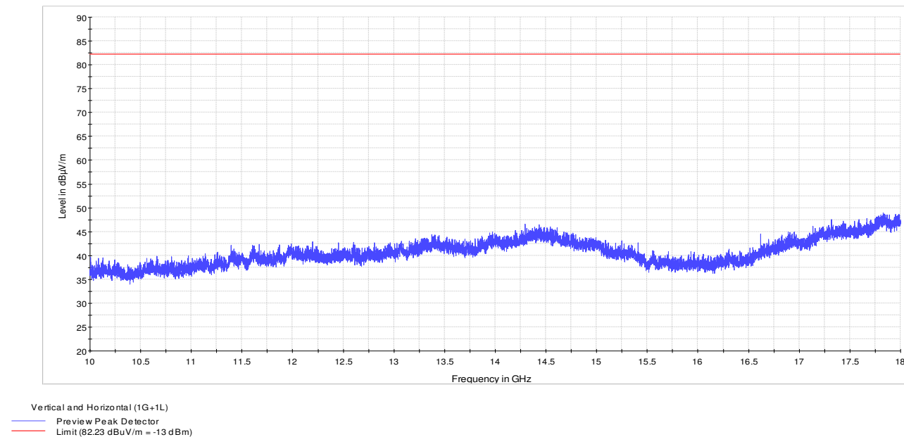
Figure 8.1-3: 10 to 18 GHz – 1G + 1L
