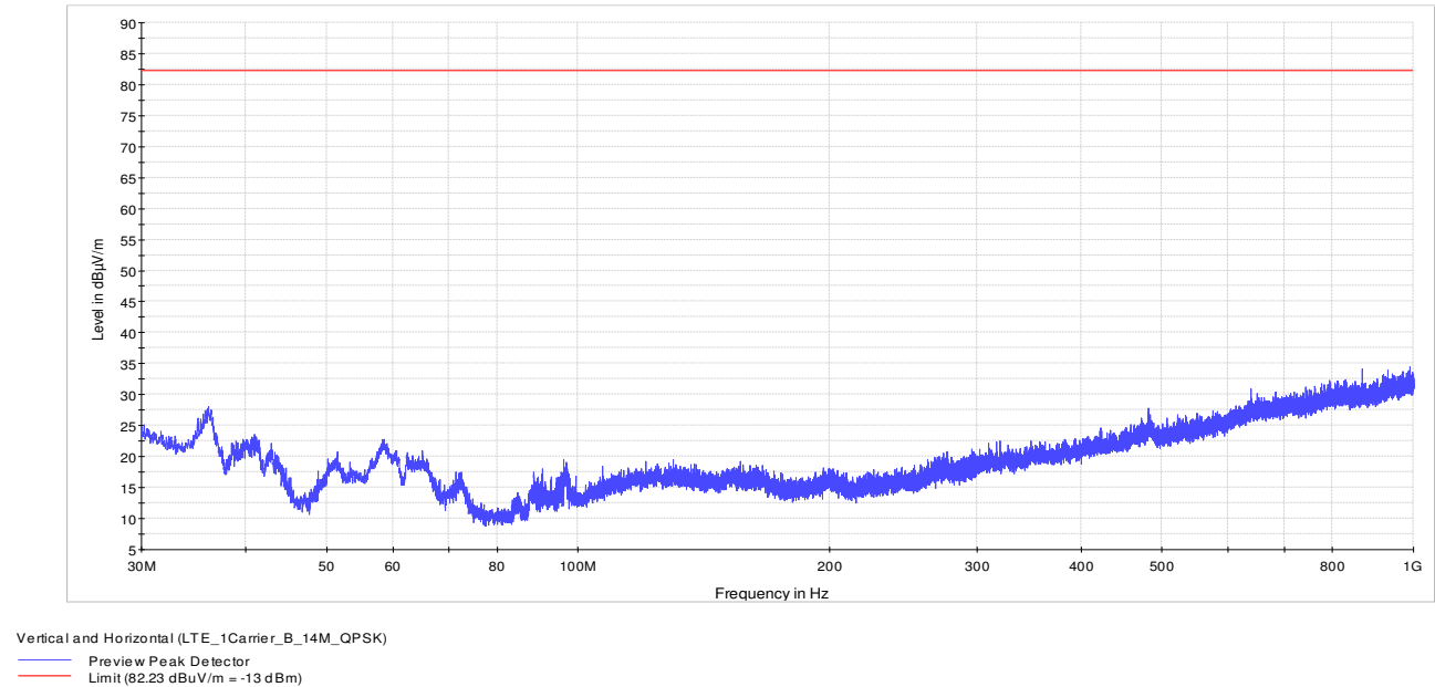
Figure 8.1-17: 30 to 1000 MHz – LTE_1Carrier_B_14M_QPSK
