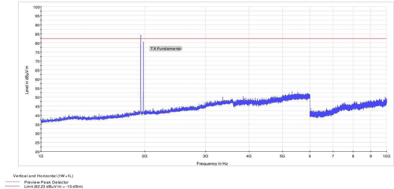
Figure 8.1-10: 1 to 10 GHz – 1W + 1L
