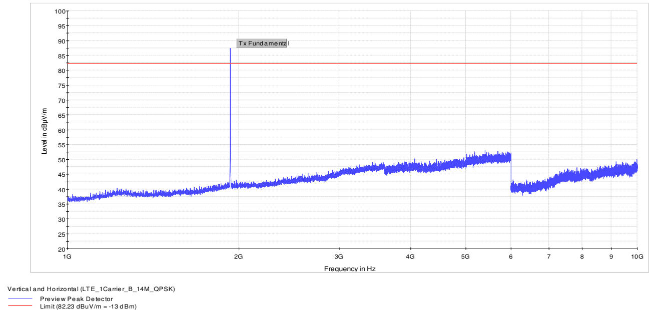
Figure 8.1-18: 1 to 10 GHz – LTE_1Carrier_B_14M_QPSK
