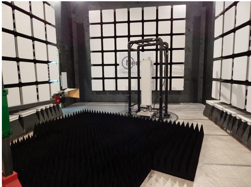
Figure 8.1-39: Setup photo – above 1 GHz
