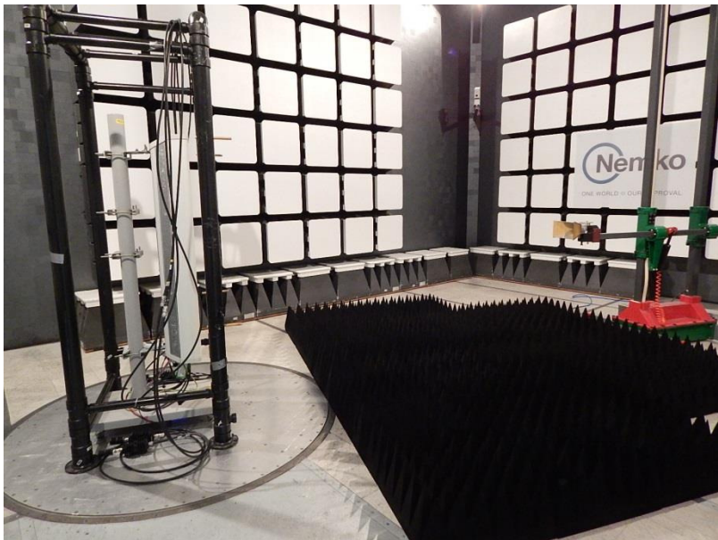
Figure 8.1-40: Setup photo – above 1 GHz
