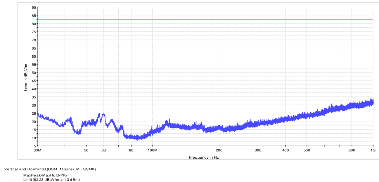
Figure 8.1-13: 30 to 1000 MHz – GSM_1Carrier_M_GSMK
