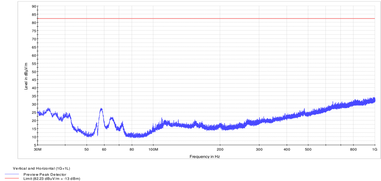
Figure 8.1-1: 30 to 1000 MHz – 1G + 1L
