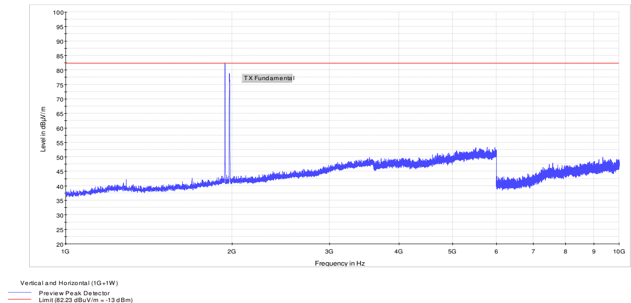
Figure 8.1-6: 1 to 10 GHz – 1G + 1W
