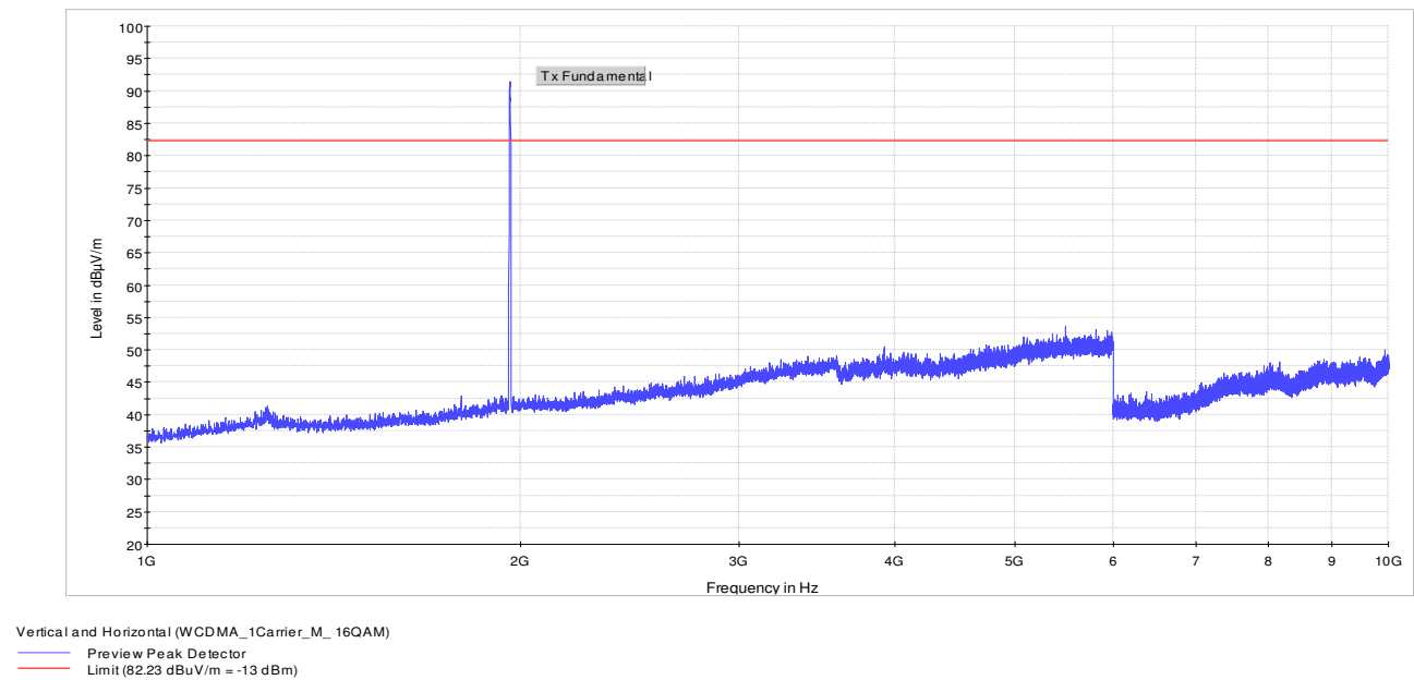
Figure 8.1-34: 1 to 10 GHz – WCDMA_1Carrier_M_16QAM
