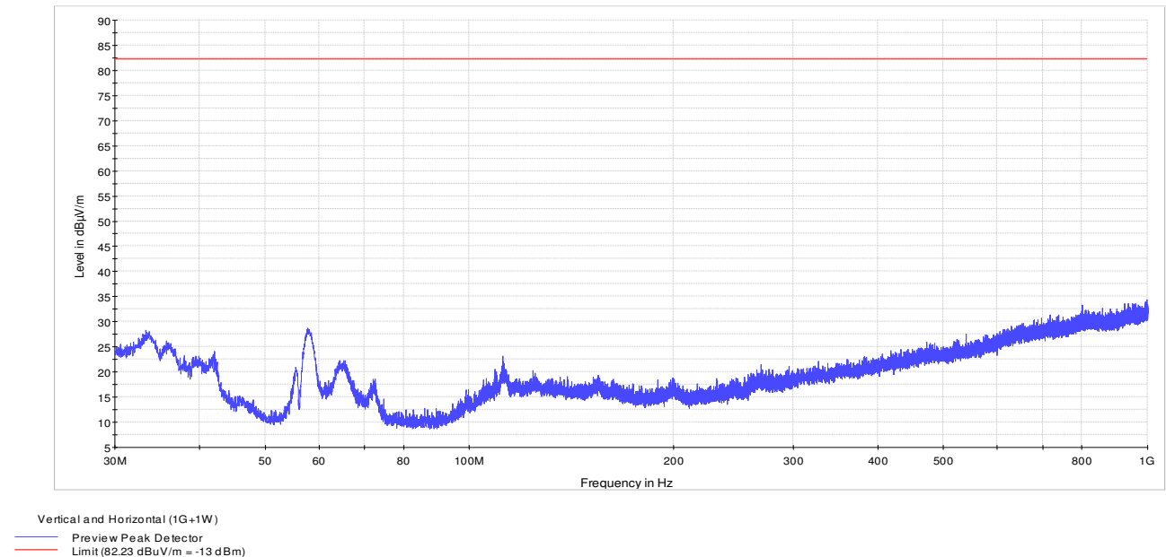
Figure 8.1-5: 30 to 1000 MHz – 1G + 1W
