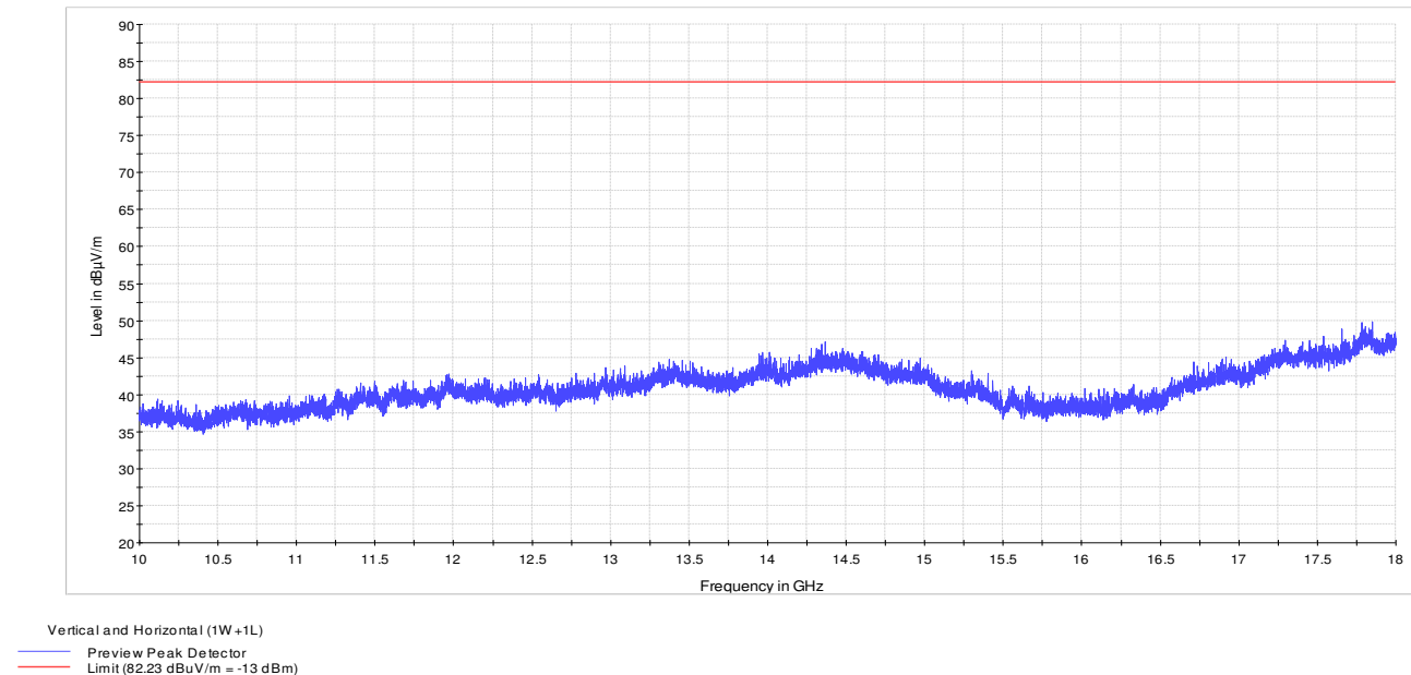
Figure 8.1-11: 10 to 18 GHz – 1W + 1L
