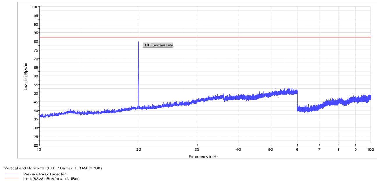
Figure 8.1-26: 1 to 10 GHz – LTE_1Carrier_T_14M_QPSK
