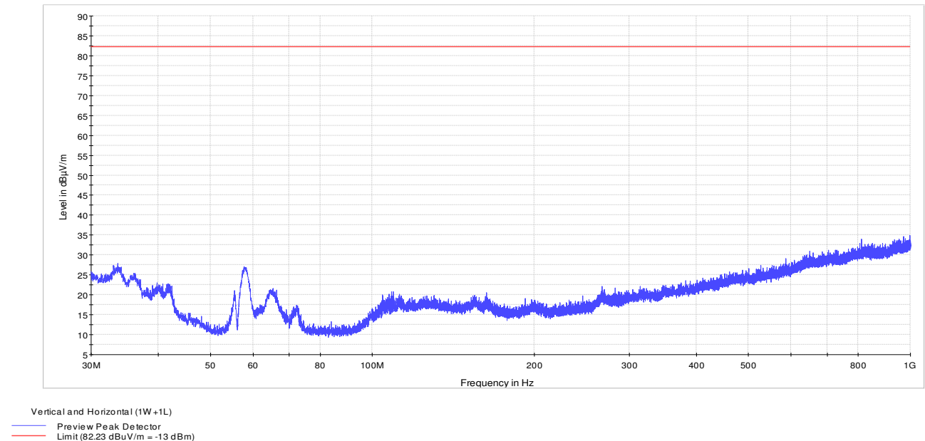
Figure 8.1-9: 30 to 1000 MHz – 1W + 1L
