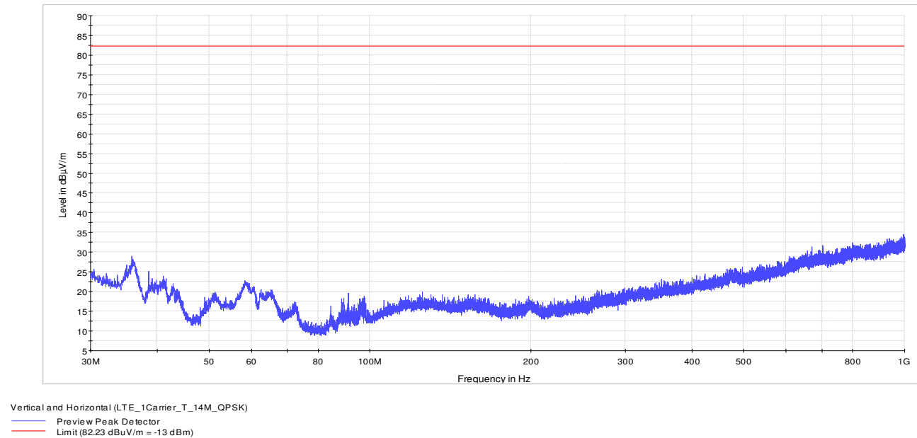
Figure 8.1-25: 30 to 1000 MHz – LTE_1Carrier_T_14M_QPSK
