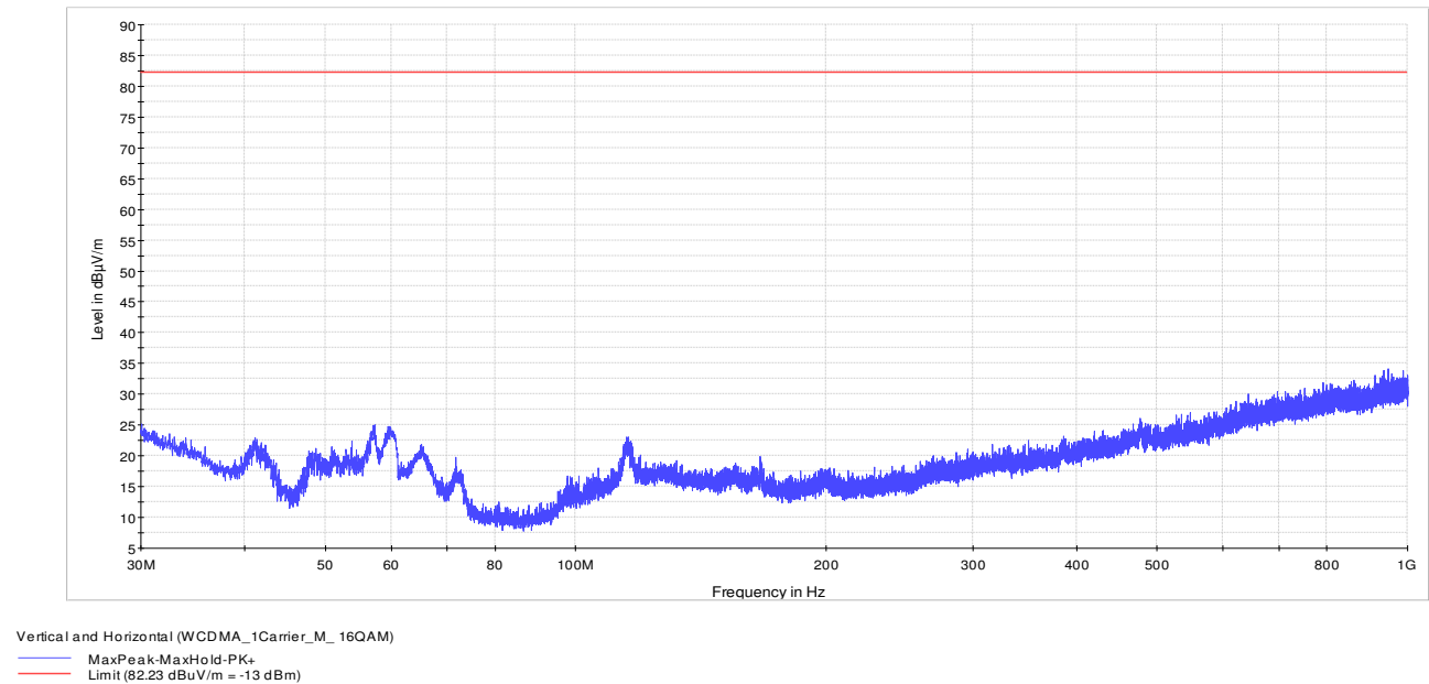
Figure 8.1-33: 30 to 1000 MHz – WCDMA_1Carrier_M_16QAM
