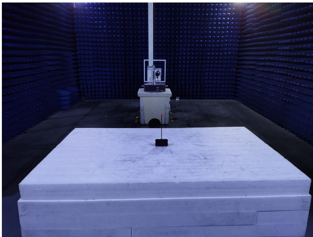
Photo of Radiated Emission Measurement (Below 30MHz)
