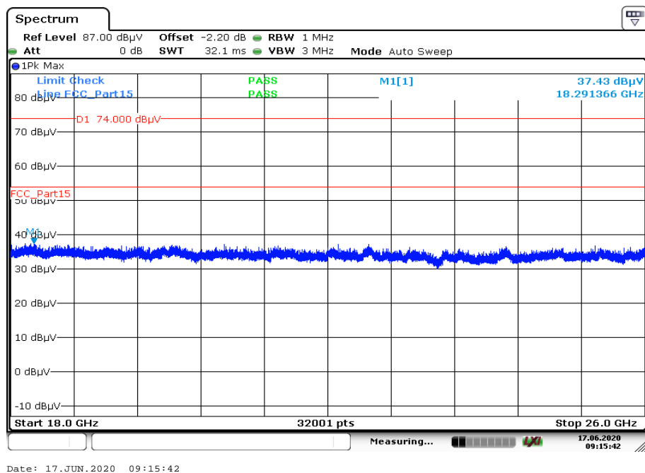
Plot 2: 18 GHz to 26 GHz, RX / idle – mode, vertical & horizontal polarization, 1 Msps
