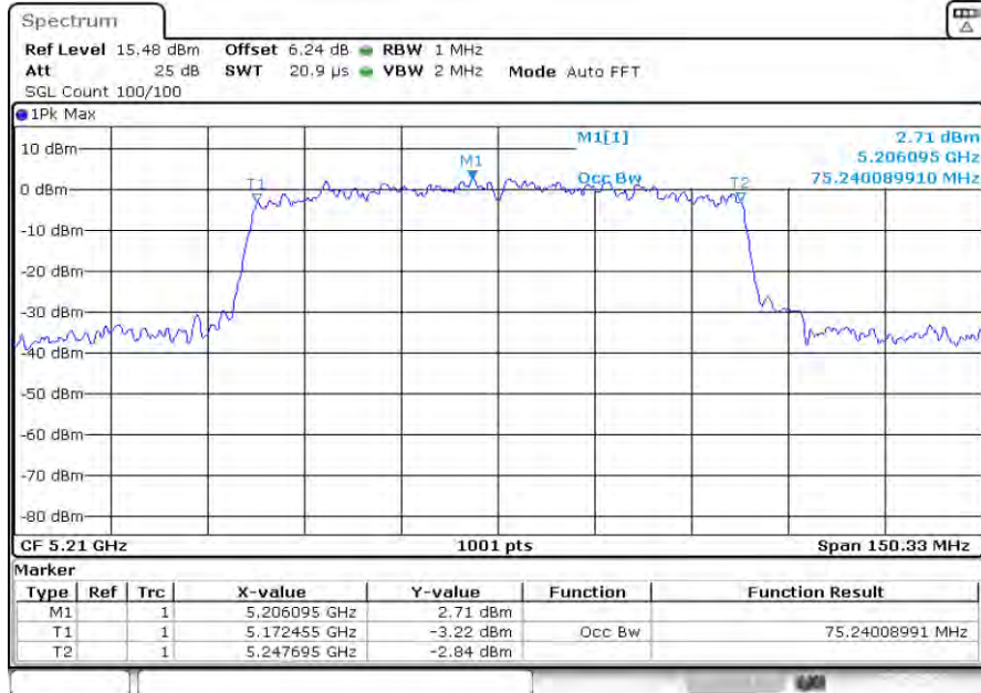
99%_OCB_NVNT_ANT1_802_11ax(HE80)_5210
