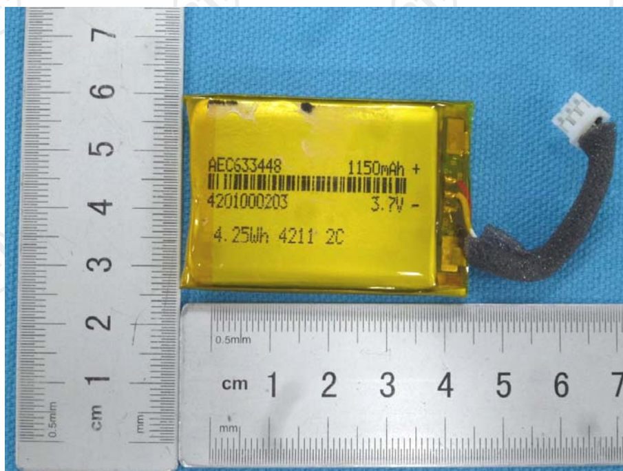
Fig.6- Battery View
