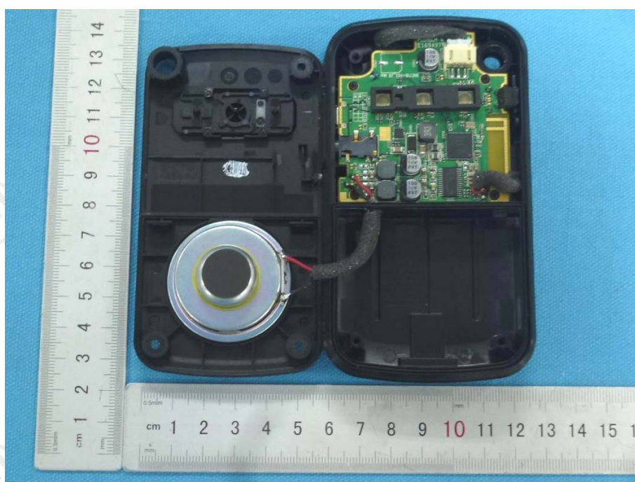
Fig.2- Inner View
