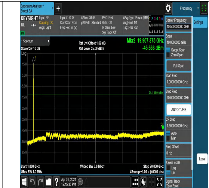
Band2-9262-3-1000~20000MHz-PASS
