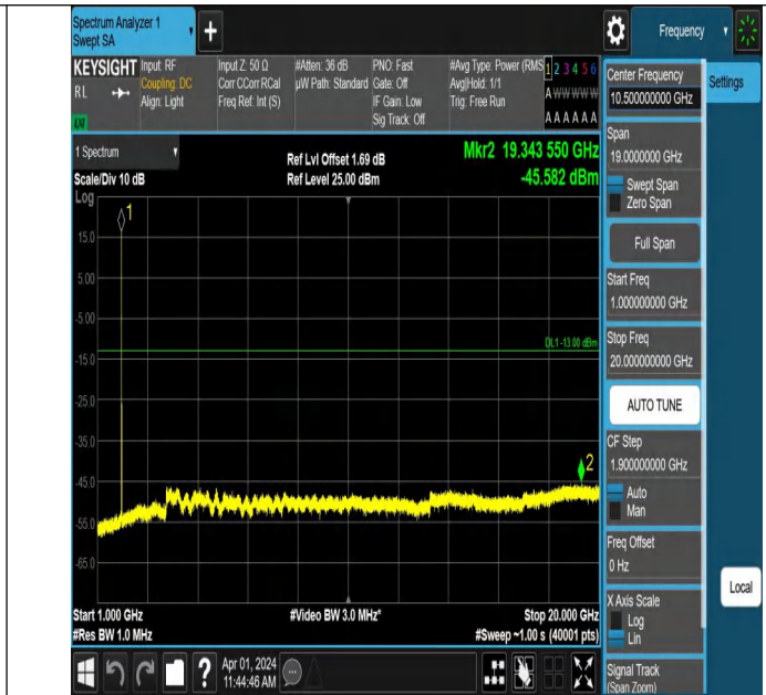
Band2-9538-2-1000~20000MHz-PASS
