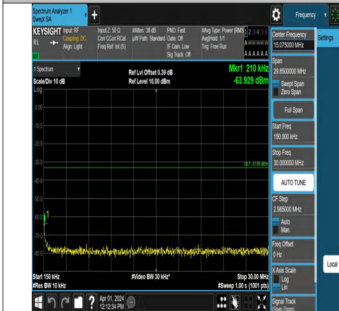
Band2-9262-2-0.15~30MHz-PASS
