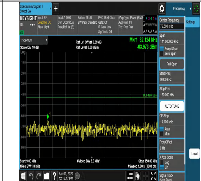
Band2-9400-4-0.009~0.15MHz-PASS
