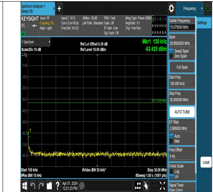
Band2-9400-5-0.15~30MHz-PASS
