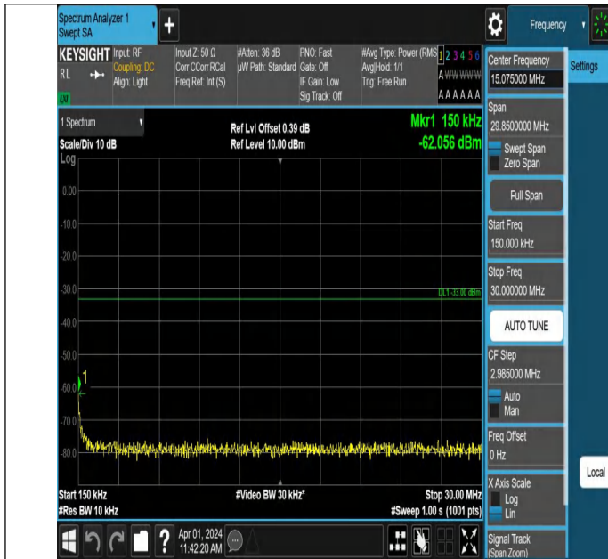
Band2-9538-1-0.15~30MHz-PASS
