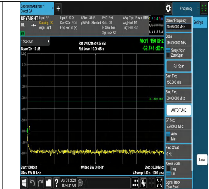
Band2-9538-2-0.15~30MHz-PASS
