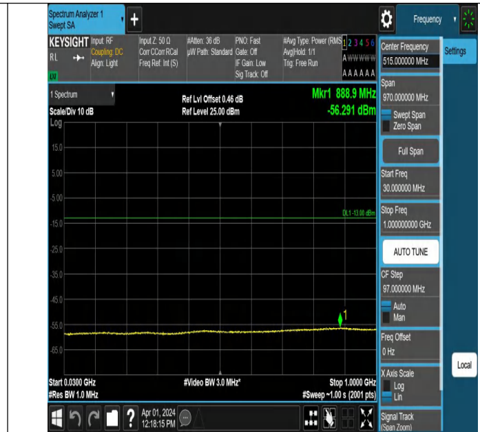
Band2-9262-4-30~1000MHz-PASS
