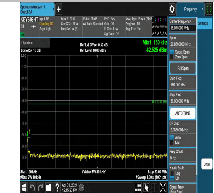
Band2-9262-3-0.15~30MHz-PASS
