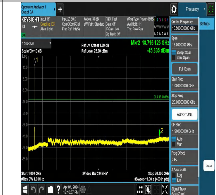
Band2-9400-1-1000~20000MHz-PASS
