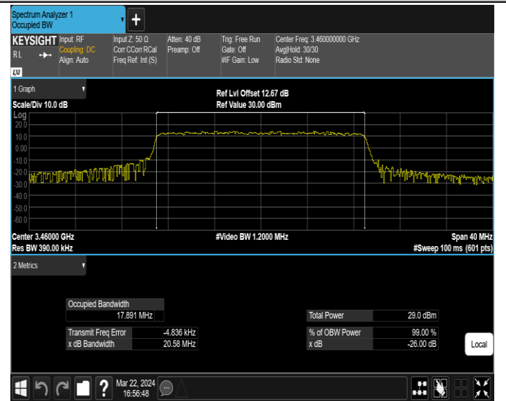
42(3450-3550)-20MHz-64QAM-42190-100RB#0-PASS
