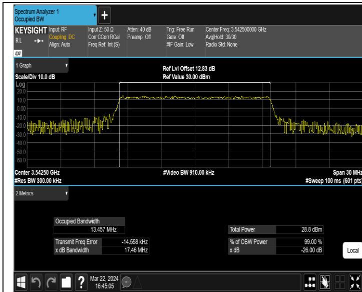
42(3450-3550)-15MHz-64QAM-43015-75RB#0-PASS
