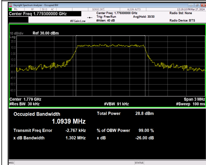
Band66-1.4MHz-64QAM-132665-6RB#0-PASS
