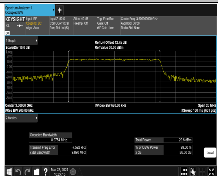
42(3450-3550)-10MHz-16QAM-42590-50RB#0-PASS
