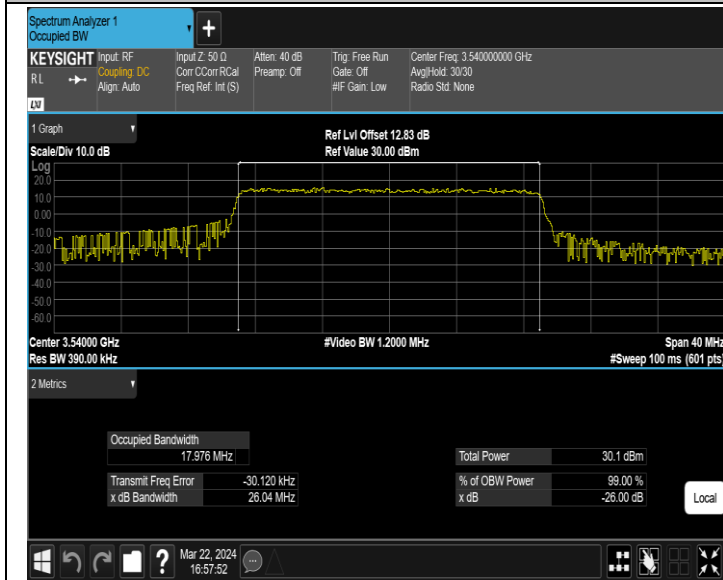
42(3450-3550)-20MHz-16QAM-42990-100RB#0-PASS
