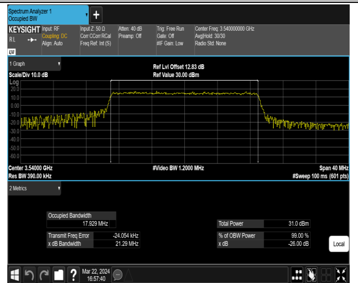
42(3450-3550)-20MHz-QPSK-42990-100RB#0-PASS
