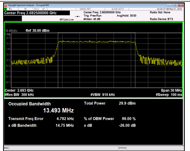
Band41-15MHz-16QAM-41515-75RB#0-PASS
