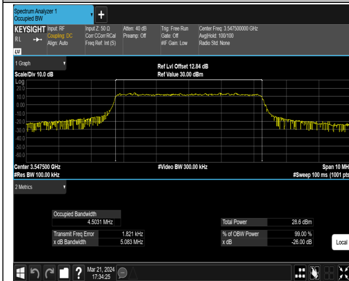
42(3450-3550)-5MHz-64QAM-43065-25RB#0-PASS
