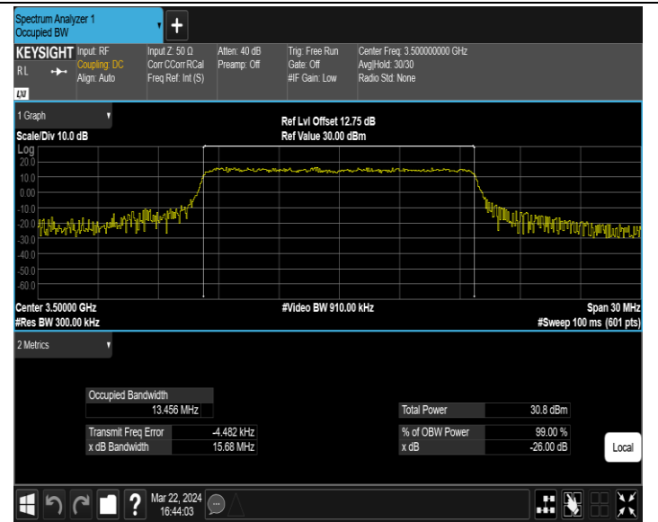
42(3450-3550)-15MHz-QPSK-42590-75RB#0-PASS
