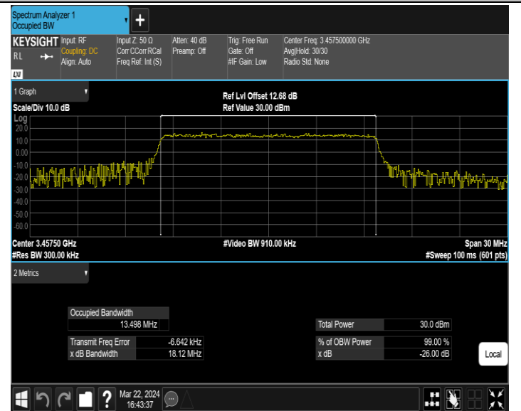
42(3450-3550)-15MHz-16QAM-42165-75RB#0-PASS
