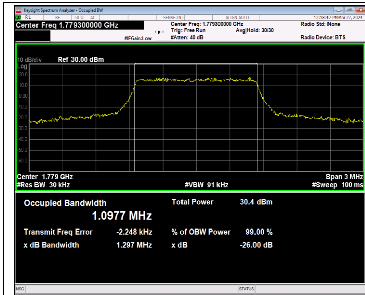
Band66-1.4MHz-QPSK-132665-6RB#0-PASS
