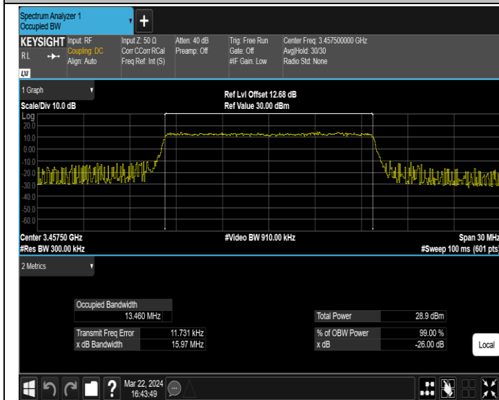
42(3450-3550)-15MHz-64QAM-42165-75RB#0-PASS
