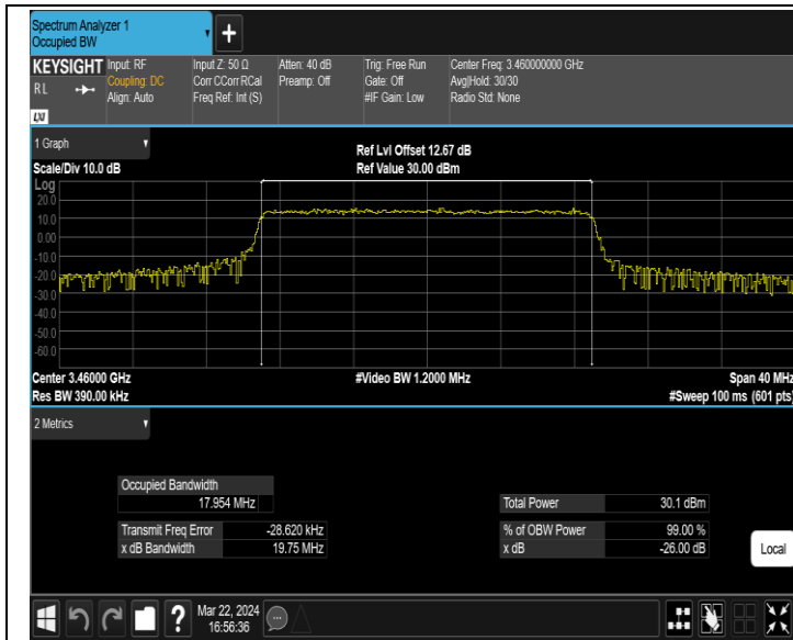
42(3450-3550)-20MHz-16QAM-42190-100RB#0-PASS
