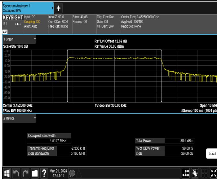
42(3450-3550)-5MHz-QPSK-42115-25RB#0-PASS
