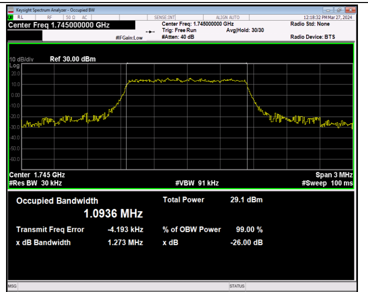
Band66-1.4MHz-64QAM-132322-6RB#0-PASS
