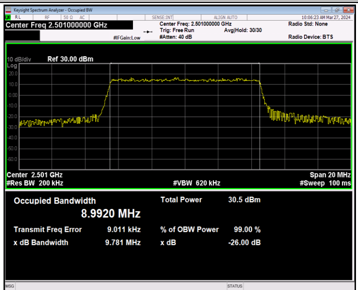
Band41-10MHz-QPSK-39700-50RB#0-PASS
