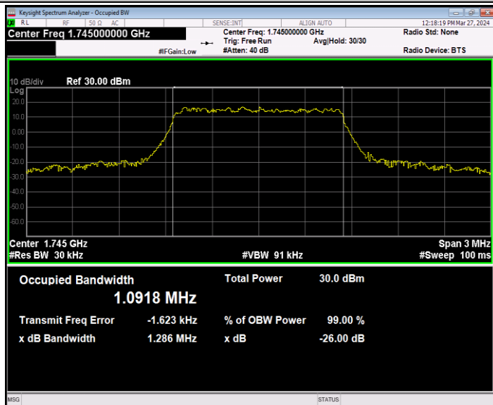
Band66-1.4MHz-16QAM-132322-6RB#0-PASS
