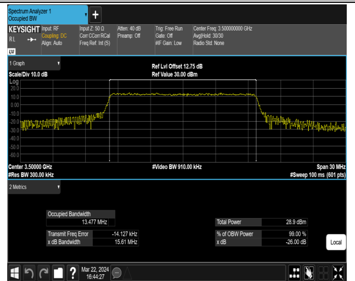
42(3450-3550)-15MHz-64QAM-42590-75RB#0-PASS
