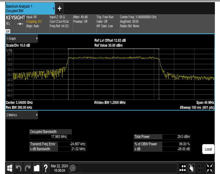
42(3450-3550)-20MHz-64QAM-42990-100RB#0-PASS
