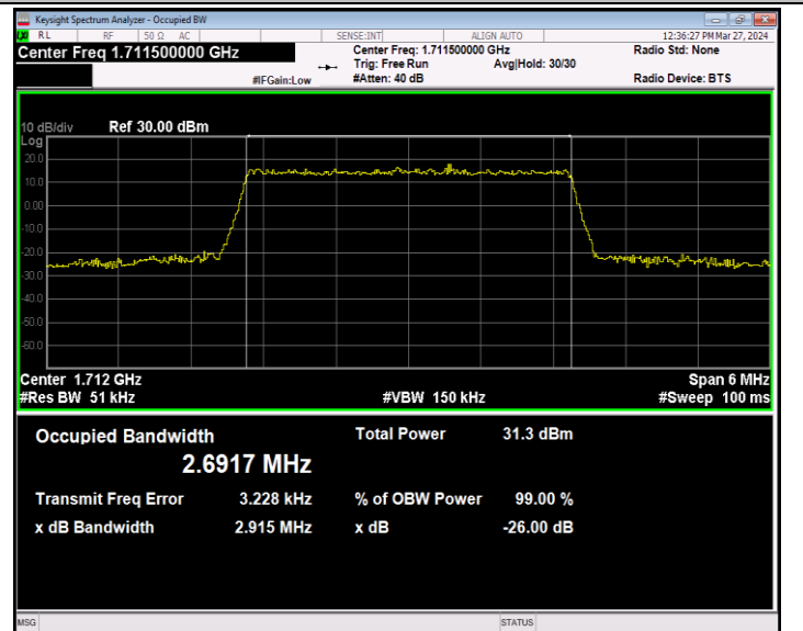
Band66-3MHz-QPSK-131987-15RB#0-PASS
