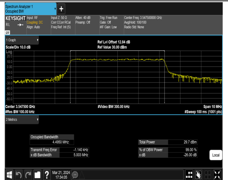
42(3450-3550)-5MHz-16QAM-43065-25RB#0-PASS
