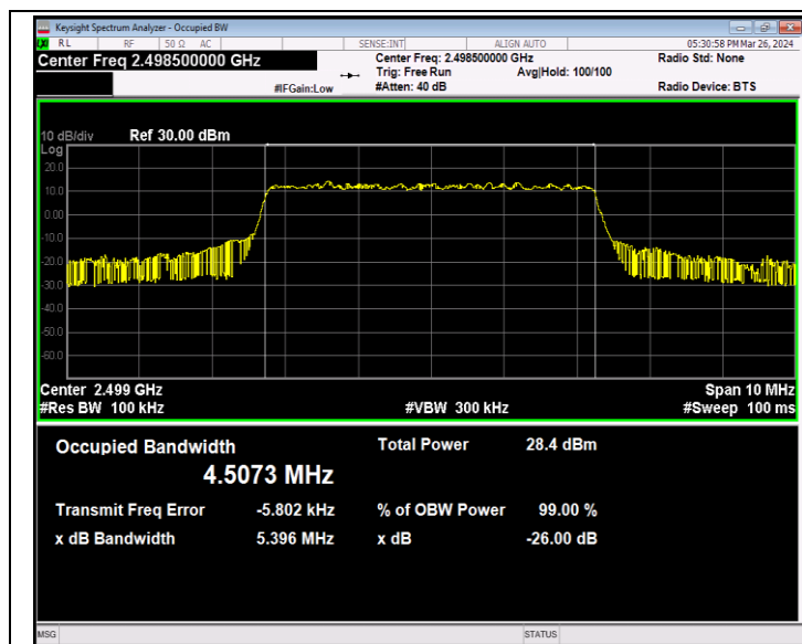
Band41-5MHz-64QAM-39675-25RB#0-PASS
