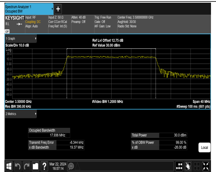
42(3450-3550)-20MHz-16QAM-42590-100RB#0-PASS
