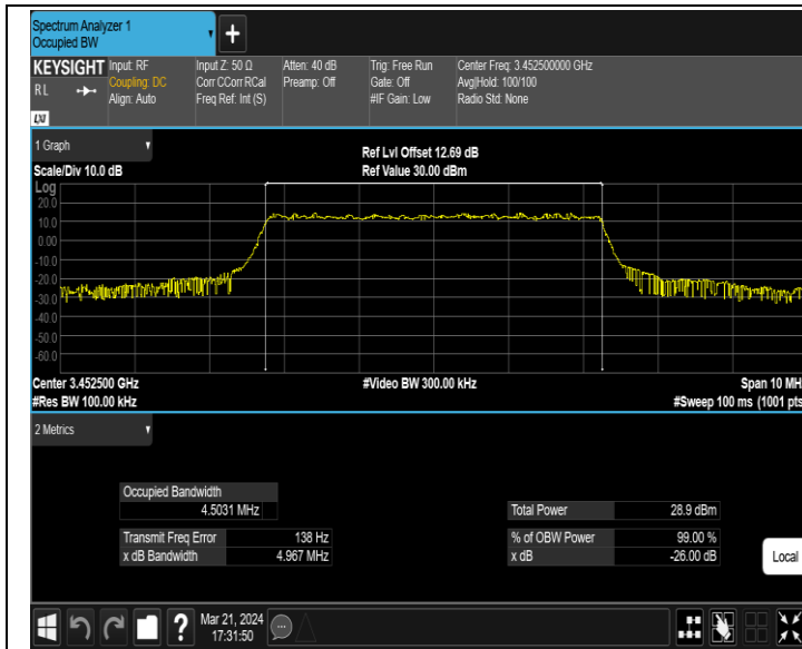
42(3450-3550)-5MHz-64QAM-42115-25RB#0-PASS
