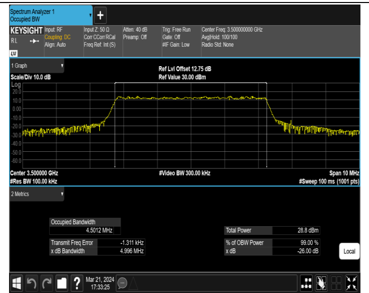
42(3450-3550)-5MHz-64QAM-42590-25RB#0-PASS
