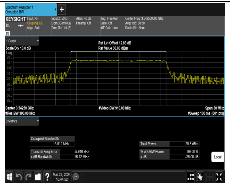
42(3450-3550)-15MHz-16QAM-43015-75RB#0-PASS
