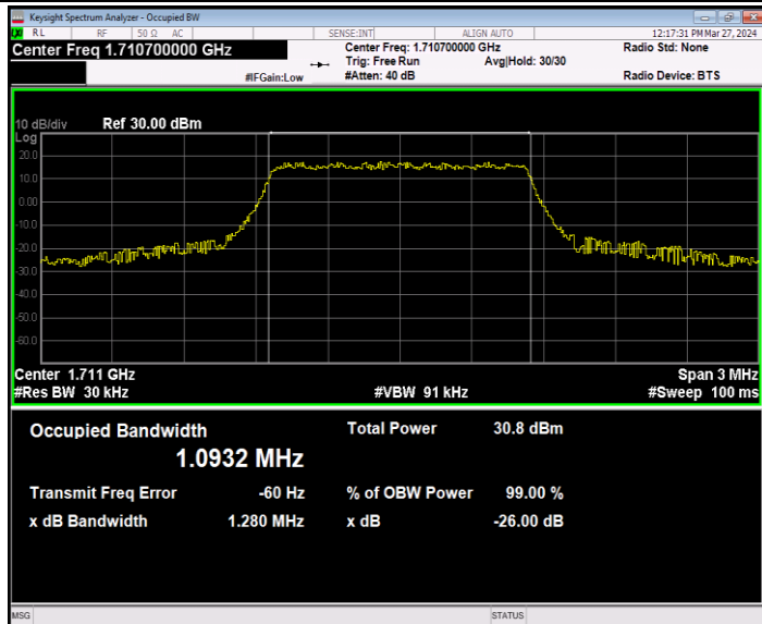
Band66-1.4MHz-QPSK-131979-6RB#0-PASS
