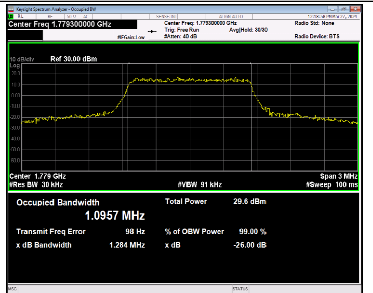
Band66-1.4MHz-16QAM-132665-6RB#0-PASS
