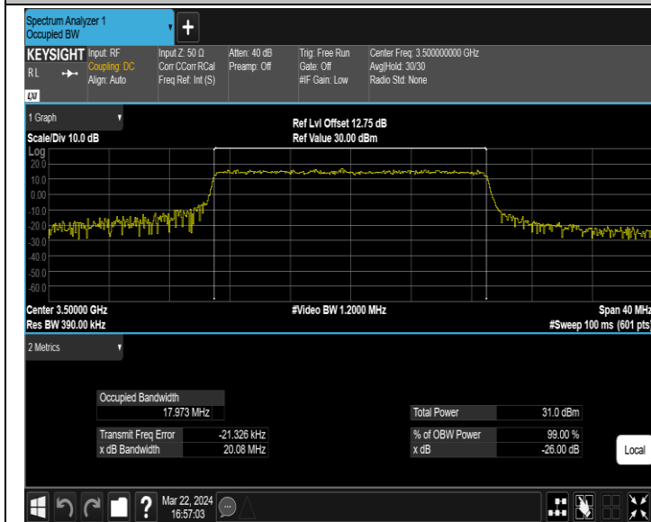
42(3450-3550)-20MHz-QPSK-42590-100RB#0-PASS
