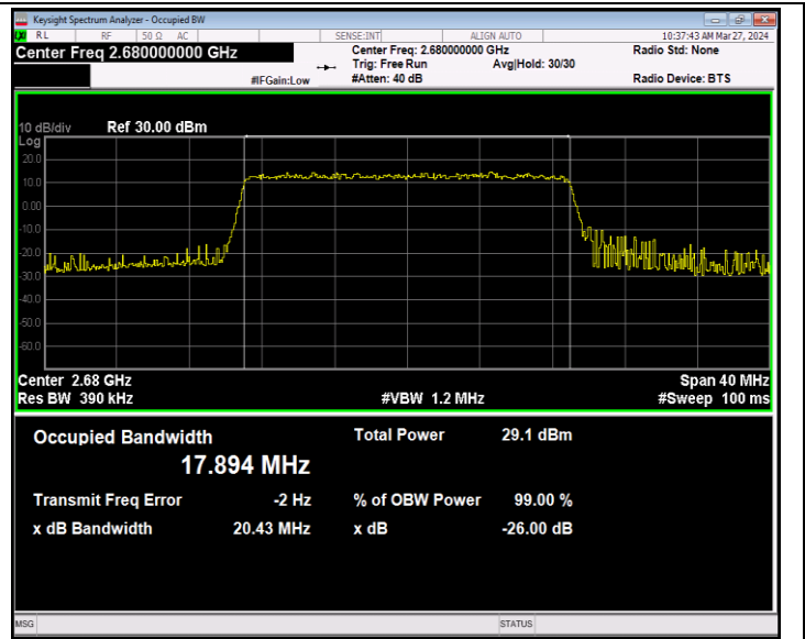
Band41-20MHz-64QAM-41490-100RB#0-PASS
