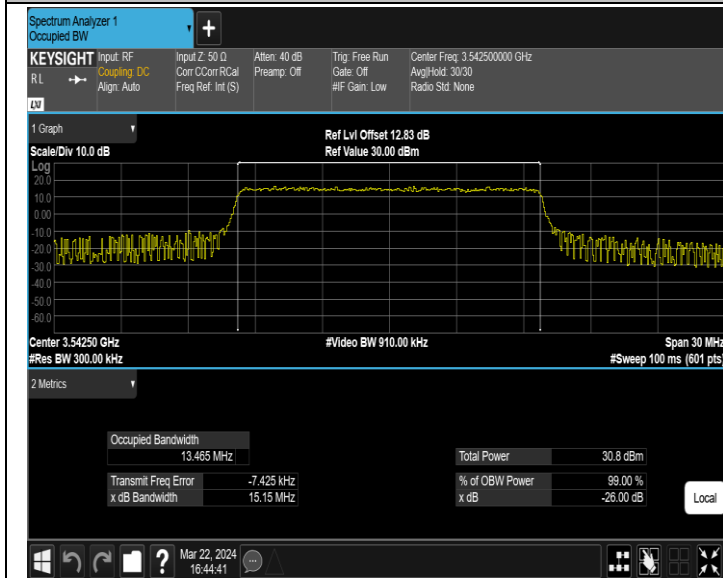
42(3450-3550)-15MHz-QPSK-43015-75RB#0-PASS
