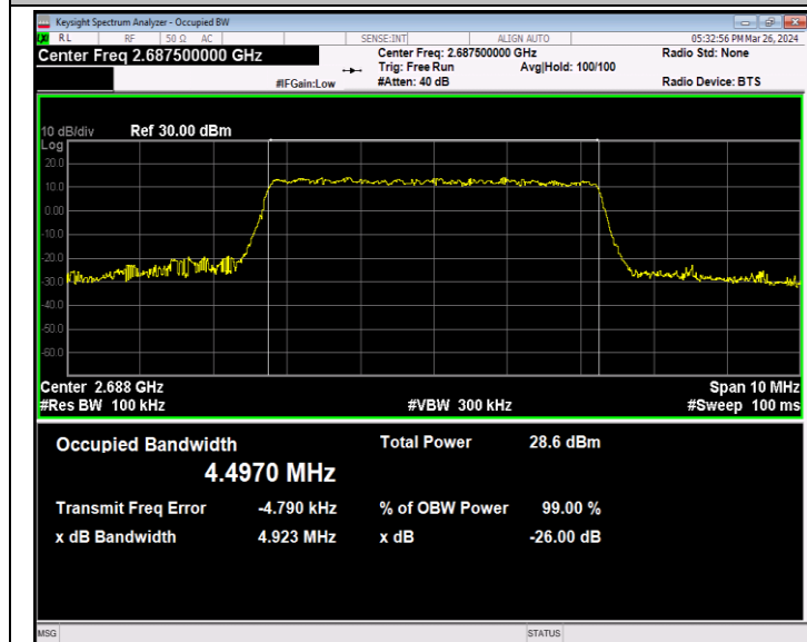
Band41-5MHz-64QAM-41565-25RB#0-PASS
