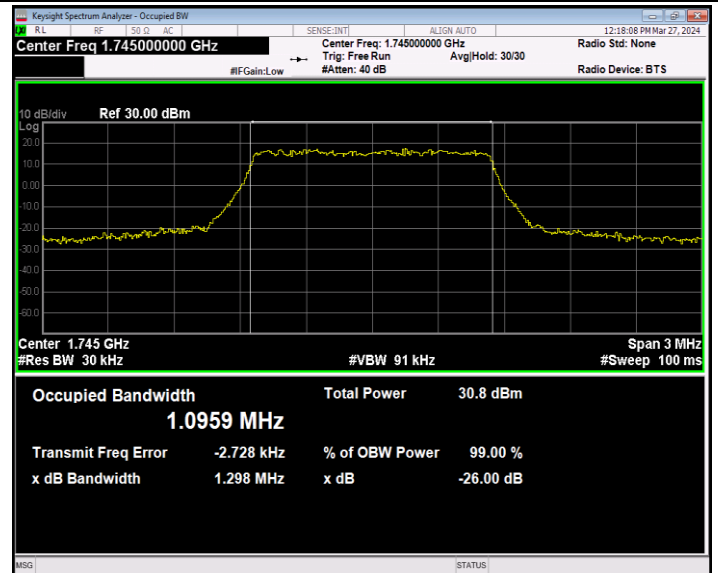
Band66-1.4MHz-QPSK-132322-6RB#0-PASS
