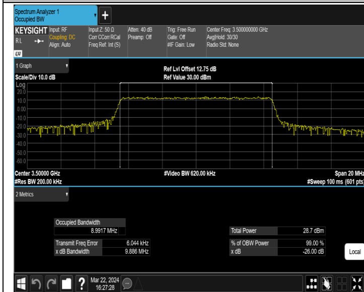
42(3450-3550)-10MHz-64QAM-42590-50RB#0-PASS
