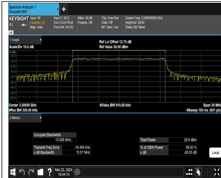
42(3450-3550)-15MHz-16QAM-42590-75RB#0-PASS
