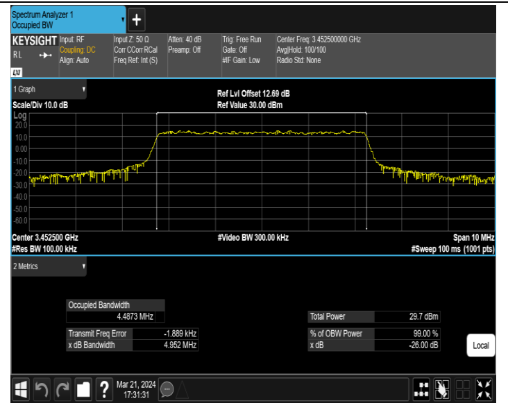
42(3450-3550)-5MHz-16QAM-42115-25RB#0-PASS
