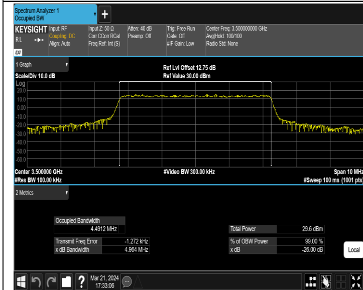
42(3450-3550)-5MHz-16QAM-42590-25RB#0-PASS
