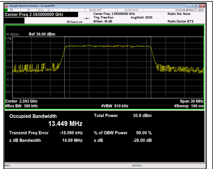
Band41-15MHz-QPSK-40620-75RB#0-PASS
