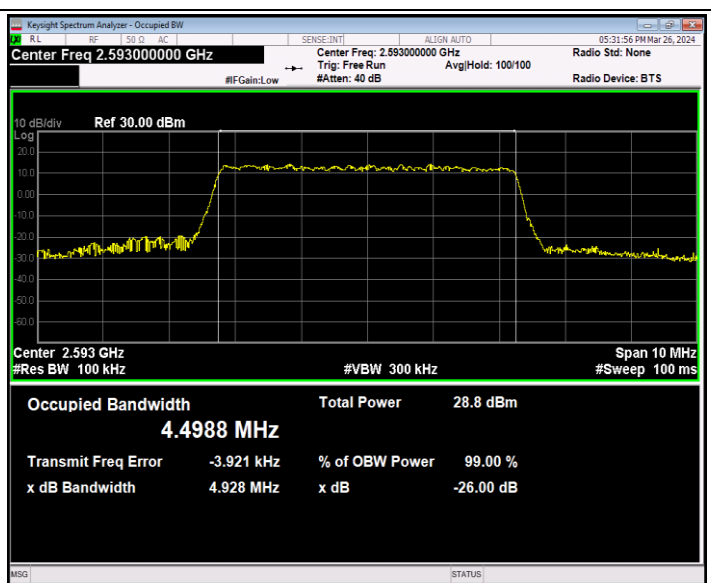
Band41-5MHz-64QAM-40620-25RB#0-PASS
