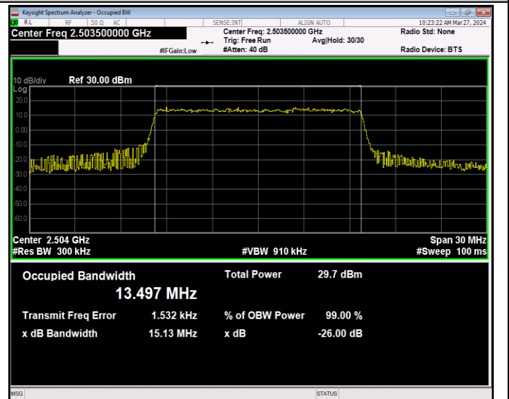
Band41-15MHz-16QAM-39725-75RB#0-PASS
