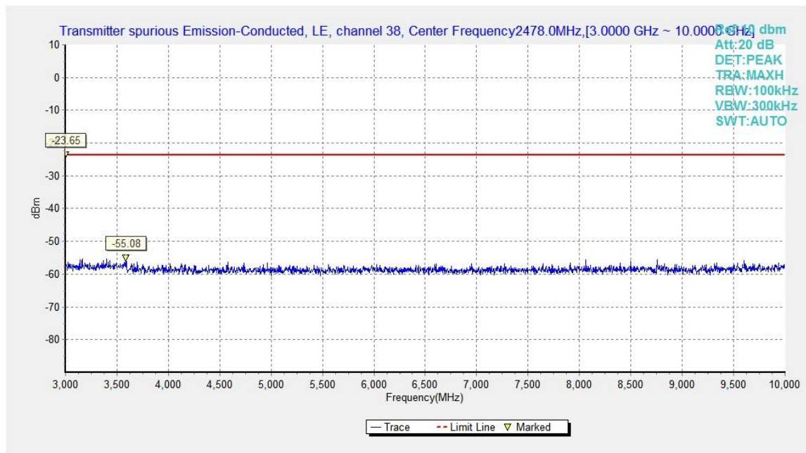
Fig.16. Transmitter Spurious Emission -Conducted:GFSK, 2478 MHz,3GHz - 10GHz
