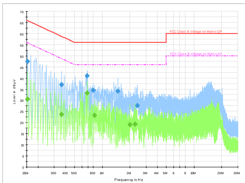
Fig.B.8.1 AC Powerline Conducted Emission-blutetooth
