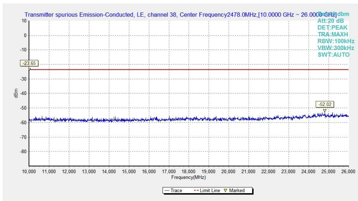
Fig.17. Transmitter Spurious Emission -Conducted: GFSK, 2478 MHz, 10GHz - 26GHz
