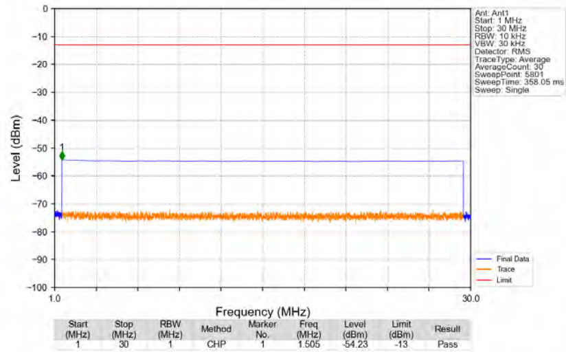
n2_15kHz_SISO_NTNV_25MHz_CP-OFDM_QPSK_1897.5MHz_Edge_1RB_Right
