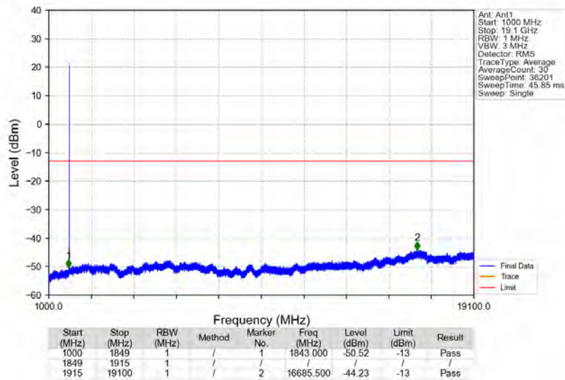
n2_15kHz_SISO_NTNV_25MHz_DFT-s-OFDM_PI/2_BPSK_1880MHz_Edge_1RB_Left
