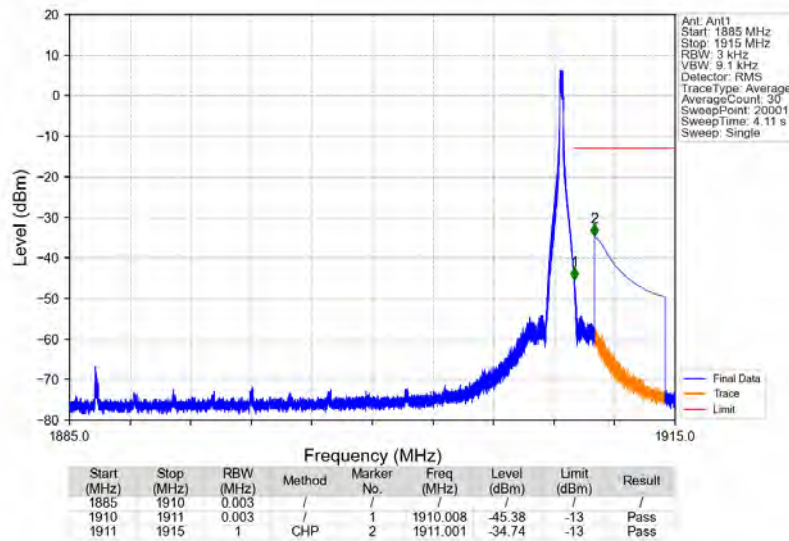
n2_15kHz_SISO_NTNV_25MHz_DFT-s-OFDM_PI/2_BPSK_1897.5MHz_Edge_1RB_Right
