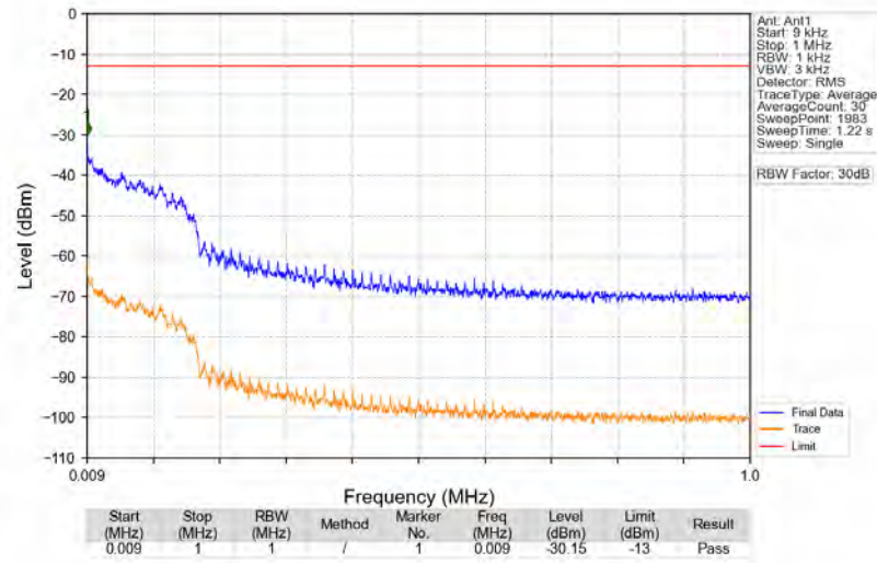
n2_15kHz_SISO_NTNV_30MHz_CP-OFDM_QPSK_1880MHz_Edge_1RB_Left
