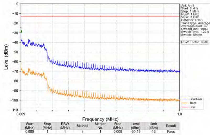
n2_15kHz_SISO_NTNV_30MHz_DFT-s-OFDM_QPSK_1880MHz_Edge_1RB_Left
