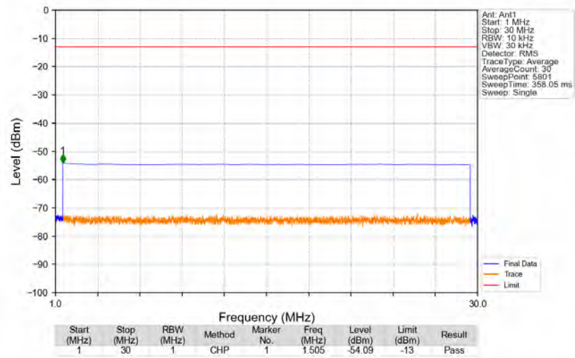
n2_15kHz_SISO_NTNV_25MHz_DFT-s-OFDM QPSK_1897.5MHz_Edge_1RB_Right
