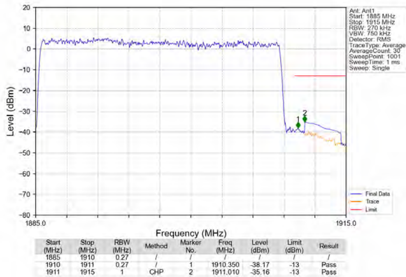
n2_15kHz_SISO_NTNV_25MHz_DFT-s-OFDM_PI/2_BPSK_1897.5MHz_Outer_Full
