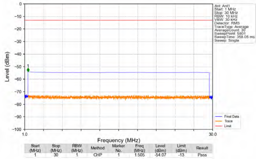
n2_15kHz_SISO_NTNV_40MHz_DFT-s-OFDM_QPSK_1890MHz_Edge_1RB_Right
