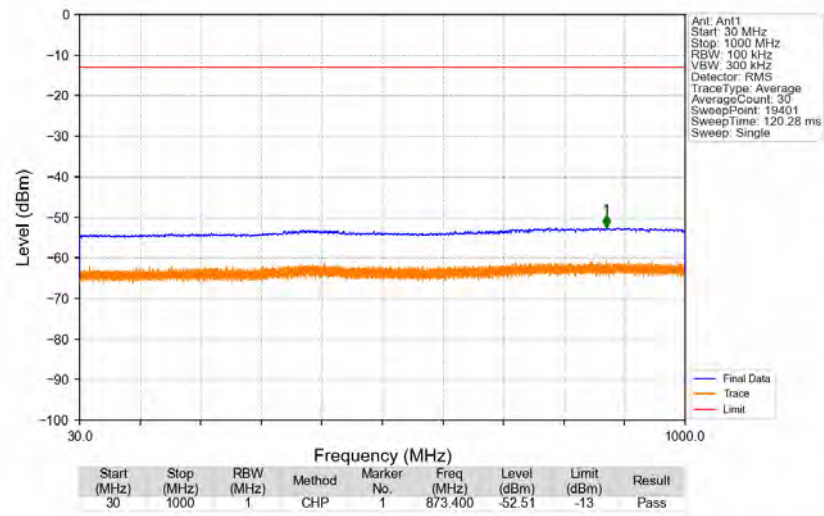
n2_15kHz_SISO_NTNV_30MHz_CP-OFDM_QPSK_1880MHz_Edge_1RB_Left
