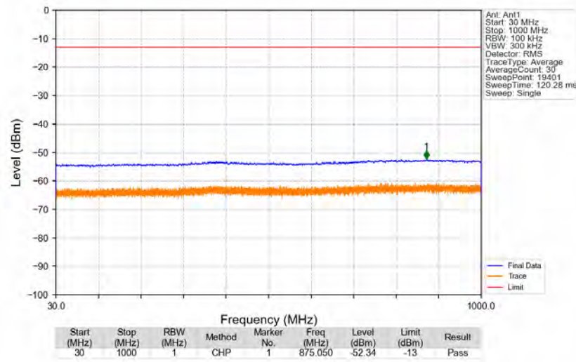
n2_15kHz_SISO_NTNV_40MHz_DFT-s-OFDM_QPSK_1880MHz_Edge_1RB_Left
