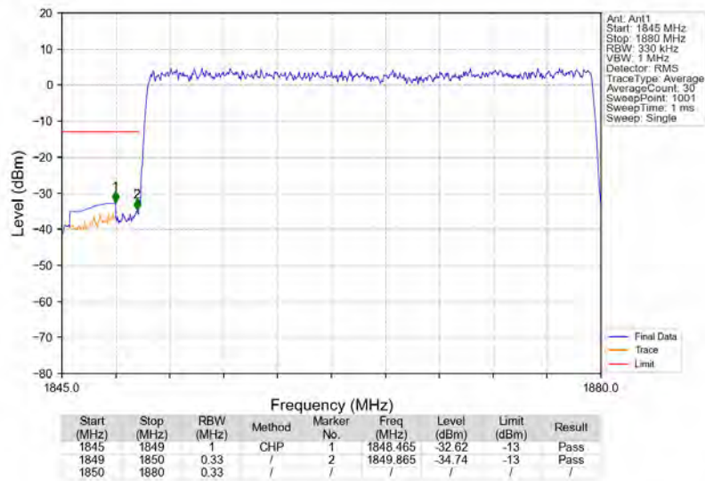
n2_15kHz_SISO_NTNV_30MHz_DFT-s-OFDM_QPSK_1865MHz_Outer_Full
