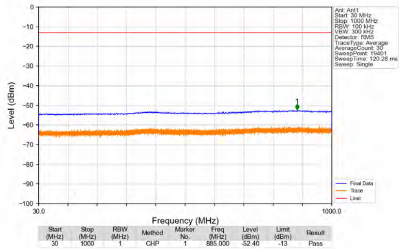
n2_15kHz_SISO_NTNV_25MHz_CP-OFDM_QPSK_1862.5MHz_Edge_1RB_Left
