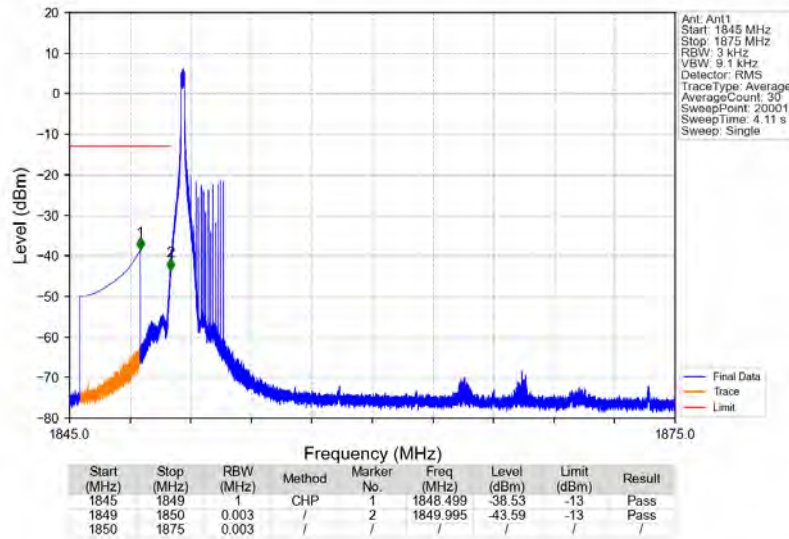
n2_15kHz_SISO_NTNV_25MHz_DFT-s-OFDM_QPSK_1862.5MHz_Edge_1RB_Left
