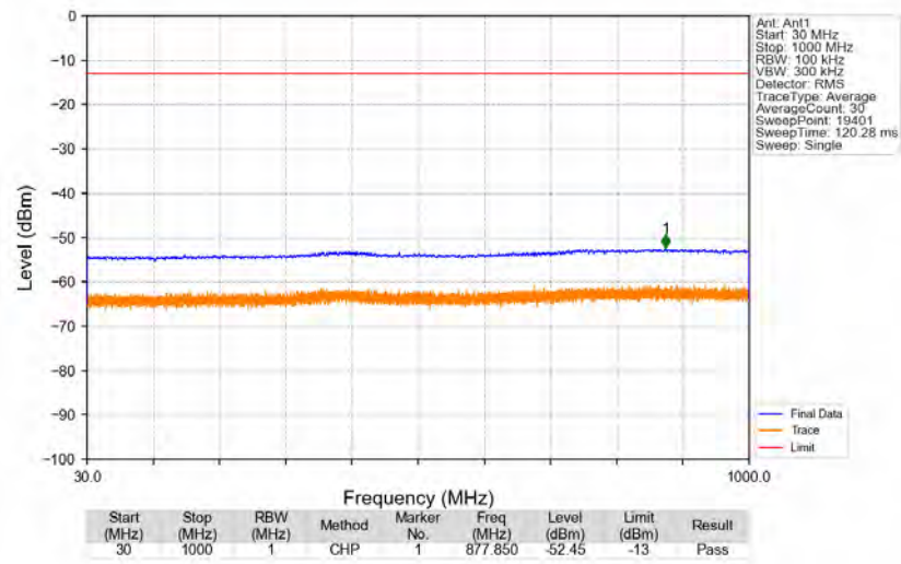
n2_15kHz_SISO_NTNV_25MHz_CP-OFDM_QPSK_1880MHz_Edge_1RB_Left
