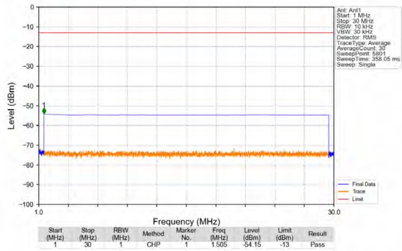
n2_15kHz_SISO_NTNV_20MHz_CP-OFDM_QPSK_1900MHz_Edge_1RB_Right
