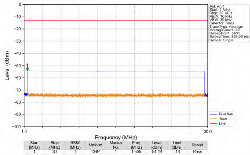
n2_15kHz_SISO_NTNV_40MHz_DFT-s-OFDM_QPSK_1880MHz_Edge_1RB_Left
