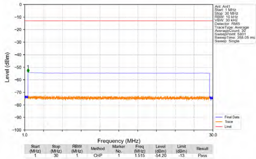
n2_15kHz_SISO_NTNV_25MHz_DFT-s-OFDM_QPSK_1880MHz_Edge_1RB_Left
