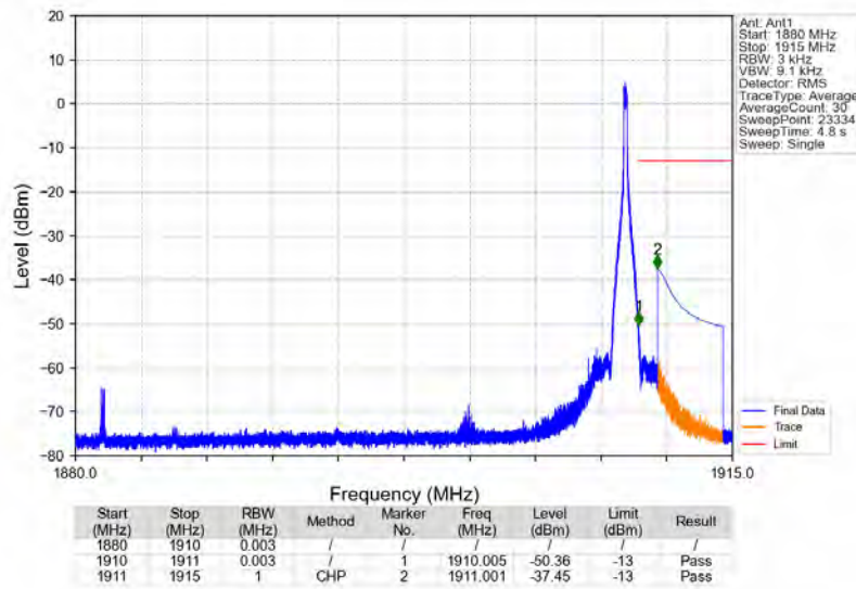
n2_15kHz_SISO_NTNV_30MHz_DFT-s-OFDM_QPSK_1895MHz_Edge_1RB_Right
