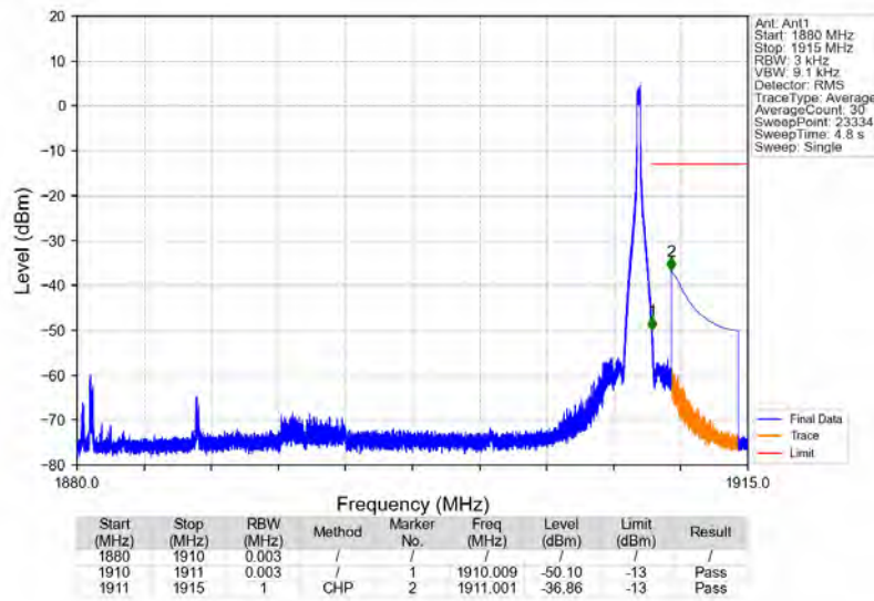
n2_15kHz_SISO_NTNV_30MHz_CP-OFDM_QPSK_1895MHz_Edge_1RB_Right
