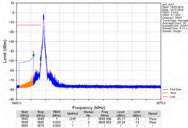
n2_15kHz_SISO_NTNV_25MHz_CP-OFDM_QPSK_1862.5MHz_Edge_1RB_Left
