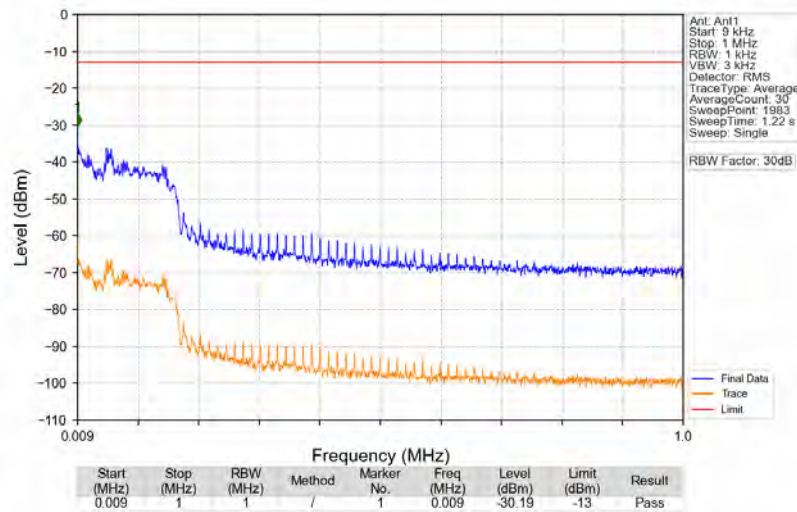
n2_15kHz_SISO_NTNV_30MHz_DFT-s-OFDM_QPSK_1895MHz_Edge_1RB_Right
