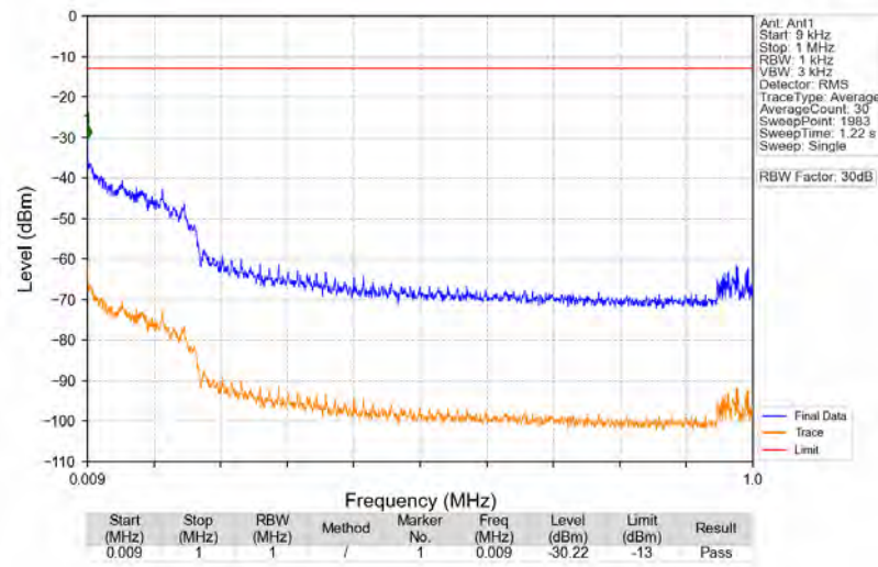
n2_15kHz_SISO_NTNV_25MHz_CP-OFDM_QPSK_1880MHz_Edge_1RB_Left
