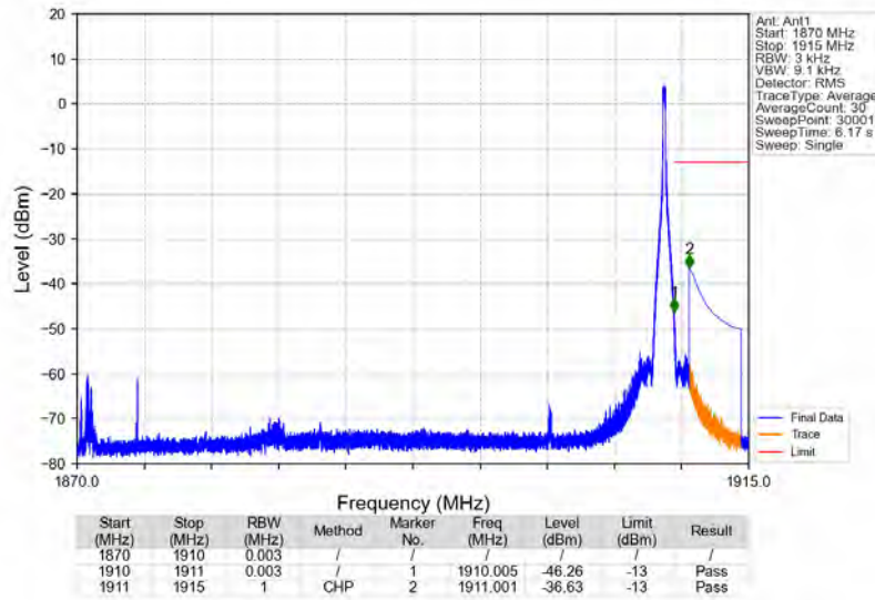
n2_15kHz_SISO_NTNV_40MHz_CP-OFDM_QPSK_1890MHz_Edge_1RB_Right
