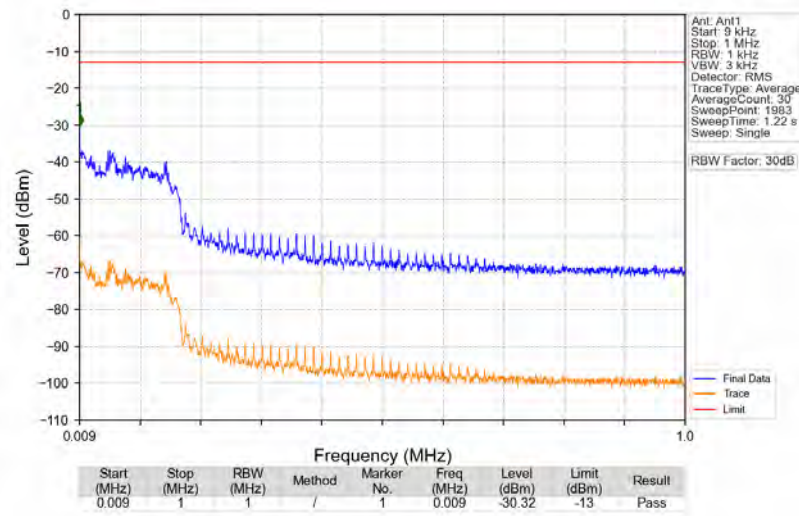
n2_15kHz_SISO_NTNV_25MHz_DFT-s-OFDM_QPSK_1880MHz_Edge_1RB_Left
