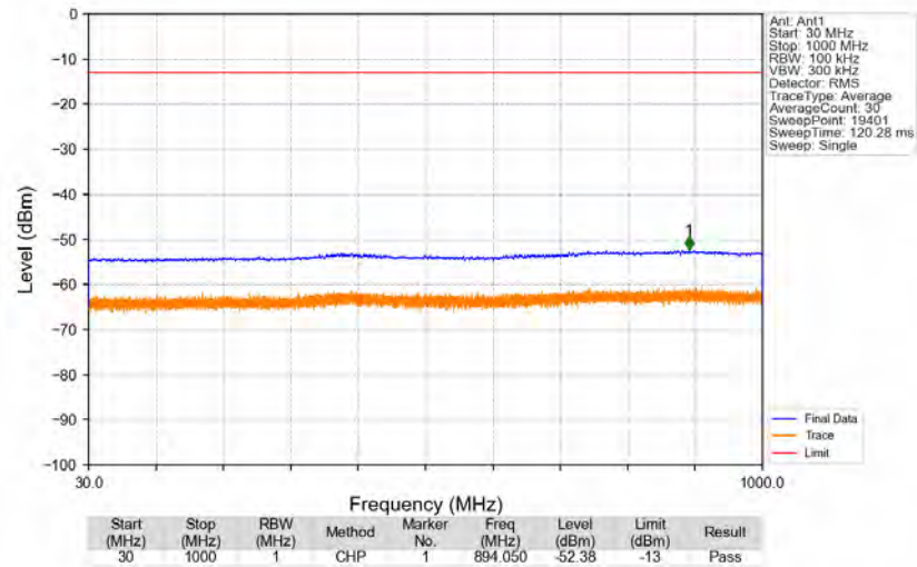
n2_15kHz_SISO_NTNV_30MHz_DFT-s-OFDM_QPSK_1895MHz_Edge_1RB_Right
