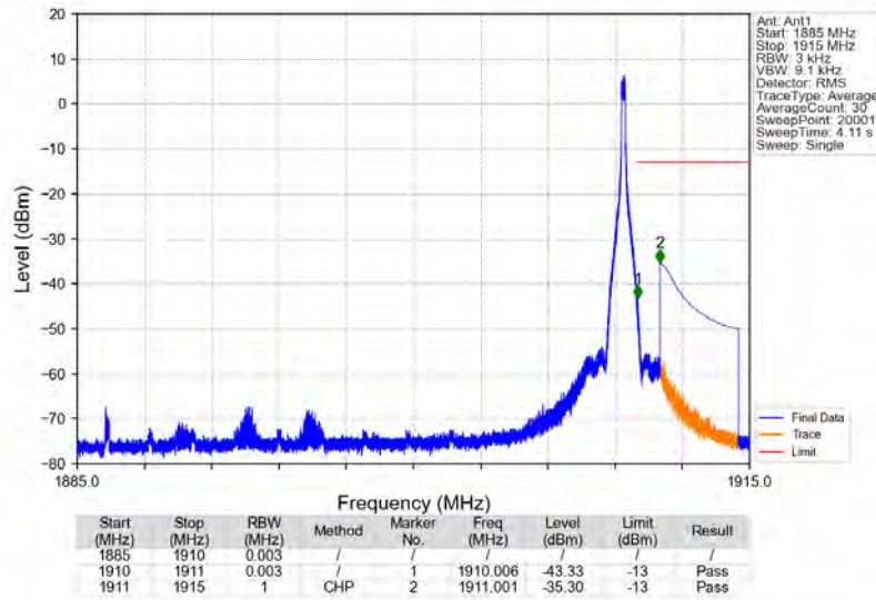
n2_15kHz_SISO_NTNV_25MHz_DFT-s-OFDM_QPSK_1897.5MHz_Edge_1RB_Right
