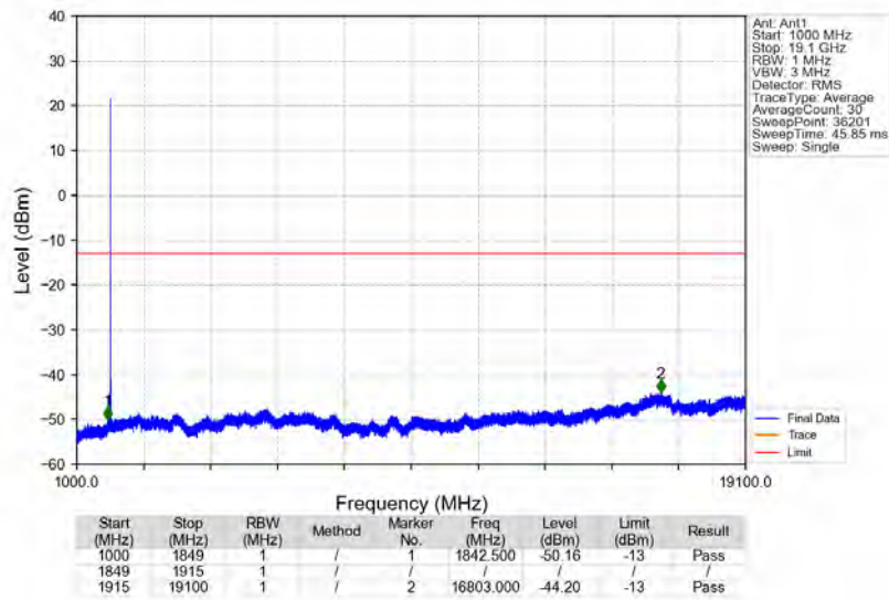
n2_15kHz_SISO_NTNV_25MHz_DFT-s-OFDM_PI/2_BPSK_1897.5MHz_Edge_1RB_Right
