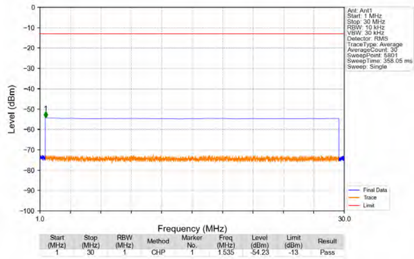
n2_15kHz_SISO_NTNV_25MHz_DFT-s-OFDM_QPSK_1862.5MHz_Edge_1RB_Left
