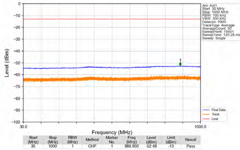
n2_15kHz_SISO_NTNV_25MHz_DFT-s-OFDM_QPSK_1880MHz_Edge_1RB_Left
