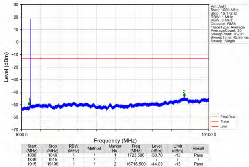
n2_15kHz_SISO_NTNV_25MHz_CP-OFDM_QPSK_1880MHz_Edge_1RB_Left
