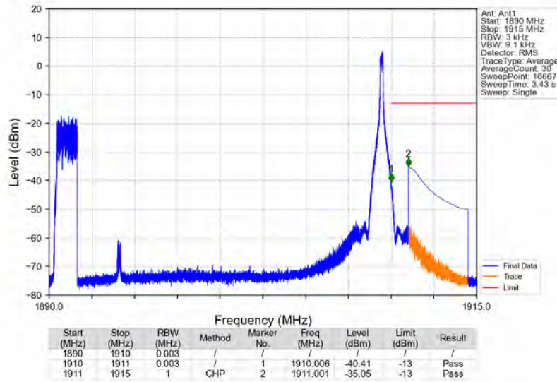
n2_15kHz_SISO_NTNV_20MHz_CP-OFDM_QPSK_1900MHz_Edge_1RB_Right
