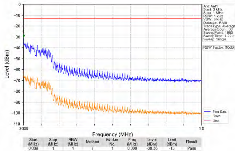
n2_15kHz_SISO_NTNV_20MHz_CP-OFDM_QPSK_1900MHz_Edge_1RB_Right
