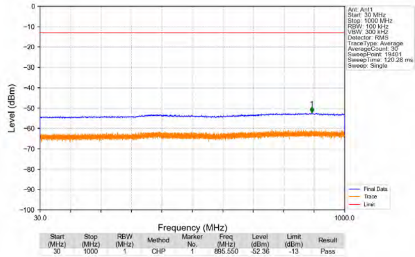
n2_15kHz_SISO_NTNV_40MHz_DFT-s-OFDM_QPSK_1890MHz_Edge_1RB_Right
