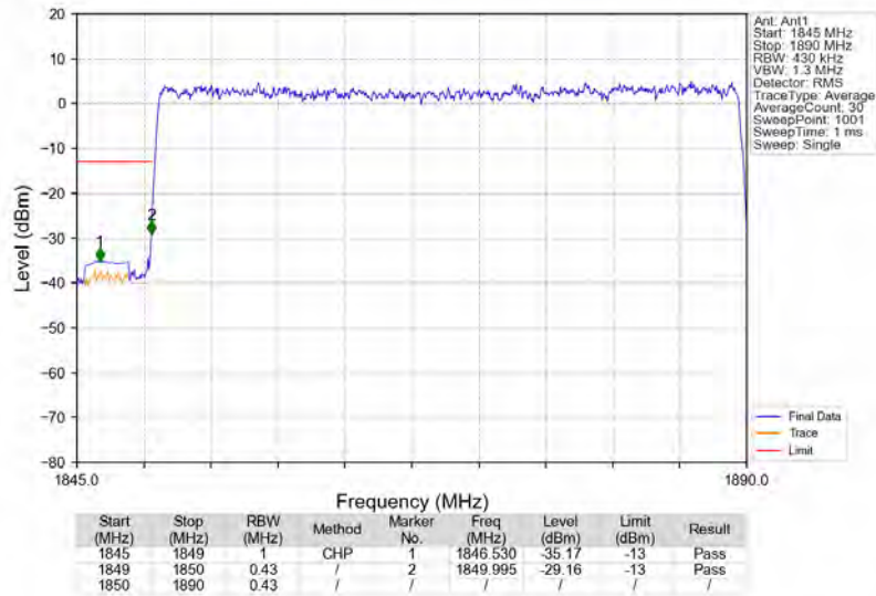
n2_15kHz_SISO_NTNV_40MHz_DFT-s-OFDM_QPSK_1870MHz_Outer_Full
