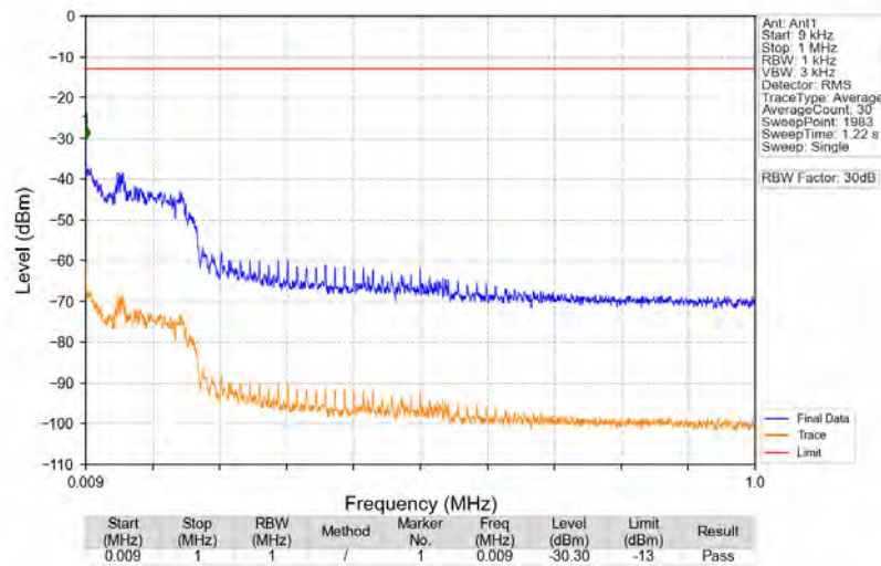
n2_15kHz_SISO_NTNV_40MHz_DFT-s-OFDM_QPSK_1890MHz_Edge_1RB_Right
