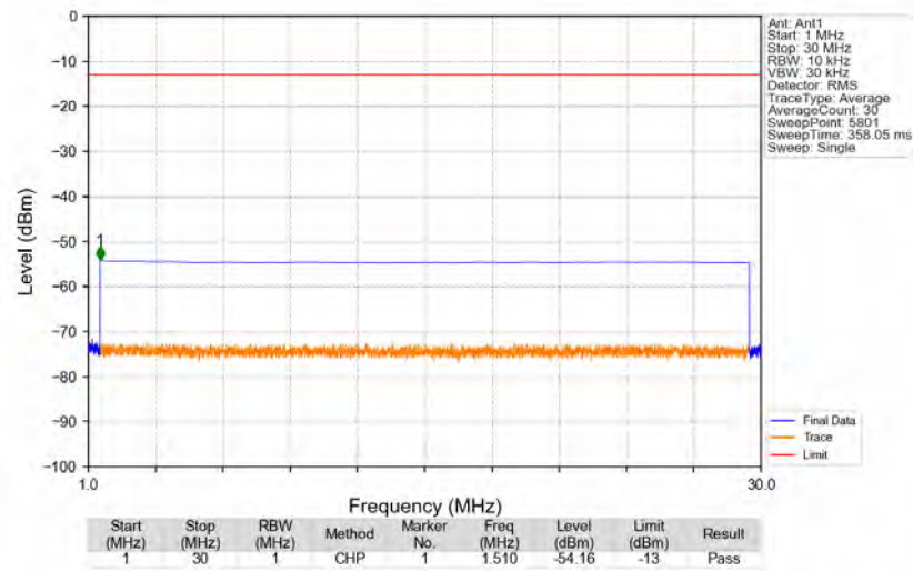
n2_15kHz_SISO_NTNV_30MHz_DFT-s-OFDM_QPSK_1880MHz_Edge_1RB_Left
