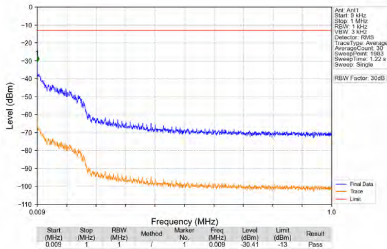
n2_15kHz_SISO_NTNV_25MHz_CP-OFDM_QPSK_1862.5MHz_Edge_1RB_Left
