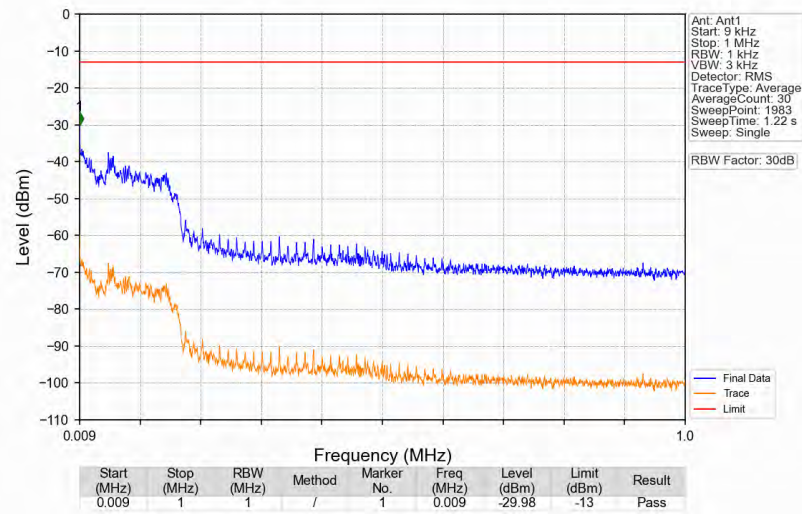
n2_15kHz_SISO_NTNV_40MHz_DFT-s-OFDM_QPSK_1880MHz_Edge_1RB_Left
