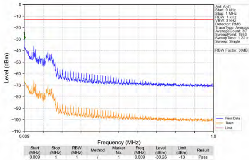
n2_15kHz_SISO_NTNV_25MHz_DFT-s-OFDM_PI/2_BPSK_1897.5MHz_Edge_1RB_Right
