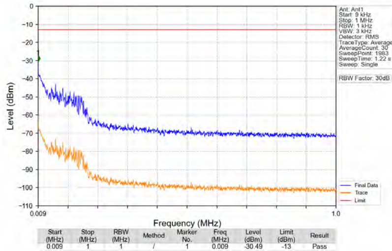
n2_15kHz_SISO_NTNV_25MHz_DFT-s-OFDM_QPSK_1862.5MHz_Edge_1RB_Left
