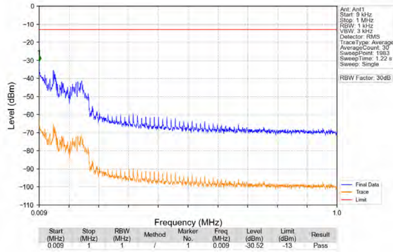
n2_15kHz_SISO_NTNV_25MHz_DFT-s-OFDM_PI/2_BPSK_1880MHz_Edge_1RB_Left
