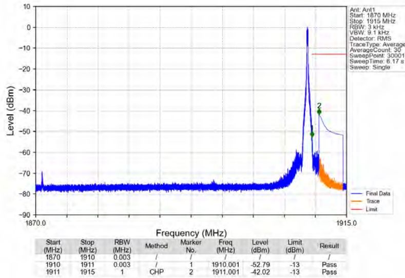
n2_15kHz_SISO_NTNV_40MHz_DFT-s-OFDM_QPSK_1890MHz_Edge_1RB_Right
