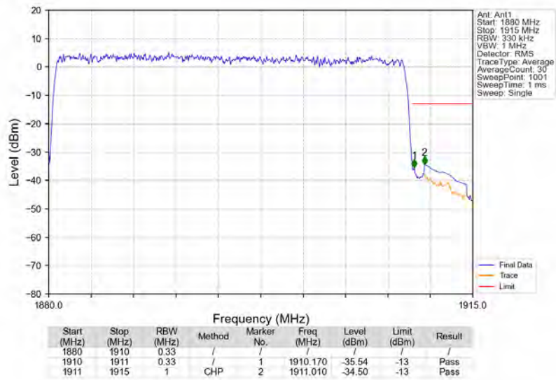
n2_15kHz_SISO_NTNV_30MHz_DFT-s-OFDM_PI/2_BPSK_1895MHz_Outer_Full
