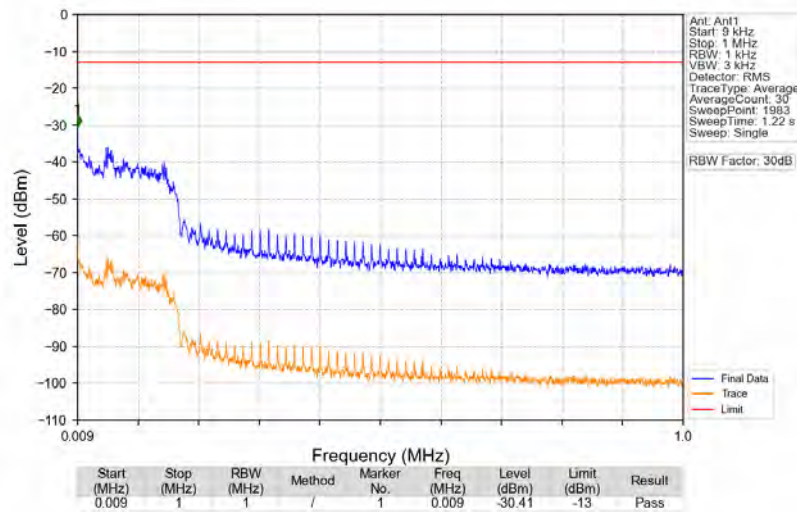
n2_15kHz_SISO_NTNV_25MHz_DFT-s-OFDM_QPSK_1897.5MHz_Edge_1RB_Right
