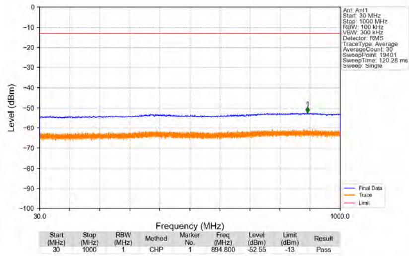
n2_15kHz_SISO_NTNV_25MHz_DFT-s-OFDM_PI/2_BPSK_1880MHz_Edge_1RB_Left
