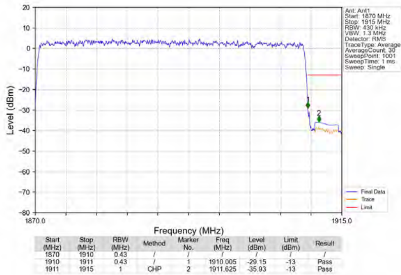
n2_15kHz_SISO_NTNV_40MHz_DFT-s-OFDM_PI/2_BPSK_1890MHz_Outer_Full
