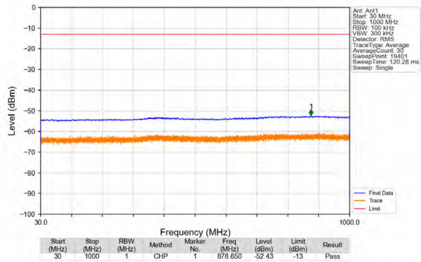
n2_15kHz_SISO_NTNV_25MHz_DFT-s-OFDM_PI/2_BPSK_1897.5MHz_Edge_1RB_Right
