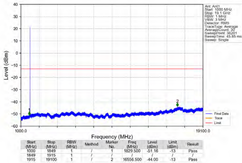
n2_15kHz_SISO_NTNV_40MHz_DFT-s-OFDM_PI/2_BPSK_1890MHz_Edge_1RB_Right
