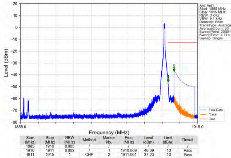
n2_15kHz_SISO_NTNV_25MHz_CP-OFDM_QPSK_1897.5MHz_Edge_1RB_Right
