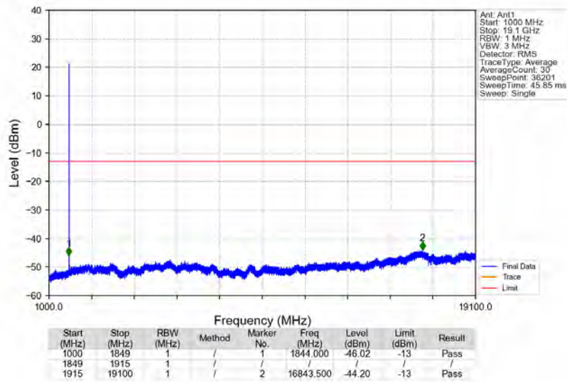
n2_15kHz_SISO_NTNV_25MHz_DFT-s-OFDM_QPSK_1862.5MHz_Edge_1RB_Left
