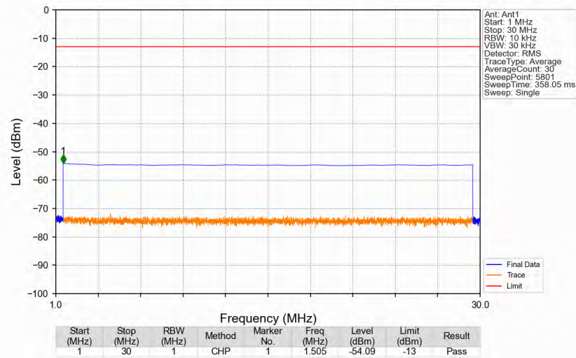
n2_15kHz_SISO_NTNV_25MHz_DFT-s-OFDM_PI/2_BPSK_1880MHz_Edge_1RB_Left
