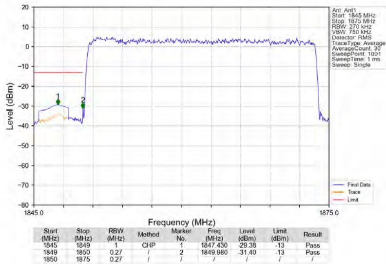
n2_15kHz_SISO_NTNV_25MHz_DFT-s-OFDM_QPSK_1862.5MHz_Outer_Full
