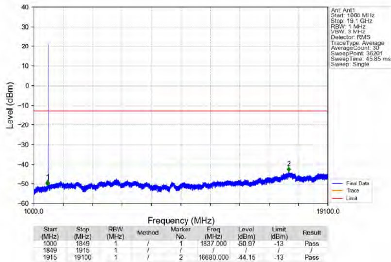
n2_15kHz_SISO_NTNV_30MHz_DFT-s-OFDM_PI/2_BPSK_1895MHz_Edge_1RB_Right
