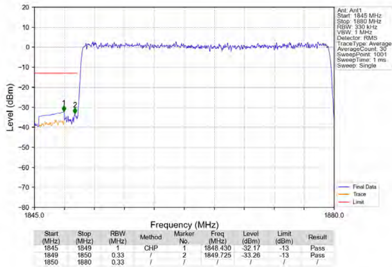
n2_15kHz_SISO_NTNV_30MHz_CP-OFDM_QPSK_1865MHz_Outer_Full
