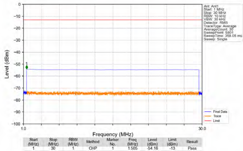
n2_15kHz_SISO_NTNV_30MHz_CP-OFDM_QPSK_1880MHz_Edge_1RB_Left
