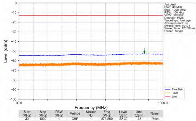
n2_15kHz_SISO_NTNV_40MHz_CP-OFDM_QPSK_1890MHz_Edge_1RB_Right
