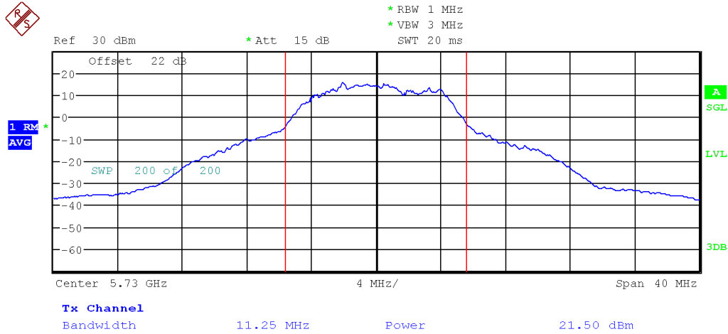
Figure 8: FCC Uncorrelated Max Conducted Power-5730 MHz-802.11n-MCS 0-10MHz-Ch1
