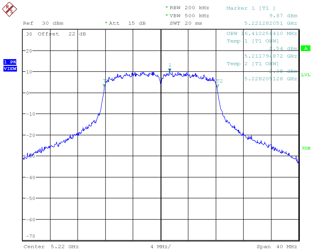
Figure 15: Occupied Bandwidth-5220 MHz-802.11a
