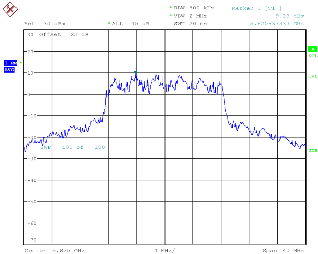
Figure 34: FCC Uncorrelated Power Spectral Density-5825 MHz-802.11a-6 Mbps-20MHz-Ch1
