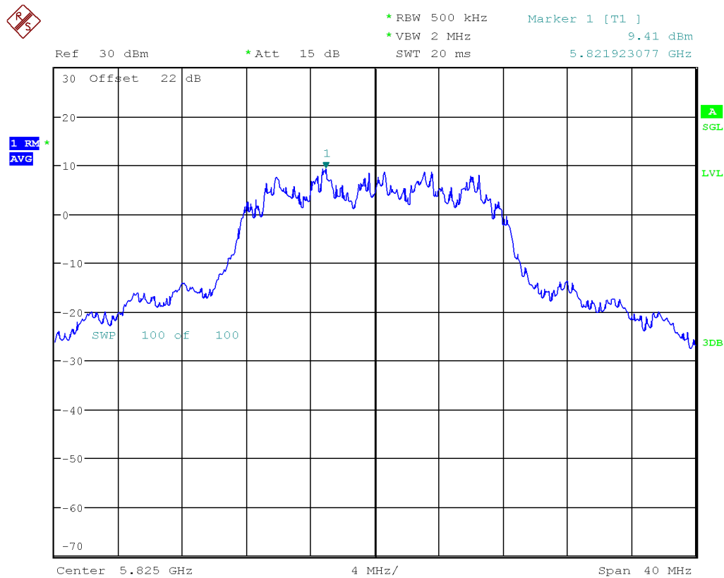
Figure 33: FCC Uncorrelated Power Spectral Density-5825 MHz-802.11a-6 Mbps-20MHz -Ch0
