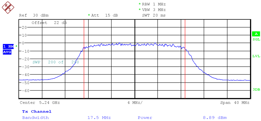
Figure 2: IC Uncorrelated Max Conducted Power-5240 MHz-802.11n-MCS 0-20MHz-Ch1
