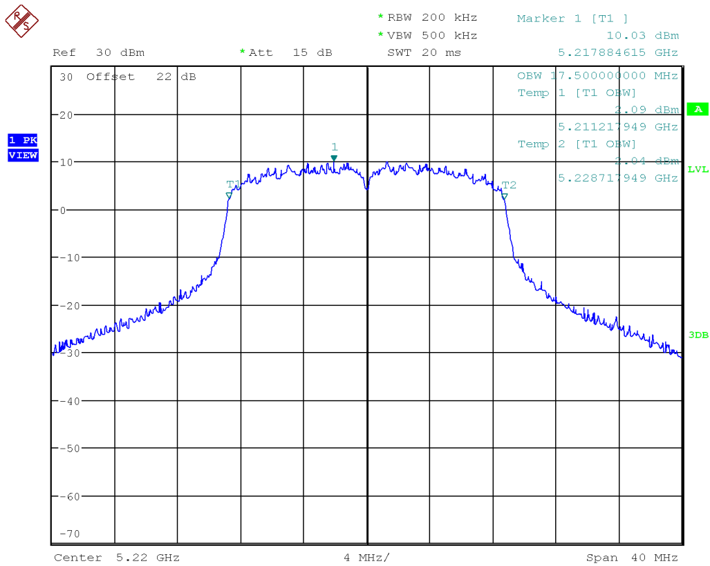
Figure 21: Occupied Bandwidth-5220 MHz-802.11ac VHT20
