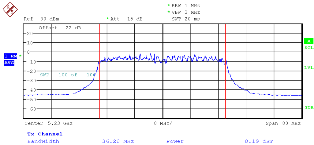
Figure 10: FCC Uncorrelated Max Conducted Power-5230 MHz-802.11ac-MCS 0-40MHz-Ch1
