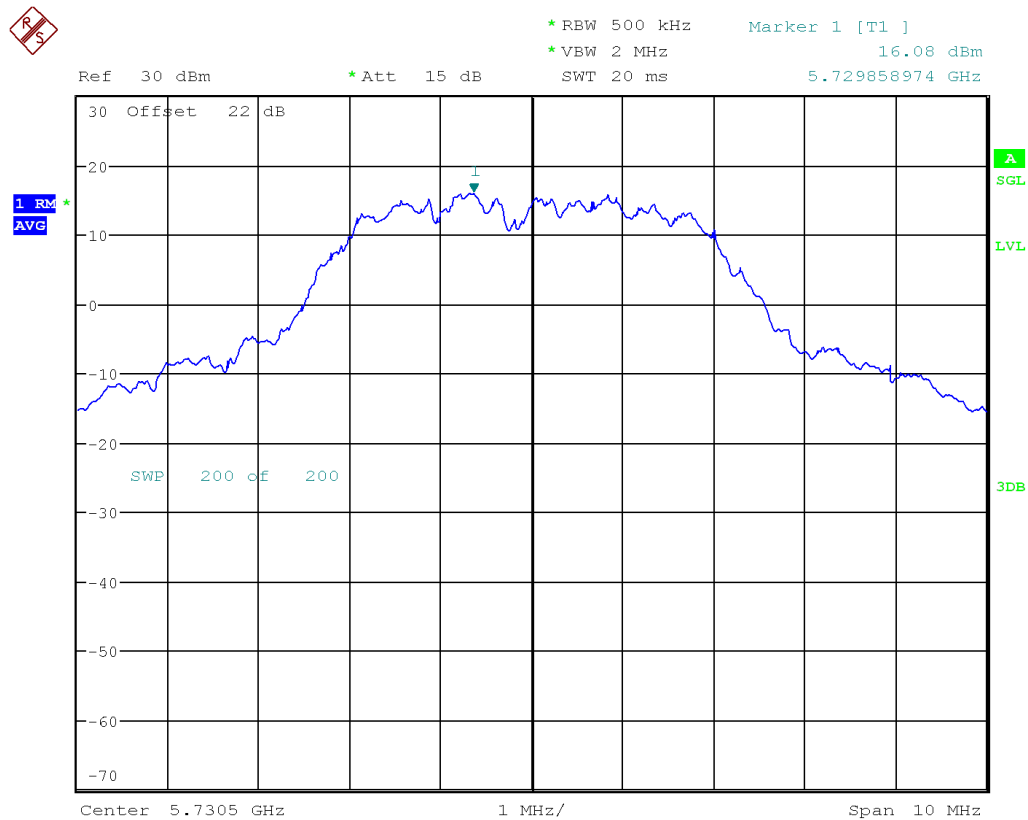
Figure 30: FCC Uncorrelated Power Spectral Density-5730.5 MHz-802.11n-HT MCSO -5MHz-Ch1
