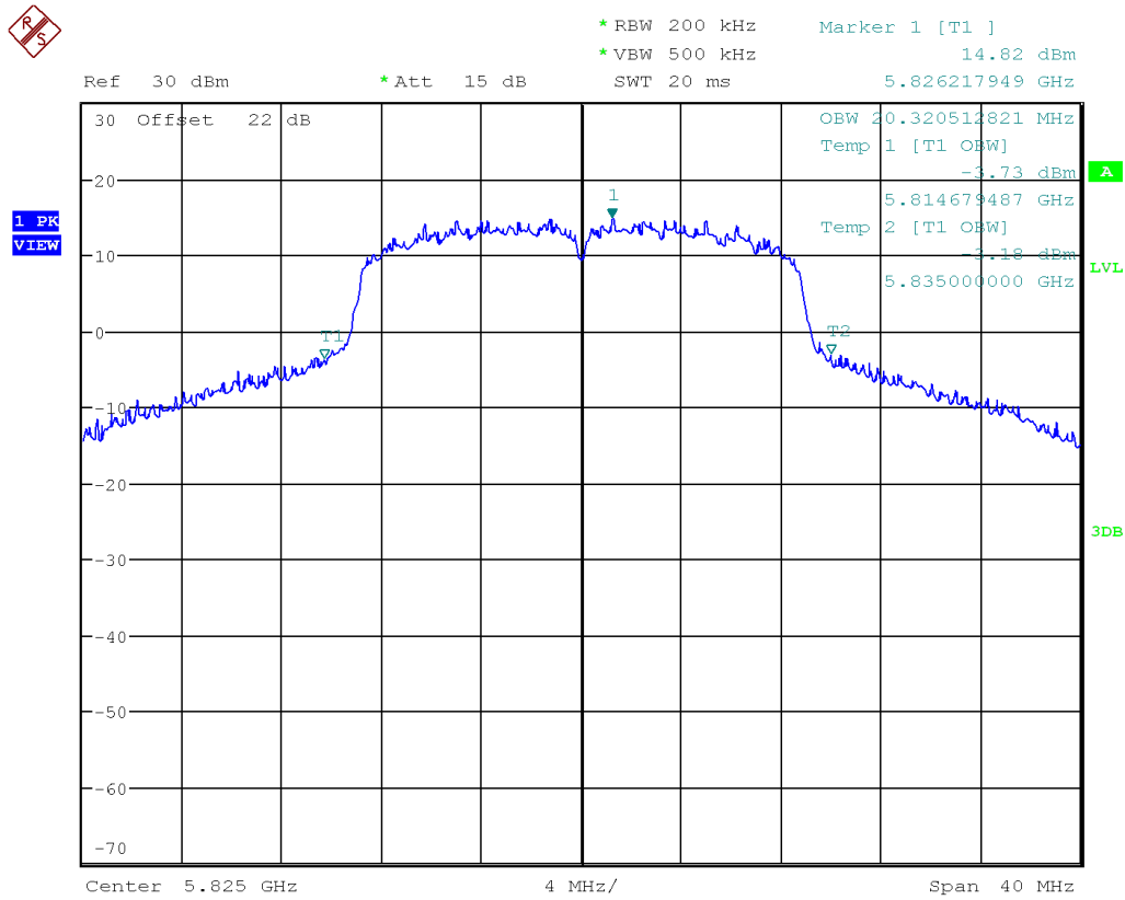
Figure 18: Occupied Bandwidth-5825 MHz-802.11n HT20
