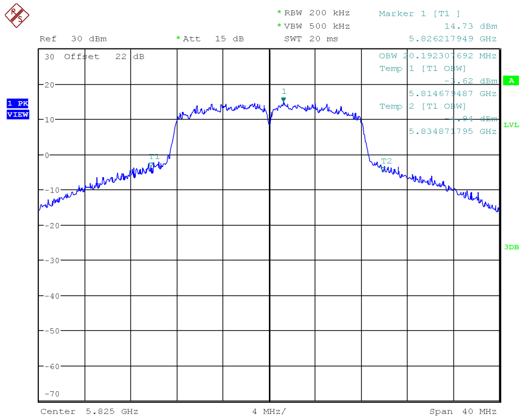
Figure 16: Occupied Bandwidth-5825 MHz-802.11a
