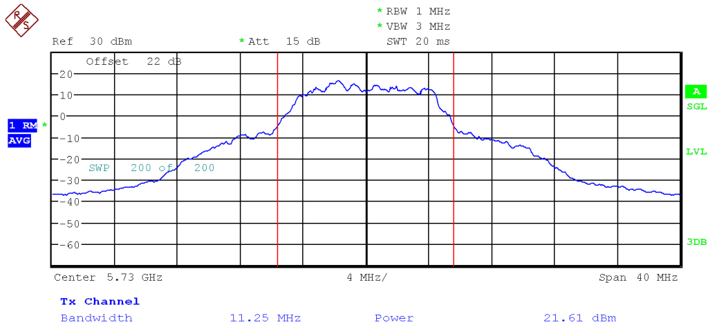
Figure 7: FCC Uncorrelated Max Conducted Power-5730 MHz-802.11n-MCS 0-10MHz-Ch0
