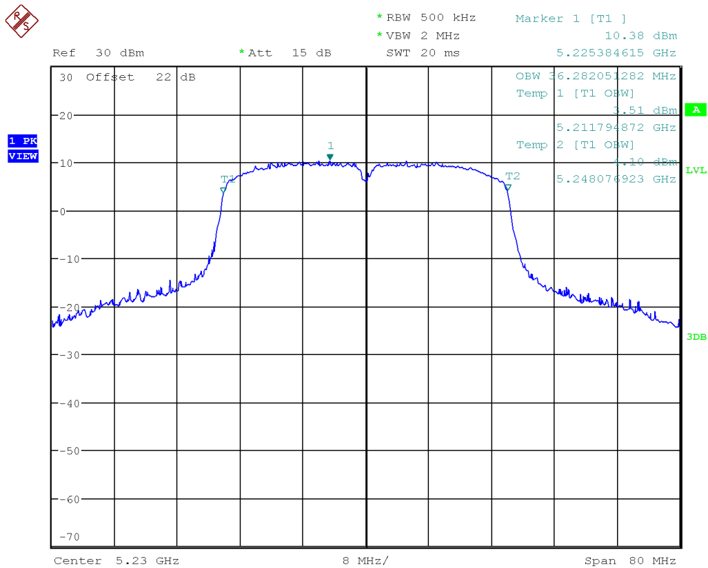
Figure 23: Occupied Bandwidth-5230 MHz-802.11ac VHT40
