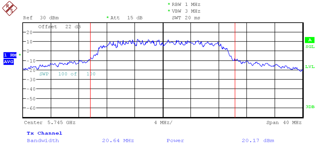
Figure 12: FCC Uncorrelated Max Conducted Power-5745 MHz-802.11ac VHT-MCS 0-20MHz- Ch1
