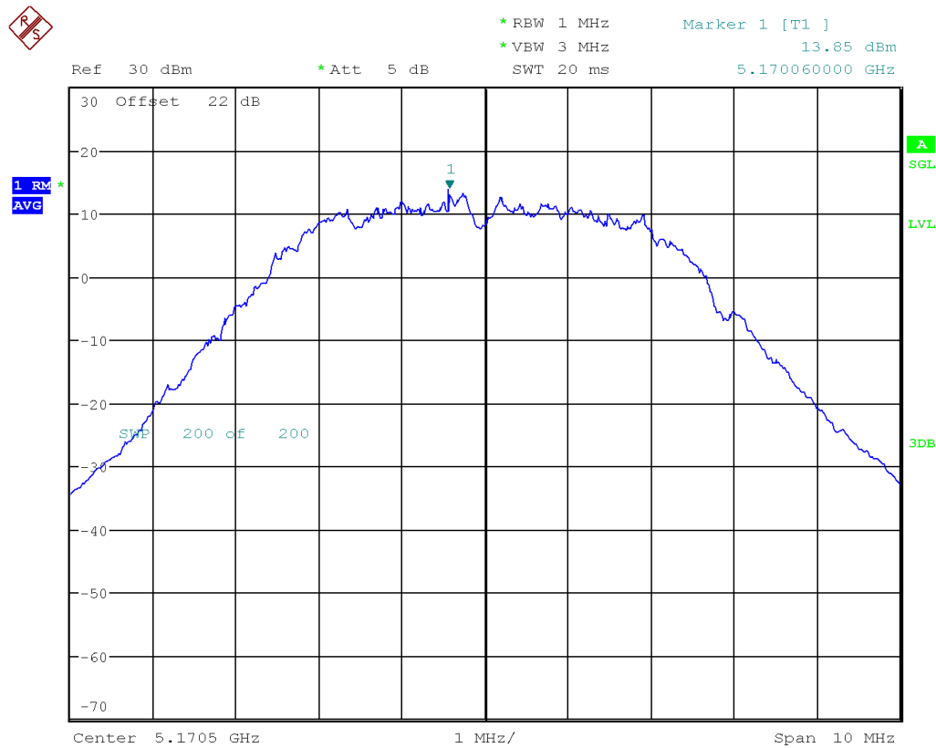
Figure 28: FCC Uncorrelated Power Spectral Density-5170.5 MHz-802.11a-6 Mbps-5MHz-Ch1
