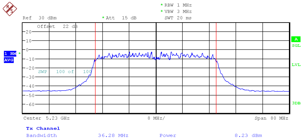
Figure 9: FCC Uncorrelated Max Conducted Power-5230 MHz-802.11ac-MCS 0-40MHz-Ch0
