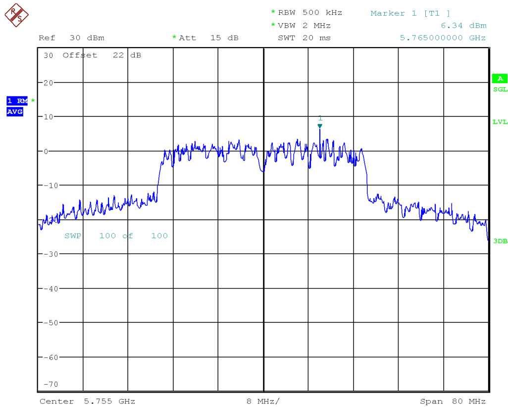
Figure 31: FCC Uncorrelated Power Spectral Density-5755 MHz-802.11n-HT MCSO-40MHz -Ch0
