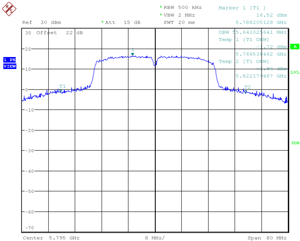
Figure 20: Occupied Bandwidth-5795 MHz-802.11n HT40
