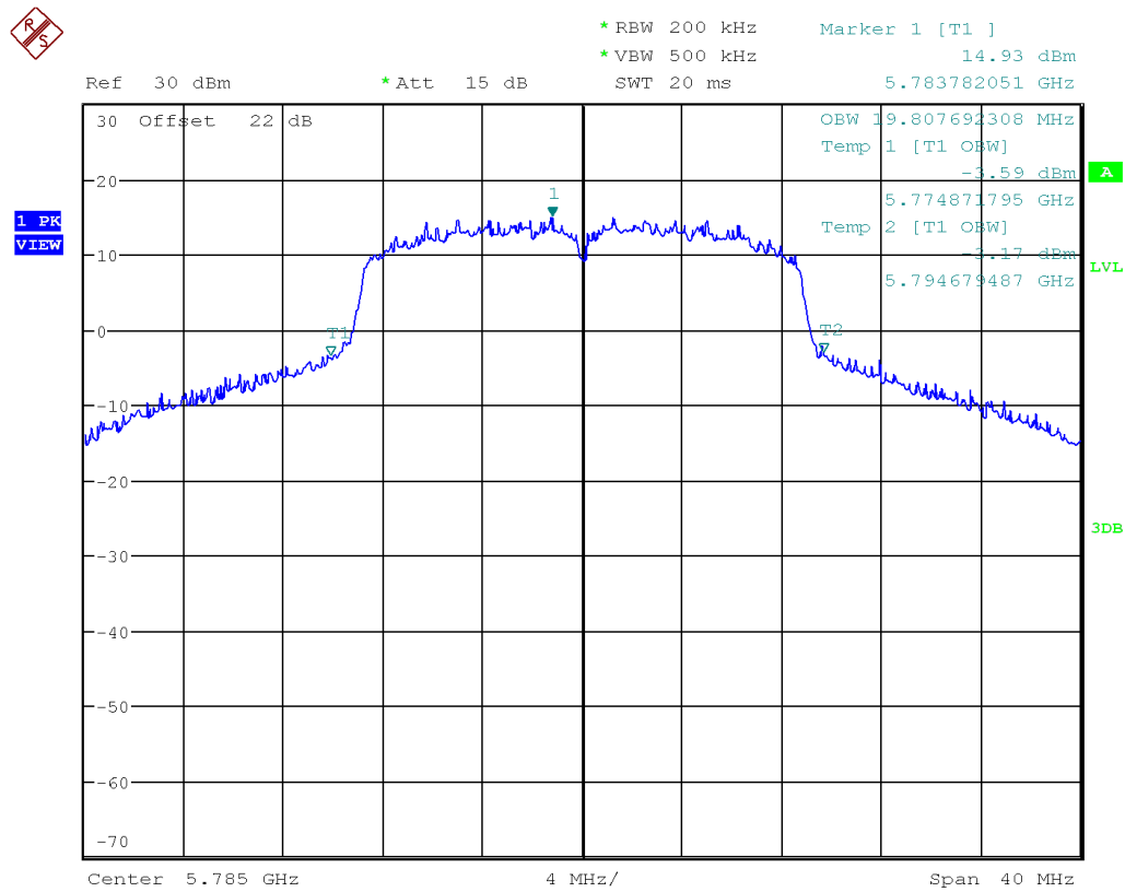
Figure 22: Occupied Bandwidth-5785 MHz-802.11ac VHT20
