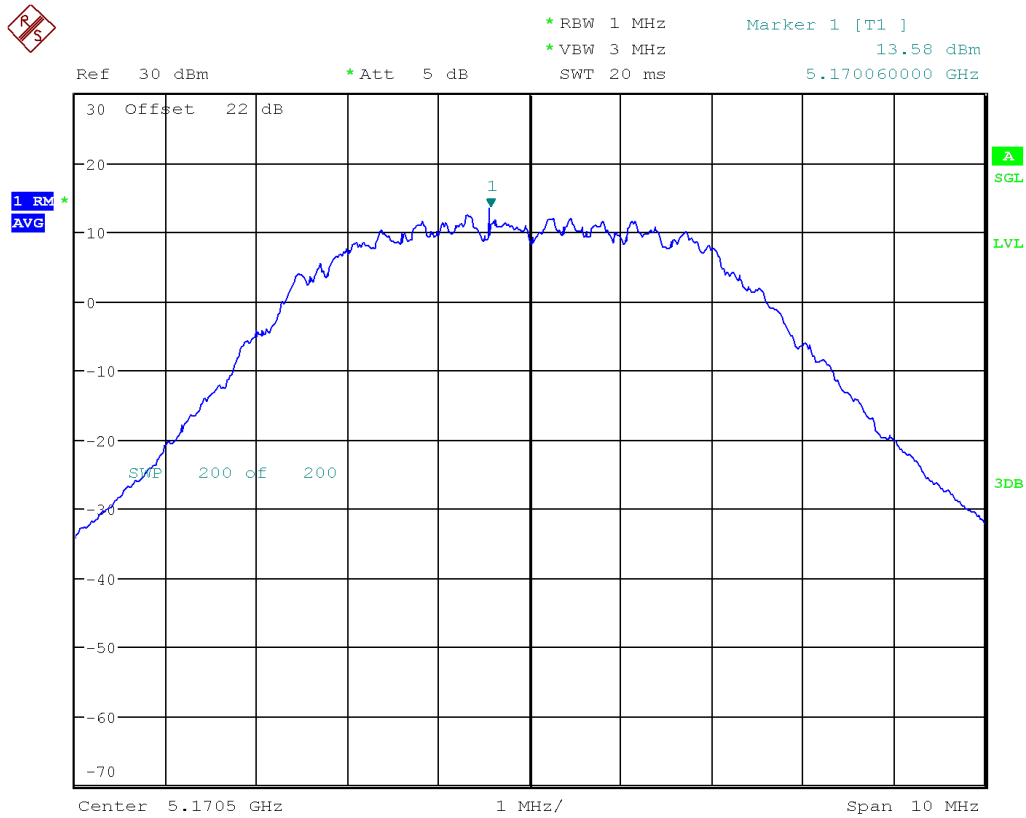
Figure 27: FCC Uncorrelated Power Spectral Density-5170.5 MHz-802.11a-6 Mbps-5MHz -Ch0
