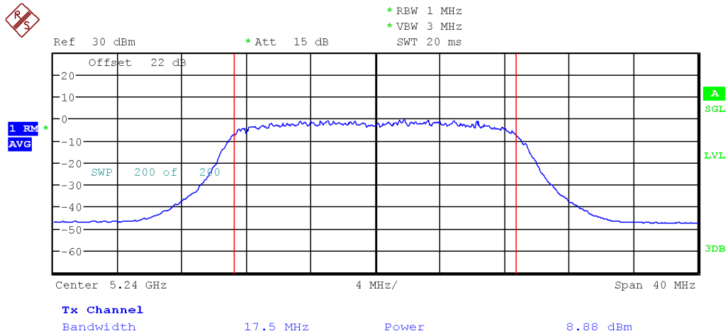
Figure 1: IC Uncorrelated Max Conducted Power-5240 MHz-802.11n-MCS 0-20MHz-Ch0
