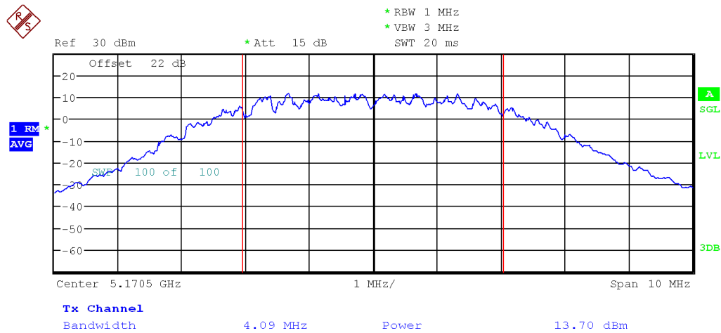
Figure 3: FCC Uncorrelated Max Conducted Power-5170.5 MHz-802.11a-6 Mnps-5MHz-Ch0
