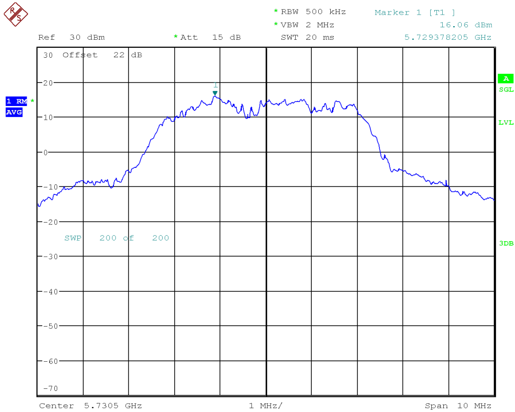
Figure 29: FCC Uncorrelated Power Spectral Density-5730.5 MHz-802.11n-HT MCSO-5MHz -Ch0
