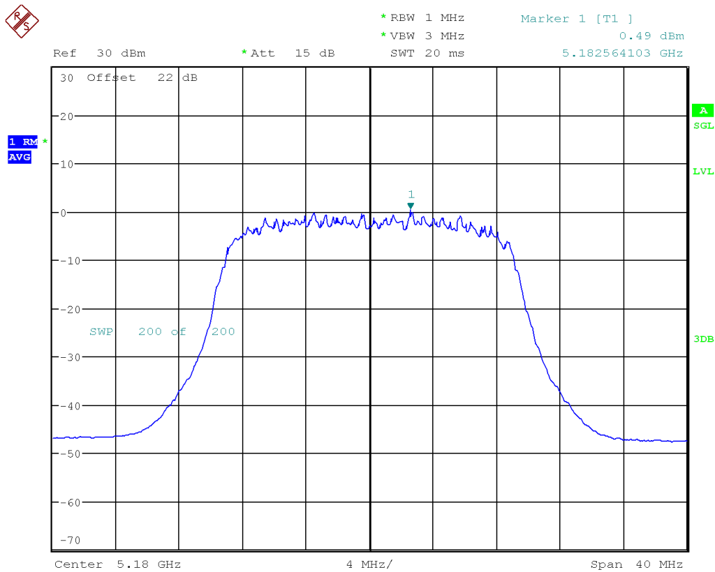
Figure 26: IC Uncorrelated Power Spectral Density-5180 MHz-802.11n-HT MCSO-20MHz-Ch1
