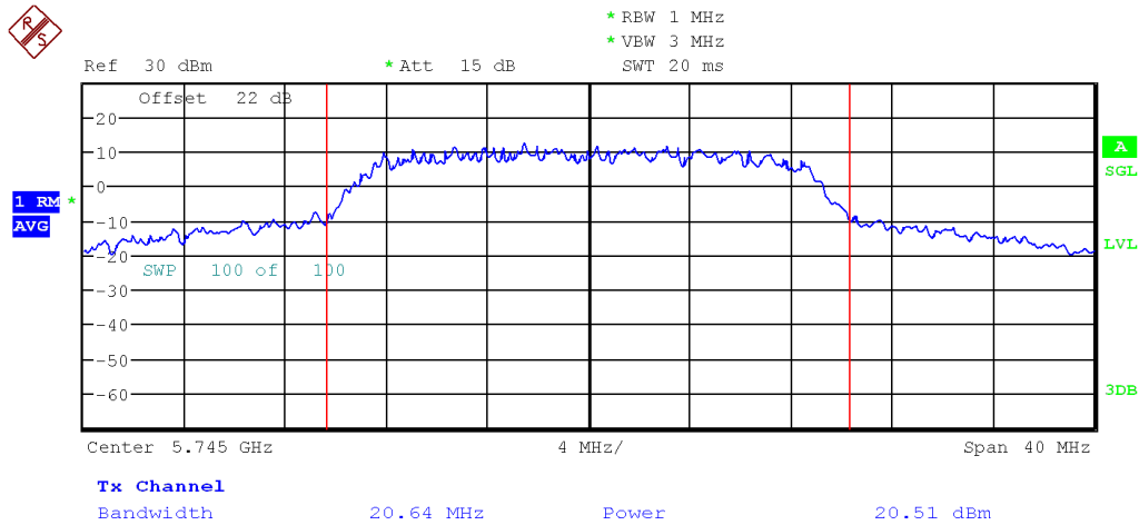
Figure 11: FCC Uncorrelated Max Conducted Power-5745 MHz-802.11ac VHT-MCS 0-20MHz - Ch0
