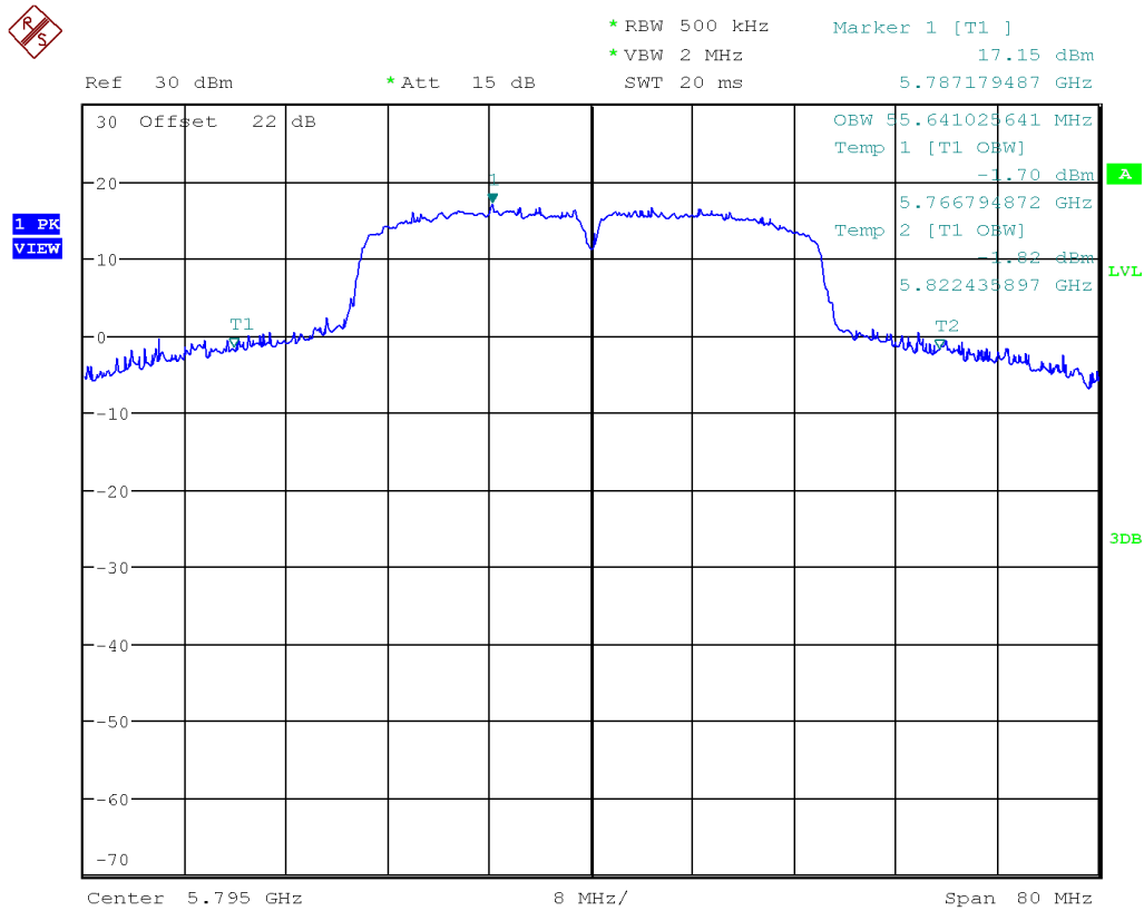
Figure 24: Occupied Bandwidth-5795 MHz-802.11ac VHT40
