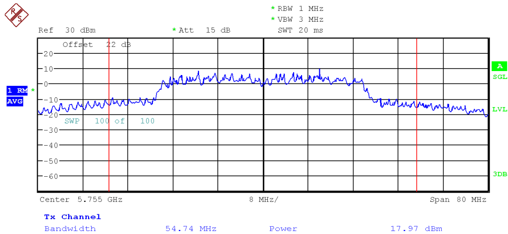
Figure 13: FCC Uncorrelated Max Conducted Power-5755 MHz-802.11ac VHT-MCS 0-40MHz - Ch0
