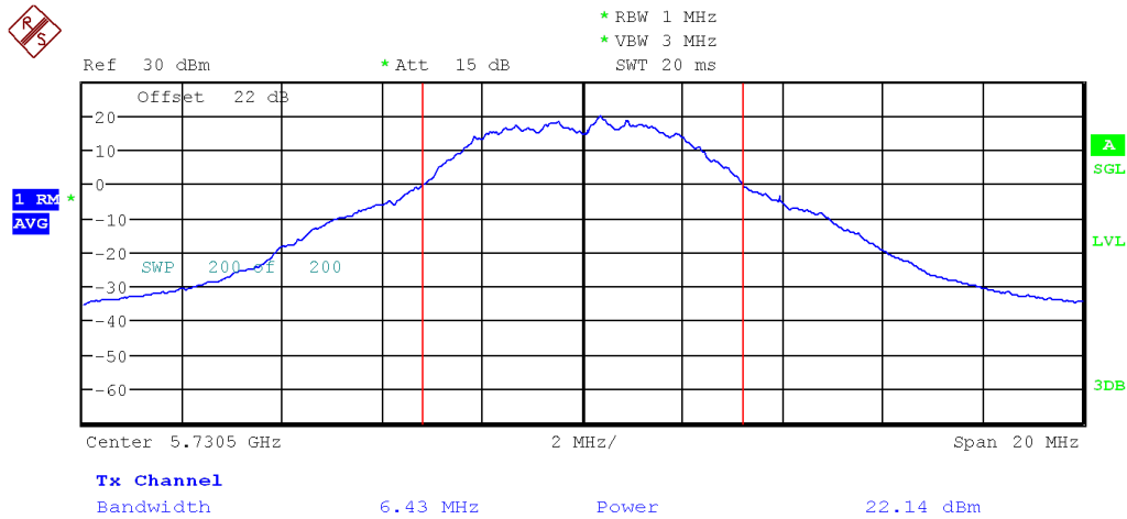
Figure 5: FCC Uncorrelated Max Conducted Power-5730.5 MHz-802.11a-6 Mnps-5MHz-Ch0
