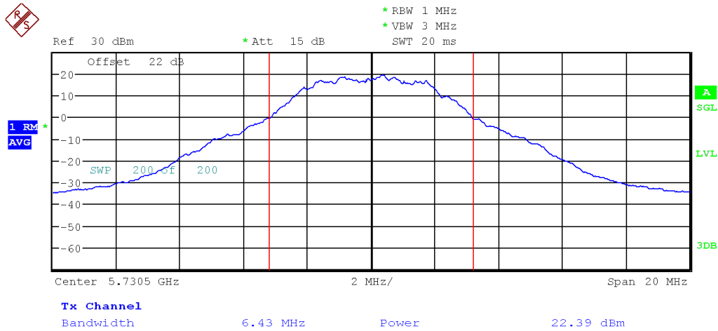
Figure 6: FCC Uncorrelated Max Conducted Power-5730.5 MHz-802.11a-6 Mbps-5MHz-Ch1
