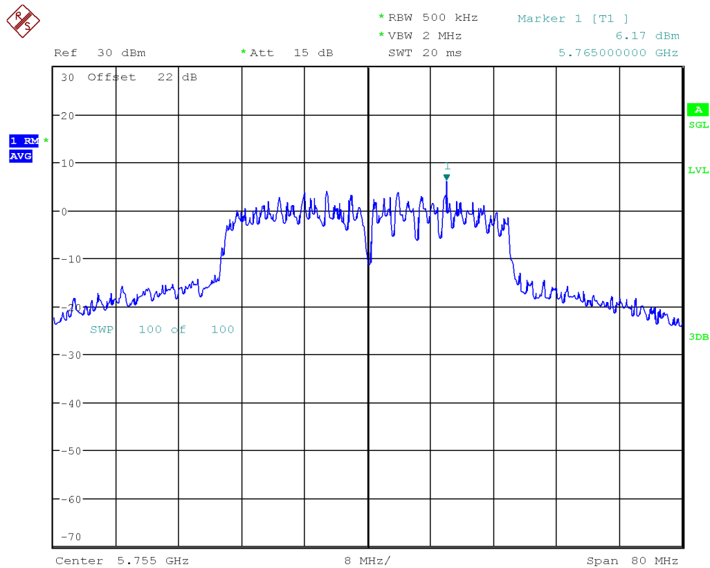
Figure 32: FCC Uncorrelated Power Spectral Density-5755 MHz-802.11n-HT MCSO -40MHz-Ch1
