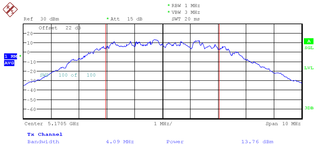
Figure 4: FCC Uncorrelated Max Conducted Power-5170.5 MHz-802.11a-6 Mbps-5MHz-Ch1
