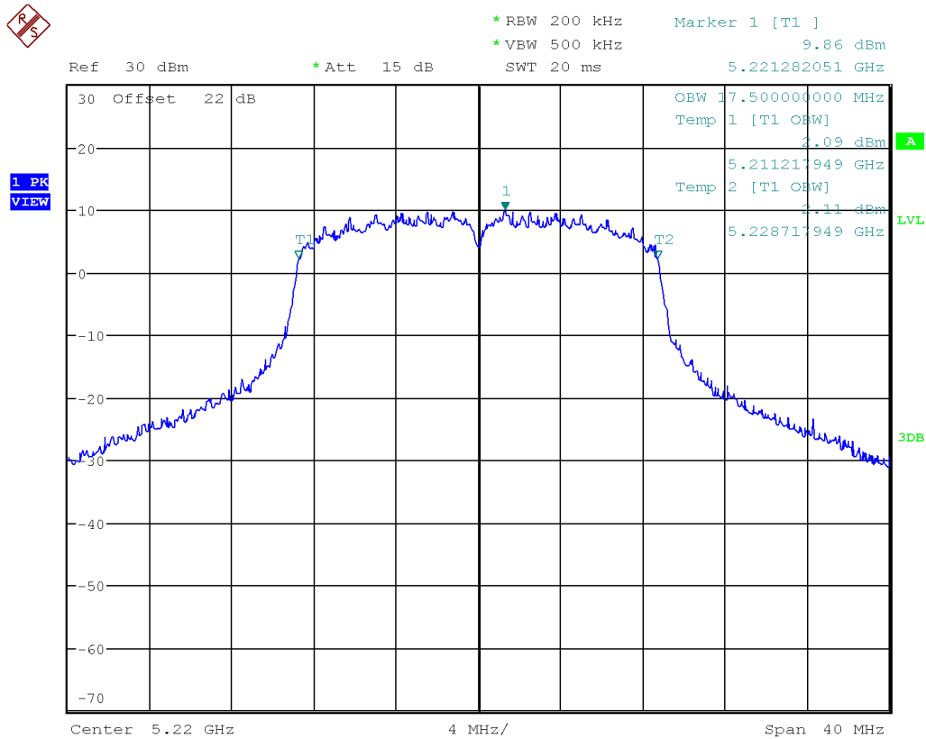
Figure 17: Occupied Bandwidth-5220 MHz-802.11n HT20
