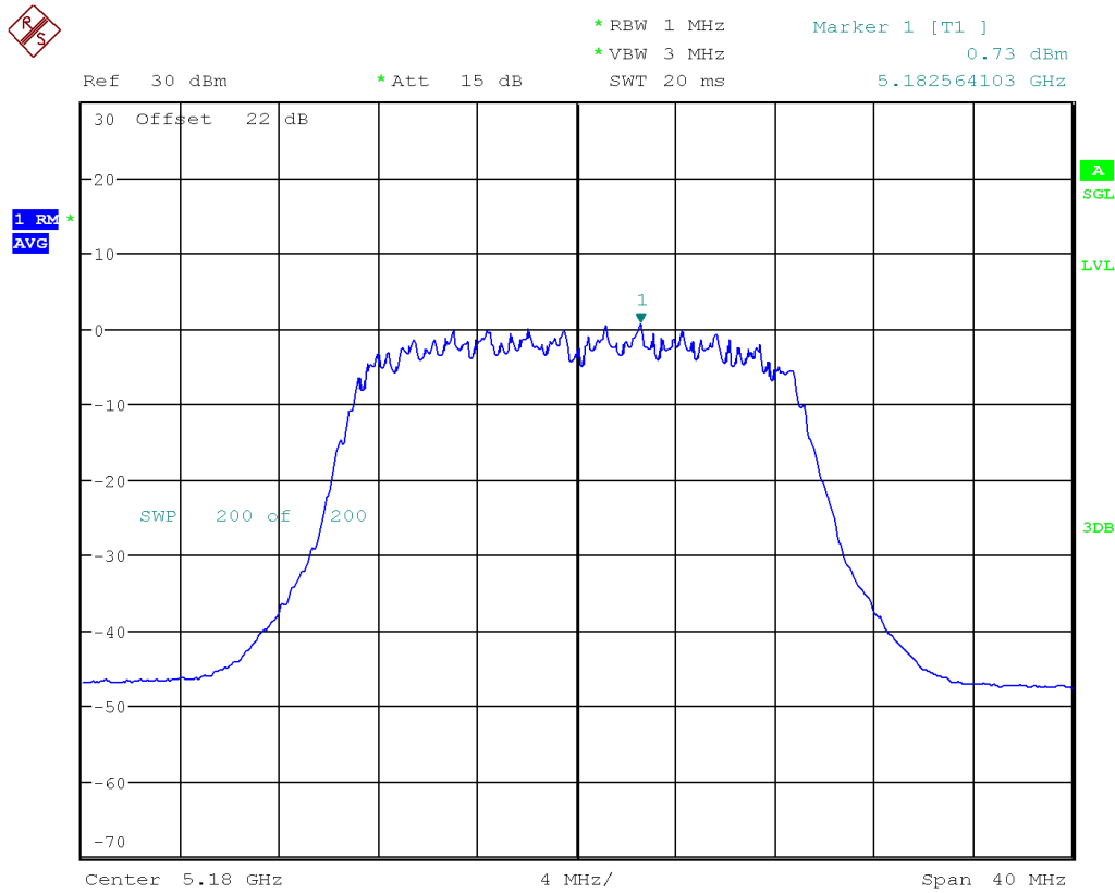
Figure 25: IC Uncorrelated Power Spectral Density-5180 MHz-802.11n-HT MCSO-20MHz -Ch0
