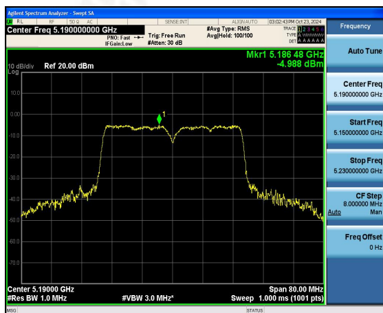
(802.11n40) PSD plot on channel 38
