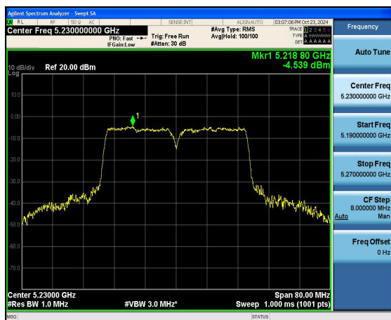
(802.11n40) PSD plot on channel 46
