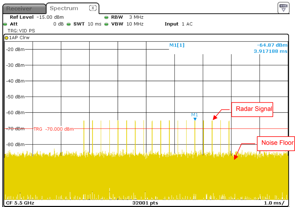
Radar Signal 3
