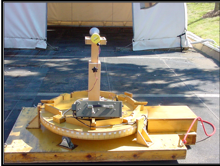
Photograph 13: Radiated Emissions Front View 24.7dBi Horn Antenna
