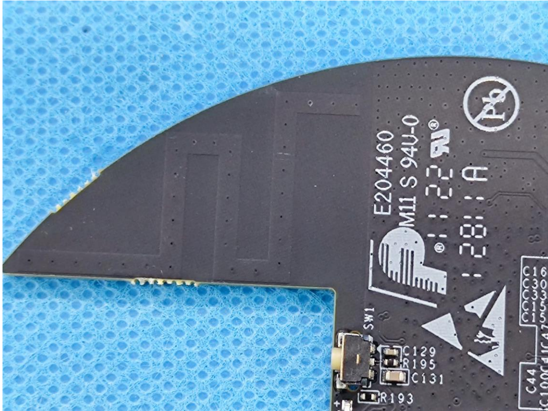
RX Antenna(Back Side)
