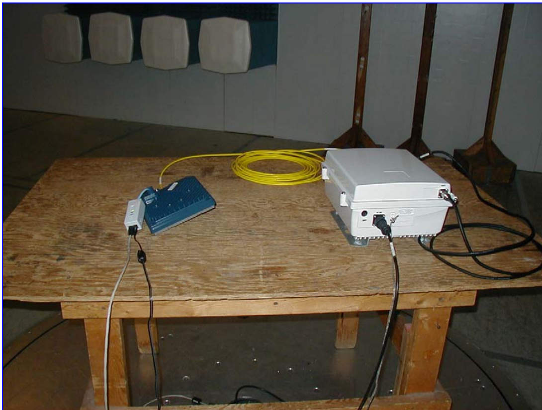
Photograph 2. Radiated Emission Limits Test Setup
