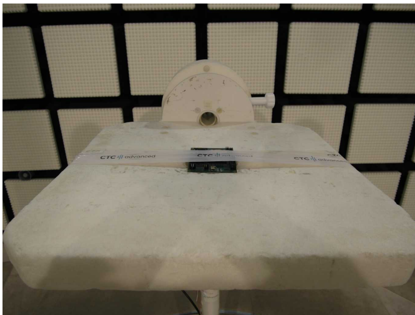
Photo 4 RSE > 1GHz
