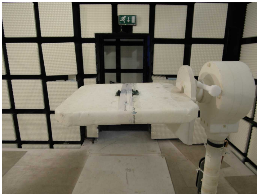
Photo 2 RSE > 1GHz
