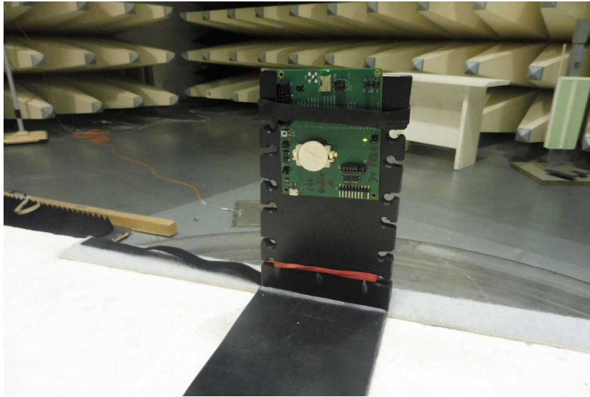
Photo 7 RSE < 1GHz
