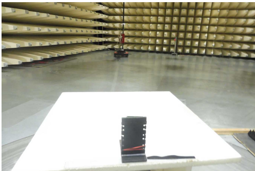
Photo 8 RSE < 1GHz
