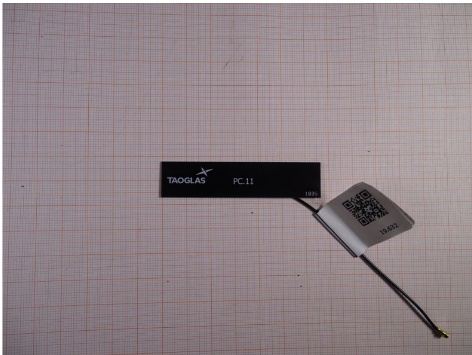
Photo 6: TAOGLAS PC11.07.0100A
