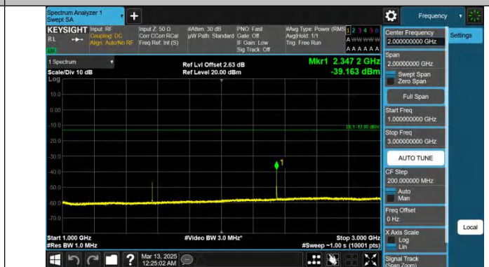
Band13-5MHz-QPSK-23255-1RB#0-1000~3000-PASS
