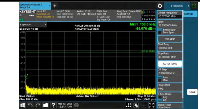
Band13-5MHz-QPSK-23255-1RB#0-0.15~30-PASS
