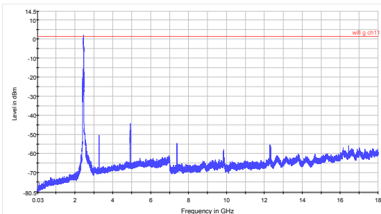
802.11g CH11 30MHz to 18GHz
