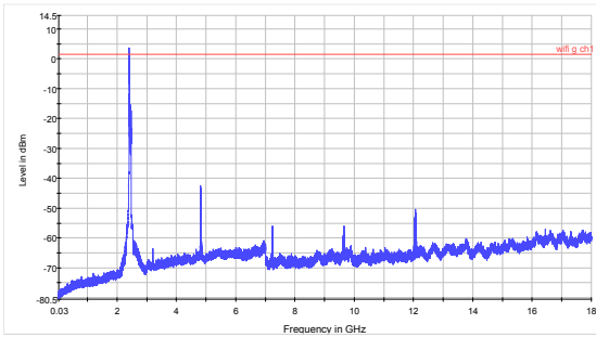
802.11g CH1 30MHz to 18GHz
