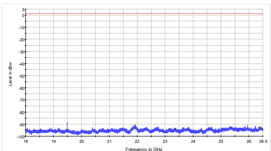
802.11g CH6 18GHz to 26.5GHz
