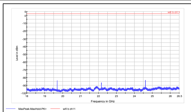
802.11b CH11 18GHz to 26.5GHz
