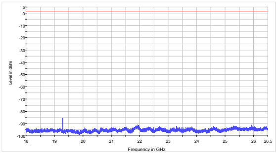
802.11g CH1 18GHz to 26.5GHz
