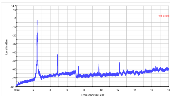
802.11g CH6 30MHz to 18GHz
