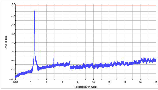
802.11n (HT20) CH11 30MHz to 18GHz
