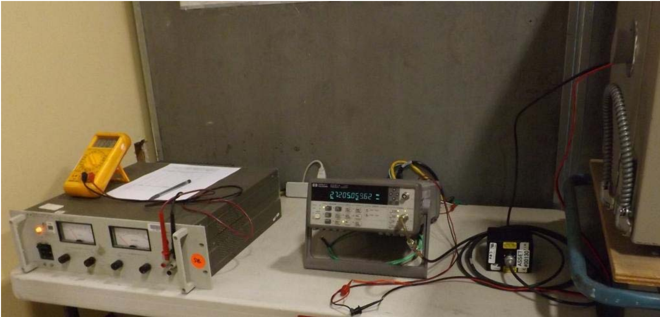
Figure E17.9 – Setup, Frequency Stability
