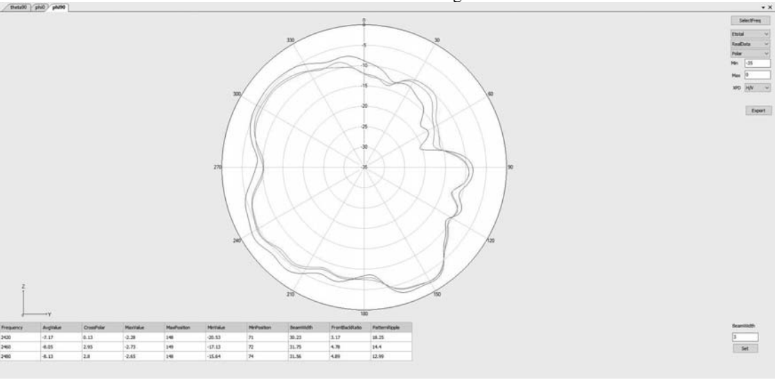
WiFi2.4 Phi=90deg
