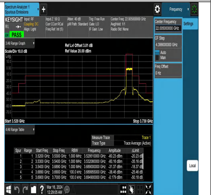
Band43_10MHz_QPSK_44540_50RB#0
