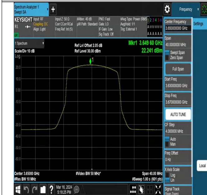
43(3600-3700)-20MHz-QPSK-44090-1RB#49-PASS
