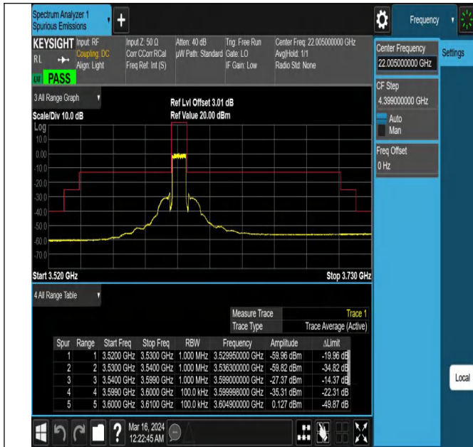
Band43_10MHz_QPSK_43640_50RB#0
