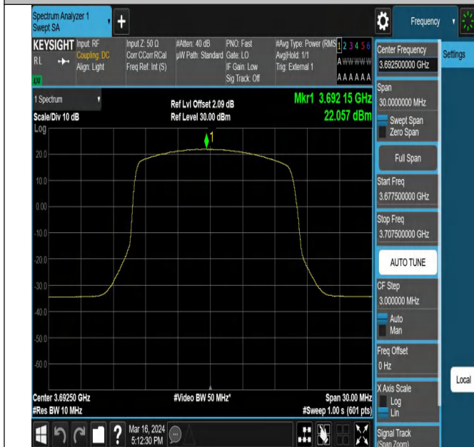
43(3600-3700)-15MHz-QPSK-44515-1RB#38-PASS
