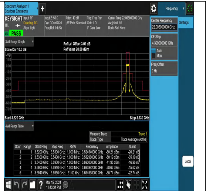
Band43_5MHz_QPSK_44565_25RB#0
