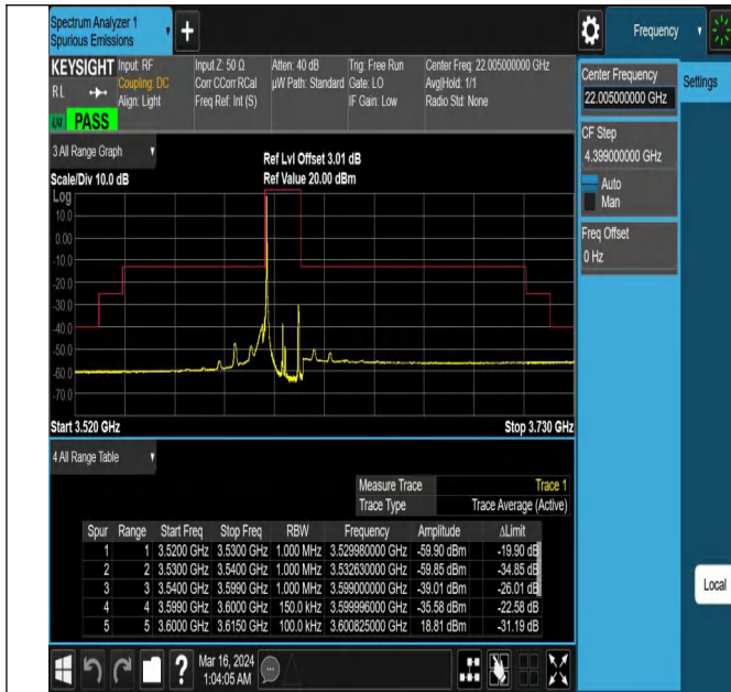
Band43_15MHz_QPSK_43665_1RB#0
