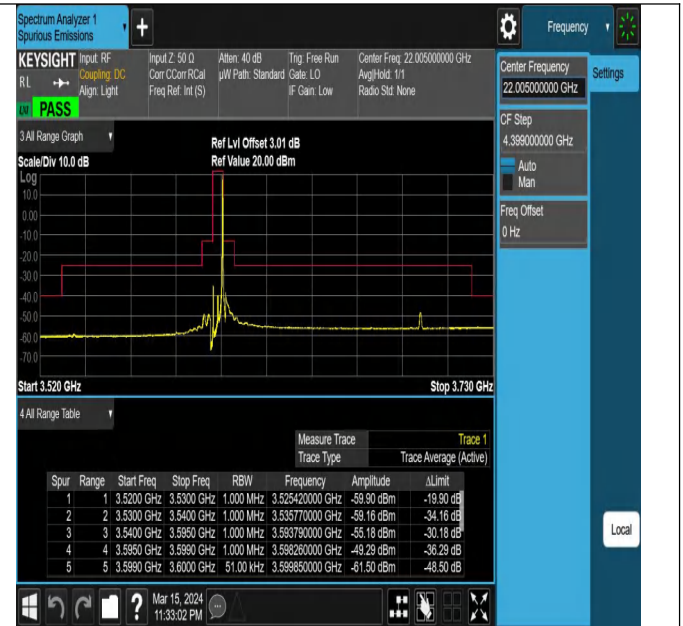
Band43_5MHz_QPSK_43615_1RB#24
