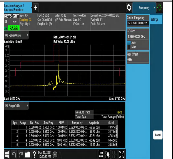
Band43_10MHz_QPSK_43640_1RB#49
