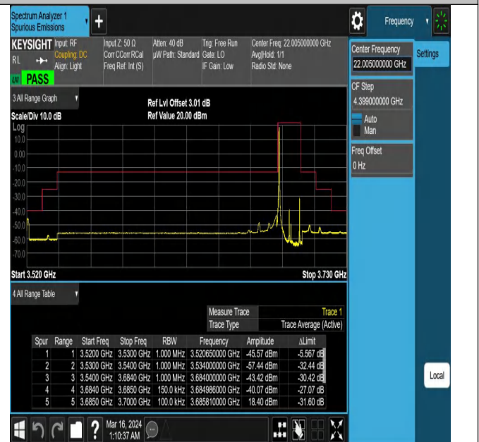
Band43_15MHz_QPSK_44515_1RB#0
