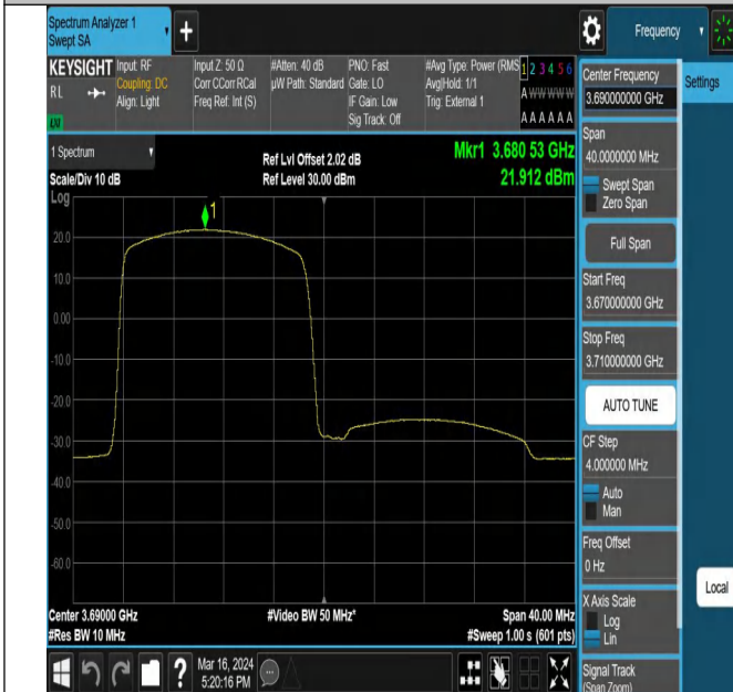
43(3600-3700)-20MHz-QPSK-44490-1RB#0-PASS
