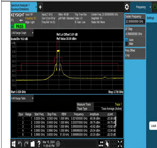
Band43_5MHz_QPSK_43615_25RB#0
