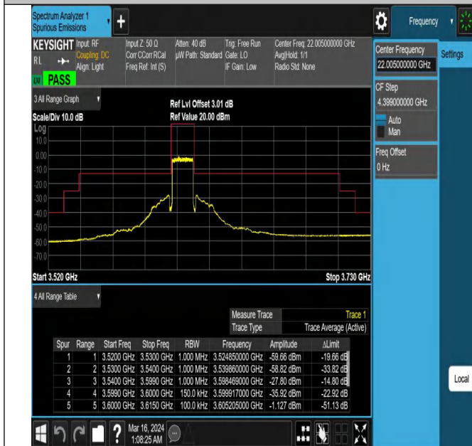
Band43_15MHz_QPSK_43665_75RB#0
