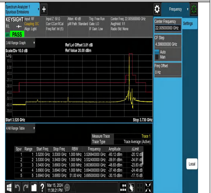
Band43_5MHz_QPSK_44565_1RB#0
