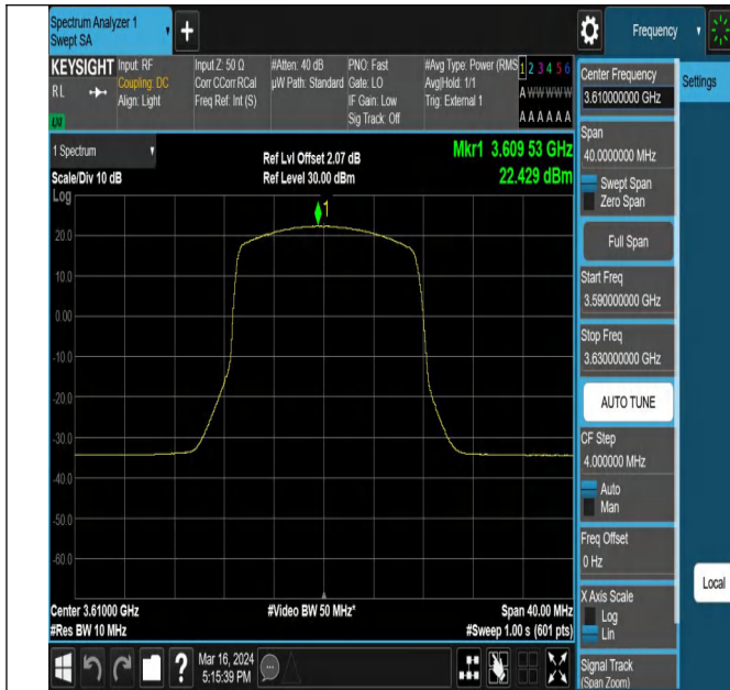
43(3600-3700)-20MHz-QPSK-43690-1RB#49-PASS
