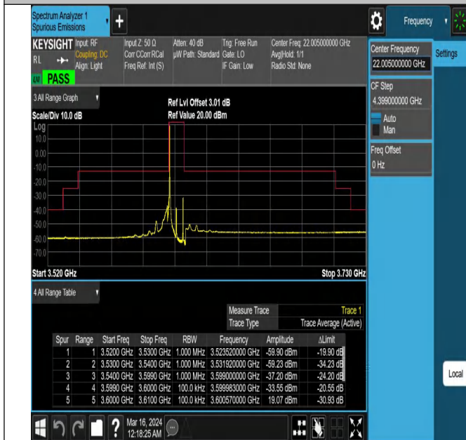
Band43_10MHz_QPSK_43640_1RB#0
