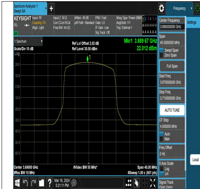
43(3600-3700)-20MHz-QPSK-44490-1RB#49-PASS
