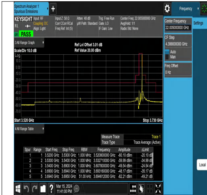
Band43_5MHz_QPSK_44565_1RB#24
