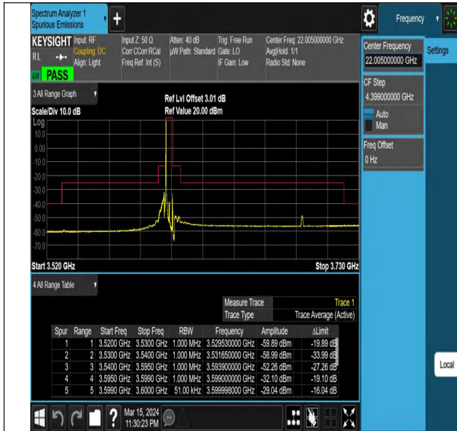
Band43_5MHz_QPSK_43615_1RB#0
