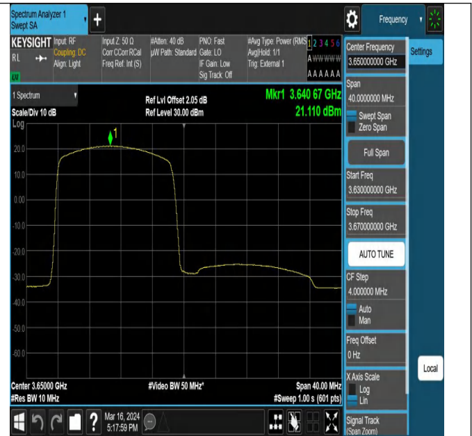
43(3600-3700)-20MHz-16QAM-44090-1RB#0-PASS
