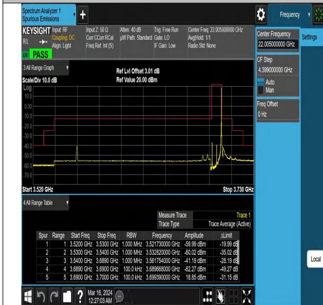
Band43_10MHz_QPSK_44540_1RB#49
