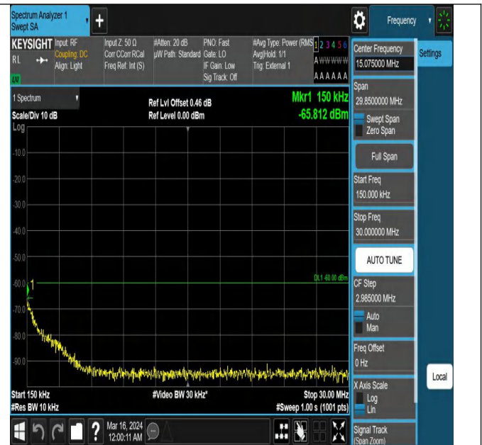
Band43_5MHz_QPSK_43615_1RB#0_0.15~30_0.15~30
