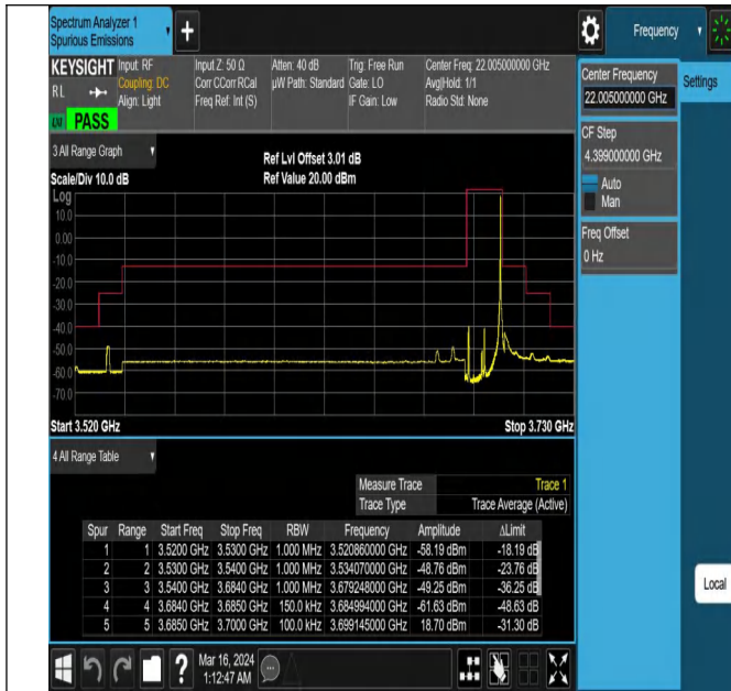
Band43_15MHz_QPSK_44515_1RB#74
