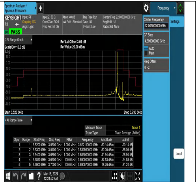
Band43_10MHz_QPSK_44540_1RB#0
