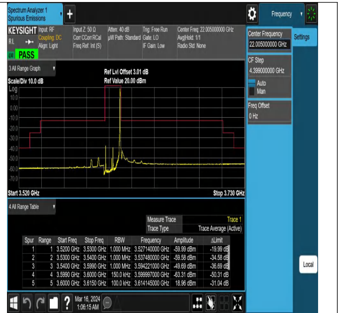
Band43_15MHz_QPSK_43665_1RB#74
