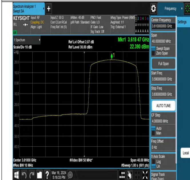
43(3600-3700)-20MHz-QPSK-43690-1RB#99-PASS
