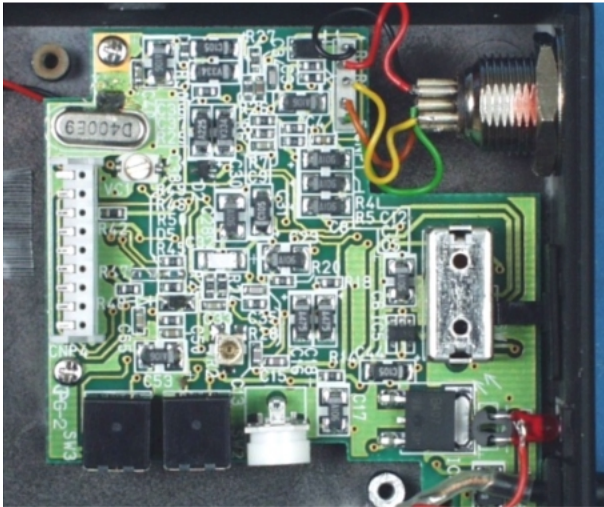
Interior (Audio Top)
