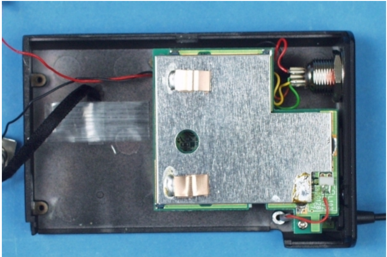
Interior (RF Top)
