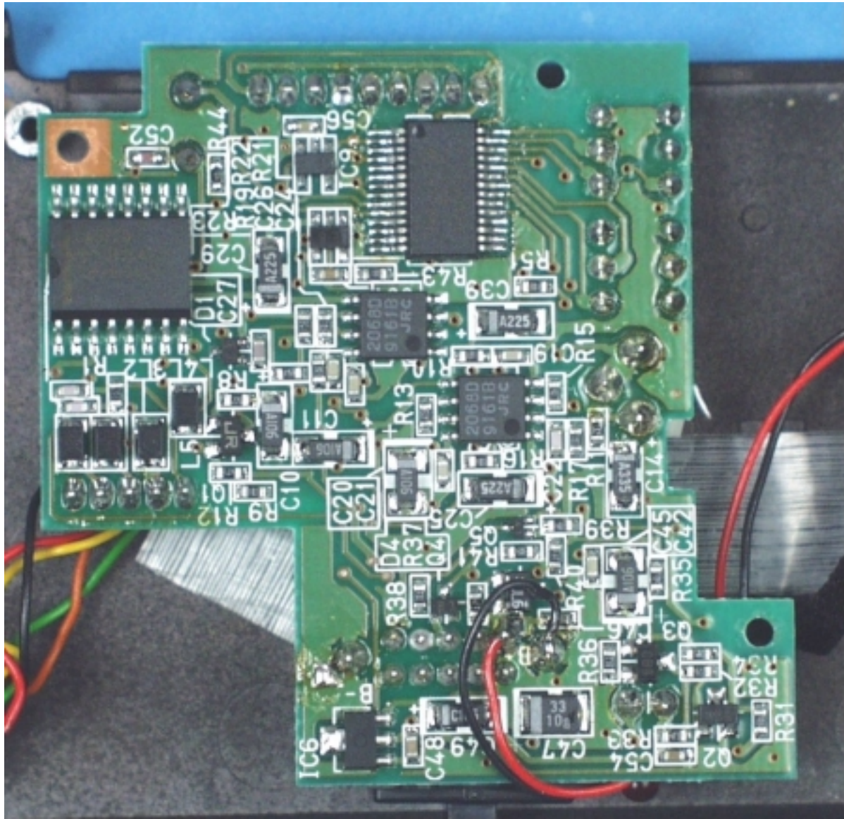
Interior (Audio Back)
