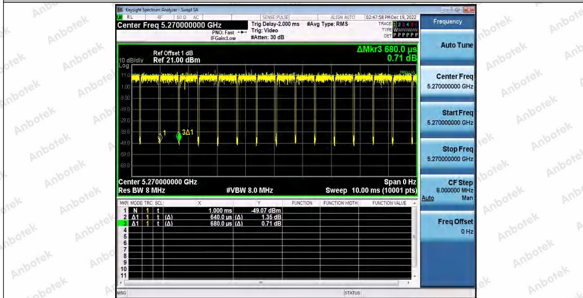
11AC40SISO_Ant2_5270
