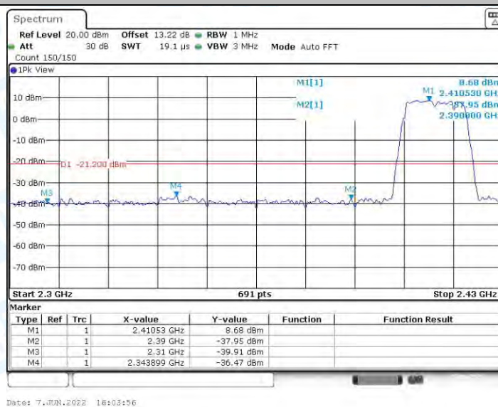
11G_Ant2_Low_2412_Peak
