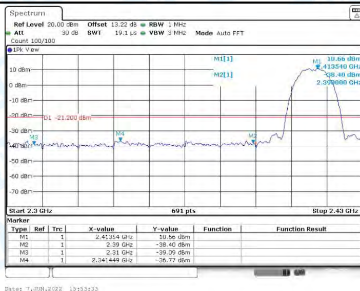
11B_Ant2_Low_2412_Peak
