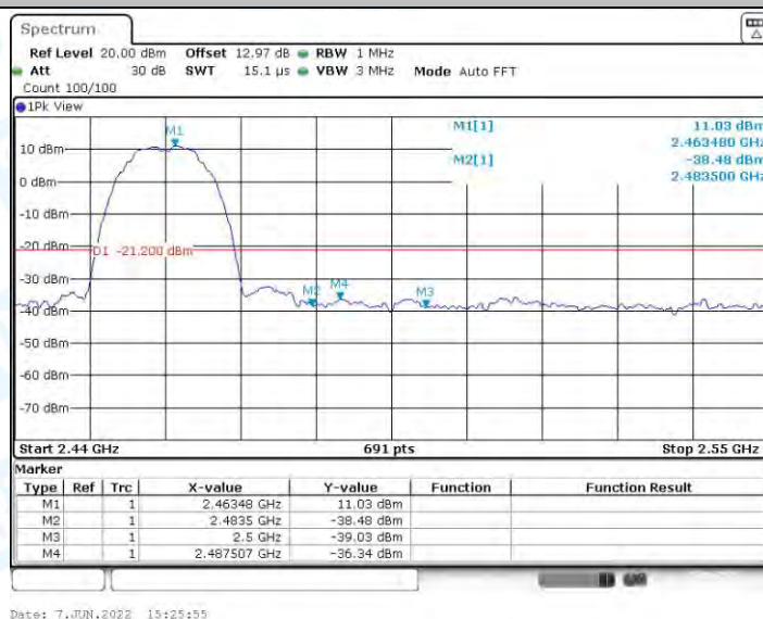
11B_Ant1_High_2462_Peak
