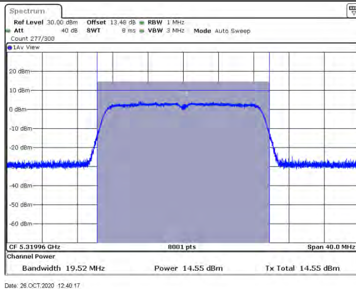
11AC20SISO_Ant2_5320
