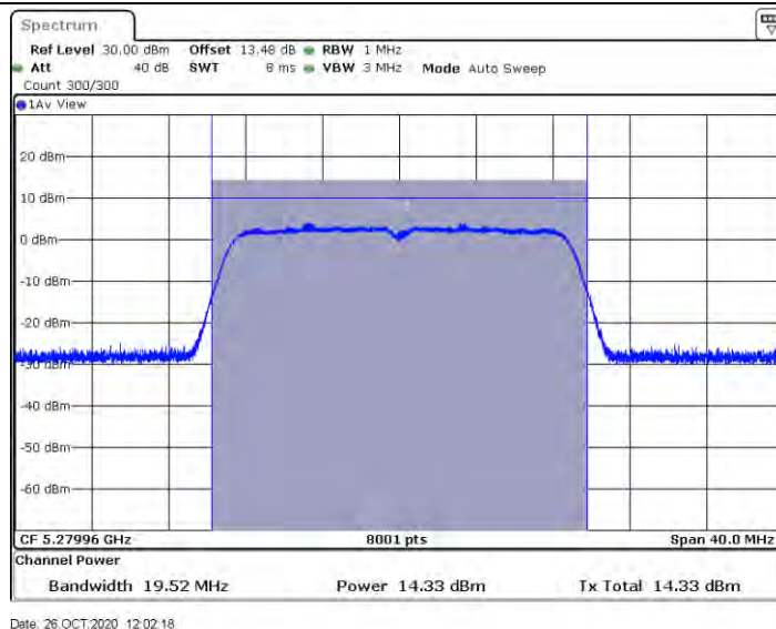
11AC20SISO_Ant2_5280
