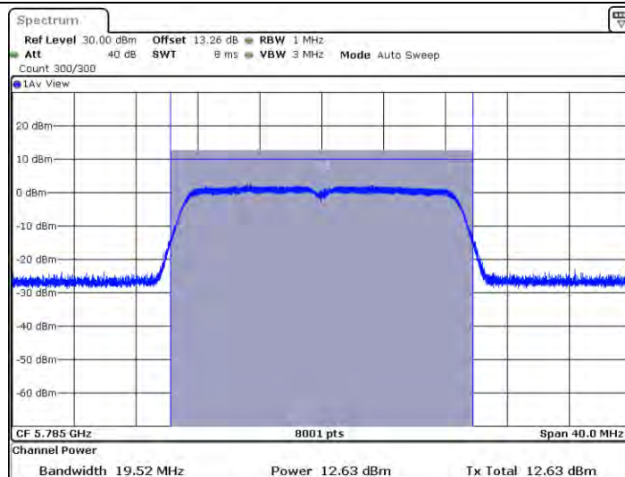
11AC20SISO_Ant2_5785
