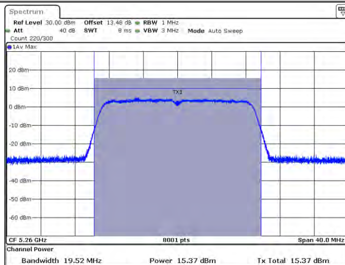
11AC20SISO_Ant2_5260
