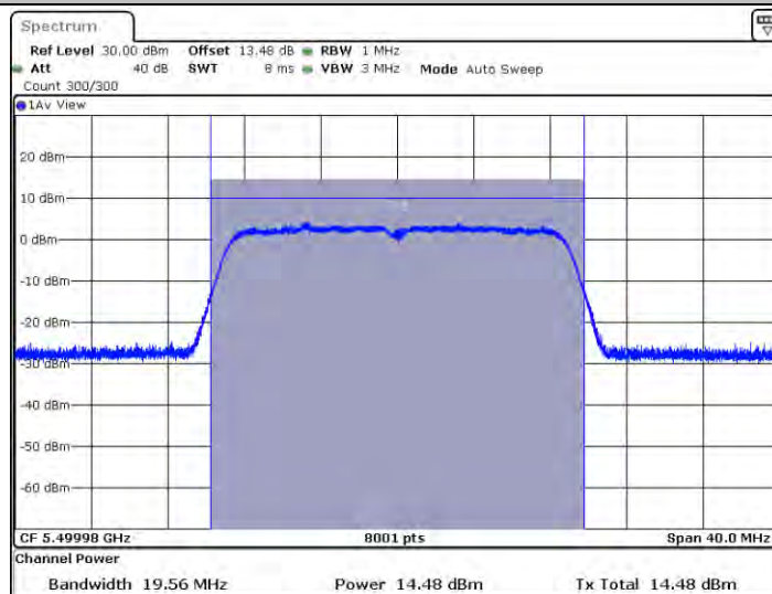
11AC20SISO_Ant2_5500
