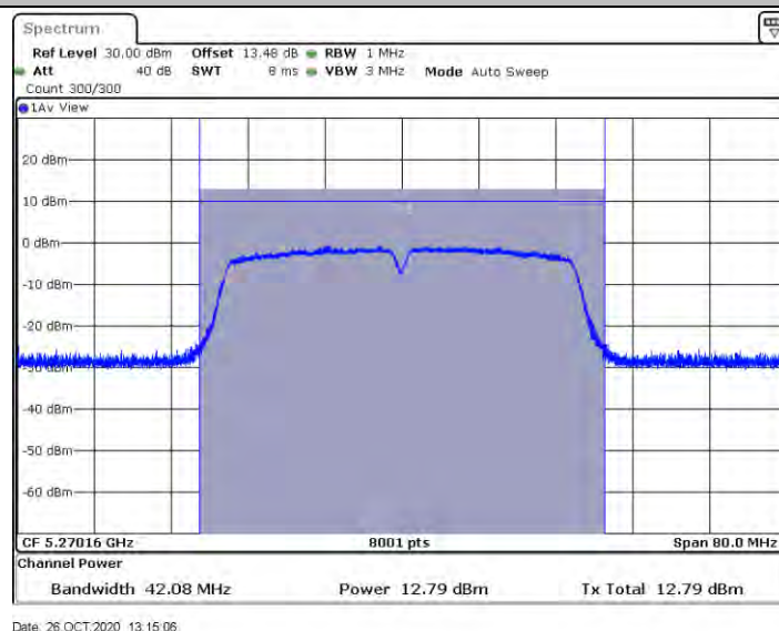
11AC40SISO_Ant2_5270
