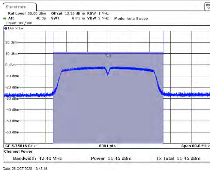
11AC40SISO_Ant2_5755
