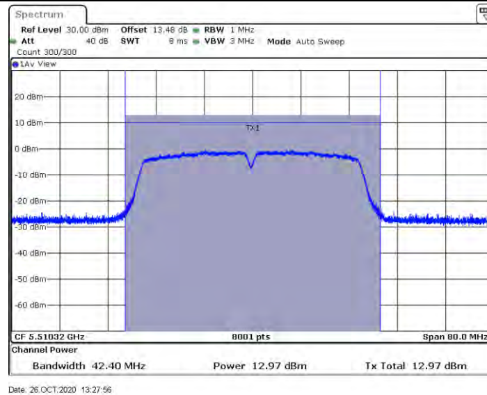
11AC40SISO_Ant2_5510
