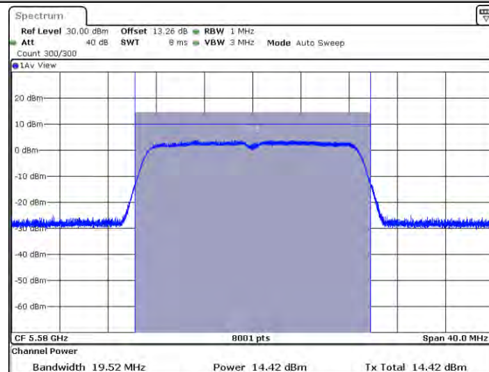
11AC20SISO_Ant2_5580
