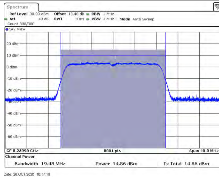
11N20SISO_Ant2_5260
