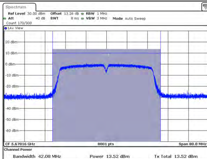
11AC40SISO_Ant2_5670
