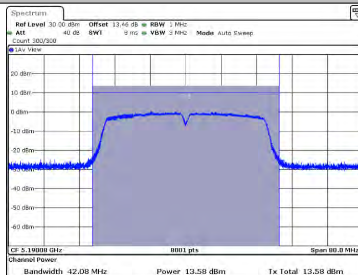
11AC40SISO_Ant2_5190
