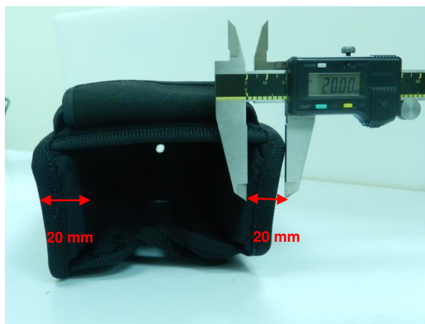
Pistol Holster(Model Name: WA6083)_ RF exposure configuration Right Side 20mm /Left Side 20mm
