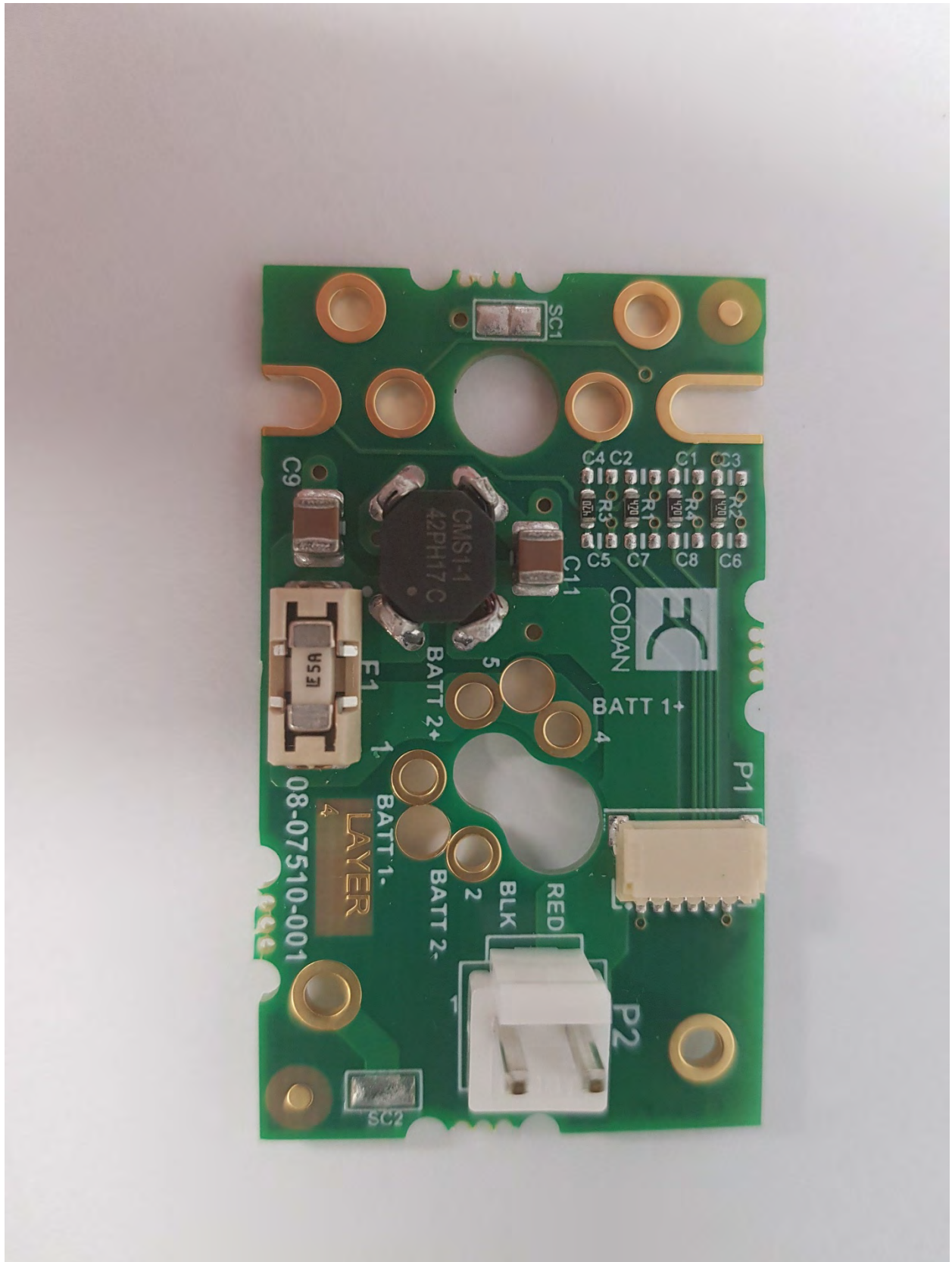
REAR PANEL PCB 08-07510 – 001 – SIDE 1
