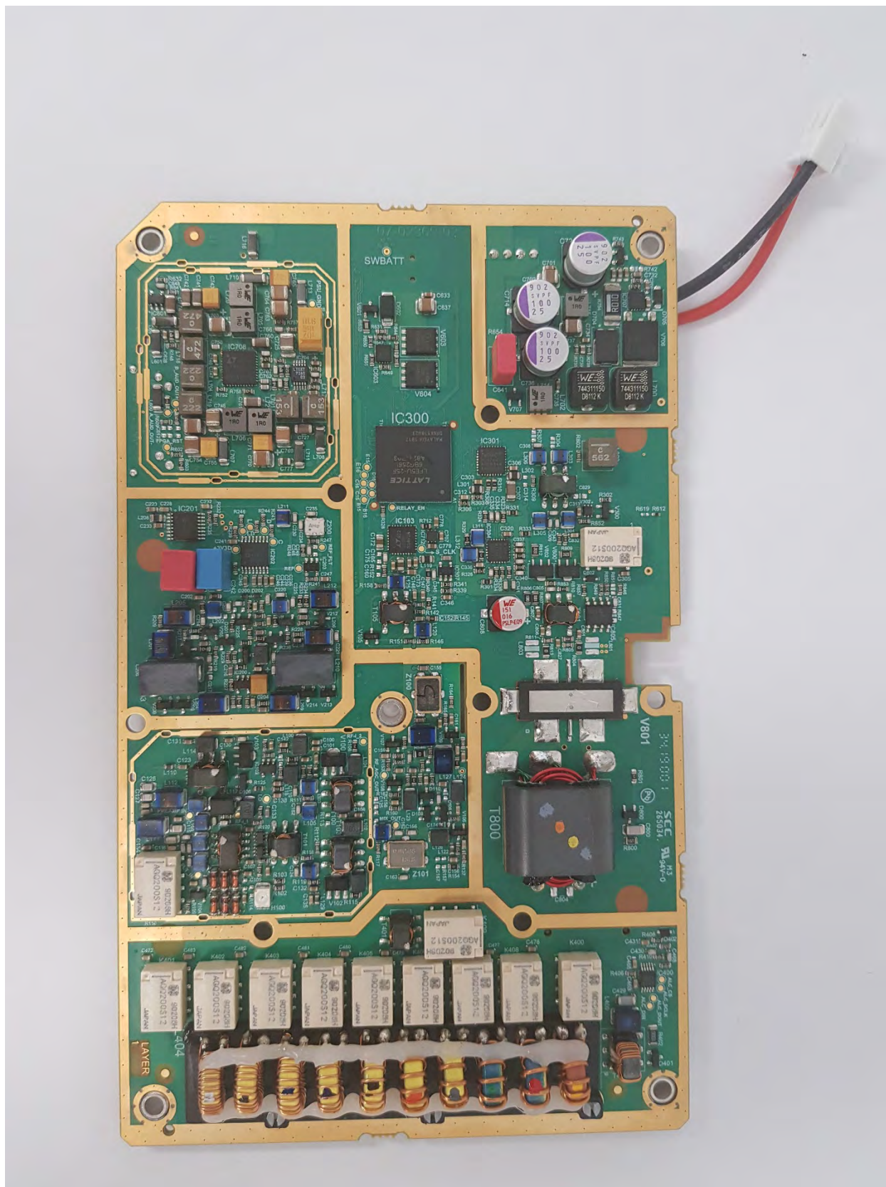
RF PCB 08-07506-001 – SIDE 1 WITHOUT SHIELDS
