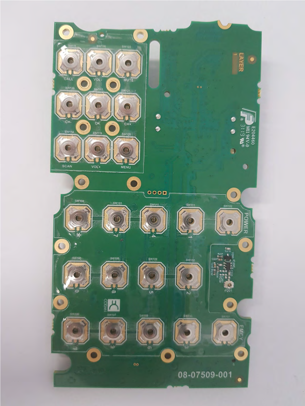
FRONT PANEL PCB 08-07509-001 – SIDE 2
