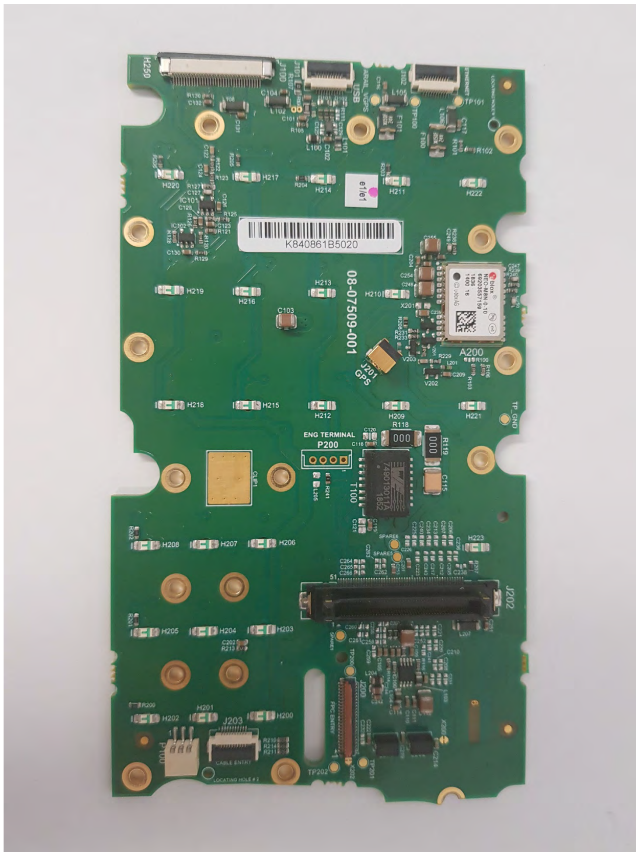
FRONT PANEL PCB 08-07509-001 – Side 1
