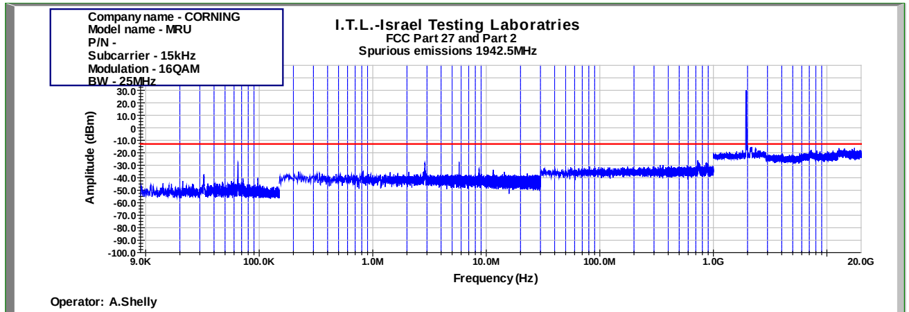
Figure 834: Spurious Emissions at Antenna Terminal 16QAM 25MHz B.W.; 1942.5MHz, 15kHz
