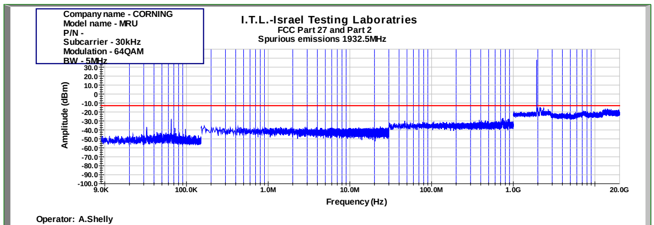
Figure 868: Spurious Emissions at Antenna Terminal 64QAM 5MHz B.W.; 1932.5MHz, 30kHz
