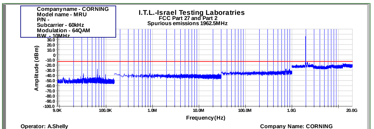
Figure 878: Spurious Emissions at Antenna Terminal 64QAM 10MHz B.W.; 1962.5MHz, 60kHz
