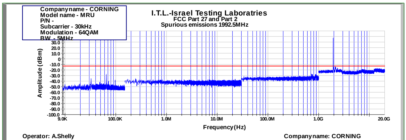
Figure 872: Spurious Emissions at Antenna Terminal 64QAM 5MHz B.W.; 1992.5MHz, 30kHz
