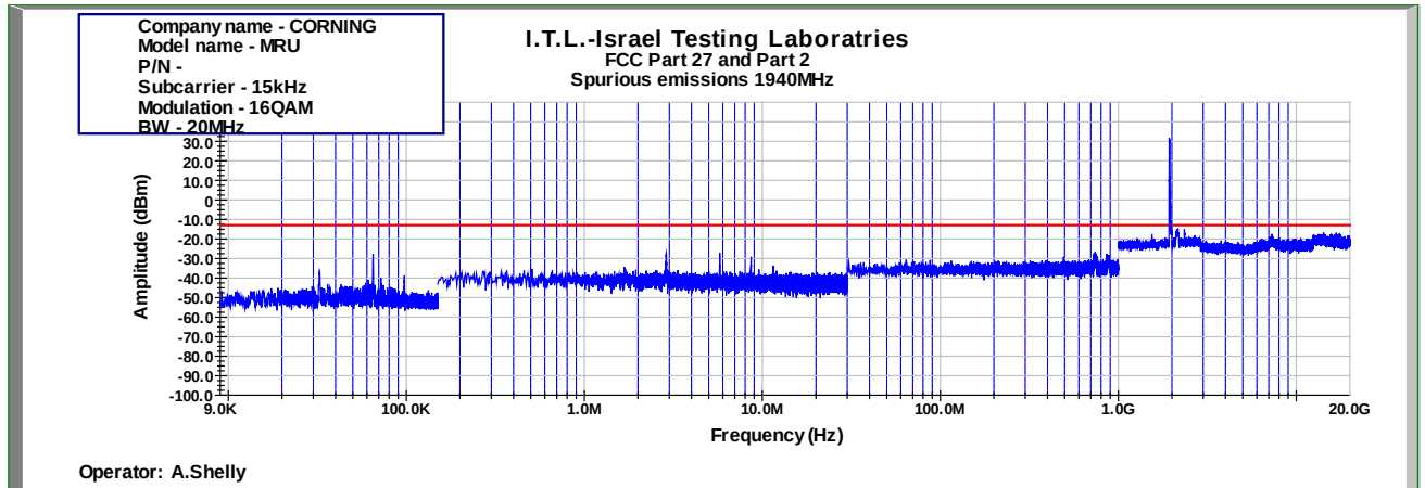
Figure 825: Spurious Emissions at Antenna Terminal 16QAM 20MHz B.W.; 1940.0MHz, 15kHz
