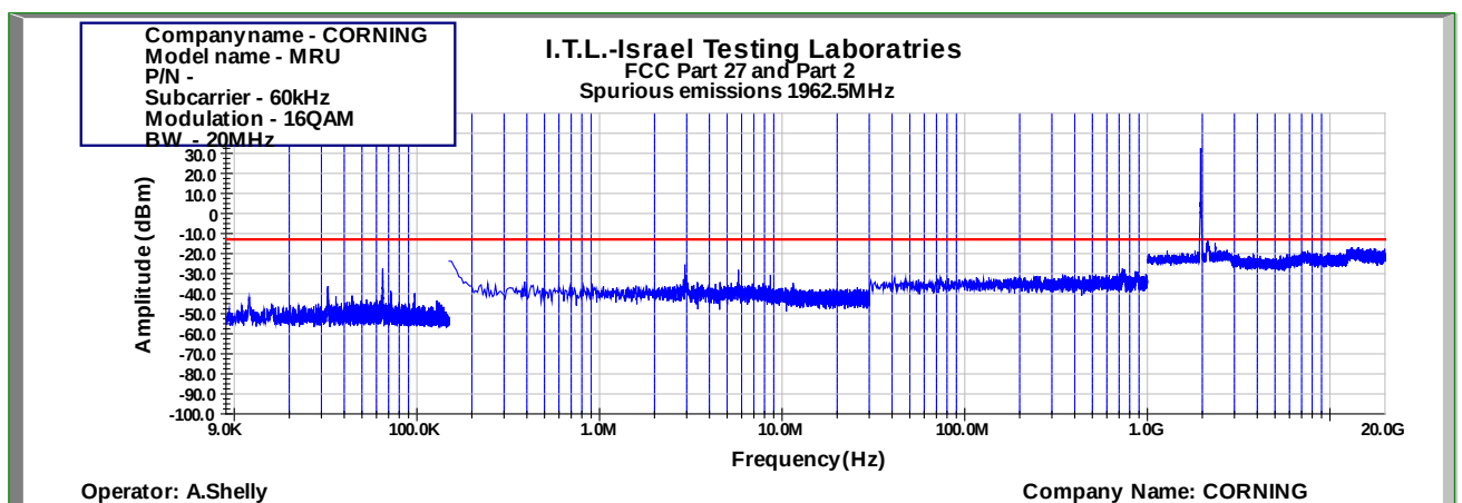
Figure 830: Spurious Emissions at Antenna Terminal 16QAM 20MHz B.W.; 1962.5MHz, 60kHz
