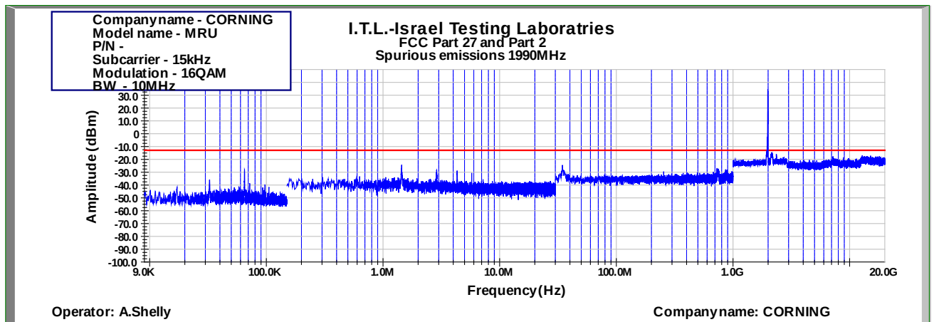
Figure 813: Spurious Emissions at Antenna Terminal 16QAM 10MHz B.W.; 1990.0MHz, 15kHz
