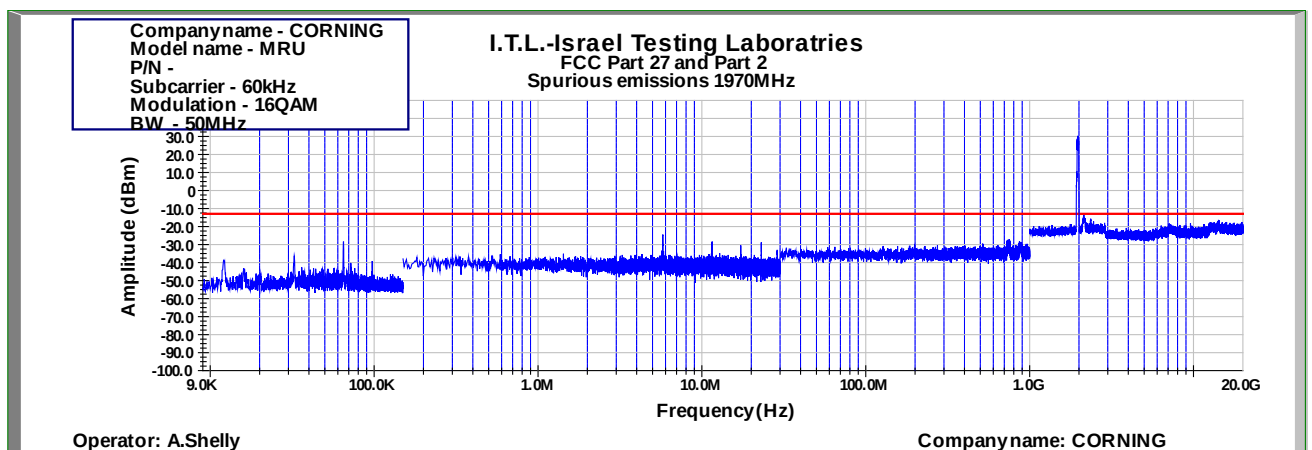
Figure 860: Spurious Emissions at Antenna Terminal 16QAM 50MHz B.W.; 1970.0MHz, 60kHz
