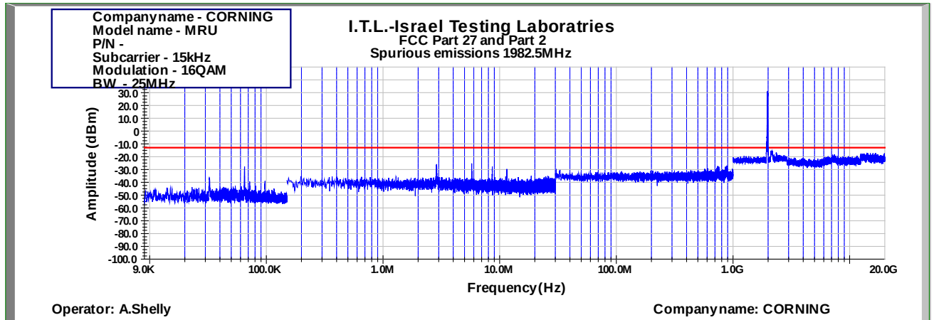
Figure 840: Spurious Emissions at Antenna Terminal 16QAM 25MHz B.W.; 1982.5MHz, 15kHz
