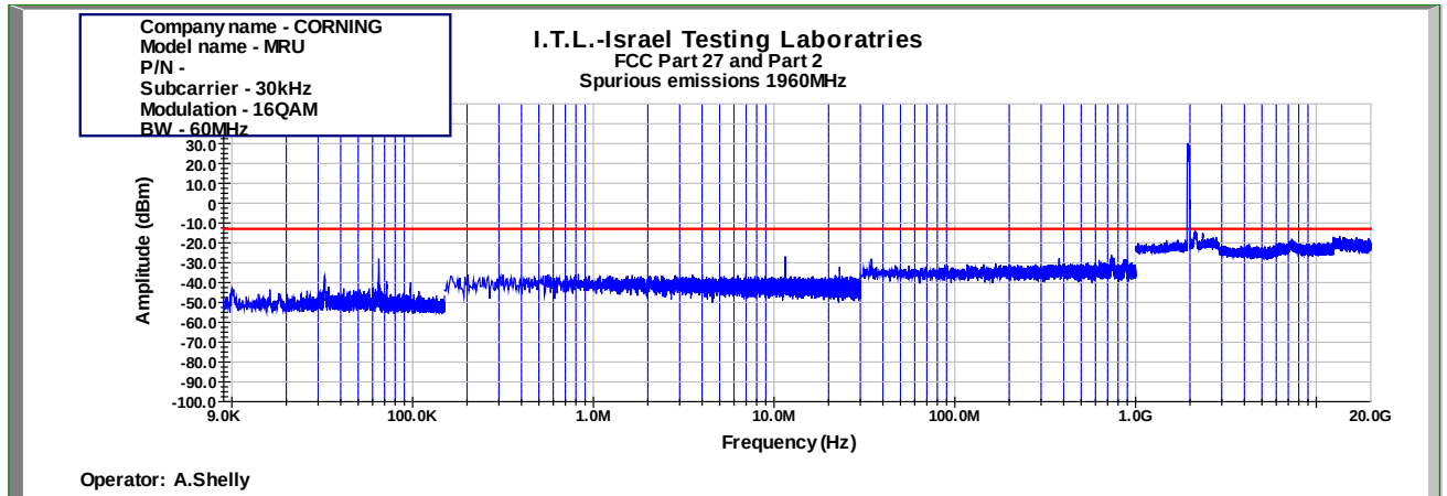
Figure 861: Spurious Emissions at Antenna Terminal 16QAM 60MHz B.W.; 1960.0MHz, 30kHz
