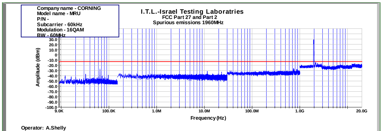
Figure 862: Spurious Emissions at Antenna Terminal 16QAM 60MHz B.W.; 1960.0MHz, 60kHz
