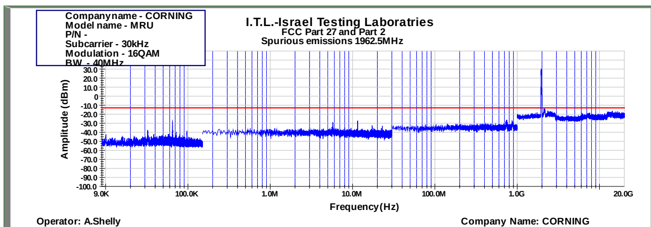
Figure 847: Spurious Emissions at Antenna Terminal 16QAM 40MHz B.W.; 1962.5MHz, 30kHz
