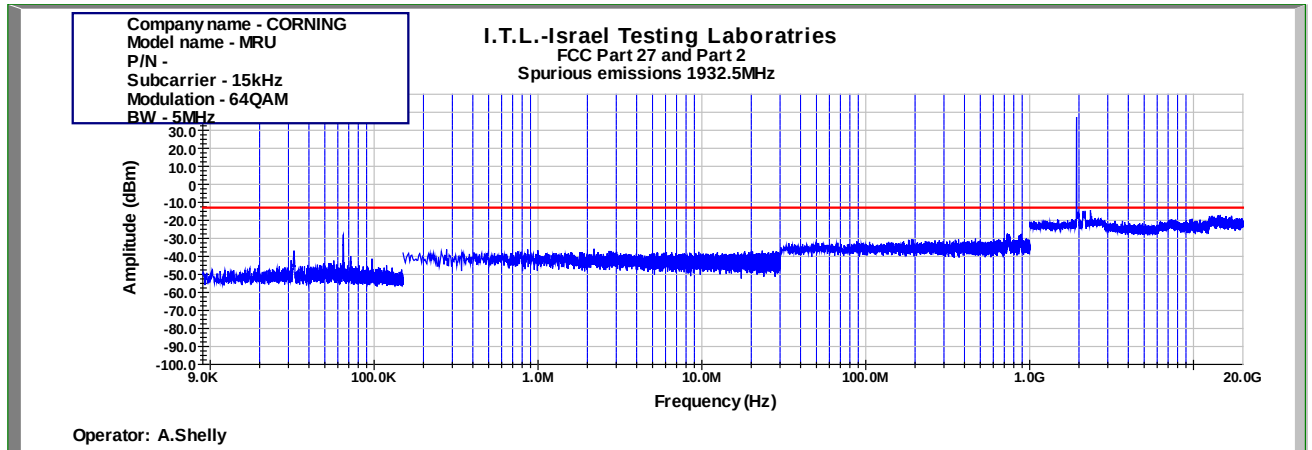
Figure 867: Spurious Emissions at Antenna Terminal 64QAM 5MHz B.W.; 1932.5MHz, 15kHz
