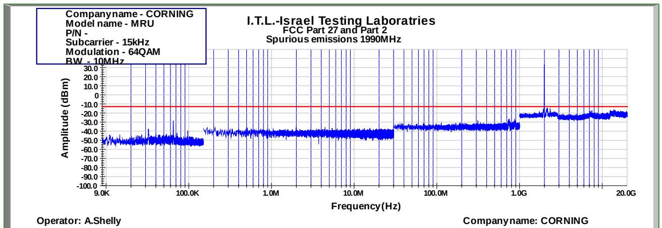
Figure 879: Spurious Emissions at Antenna Terminal 64QAM 10MHz B.W.; 1990.0MHz, 15kHz
