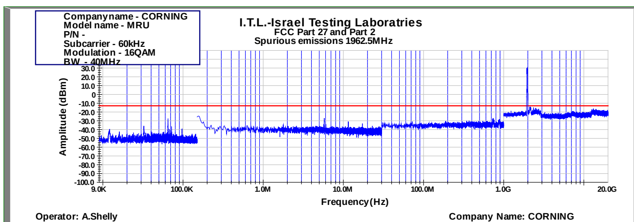
Figure 848: Spurious Emissions at Antenna Terminal 16QAM 40MHz B.W.; 1962.5MHz, 60kHz
