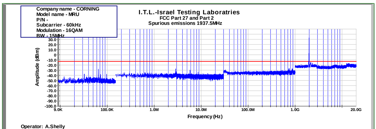
Figure 818: Spurious Emissions at Antenna Terminal 16QAM 15MHz B.W.; 1937.5MHz, 60kHz
