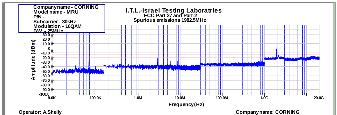
Figure 841: Spurious Emissions at Antenna Terminal 16QAM 25MHz B.W.; 1982.5MHz, 30kHz
