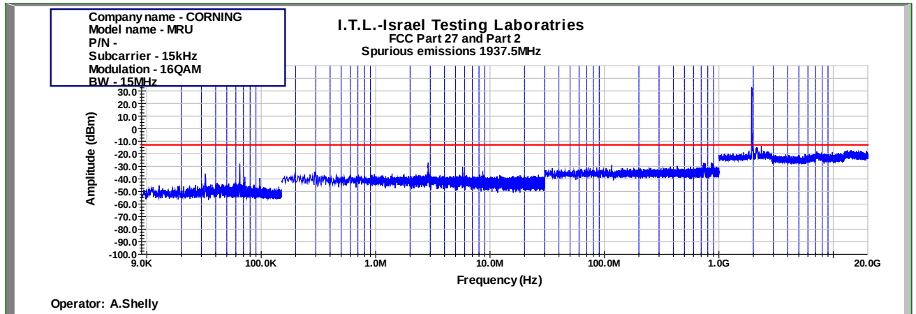
Figure 816: Spurious Emissions at Antenna Terminal 16QAM 15MHz B.W.; 1937.5MHz, 15kHz
