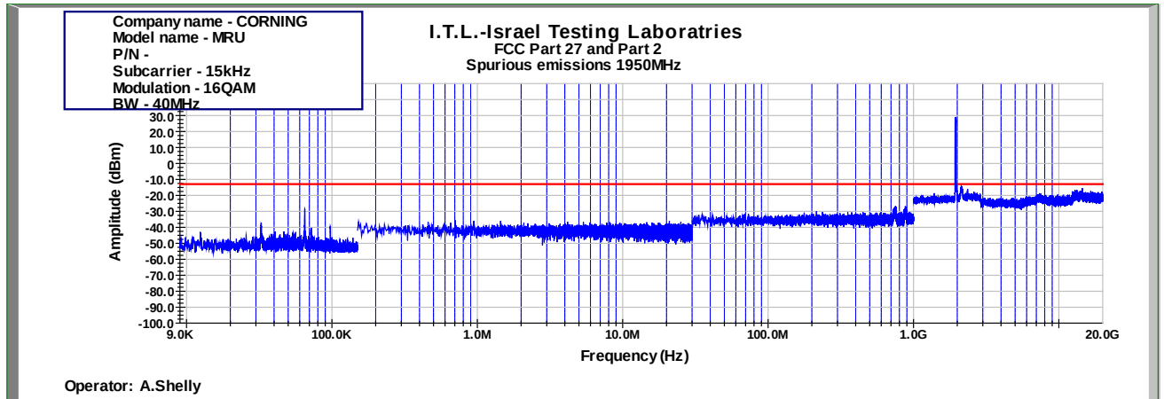
Figure 843: Spurious Emissions at Antenna Terminal 16QAM 40MHz B.W.; 1950.0MHz, 15kHz
