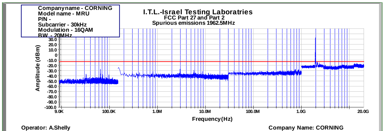
Figure 829: Spurious Emissions at Antenna Terminal 16QAM 20MHz B.W.; 1962.5MHz, 30kHz
