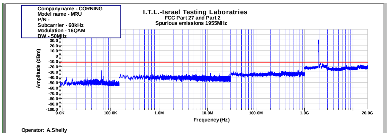
Figure 854: Spurious Emissions at Antenna Terminal 16QAM 50MHz B.W.; 1955.0MHz, 60kHz
