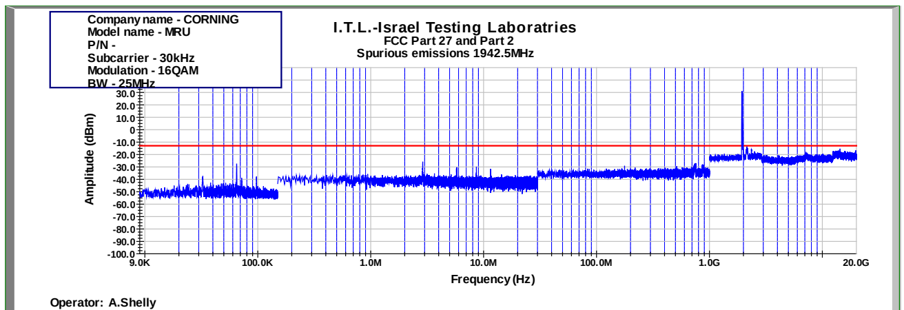
Figure 835: Spurious Emissions at Antenna Terminal 16QAM 25MHz B.W.; 1942.5MHz, 30kHz
