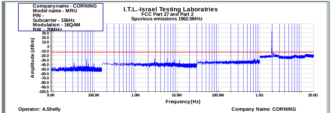
Figure 828: Spurious Emissions at Antenna Terminal 16QAM 20MHz B.W.; 1962.5MHz, 15kHz
