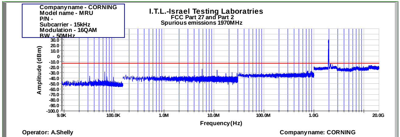
Figure 858: Spurious Emissions at Antenna Terminal 16QAM 50MHz B.W.; 1970.0MHz, 15kHz
