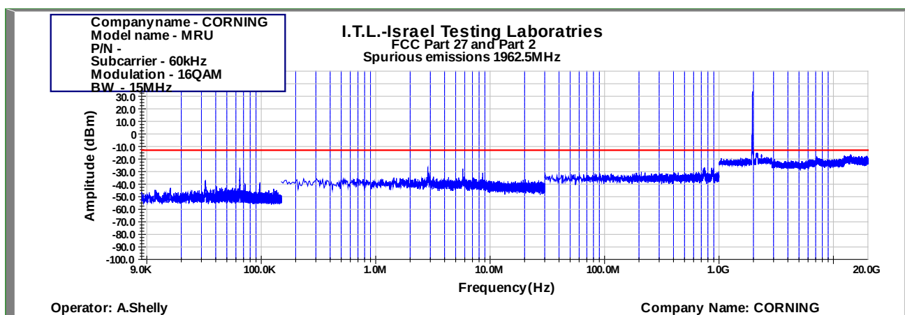
Figure 821: Spurious Emissions at Antenna Terminal 16QAM 15MHz B.W.; 1962.5MHz, 60kHz
