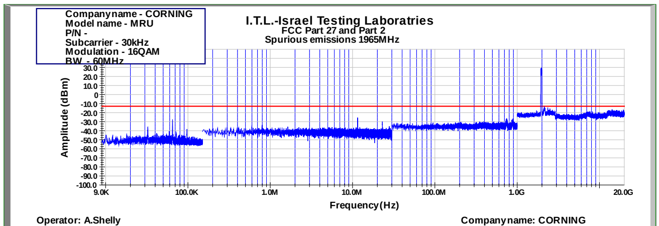
Figure 865: Spurious Emissions at Antenna Terminal 16QAM 60MHz B.W.; 1965.0MHz, 30kHz
