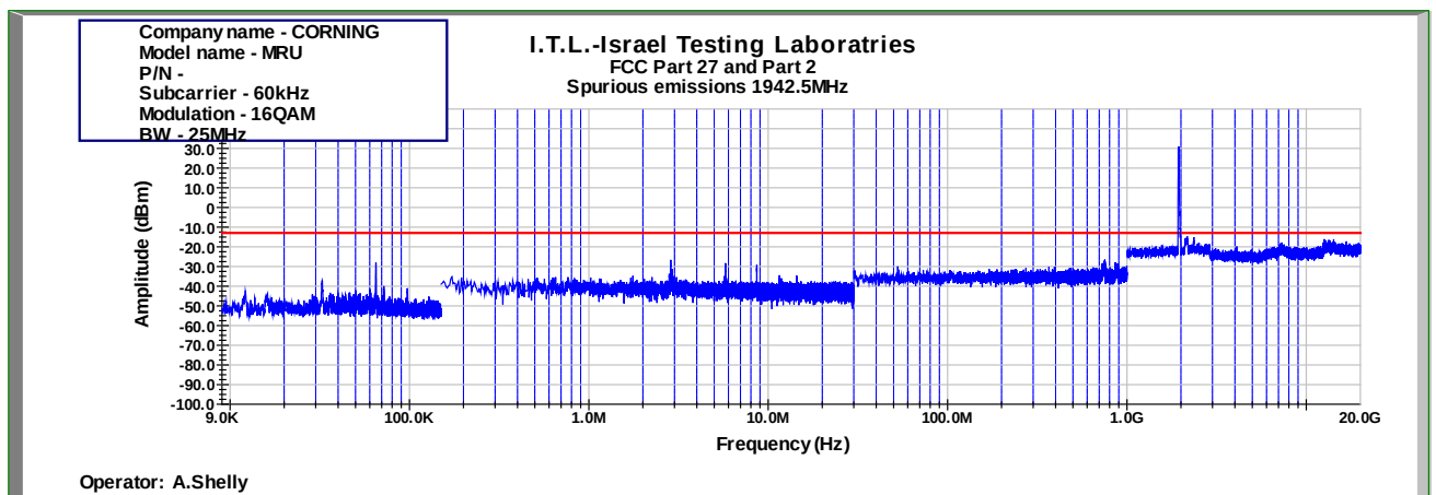
Figure 836: Spurious Emissions at Antenna Terminal 16QAM 25MHz B.W.; 1942.5MHz, 60kHz
