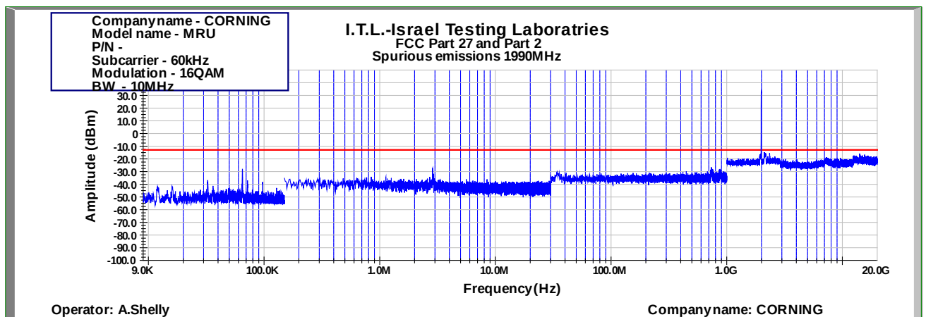
Figure 815: Spurious Emissions at Antenna Terminal 16QAM 10MHz B.W.; 1990.0MHz, 60kHz
