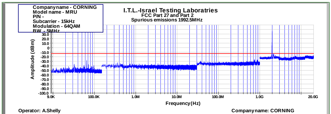
Figure 871: Spurious Emissions at Antenna Terminal 64QAM 5MHz B.W.; 1992.5MHz, 15kHz
