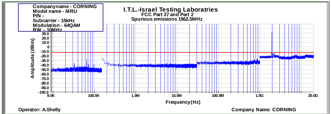
Figure 876: Spurious Emissions at Antenna Terminal 64QAM 10MHz B.W.; 1962.5MHz, 15kHz
