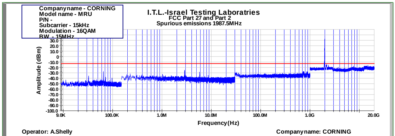
Figure 822: Spurious Emissions at Antenna Terminal 16QAM 15MHz B.W.; 1987.5MHz, 15kHz
