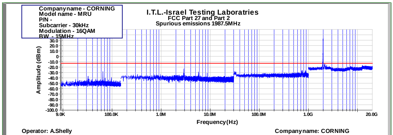
Figure 823: Spurious Emissions at Antenna Terminal 16QAM 15MHz B.W.; 1987.5MHz, 30kHz
