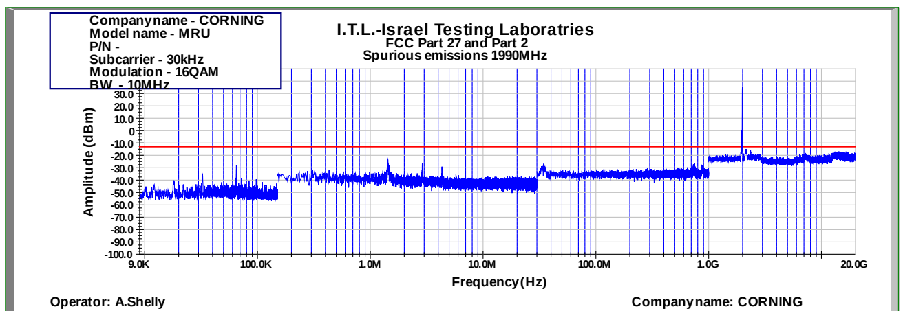
Figure 814: Spurious Emissions at Antenna Terminal 16QAM 10MHz B.W.; 1990.0MHz, 30kHz
