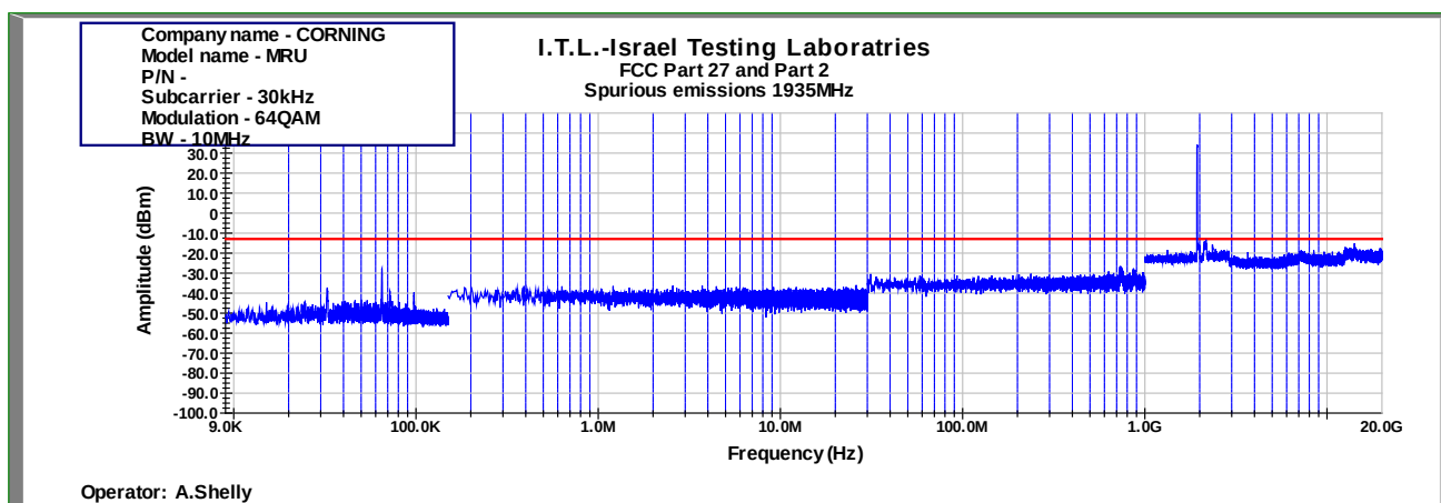
Figure 874: Spurious Emissions at Antenna Terminal 64QAM 10MHz B.W.; 1935.00MHz, 30kHz
