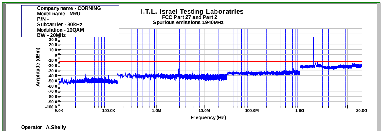
Figure 826: Spurious Emissions at Antenna Terminal 16QAM 20MHz B.W.; 1940.0MHz, 30kHz
