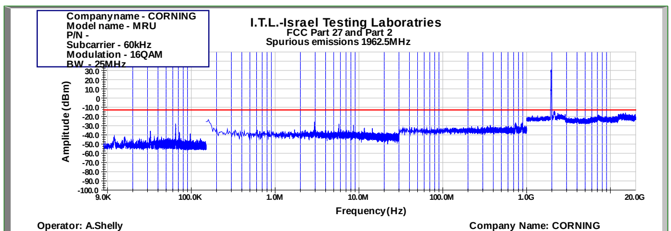
Figure 839: Spurious Emissions at Antenna Terminal 16QAM 25MHz B.W.; 1962.5MHz, 60kHz
