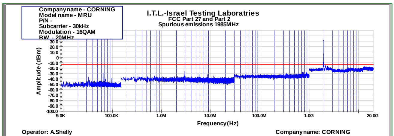
Figure 832: Spurious Emissions at Antenna Terminal 16QAM 20MHz B.W.; 1985.0MHz, 30kHz
