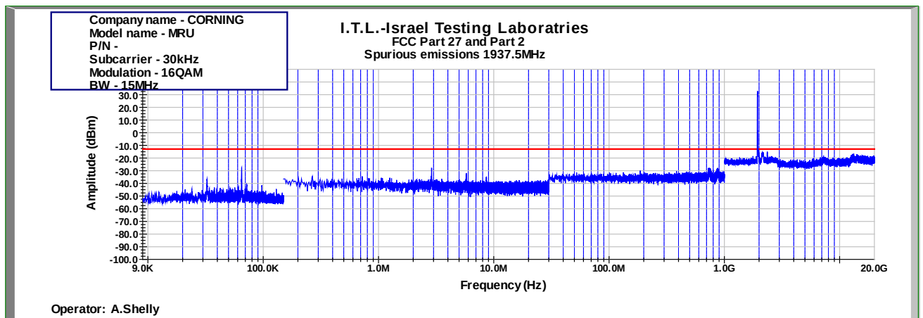
Figure 817: Spurious Emissions at Antenna Terminal 16QAM 15MHz B.W.; 1937.5MHz, 30kHz
