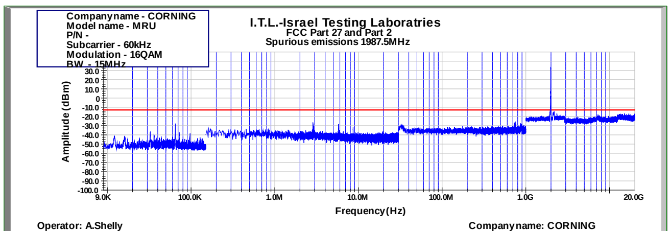
Figure 824: Spurious Emissions at Antenna Terminal 16QAM 15MHz B.W.; 1987.5MHz, 60kHz
