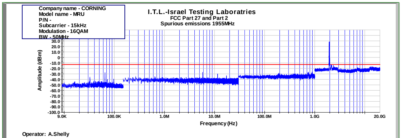
Figure 852: Spurious Emissions at Antenna Terminal 16QAM 50MHz B.W.; 1955.0MHz, 15kHz
