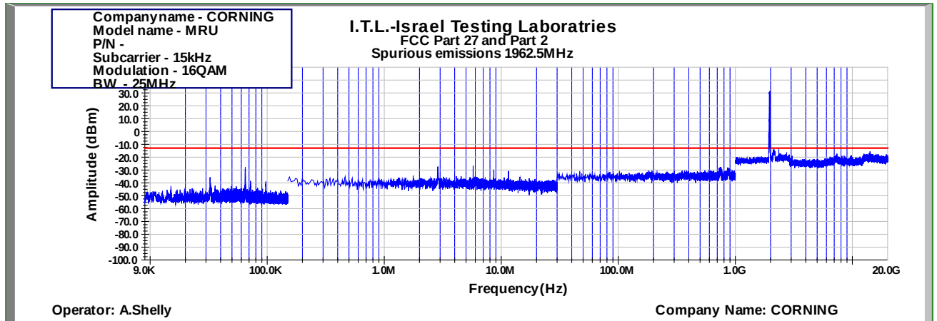
Figure 837: Spurious Emissions at Antenna Terminal 16QAM 25MHz B.W.; 1962.5MHz, 15kHz
