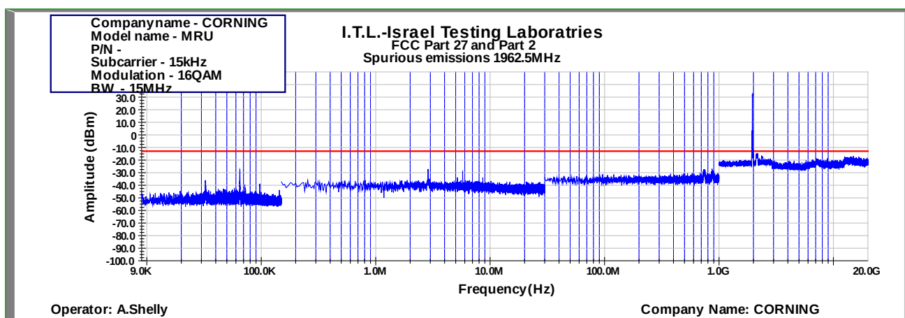
Figure 819: Spurious Emissions at Antenna Terminal 16QAM 15MHz B.W.; 1962.5MHz, 15kHz
