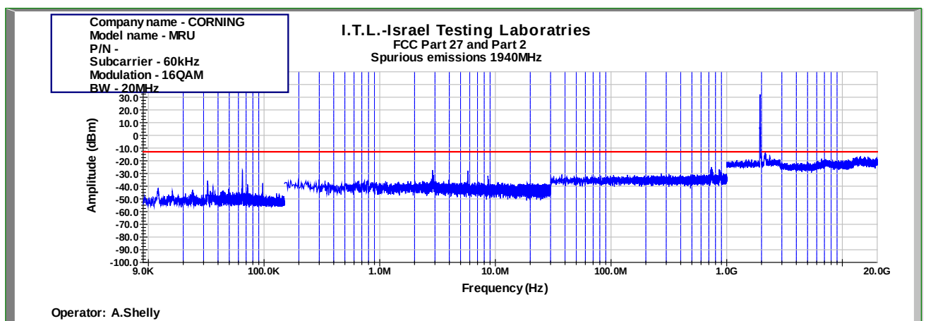
Figure 827: Spurious Emissions at Antenna Terminal 16QAM 20MHz B.W.; 1940.0MHz, 60kHz
