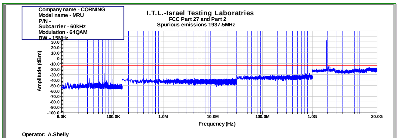
Figure 884: Spurious Emissions at Antenna Terminal 64QAM 15MHz B.W.; 1937.5MHz, 60kHz
