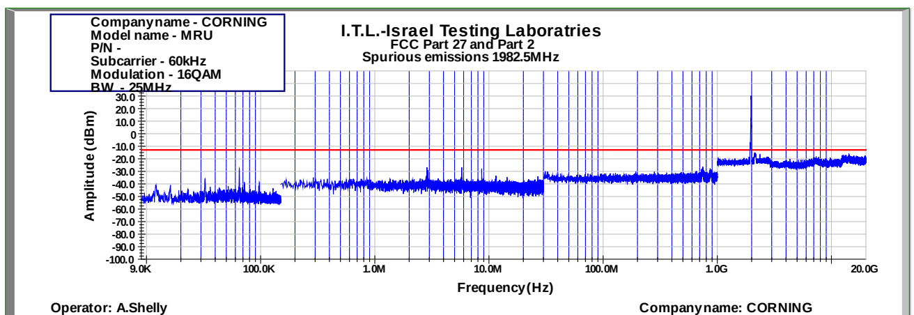
Figure 842: Spurious Emissions at Antenna Terminal 16QAM 25MHz B.W.; 1982.5MHz, 60kHz
