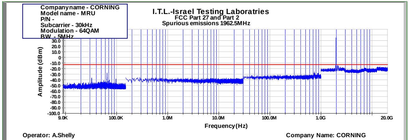
Figure 870: Spurious Emissions at Antenna Terminal 64QAM 5MHz B.W.; 1962.5MHz, 30kHz
