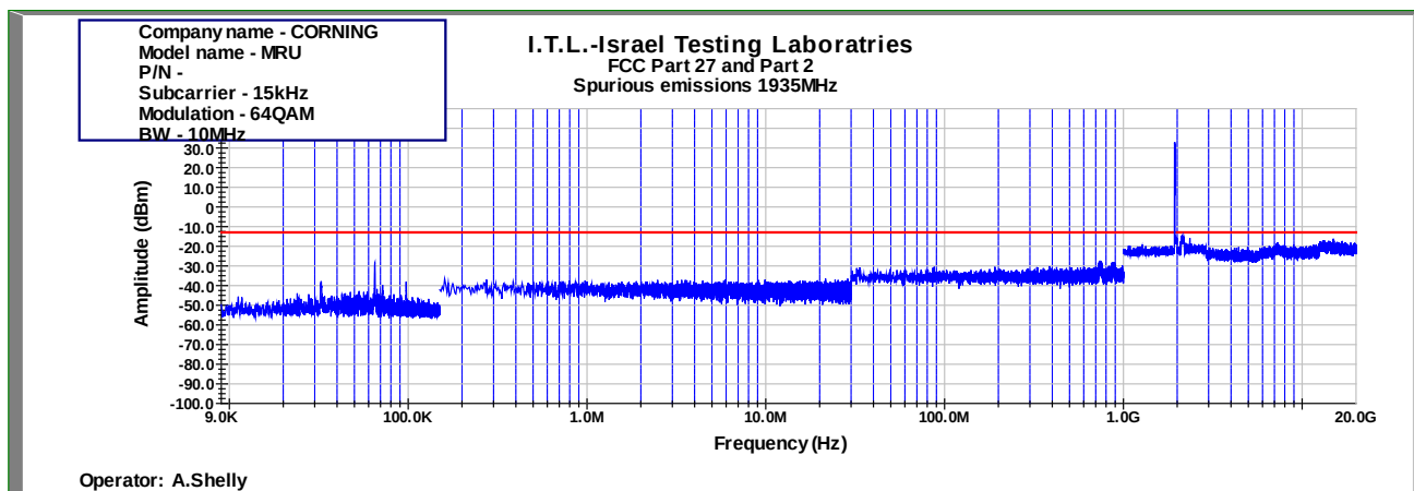
Figure 873: Spurious Emissions at Antenna Terminal 64QAM 10MHz B.W.; 1935.00MHz, 15kHz
