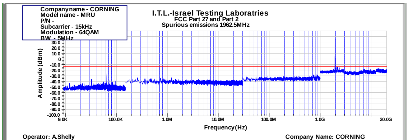
Figure 869: Spurious Emissions at Antenna Terminal 64QAM 5MHz B.W.; 1962.5MHz, 15kHz
