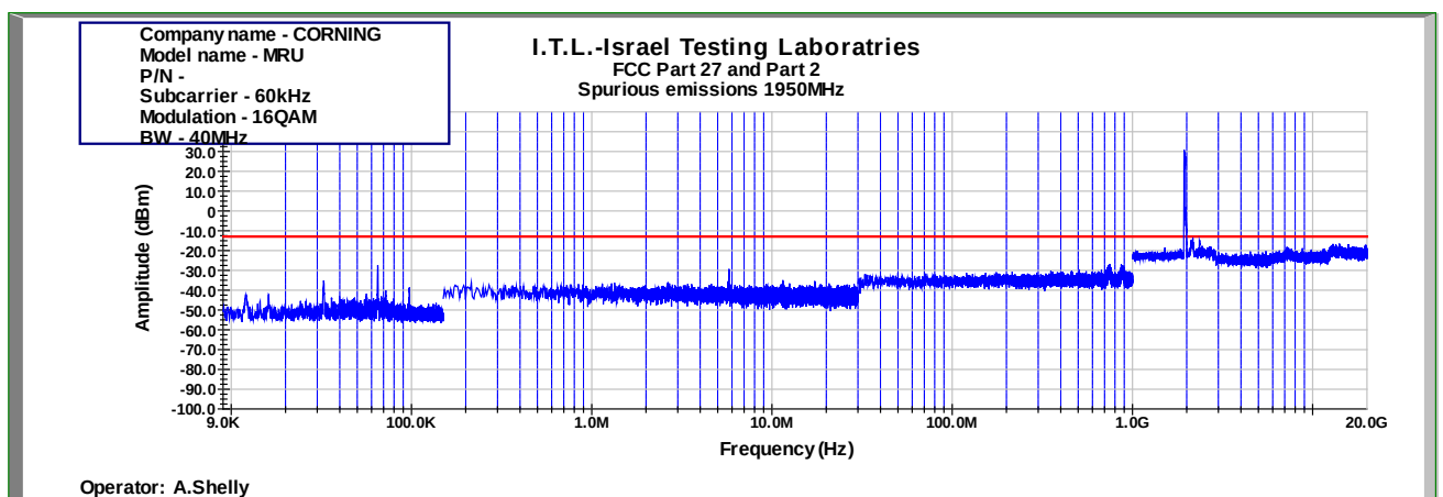
Figure 845: Spurious Emissions at Antenna Terminal 16QAM 40MHz B.W.; 1950.0MHz, 60kHz
