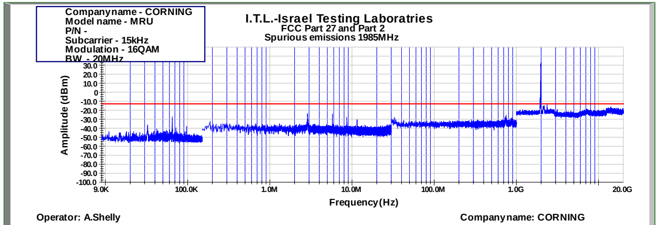
Figure 831: Spurious Emissions at Antenna Terminal 16QAM 20MHz B.W.; 1985.0MHz, 15kHz
