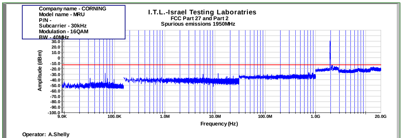
Figure 844: Spurious Emissions at Antenna Terminal 16QAM 40MHz B.W.; 1950.0MHz, 30kHz
