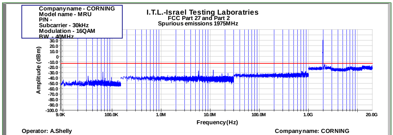
Figure 850: Spurious Emissions at Antenna Terminal 16QAM 40MHz B.W.; 1975.0MHz, 30kHz
