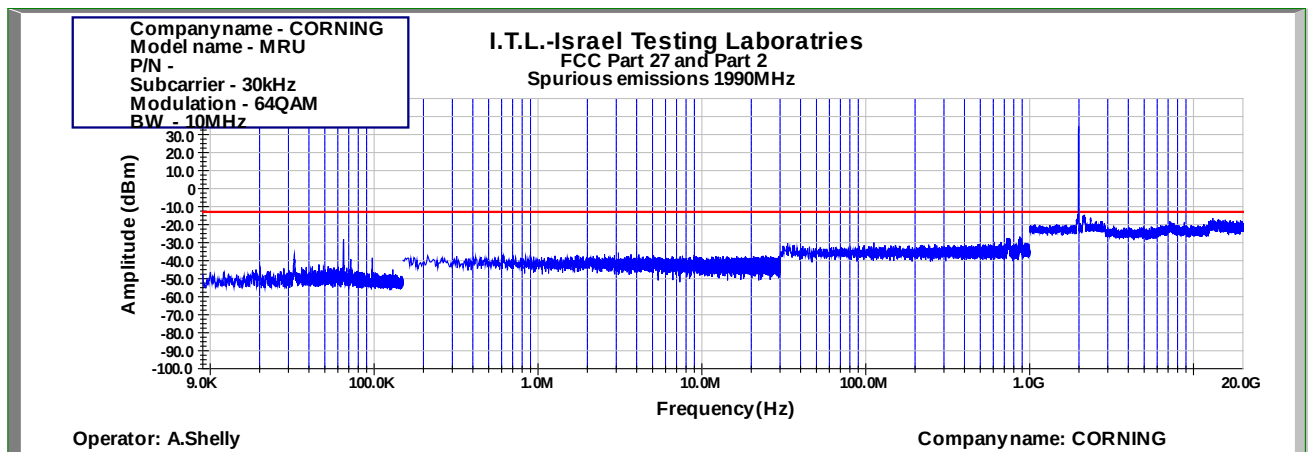
Figure 880: Spurious Emissions at Antenna Terminal 64QAM 10MHz B.W.; 1990.0MHz, 30kHz
