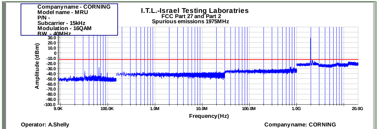
Figure 849: Spurious Emissions at Antenna Terminal 16QAM 40MHz B.W.; 1975.0MHz, 15kHz
