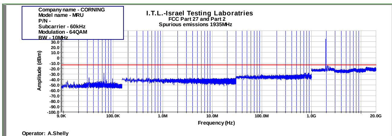
Figure 875: Spurious Emissions at Antenna Terminal 64QAM 10MHz B.W.; 1935.00MHz, 60kHz
