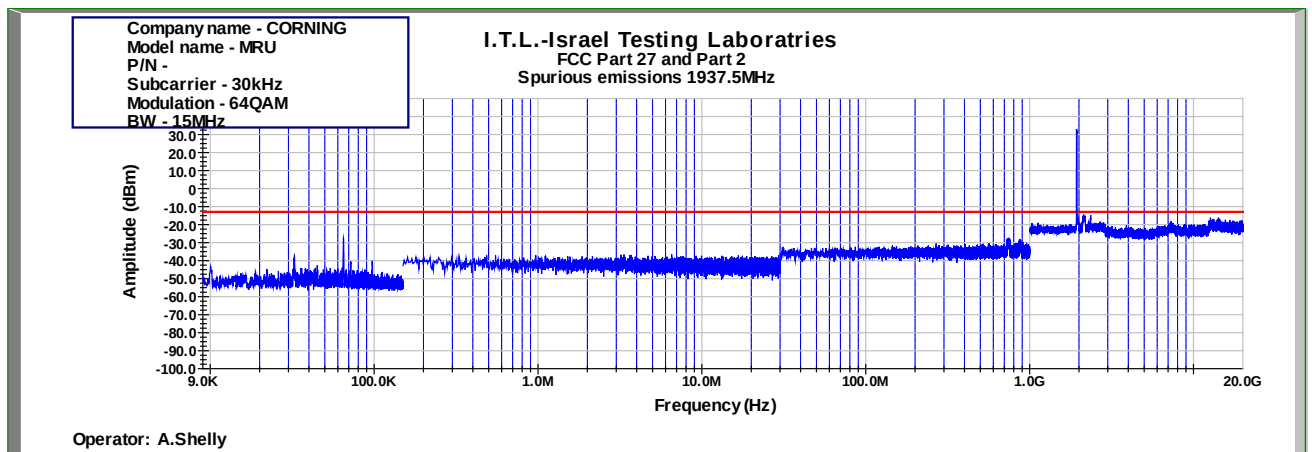
Figure 883: Spurious Emissions at Antenna Terminal 64QAM 15MHz B.W.; 1937.5MHz, 30kHz
