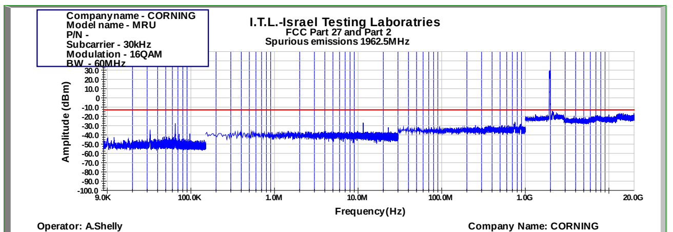
Figure 863: Spurious Emissions at Antenna Terminal 16QAM 60MHz B.W.; 1962.5MHz, 30kHz
