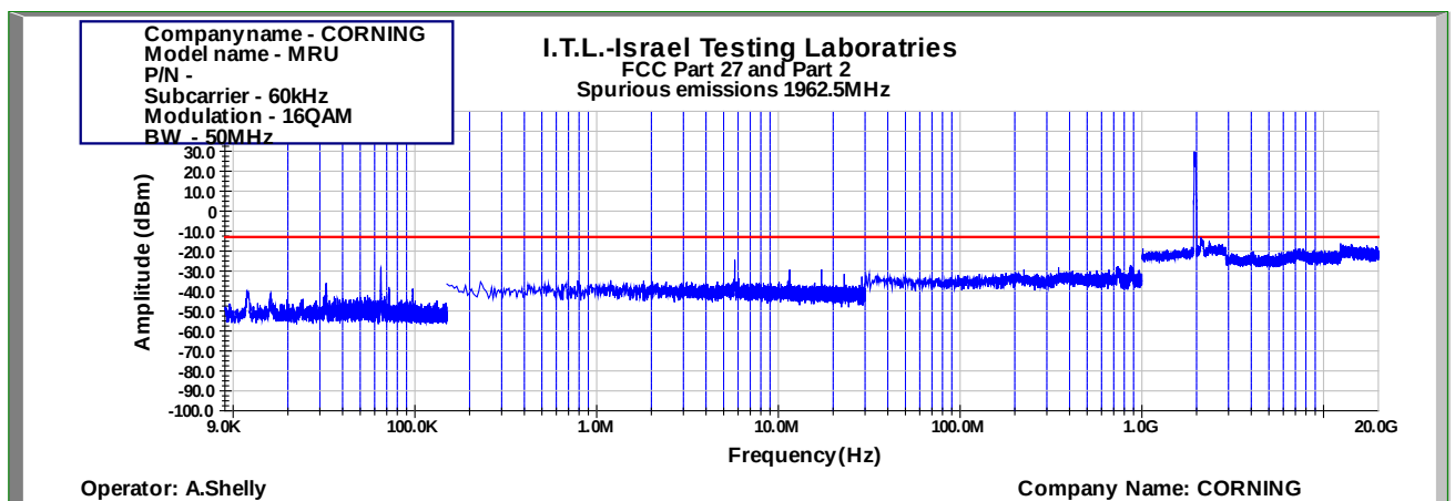
Figure 857: Spurious Emissions at Antenna Terminal 16QAM 50MHz B.W.; 1962.5MHz, 60kHz
