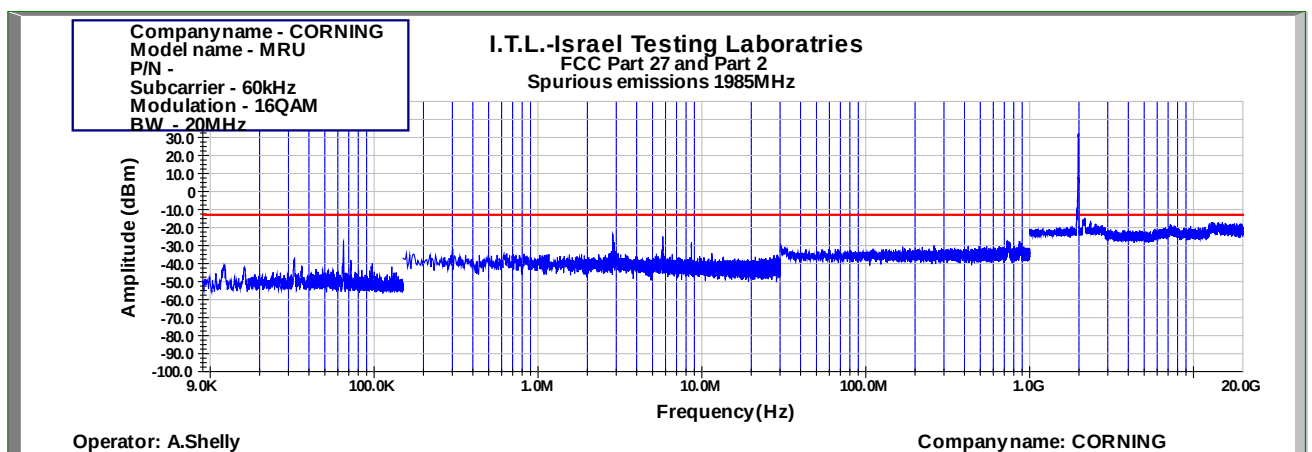
Figure 833: Spurious Emissions at Antenna Terminal 16QAM 20MHz B.W.; 1985.0MHz, 60kHz
