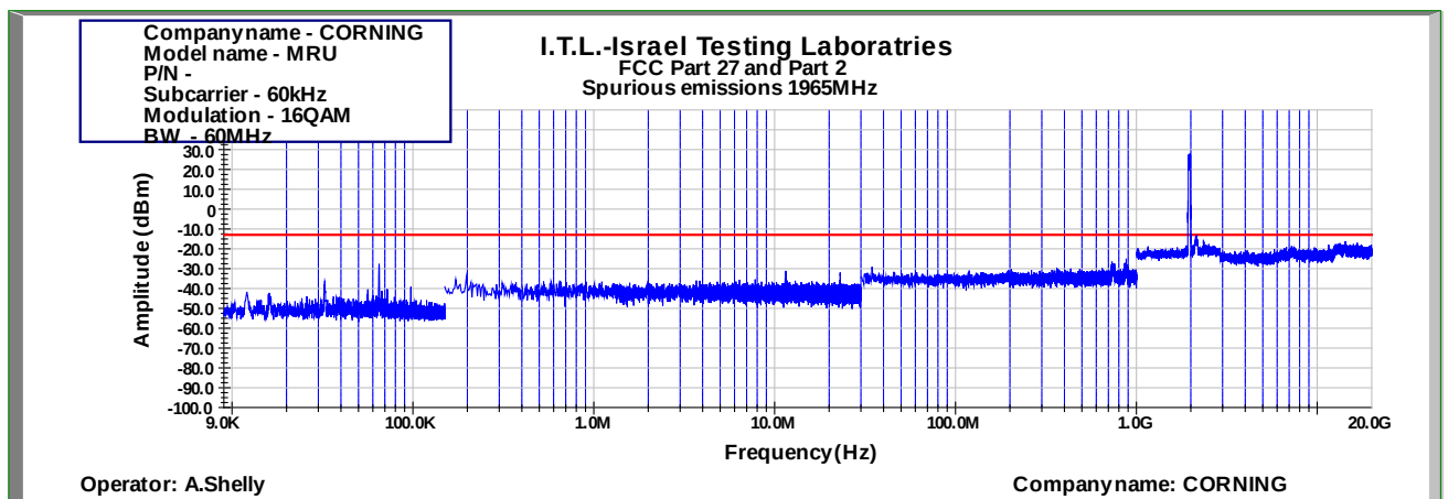
Figure 866: Spurious Emissions at Antenna Terminal 16QAM 60MHz B.W.; 1965.0MHz, 60kHz
