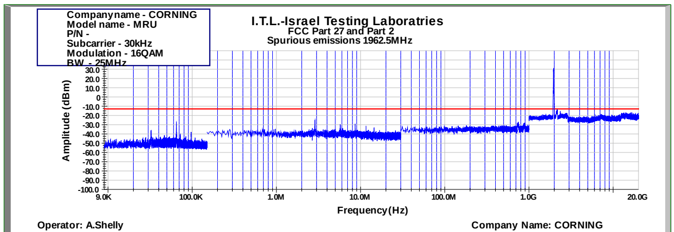
Figure 838: Spurious Emissions at Antenna Terminal 16QAM 25MHz B.W.; 1962.5MHz, 30kHz
