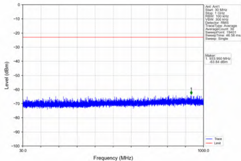
n38_15kHz_SISO_NTNV_10MHz_DFT-s-OFDM_QPSK_2615MHz_Edge_1RB_Right
