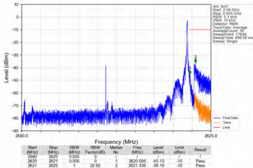
n38_15kHz_SISO_NTNV_40MHz_CP-OFDM QPSK_2600MHz_Edge_1RB_Right
