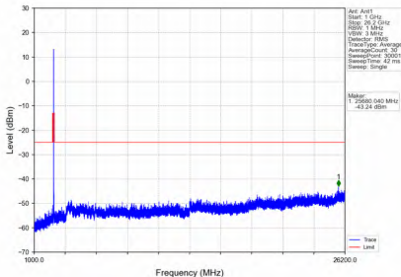
n38_15kHz_SISO_NTNV_20MHz_CP-OFDM QPSK_2580MHz_Outer_Full
