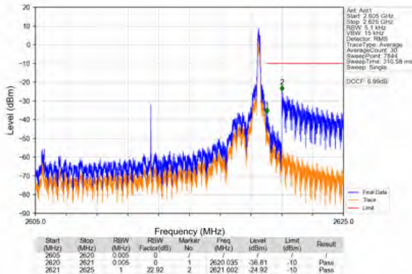
n38_15kHz_SISO_NTNV_15MHz_DFT-s-OFDM PI/2 BPSK_2612.5MHz_Edge_1RB_Right
