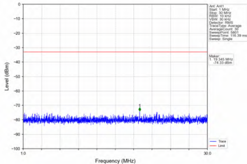
n38_15kHz_SISO_NTNV_20MHz_DFT-s-OFDM_QPSK_2610MHz_Edge_1RB_Right
