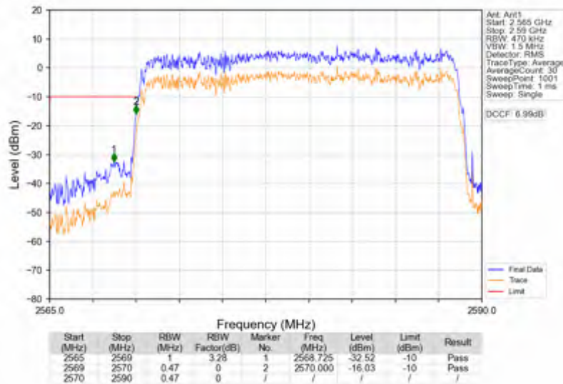
n38_15kHz_SISO_NTNV_20MHz_DFT-s-OFDM PI/2 BPSK_2580MHz_Outer_Full
