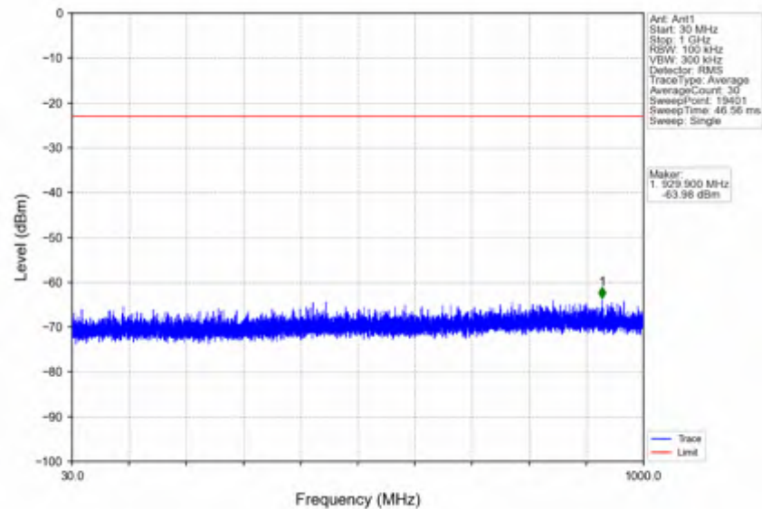
n38_15kHz_SISO_NTNV_30MHz_CP-OFDM QPSK_2605MHz_Edge_1RB_Right
