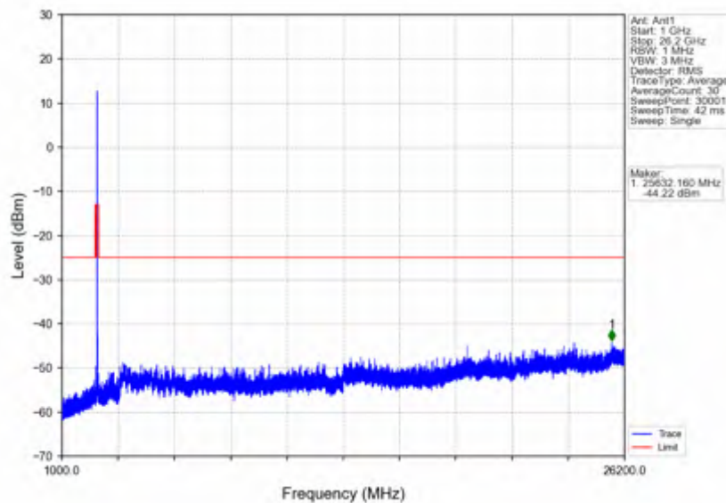
n38_15kHz_SISO_NTNV_25MHz_DFT-s-OFDM PI/2 BPSK_2582.5MHz_Outer_Full
