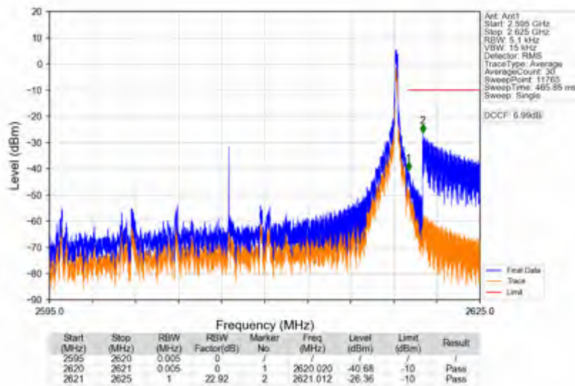
n38_15kHz_SISO_NTNV_25MHz_DFT-s-OFDM PI/2 BPSK_2607.5MHz_Inner_1RB_Right
