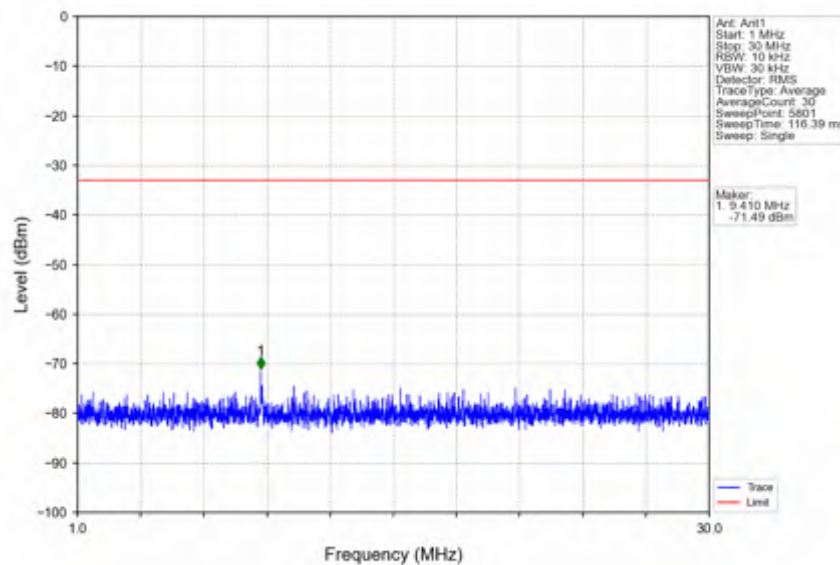
n38_15kHz_SISO_NTNV_30MHz_CP-OFDM QPSK_2585MHz_Edge_1RB_Left
