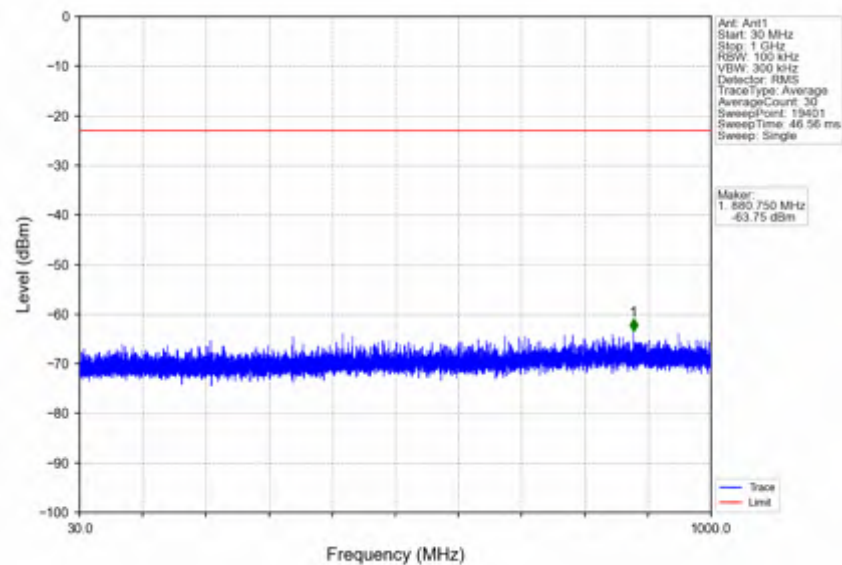
n38_15kHz_SISO_NTNV_20MHz_DFT-s-OFDM_PI/2_BPSK_2610MHz_Edge_1RB_Right
