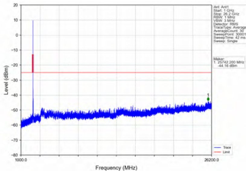
n38_15kHz_SISO_NTNV_30MHz_CP-OFDM QPSK_2605MHz_Edge_1RB_Right
