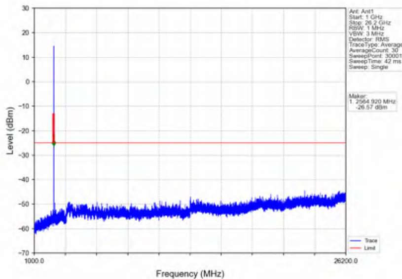
n38_15kHz_SISO_NTNV_10MHz_DFT-s-OFDM PI/2 BPSK_2575MHz_Outer_Full
