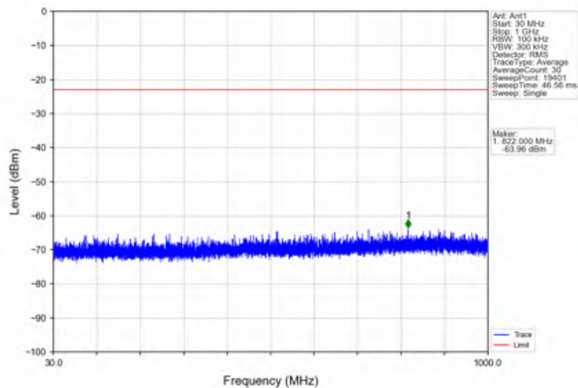
n38_15kHz_SISO_NTNV_5MHz_CP-OFDM_QPSK_2617.5MHz_Edge_1RB_Right
