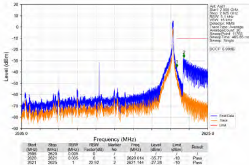
n38_15kHz_SISO_NTNV_25MHz_DFT-s-OFDM QPSK_2607.5MHz_Edge_1RB_Right
