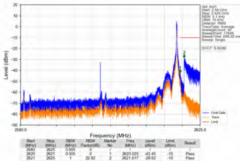
n38_15kHz_SISO_NTNV_40MHz_CP-OFDM QPSK_2600MHz_Inner_1RB_Right
