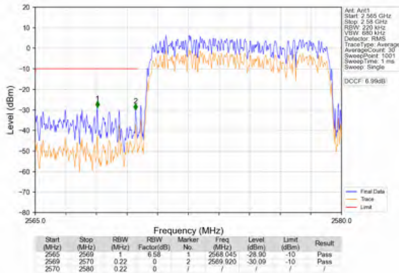
n38_30kHz_SISO_NTNV_10MHz_DFT-s-OFDM PI/2 BPSK_2575MHz_Outer_Full
