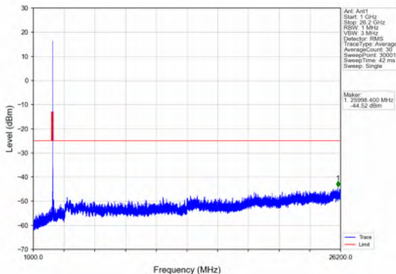
n38_15kHz_SISO_NTNV_20MHz_DFT-s-OFDM PI/2 BPSK_2610MHz_Edge_1RB_Right
