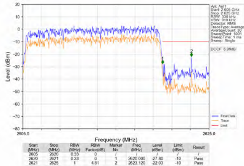
n38_15kHz_SISO_NTNV_15MHz_CP-OFDM QPSK_2612.5MHz_Outer_Full
