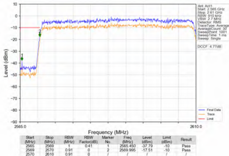
n38_15kHz_SISO_NTNV_40MHz_DFT-s-OFDM PI/2 BPSK_2590MHz_Outer_Full
