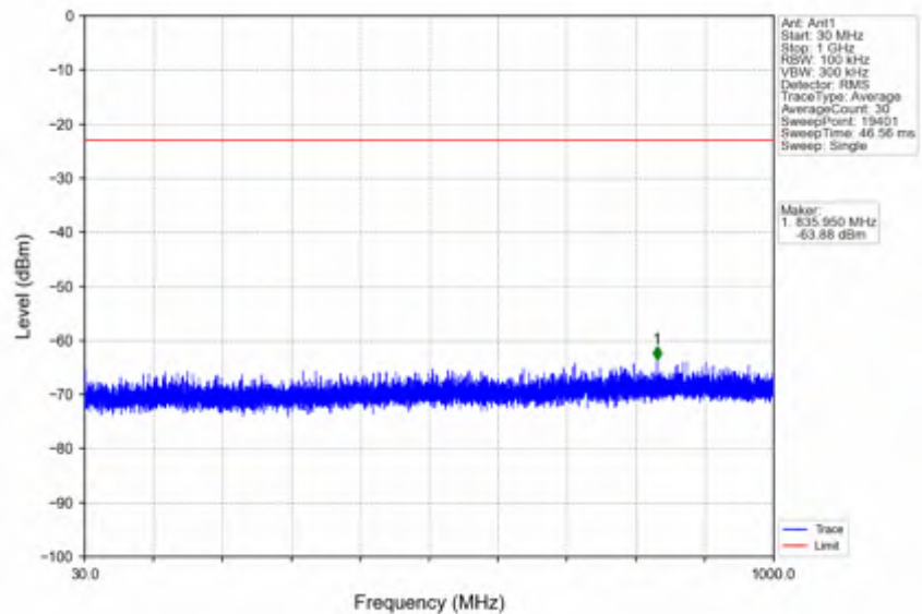
n38_15kHz_SISO_NTNV_25MHz_CP-OFDM QPSK_2582.5MHz_Edge_1RB_Left
