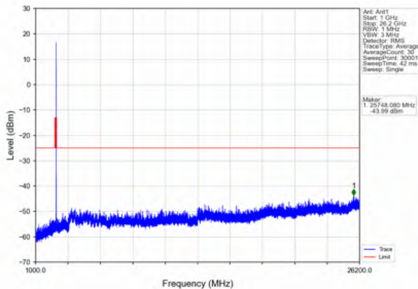
n38_15kHz_SISO_NTNV_10MHz_DFT-s-OFDM PI/2 BPSK_2615MHz_Edge_1RB_Right
