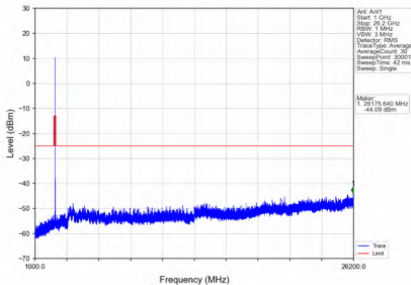
n38_15kHz_SISO_NTNV_25MHz_DFT-s-OFDM QPSK_2607.5MHz_Edge_1RB_Right
