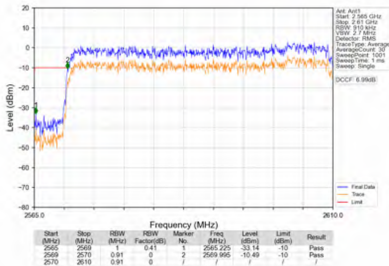
n38_15kHz_SISO_NTNV_40MHz_CP-OFDM QPSK_2590MHz_Outer_Full
