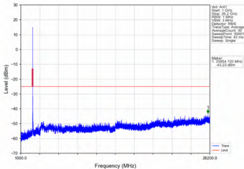
n38_15kHz_SISO_NTNV_30MHz_DFT-s-OFDM PI/2 BPSK_2605MHz_Edge_1RB_Right
