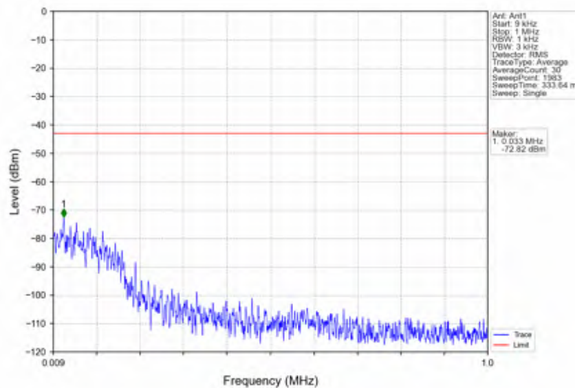
n38_15kHz_SISO_NTNV_30MHz_CP-OFDM_QPSK_2595MHz_Edge_1RB_Left
