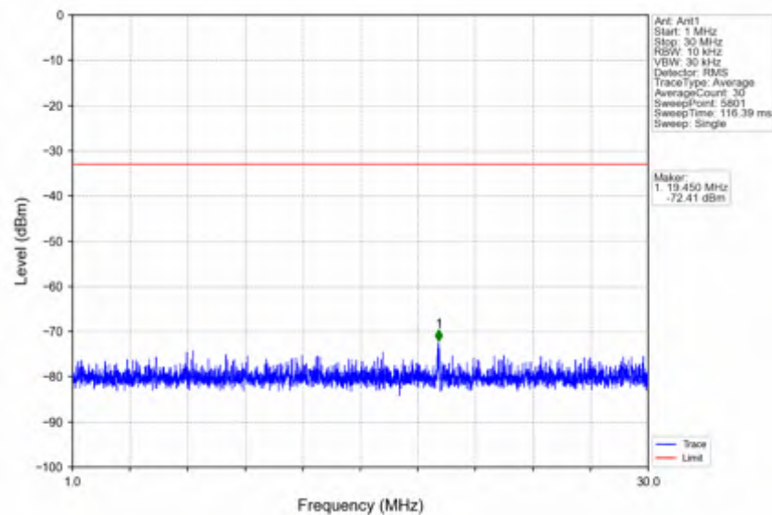
n38_15kHz_SISO_NTNV_30MHz_DFT-s-OFDM QPSK_2595MHz_Edge_1RB_Left
