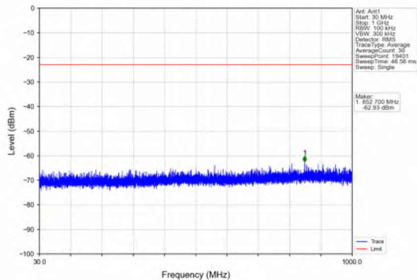
n38_30kHz_SISO_NTNV_10MHz_DFT-s-OFDM QPSK_2575MHz_Edge_1RB_Left
