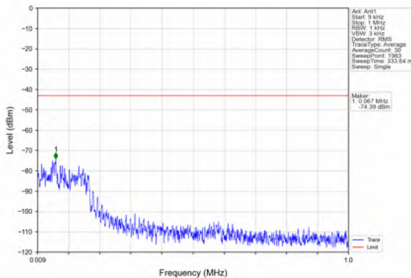
n38_15kHz_SISO_NTNV_25MHz_DFT-s-OFDM_PI/2_BPSK_2595MHz_Edge_1RB_Left
