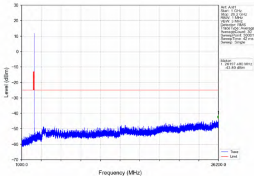
n38_15kHz_SISO_NTNV_5MHz_CP-OFDM_QPSK_2617.5MHz_Edge_1RB_Right
