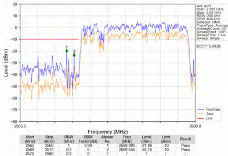
n38_15kHz_SISO_NTNV_10MHz_DFT-s-OFDM QPSK_2575MHz_Outer_Full
