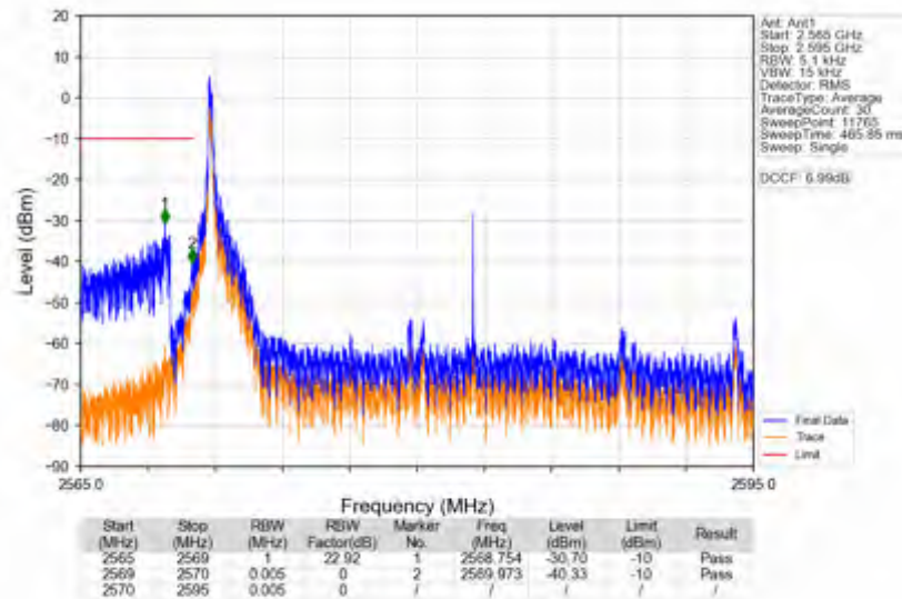
n38_15kHz_SISO_NTNV_25MHz_CP-OFDM QPSK_2582.5MHz_Inner_1RB_Left
