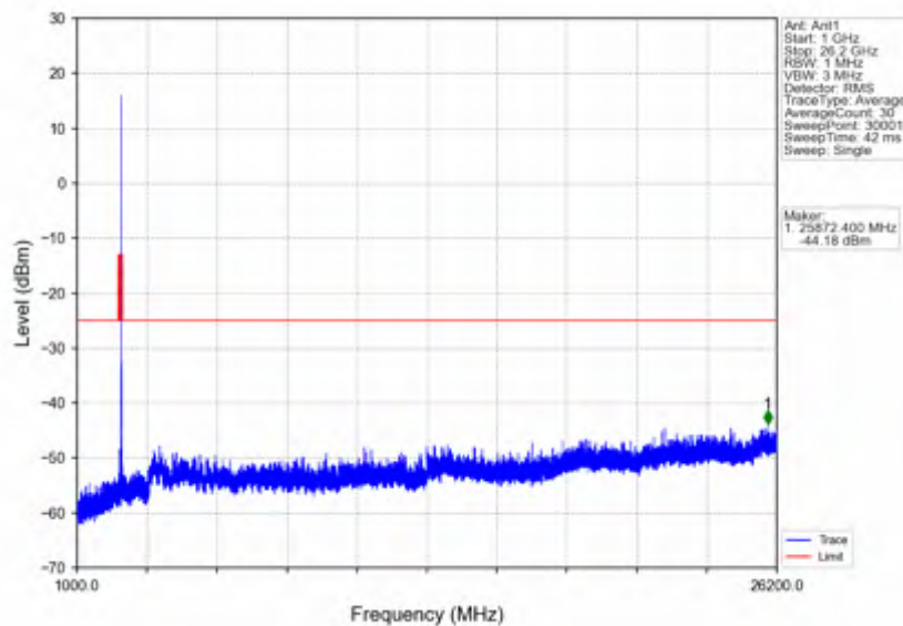
n38_15kHz_SISO_NTNV_15MHz_CP-OFDM QPSK_2612.5MHz_Edge_1RB_Right
