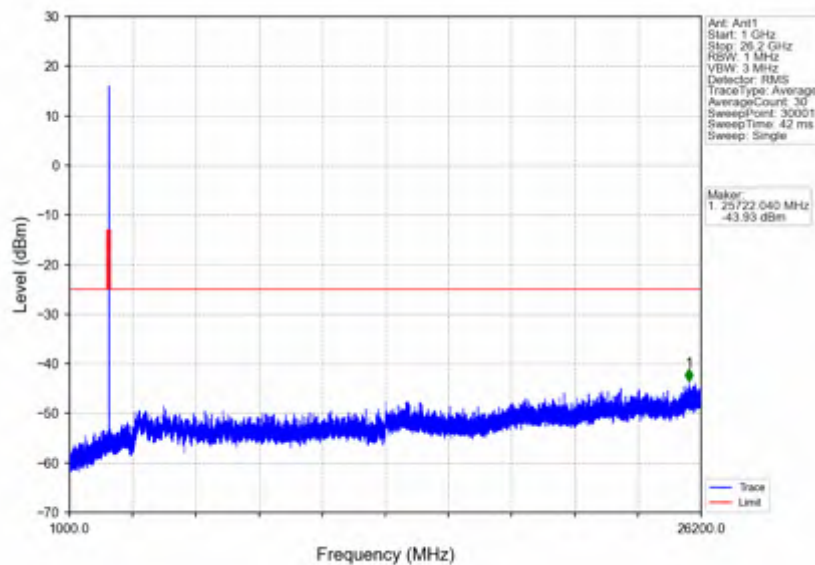
n38_30kHz_SISO_NTNV_10MHz_DFT-s-OFDM QPSK_2575MHz_Outer_Full
