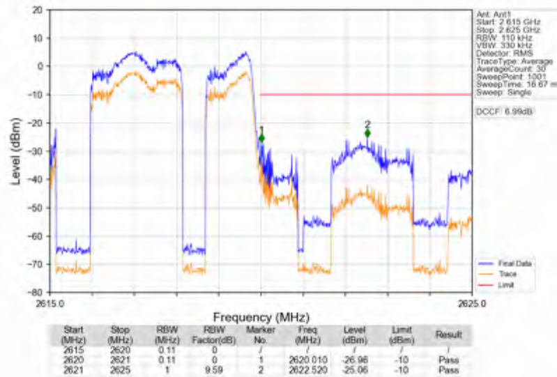
n38_15kHz_SISO_NTNV_5MHz_CP-OFDM QPSK_2617.5MHz_Outer_Full
