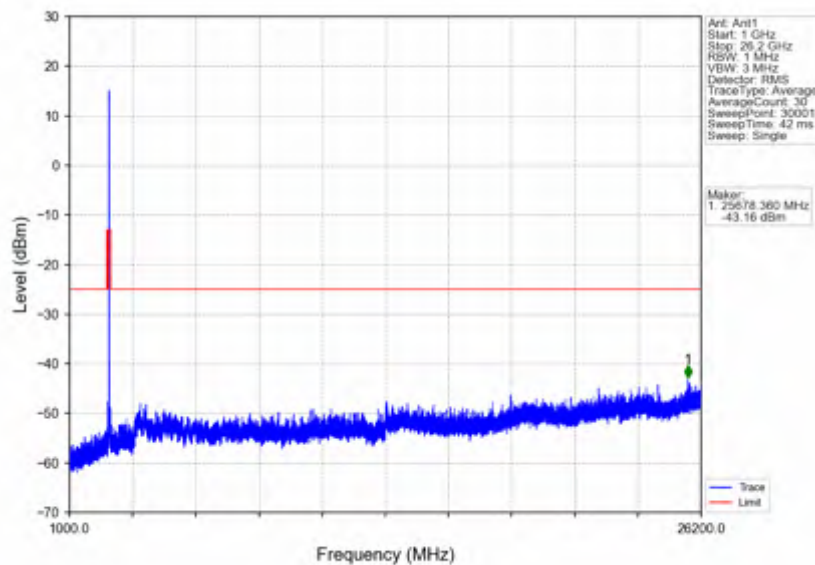
n38_15kHz_SISO_NTNV_20MHz_DFT-s-OFDM PI/2 BPSK_2580MHz_Outer_Full
