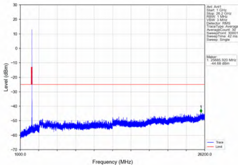
n38_15kHz_SISO_NTNV_20MHz_CP-OFDM QPSK_2610MHz_Edge_1RB_Right
