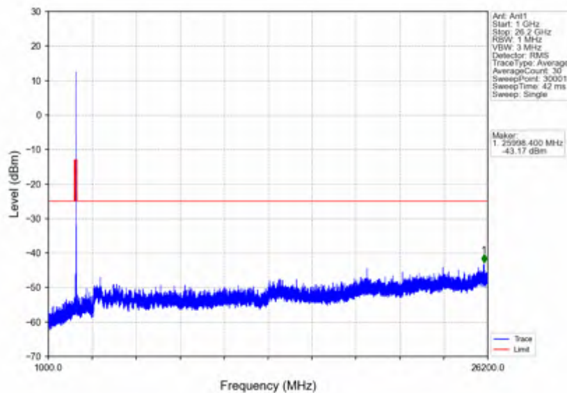
n38_15kHz_SISO_NTNV_20MHz_DFT-s-OFDM QPSK_2610MHz_Edge_1RB_Right
