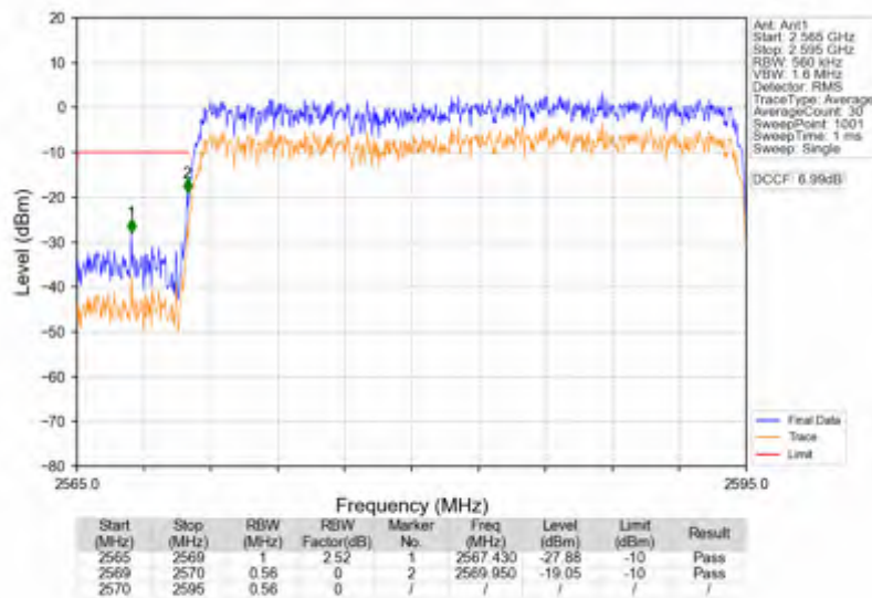
n38_15kHz_SISO_NTV_25MHz_CP-OFDM_QPSK_2582.5MHz_Outer_Full
