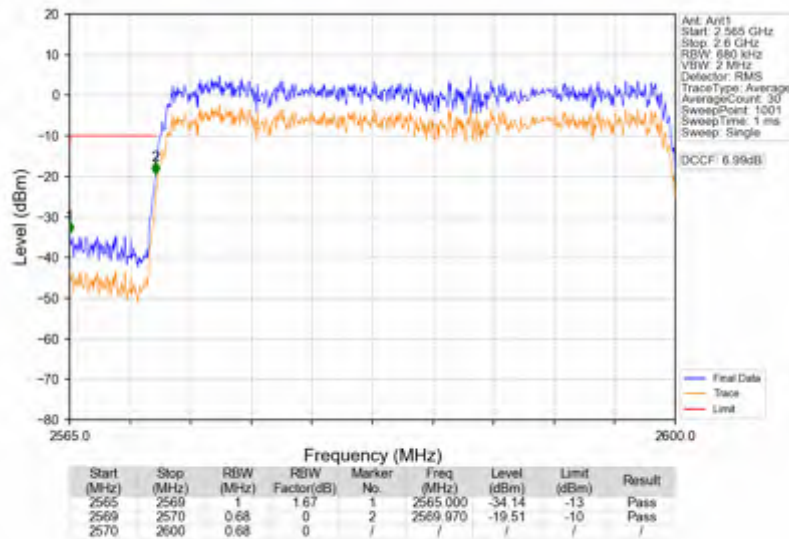
n38_15kHz_SISO_NTNV_30MHz_DFT-s-OFDM_QPSK_2585MHz_Outer_Full
