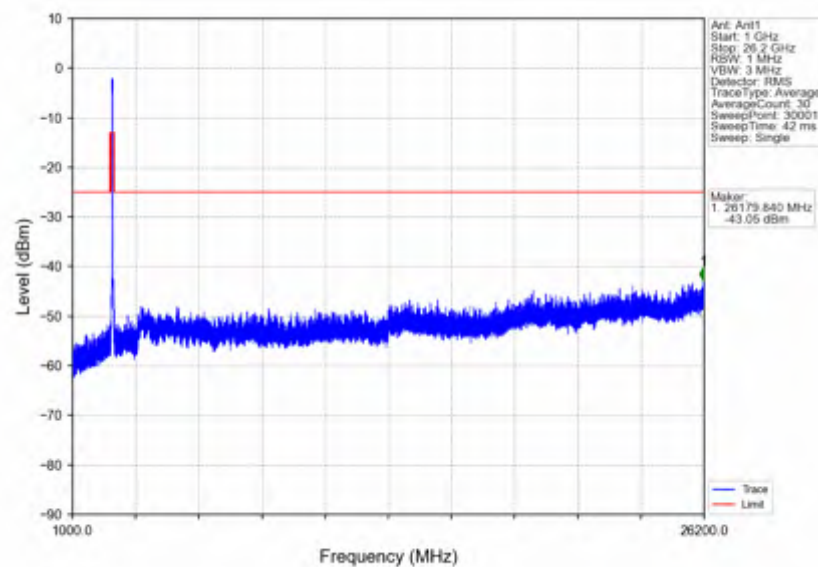
n38 15kHz SISO NTV 40MHz DFT-s-OFDM QPSK 2590MHz Outer Full
