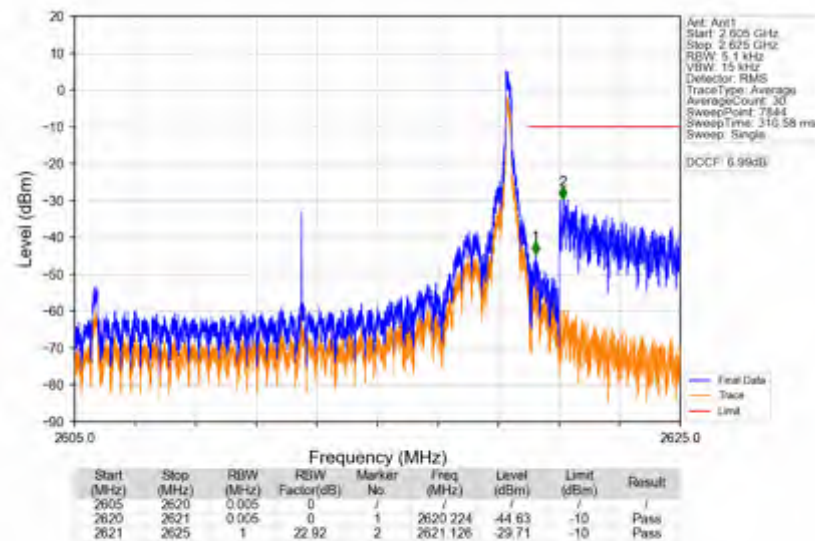
n38_15kHz_SISO_NTNV_15MHz_CP-OFDM QPSK_2612.5MHz_Inner_1RB_Right
