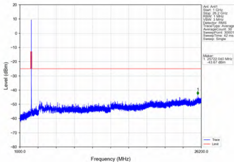
n38_15kHz_SISO_NTNV_40MHz_CP-OFDM QPSK_2590MHz_Outer_Full
