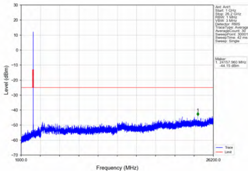
n38_15kHz_SISO_NTNV_10MHz_CP-OFDM QPSK_2575MHz_Outer_Full
