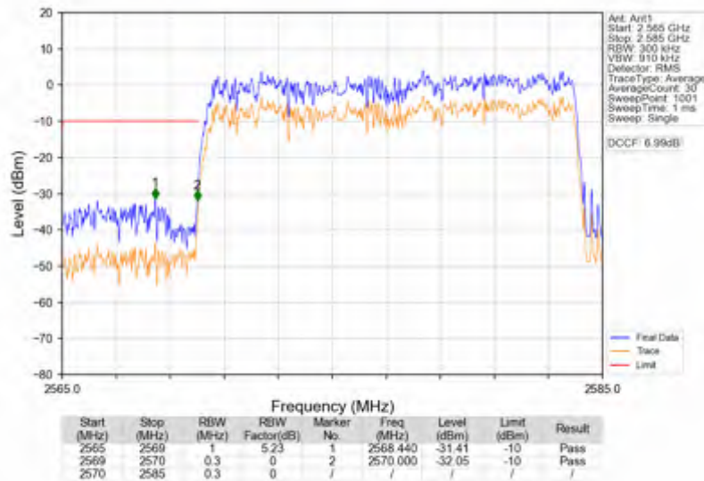
n38_15kHz_SISO_NTNV_15MHz_DFT-s-OFDM QPSK_2577.5MHz_Outer_Full
