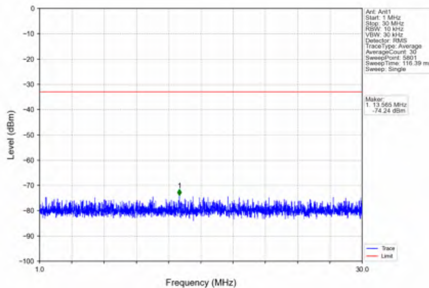
n38_15kHz_SISO_NTNV_40MHz_DFT-s-OFDM_PI/2_BPSK_2590MHz_Outer_Full
