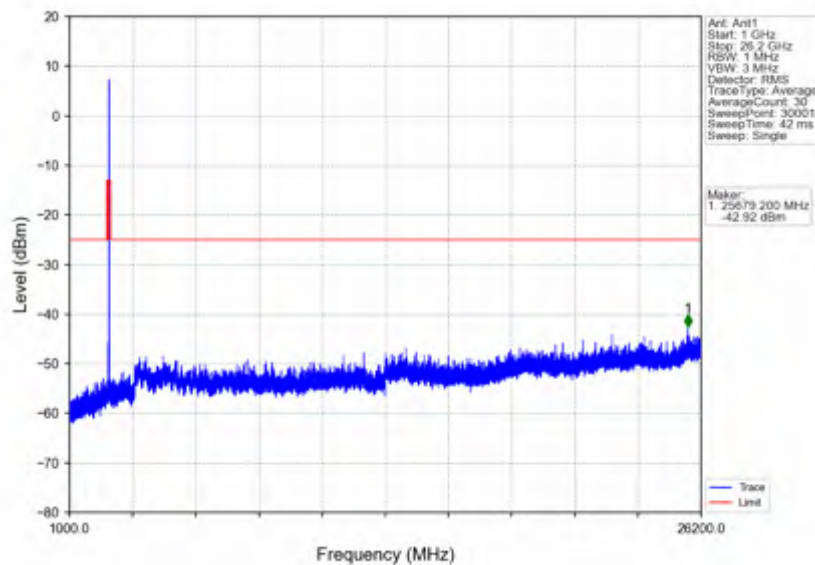
n38_15kHz_SISO_NTNV_15MHz_CP-OFDM QPSK_2577.5MHz_Outer_Full
