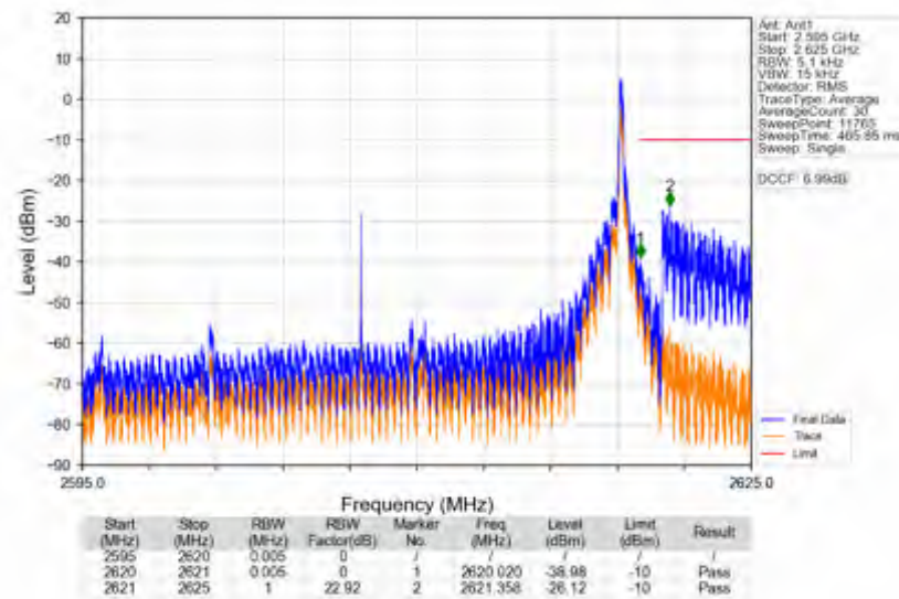
n38_15kHz_SISO_NTNV_25MHz_CP-OFDM QPSK_2607.5MHz_Inner_1RB_Right
