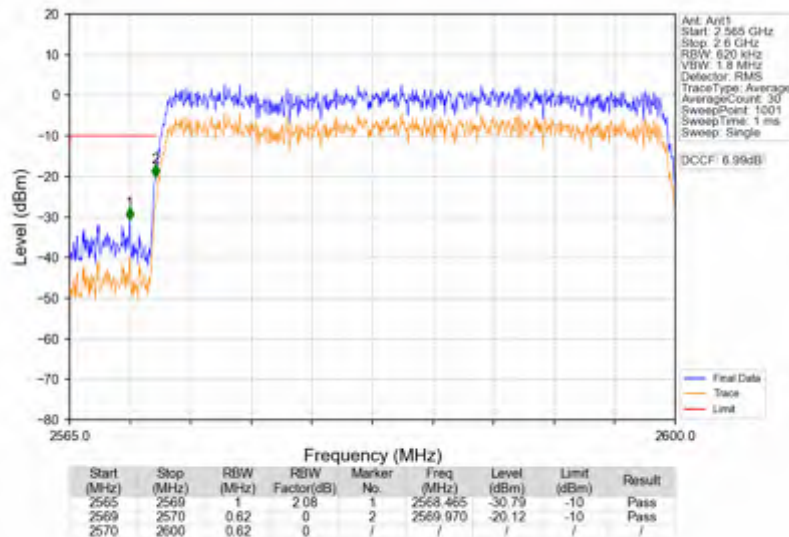
n38_15kHz_SISO_NTNV_30MHz_CP-OFDM QPSK_2585MHz_Outer_Full
