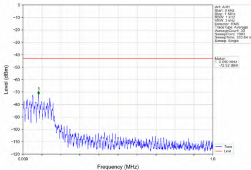
n38_15kHz_SISO_NTNV_10MHz_DFT-s-OFDM_QPSK_2595MHz_Edge_1RB_Left
