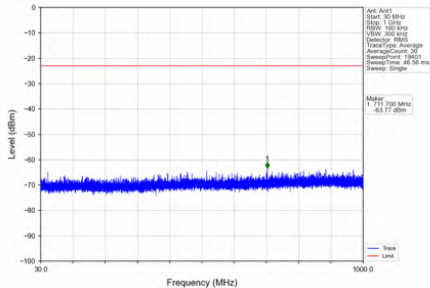
n38_15kHz_SISO_NTNV_25MHz_DFT-s-OFDM QPSK_2595MHz_Edge_1RB_Left
