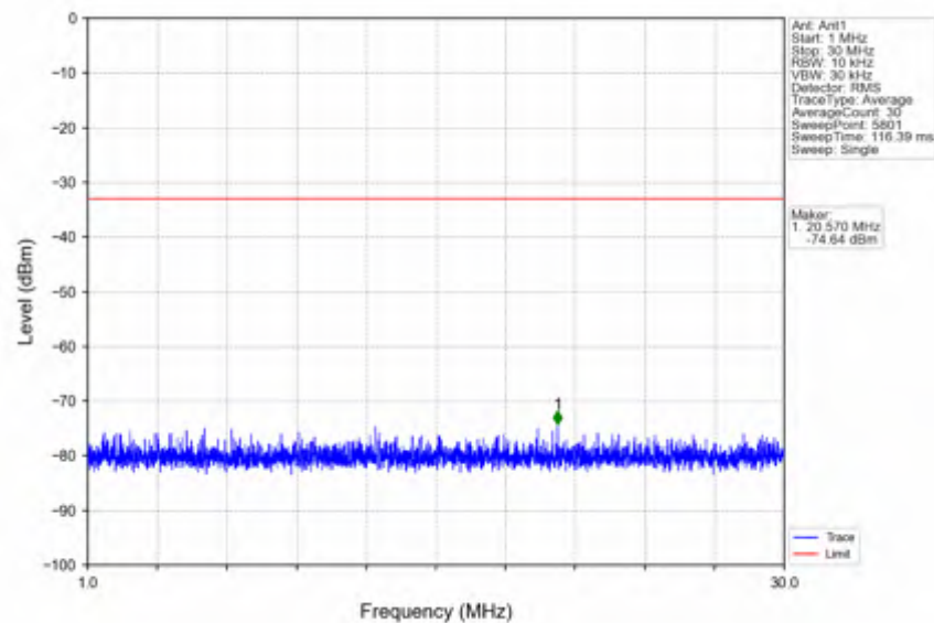
n38_15kHz_SISO_NTNV_20MHz_CP-OFDM QPSK_2610MHz_Edge_1RB_Right
