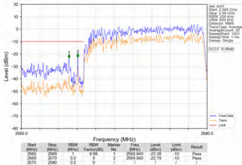
n38_15kHz_SISO_NTNV_10MHz_CP-OFDM QPSK_2575MHz_Outer_Full
