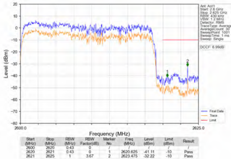
n38_15kHz_SISO_NTNV_20MHz_DFT-s-OFDM_PI/2_BPSK_2610MHz_Outer_Full
