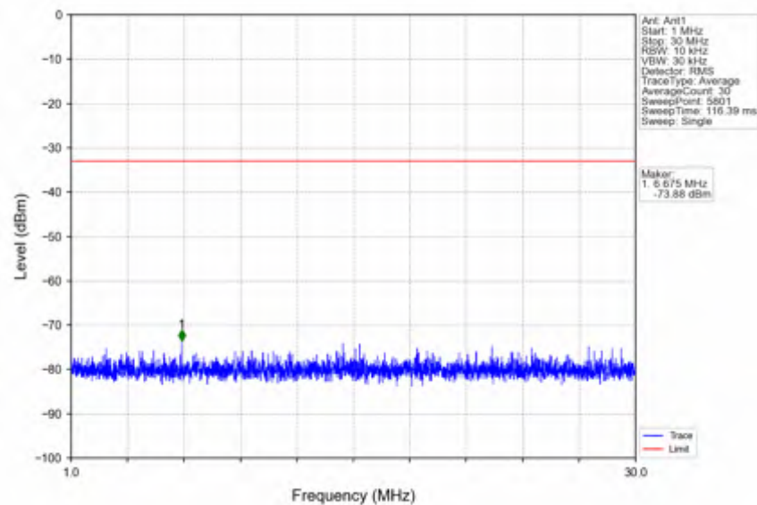
n38_15kHz_SISO_NTNV_40MHz_DFT-s-OFDM_QPSK_2600MHz_Edge_1RB_Right
