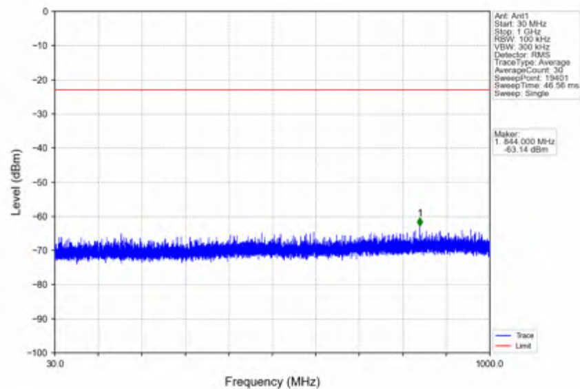
n38_15kHz_SISO_NTNV_10MHz_CP-OFDM_QPSK_2595MHz_Edge_1RB_Left
