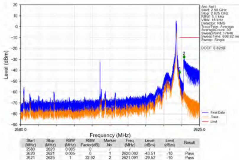
n38_15kHz_SISO_NTNV_40MHz_DFT-s-OFDM_PI/2_BPSK_2600MHz_Inner_1RB_Right
