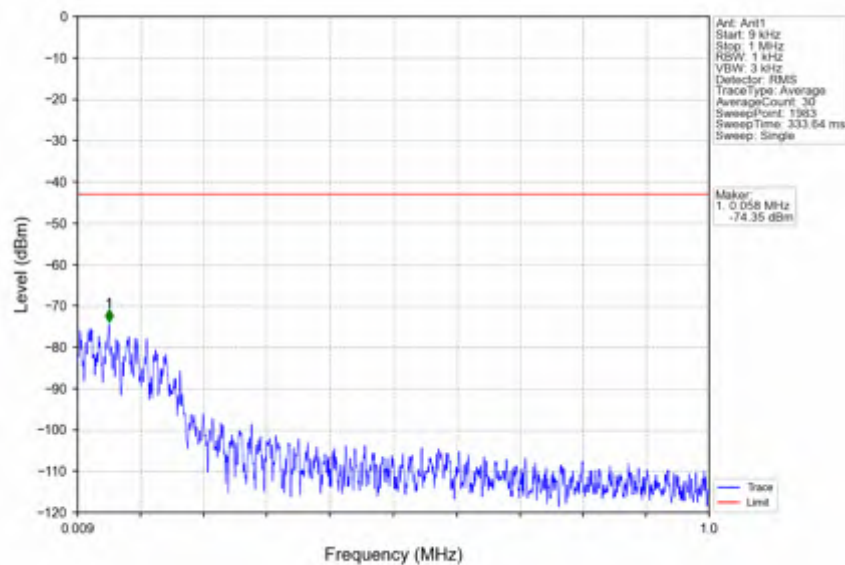
n38_15kHz_SISO_NTNV_25MHz_CP-OFDM QPSK_2607.5MHz_Edge_1RB_Right
