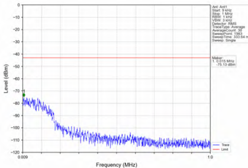
n38_15kHz_SISO_NTNV_25MHz_CP-OFDM_QPSK_2582.5MHz_Edge_1RB_Left
