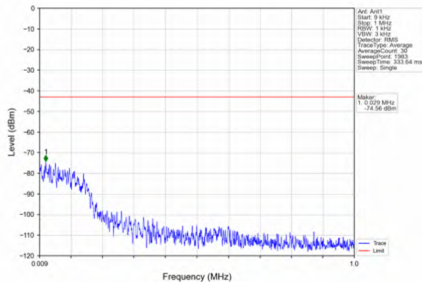
n38_15kHz_SISO_NTNV_10MHz_CP-OFDM QPSK_2615MHz_Edge_1RB_Right
