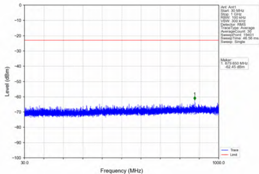
n38_15kHz_SISO_NTNV_20MHz_CP-OFDM QPSK_2610MHz_Edge_1RB_Right
