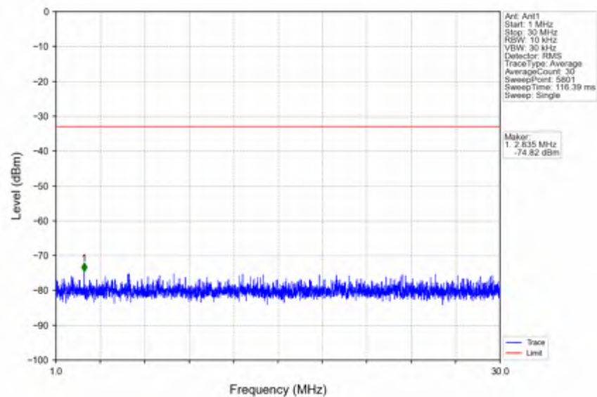
n38_15kHz_SISO_NTNV_10MHz_DFT-s-OFDM PI/2 BPSK_2615MHz_Edge_1RB_Right
