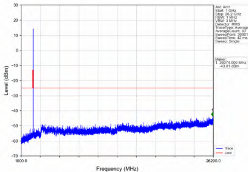
n38_30kHz_SISO_NTNV_10MHz_DFT-s-OFDM PI/2 BPSK_2575MHz_Outer_Full
