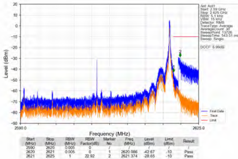
n38_15kHz_SISO_NTNV_30MHz_DFT-s-OFDM QPSK_2605MHz_Edge_1RB_Right
