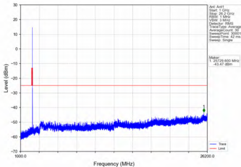
n38_15kHz_SISO_NTNV_10MHz_DFT-s-OFDM QPSK_2615MHz_Edge_1RB_Right
