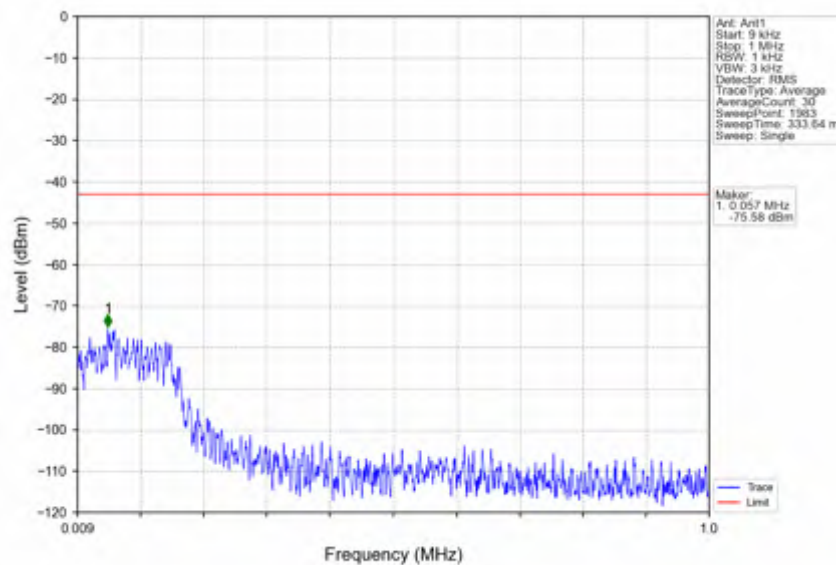
n38_15kHz_SISO_NTNV_40MHz_DFT-s-OFDM QPSK_2595MHz_Edge_1RB_Left
