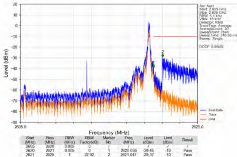
n38_15kHz_SISO_NTNV_15MHz_CP-OFDM QPSK_2612.5MHz_Edge_1RB_Right
