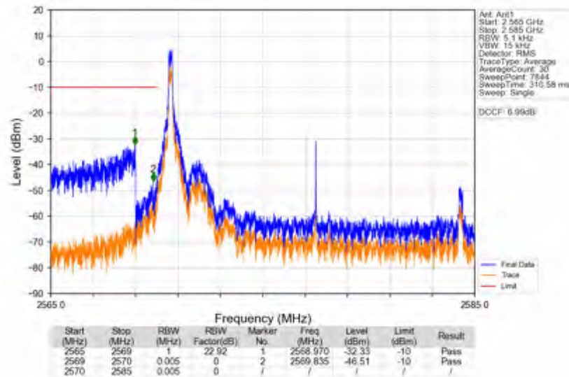
n38_15kHz_SISO_NTNV_15MHz_CP-OFDM_QPSK_2577.5MHz_Inner_1RB_Left
