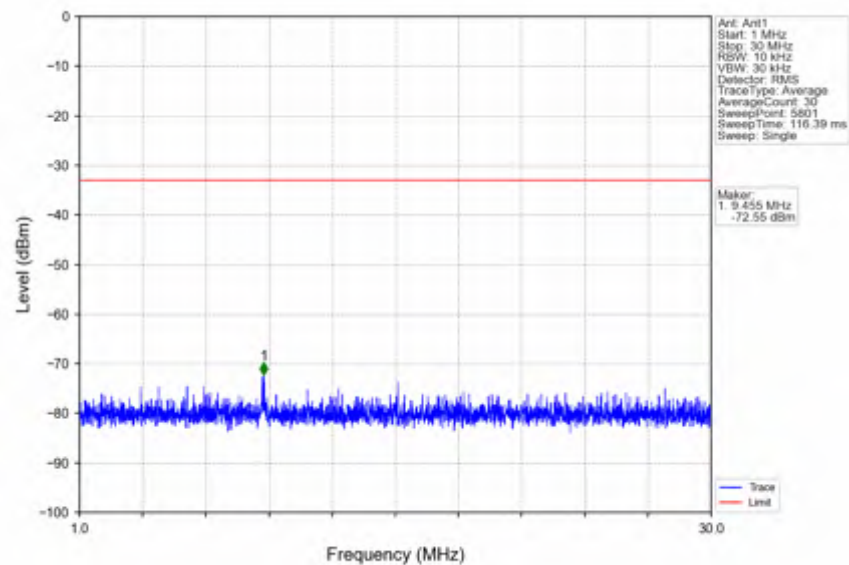
n38_15kHz_SISO_NTNV_30MHz_DFT-s-OFDM PI/2 BPSK_2585MHz_Edge_1RB_Left
