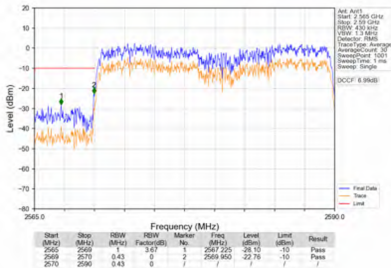
n38_15kHz_SISO_NTNV_20MHz_CP-OFDM QPSK_2580MHz_Outer_Full
