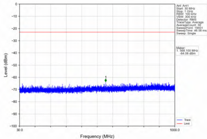
n38_15kHz_SISO_NTNV_30MHz_DFT-s-OFDM QPSK_2595MHz_Edge_1RB_Left
