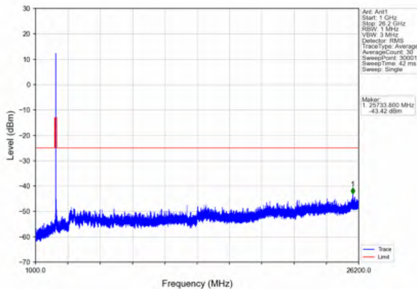
n38_15kHz_SISO_NTNV_30MHz_CP-OFDM QPSK_2585MHz_Outer_Full
