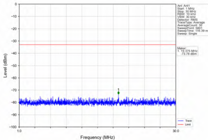
n38_15kHz_SISO_NTNV_15MHz_CP-OFDM_QPSK_2595MHz_Edge_1RB_Left
