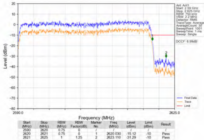
n38_15kHz_SISO_NTV_30MHz_CP-OFDM_QPSK_2605MHz_Outer_Full
