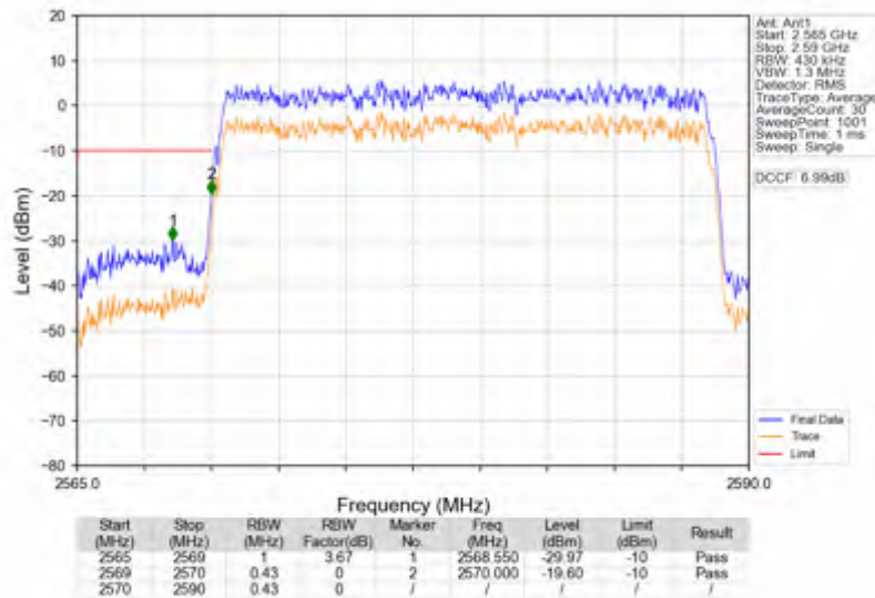
n38_15kHz_SISO_NTNV_20MHz_DFT-s-OFDM QPSK_2580MHz_Outer_Full
