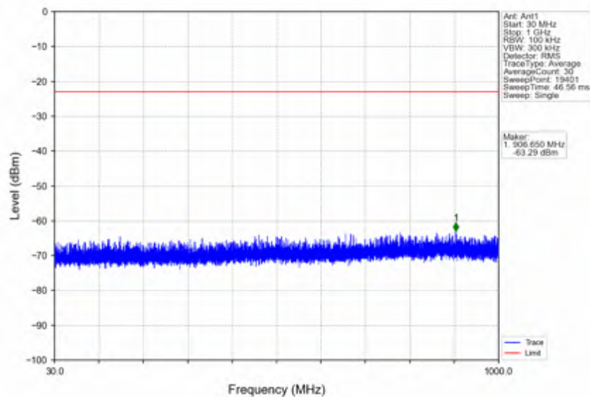
n38_15kHz_SISO_NTNV_40MHz_DFT-s-OFDM_PI/2_BPSK_2600MHz_Outer_Full
