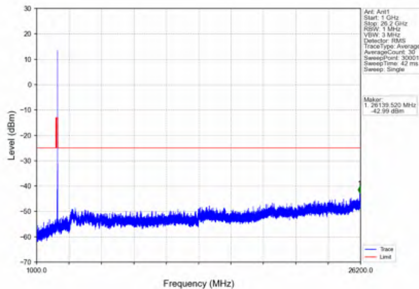
n38_15kHz_SISO_NTNV_20MHz_DFT-s-OFDM_PI/2_BPSK_2610MHz_Edge_1RB_Right
