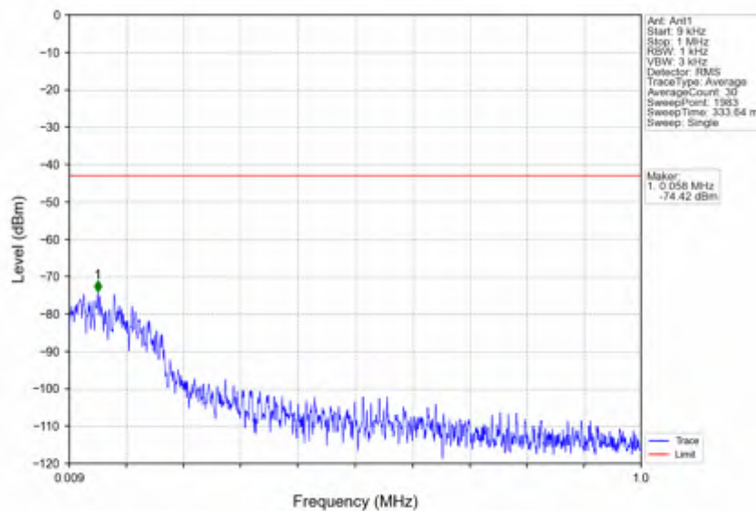
n38_15kHz_SISO_NTNV_15MHz_CP-OFDM_QPSK_2577.5MHz_Edge_1RB_Left
