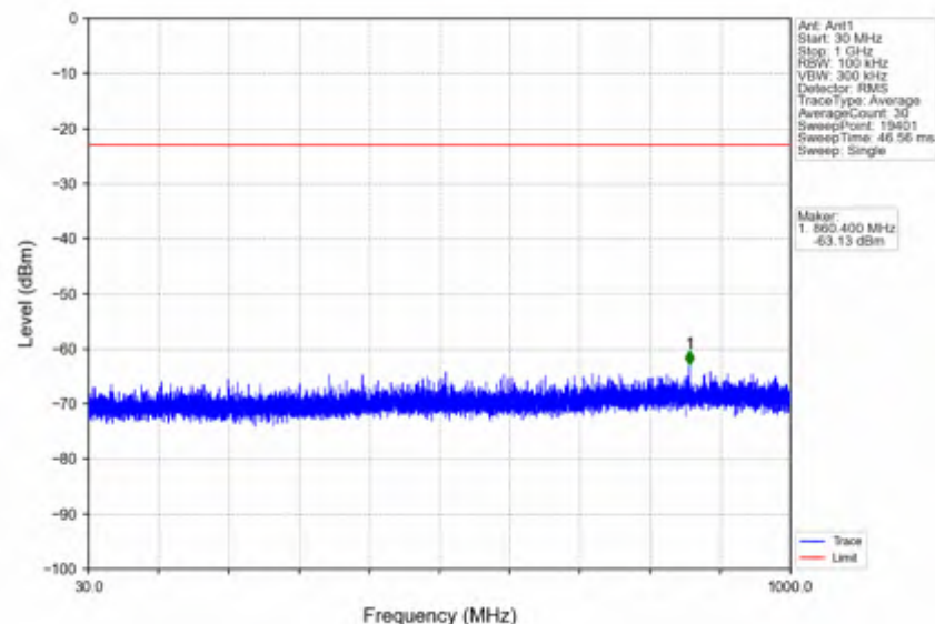
n38_15kHz_SISO_NTNV_25MHz_CP-OFDM_QPSK_2595MHz_Edge_1RB_Left
