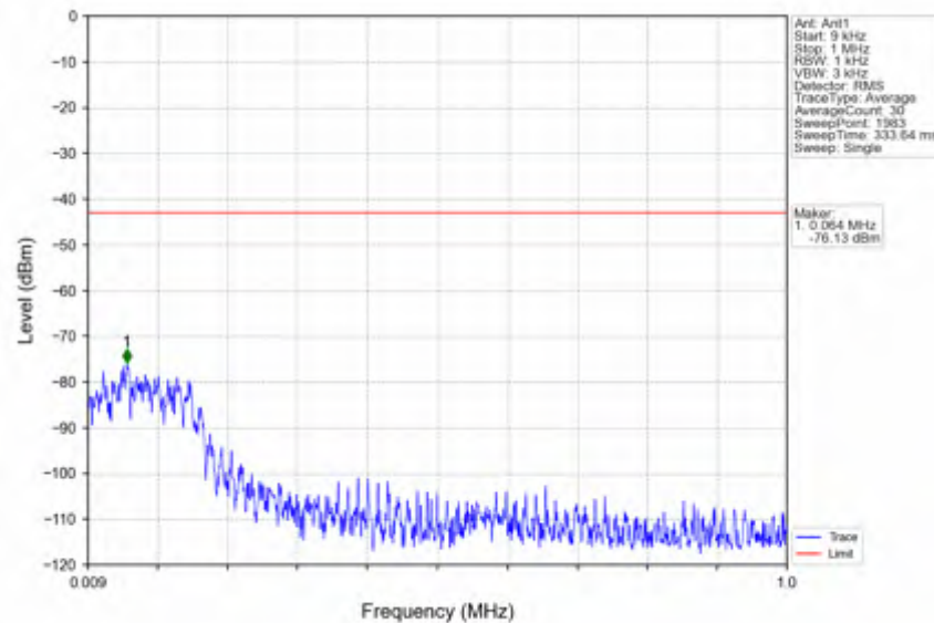
n38_15kHz_SISO_NTNV_30MHz_DFT-s-OFDM_QPSK_2605MHz_Edge_1RB_Right
