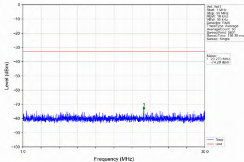
n38_15kHz_SISO_NTNV_40MHz_DFT-s-OFDM_PI/2_BPSK_2600MHz_Edge_1RB_Right
