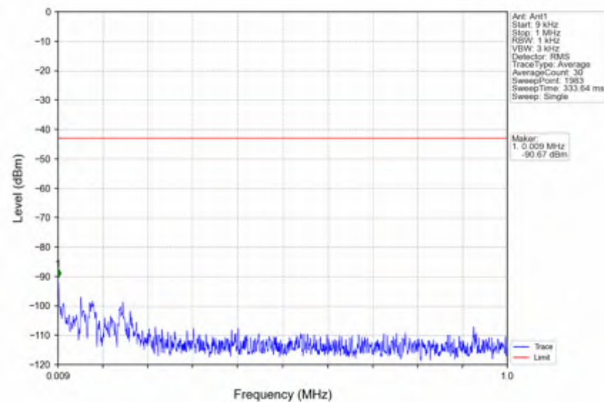
n38_15kHz_SISO_NTNV_40MHz_DFT-s-OFDM_QPSK_2590MHz_Outer_Full
