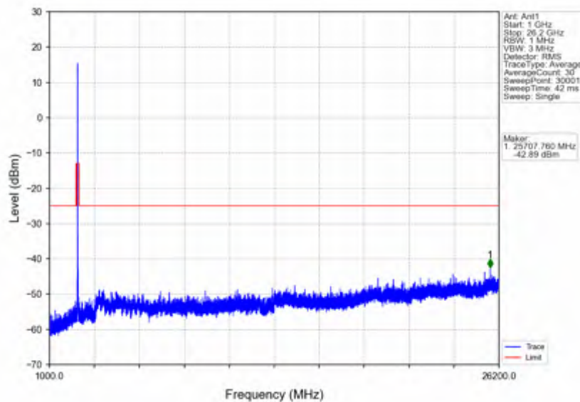
n38_15kHz_SISO_NTNV_40MHz_DFT-s-OFDM QPSK_2590MHz_Outer_Full
