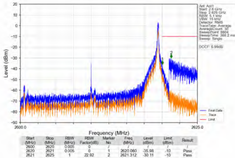
n38_15kHz_SISO_NTNV_20MHz_CP-OFDM QPSK_2610MHz_Edge_1RB_Right
