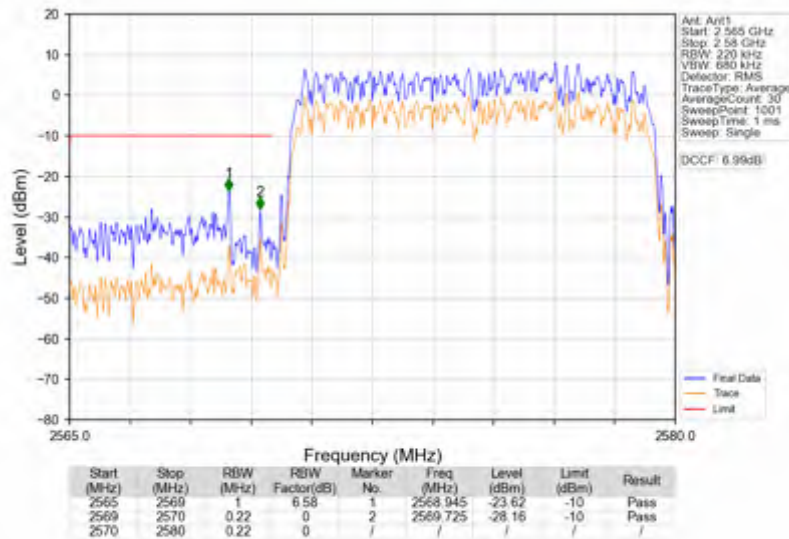
n38_30kHz_SISO_NTNV_10MHz_DFT-s-OFDM QPSK_2575MHz_Outer_Full
