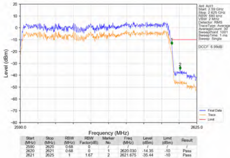
n38_15kHz_SISO_NTNV_30MHz_DFT-s-OFDM_PI/2_BPSK_2605MHz_Outer_Full
