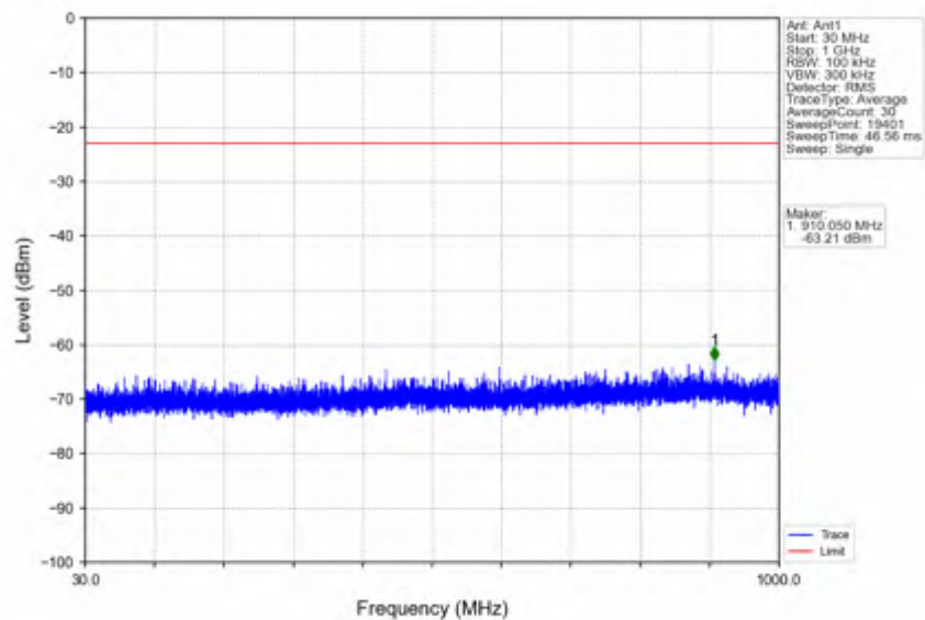
n38_15kHz_SISO_NTNV_30MHz_CP-OFDM QPSK_2595MHz_Edge_1RB_Left
