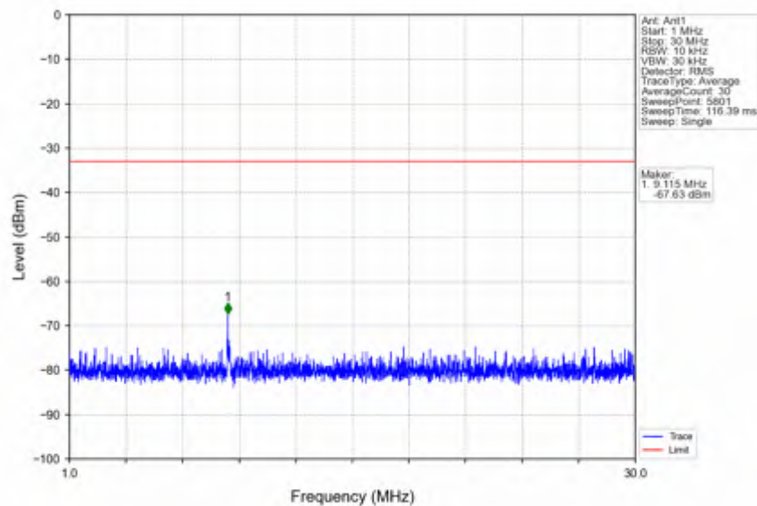
n38_15kHz_SISO_NTNV_10MHz_DFT-s-OFDM PI/2 BPSK_2575MHz_Edge_1RB_Left
