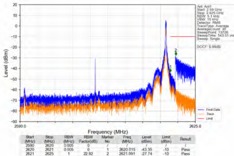
n38_15kHz_SISO_NTNV_30MHz_CP-OFDM_QPSK_2605MHz_Inner_1RB_Right
