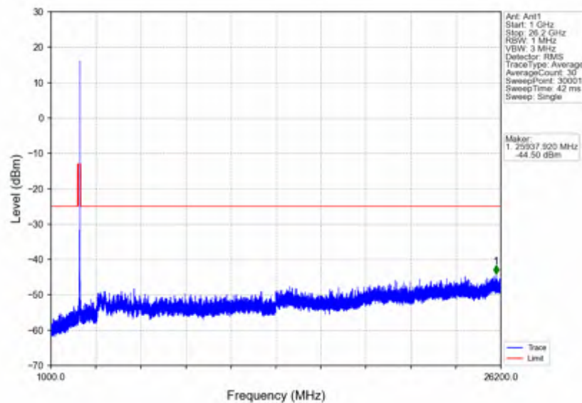
n38_15kHz_SISO_NTNV_40MHz_DFT-s-OFDM QPSK_2600MHz_Edge_1RB_Right
