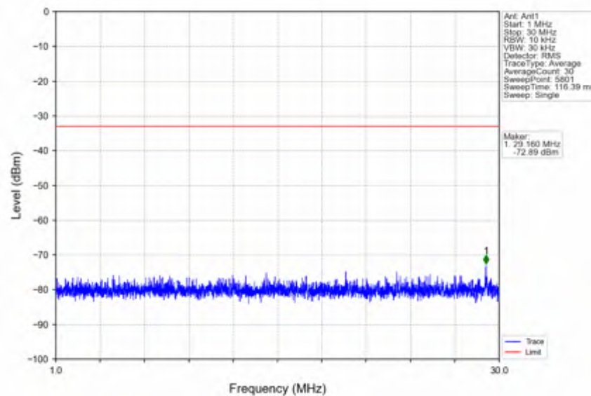
n38_15kHz_SISO_NTNV_10MHz_DFT-s-OFDM QPSK_2595MHz_Edge_1RB_Left
