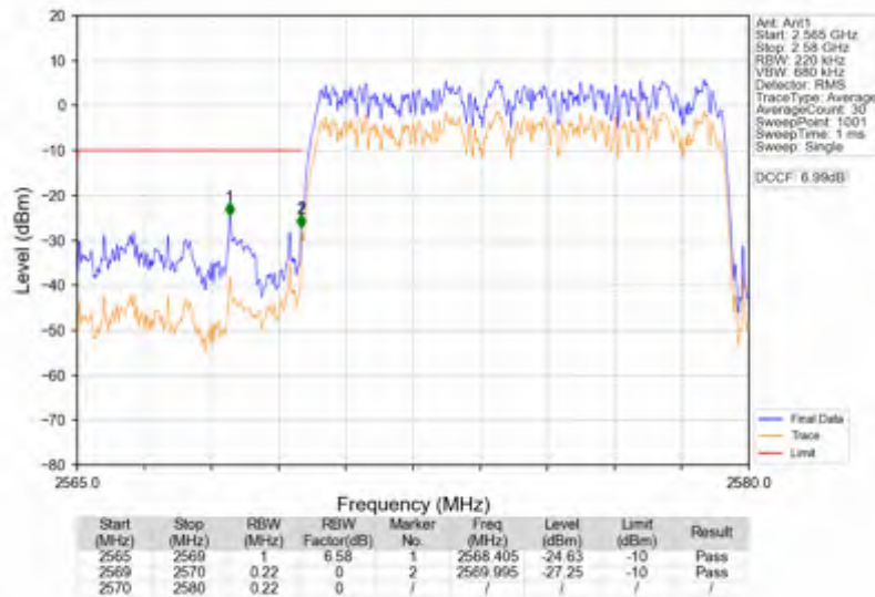
n38_15kHz_SISO_NTNV_10MHz_DFT-s-OFDM PI/2 BPSK_2575MHz_Outer_Full
