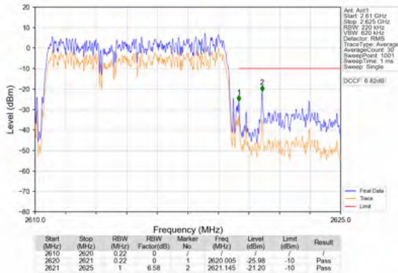
n38_30kHz_SISO_NTNV_10MHz_DFT-s-OFDM PI/2 BPSK_2615MHz_Outer_Full
