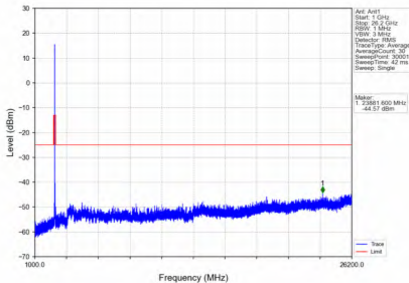
n38_15kHz_SISO_NTNV_30MHz_DFT-s-OFDM_QPSK_2585MHz_Outer_Full
