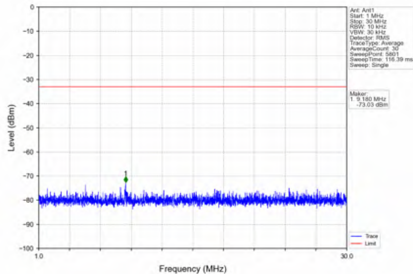
n38_15kHz_SISO_NTNV_10MHz_DFT-s-OFDM QPSK_2575MHz_Edge_1RB_Left
