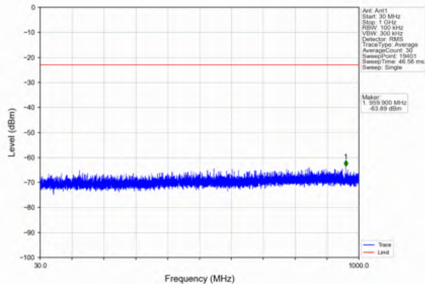
n38_15kHz_SISO_NTNV_10MHz_DFT-s-OFDM_PI/2_BPSK_2615MHz_Edge_1RB_Right
