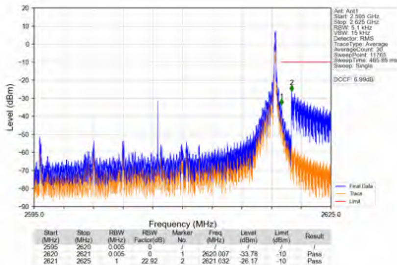
n38_15kHz_SISO_NTNV_25MHz_DFT-s-OFDM PI/2 BPSK_2607.5MHz_Edge_1RB_Right
