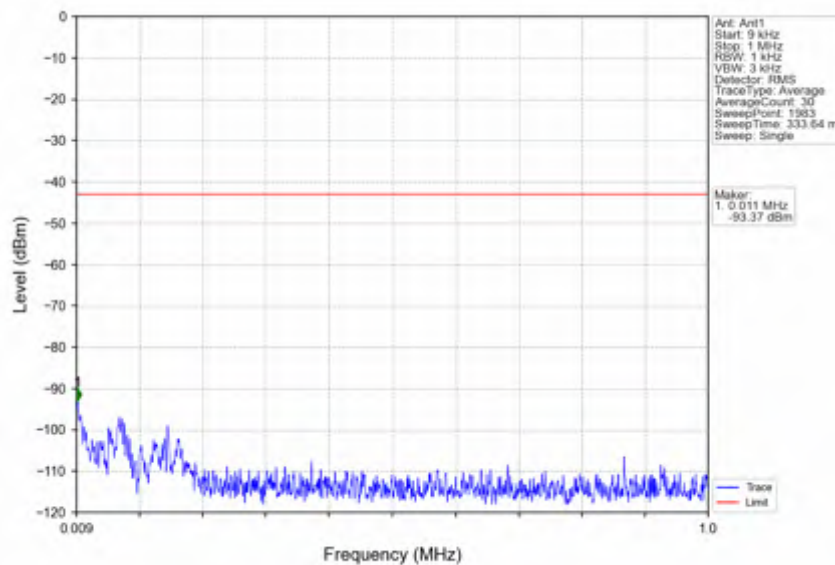
n38_15kHz_SISO_NTNV_40MHz_DFT-s-OFDM_PI/2_BPSK_2600MHz_Outer_Full
