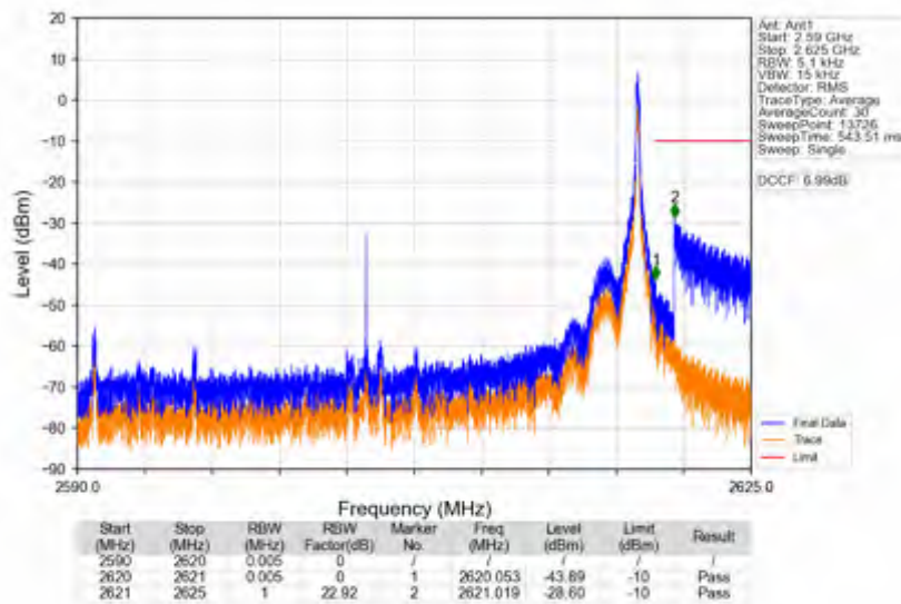
n38_15kHz_SISO_NTNV_30MHz_DFT-s-OFDM_PI/2_BPSK_2605MHz_Inner_1RB_Right
