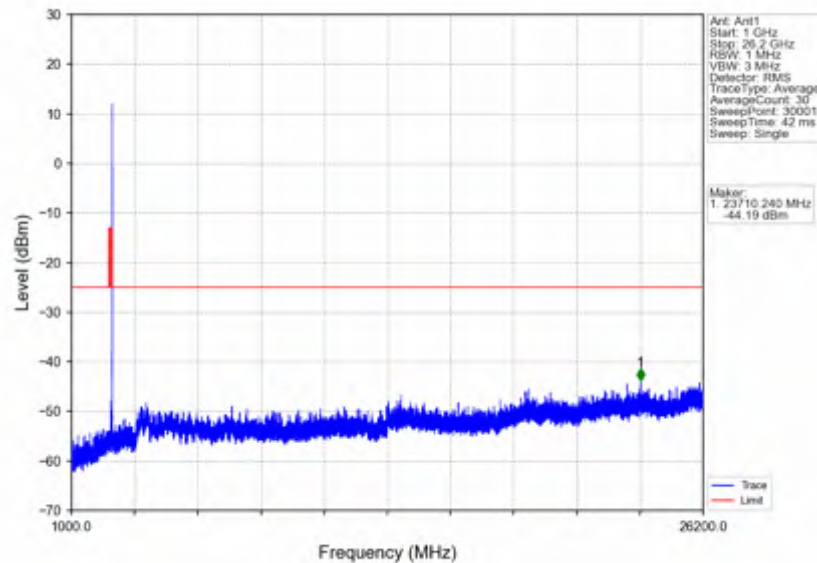
n38_15kHz_SISO_NTNV_10MHz_DFT-s-OFDM_PI/2_BPSK_2615MHz_Edge_1RB_Right
