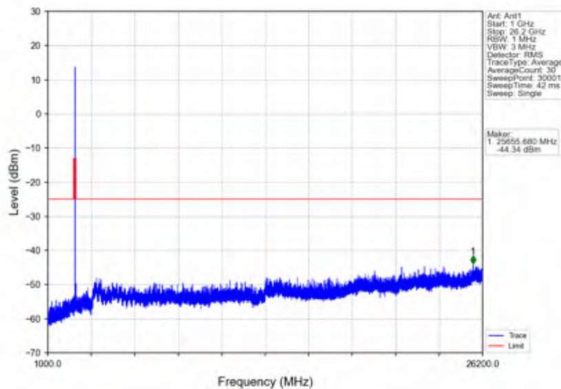
n38_15kHz_SISO_NTNV_15MHz_DFT-s-OFDM QPSK_2577.5MHz_Outer_Full
