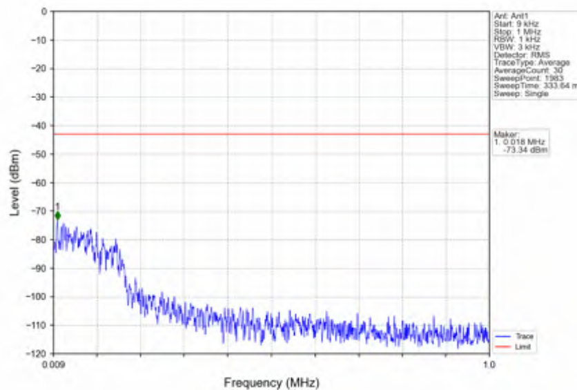
n38_15kHz_SISO_NTNV_25MHz_CP-OFDM QPSK_2595MHz_Edge_1RB_Left
