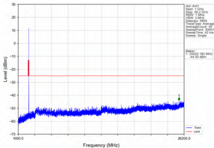
n38_15kHz_SISO_NTNV_15MHz_DFT-s-OFDM PI/2 BPSK_2612.5MHz_Edge_1RB_Right
