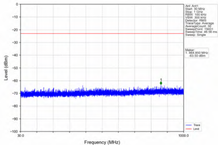
n38_15kHz_SISO_NTNV_30MHz_DFT-s-OFDM QPSK_2585MHz_Edge_1RB_Left
