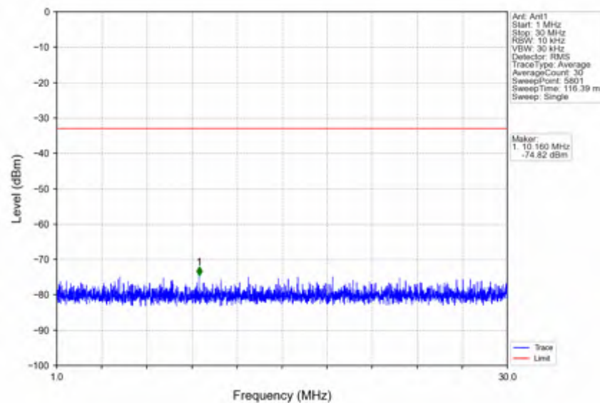
n38_15kHz_SISO_NTNV_30MHz_CP-OFDM QPSK_2605MHz_Edge_1RB_Right
