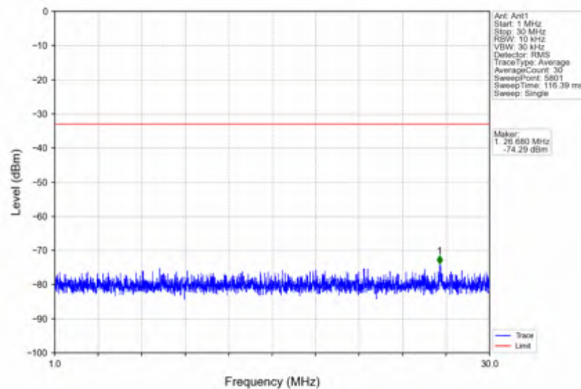
n38_15kHz_SISO_NTNV_15MHz_DFT-s-OFDM QPSK_2595MHz_Edge_1RB_Left
