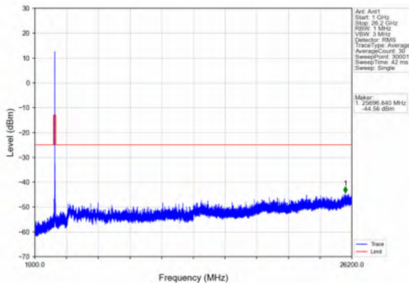
n38_15kHz_SISO_NTNV_40MHz_DFT-s-OFDM PI/2 BPSK_2600MHz_Edge_1RB_Right
