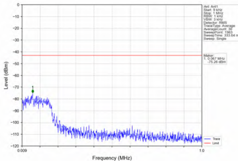
n38_15kHz_SISO_NTNV_30MHz_DFT-s-OFDM_QPSK_2595MHz_Edge_1RB_Left
