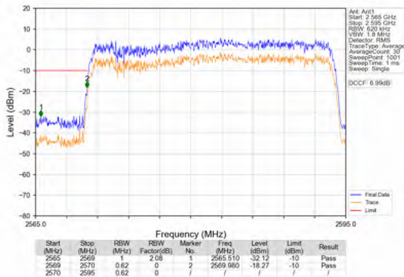
n38 15kHz SISO NTNV 25MHz DFT-s-OFDM QPSK 2582.5MHz Outer Full
