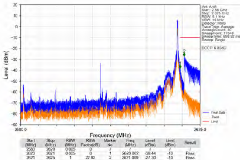
n38_15kHz_SISO_NTNV_40MHz_DFT-s-OFDM PI/2 BPSK_2600MHz_Edge_1RB_Right
