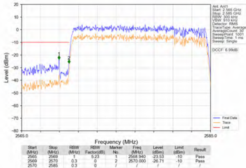
n38_15kHz_SISO_NTNV_15MHz_CP-OFDM QPSK_2577.5MHz_Outer_Full
