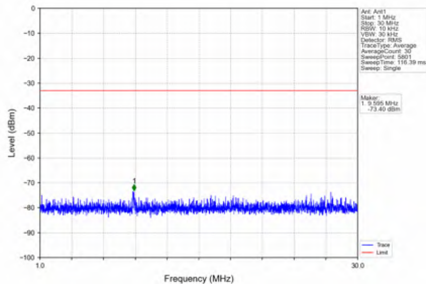
n38_30kHz_SISO_NTNV_10MHz_DFT-s-OFDM QPSK_2575MHz_Edge_1RB_Left
