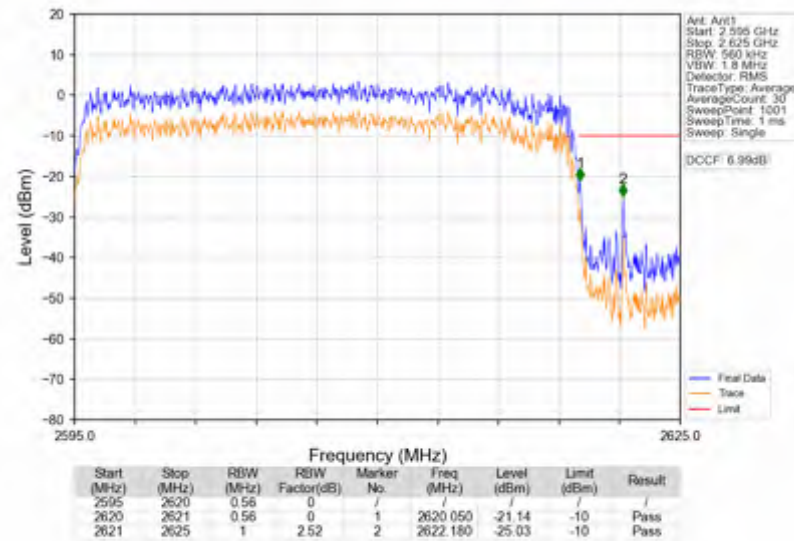
n38_15kHz_SISO_NTNV_25MHz_CP-OFDM QPSK_2607.5MHz_Outer_Full
