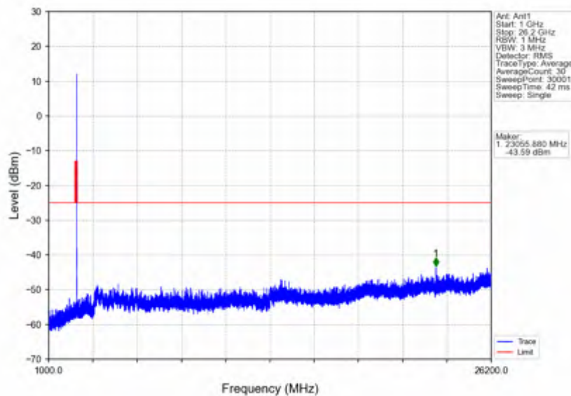
n38_30kHz_SISO_NTNV_10MHz_DFT-s-OFDM PI/2 BPSK_2615MHz_Edge_1RB_Right
