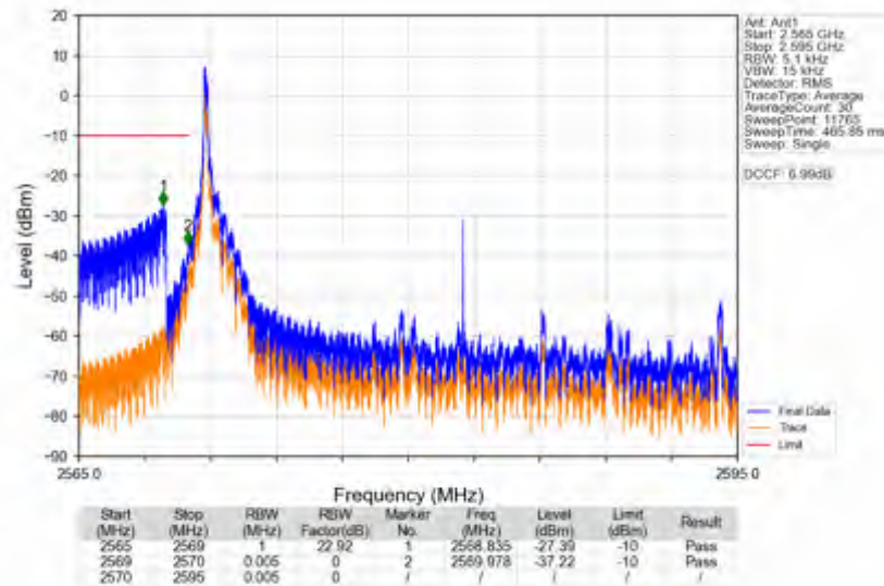
n38_15kHz_SISO_NTNV_25MHz_DFT-s-OFDM_PI/2_BPSK_2582.5MHz_Inner_1RB_Left
