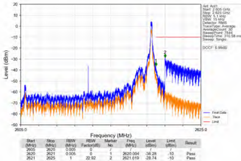
n38_15kHz_SISO_NTNV_15MHz_DFT-s-OFDM_QPSK_2612.5MHz_Edge_1RB_Right
