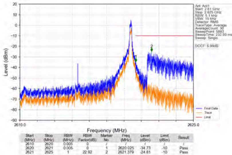
n38_15kHz_SISO_NTNV_10MHz_CP-OFDM QPSK_2615MHz_Edge_1RB_Right
