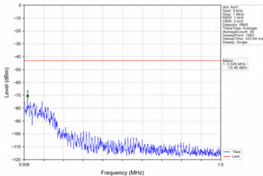
n38_15kHz_SISO_NTNV_15MHz_CP-OFDM QPSK_2612.5MHz_Edge_1RB_Right
