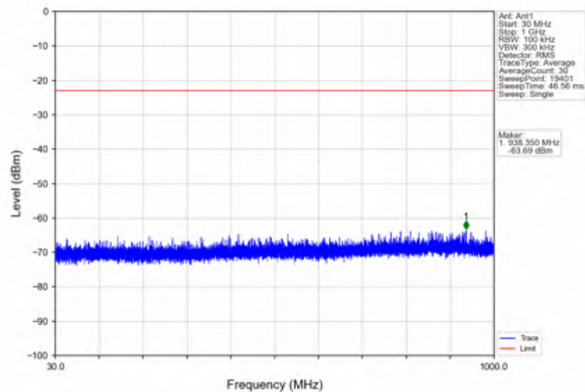
n38_15kHz_SISO_NTNV_10MHz_CP-OFDM QPSK_2615MHz_Edge_1RB_Right
