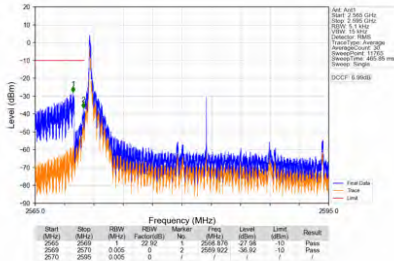
n38_15kHz_SISO_NTNV_25MHz_CP-OFDM_QPSK_2582.5MHz_Edge_1RB_Left
