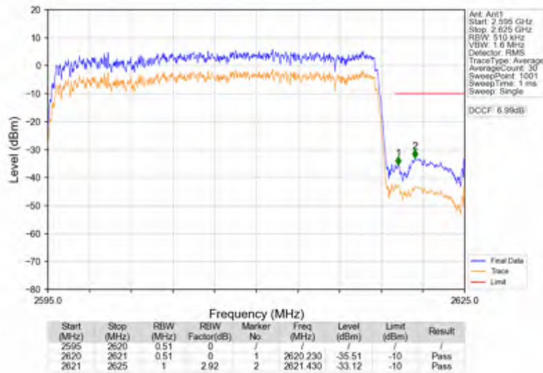
n38_15kHz_SISO_NTNV_25MHz_DFT-s-OFDM PI/2 BPSK_2607.5MHz_Outer_Full
