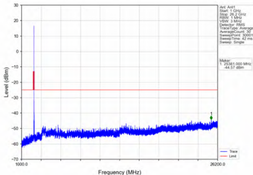
n38_15kHz_SISO_NTNV_25MHz_DFT-s-OFDM PI/2 BPSK_2607.5MHz_Edge_1RB_Right
