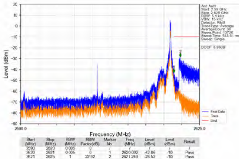
n38_15kHz_SISO_NTNV_30MHz_CP-OFDM QPSK_2605MHz_Edge_1RB_Right
