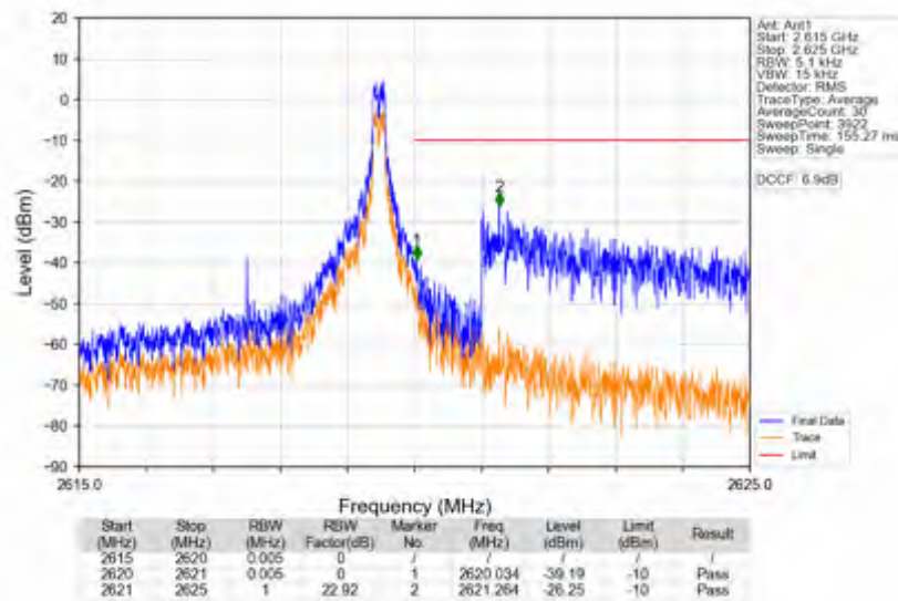
n38_15kHz_SISO_NTNV_5MHz_CP-OFDM QPSK_2617.5MHz_Inner_1RB_Right
