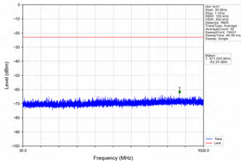
n38_15kHz_SISO_NTNV_15MHz_DFT-s-OFDM QPSK_2612.5MHz_Edge_1RB_Right
