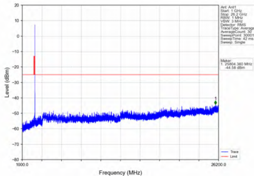
n38_15kHz_SISO_NTNV_10MHz_CP-OFDM QPSK_2615MHz_Edge_1RB_Right
