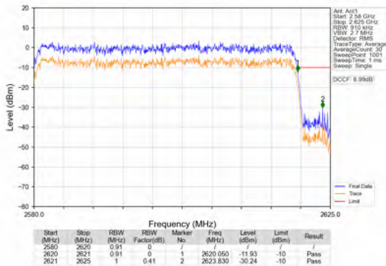
n38_15kHz_SISO_NTNV_40MHz_CP-OFDM QPSK_2600MHz_Outer_Full
