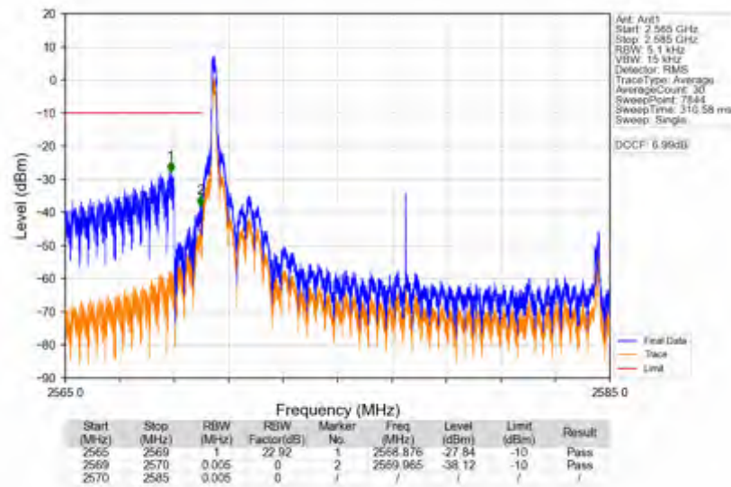
n38_15kHz_SISO_NTNV_15MHz_DFT-s-OFDM PI/2 BPSK_2577.5MHz_Edge_1RB_Left
