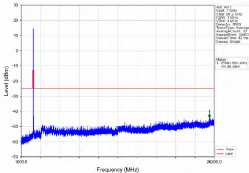
n38_15kHz_SISO_NTNV_30MHz_DFT-s-OFDM PI/2 BPSK_2585MHz_Outer_Full
