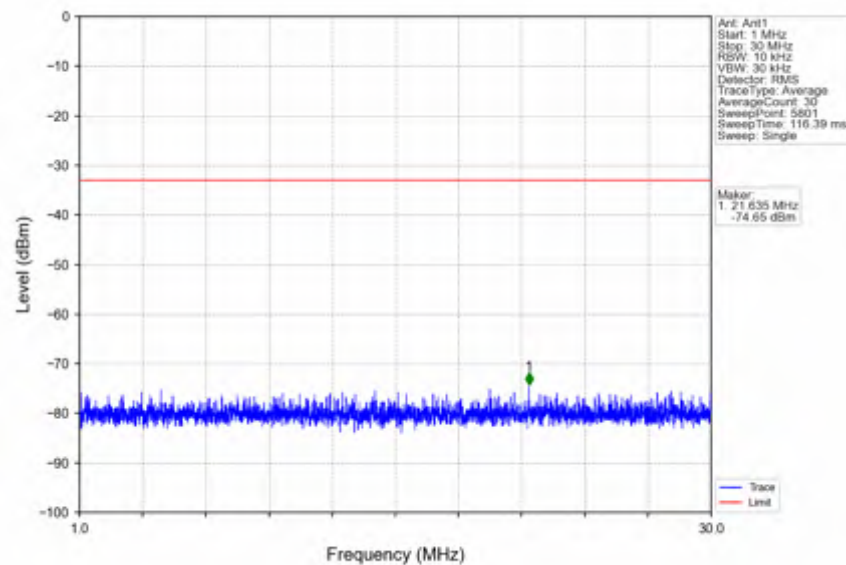
n38_15kHz_SISO_NTNV_10MHz_DFT-s-OFDM_QPSK_2615MHz_Edge_1RB_Right
