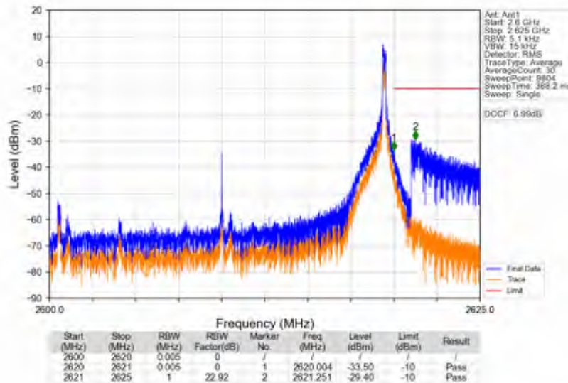
n38_15kHz_SISO_NTNV_20MHz_DFT-s-OFDM QPSK_2610MHz_Edge_1RB_Right
