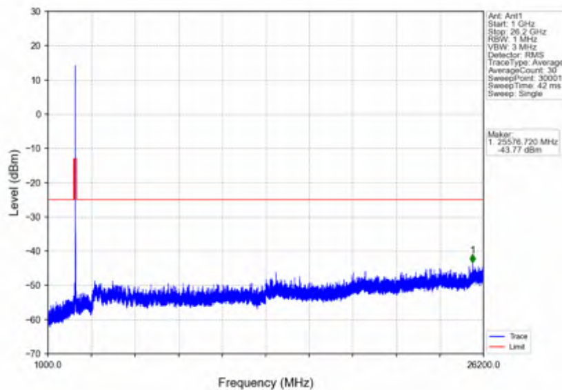
n38_15kHz_SISO_NTNV_30MHz_DFT-s-OFDM QPSK_2605MHz_Edge_1RB_Right
