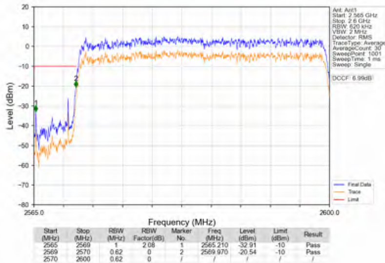
n38_15kHz_SISO_NTNV_30MHz_DFT-s-OFDM PI/2 BPSK_2585MHz_Outer_Full
