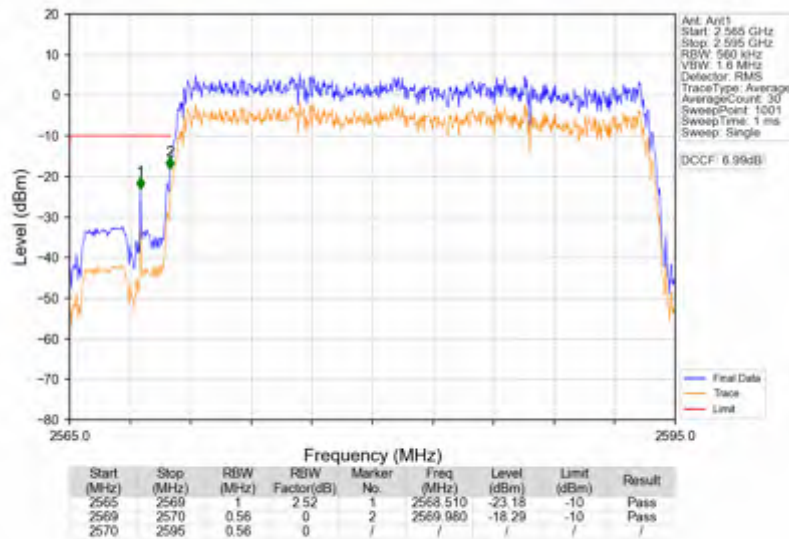
n38_15kHz_SISO_NTNV_25MHz_DFT-s-OFDM PI/2 BPSK_2582.5MHz_Outer_Full
