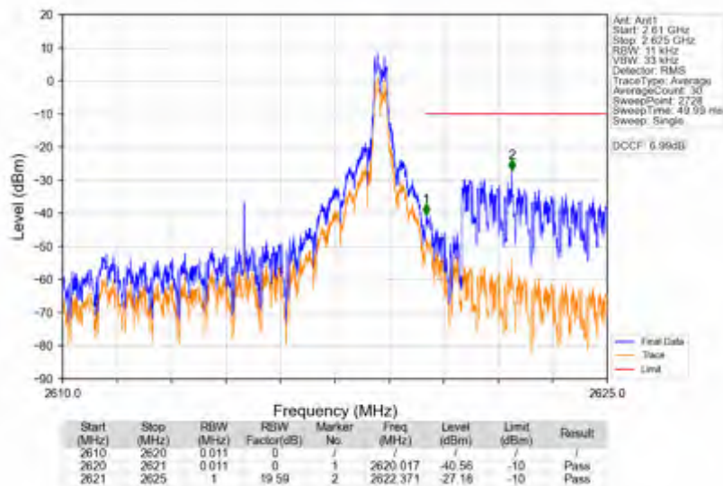
n38_30kHz_SISO_NTNV_10MHz_DFT-s-OFDM PI/2 BPSK_2615MHz_Inner_1RB_Right
