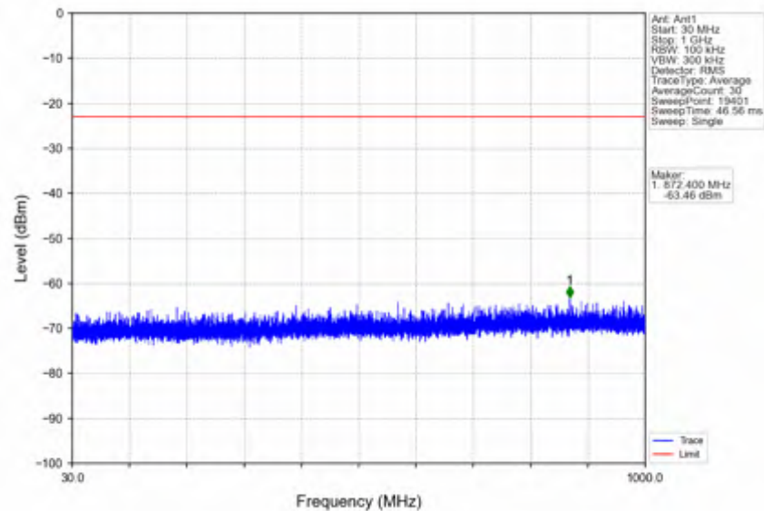
n38_15kHz_SISO_NTNV_40MHz_DFT-s-OFDM QPSK_2595MHz_Edge_1RB_Left
