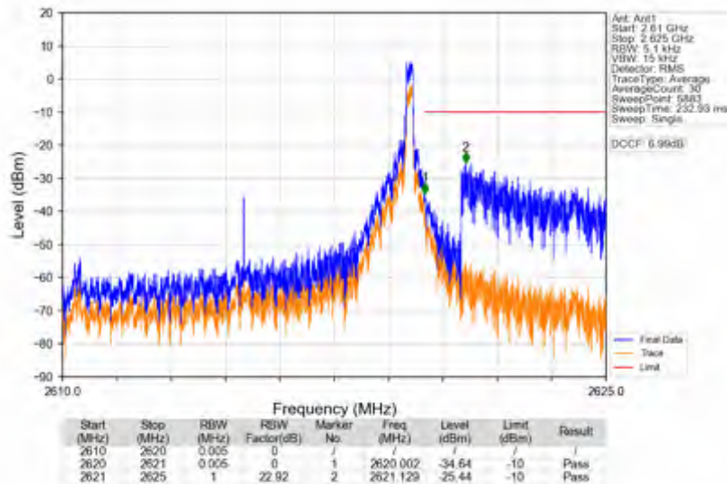
n38_15kHz_SISO_NTNV_10MHz_DFT-s-OFDM QPSK_2615MHz_Edge_1RB_Right
