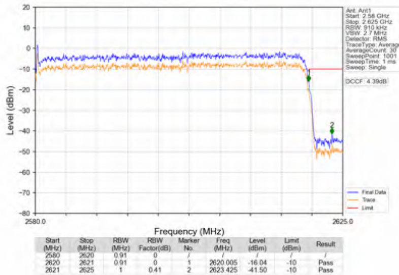
n38_15kHz_SISO_NTNV_40MHz_DFT-s-OFDM_PI/2_BPSK_2600MHz_Outer_Full
