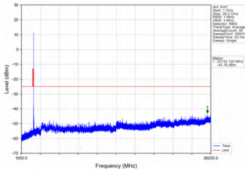
n38_15kHz_SISO_NTNV_15MHz_DFT-s-OFDM QPSK_2612.5MHz_Edge_1RB_Right
