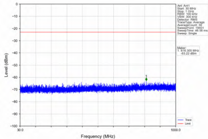
n38 15kHz SISO NTV 40MHz DFT-s-OFDM QPSK 2590MHz Outer Full
