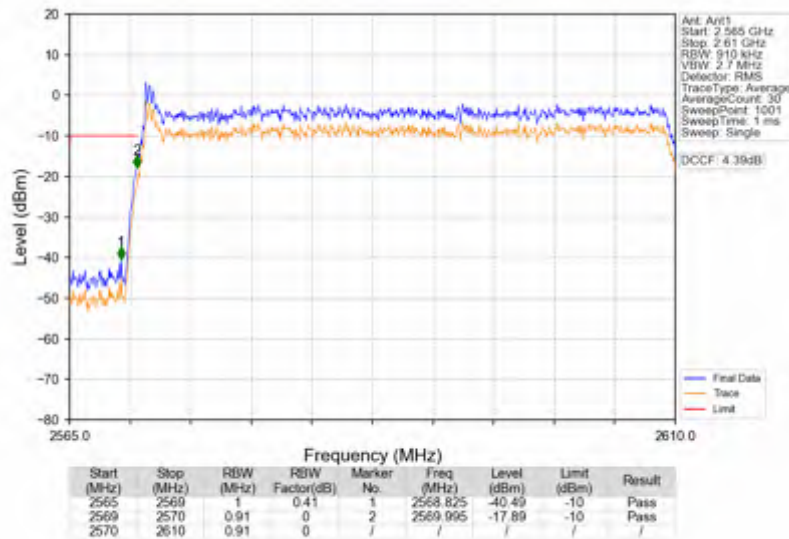
n38_15kHz_SISO_NTNV_40MHz_DFT-s-OFDM QPSK_2590MHz_Outer_Full
