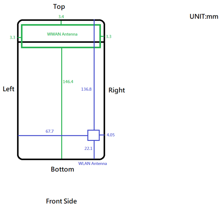
Fig.11 Antenna position of EUT
