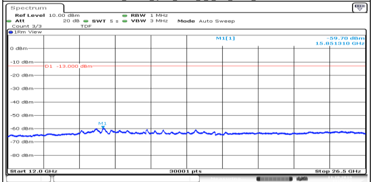
Band26_1.4MHz_QPSK_26797_1_0_Low_12000_26500
