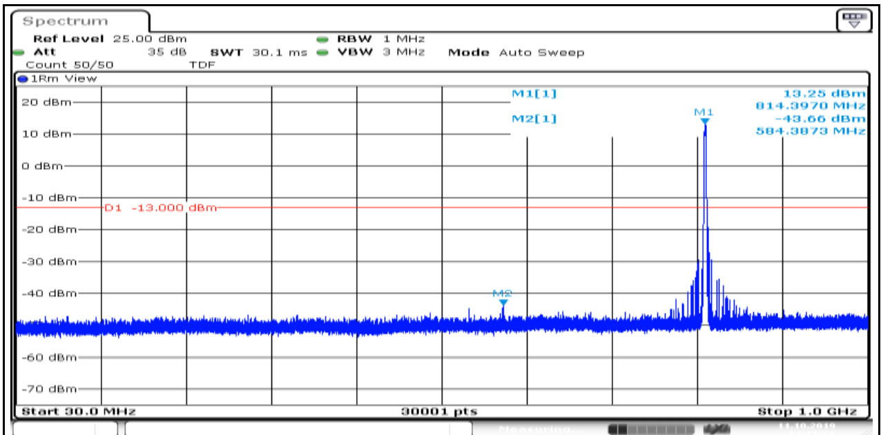
Band26_1.4MHz_QPSK_26697_1_0_Low_5000_12000
