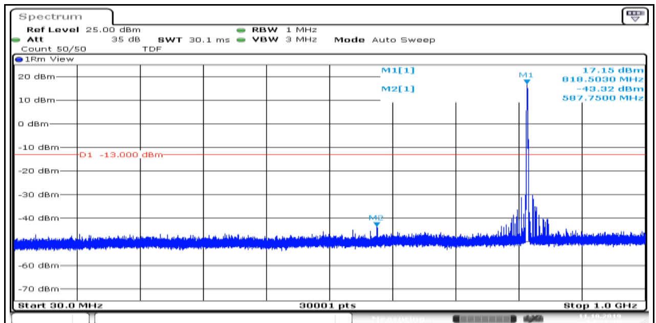
Band26_1.4MHz_QPSK_26740_1_0_Low_1000_5000
