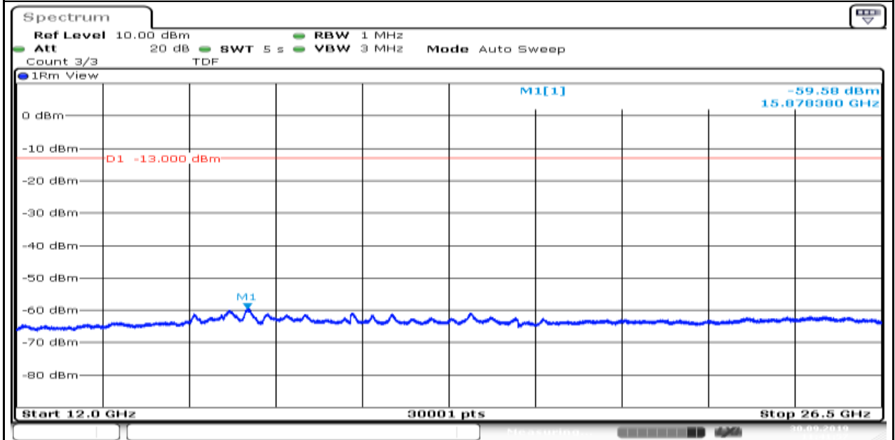
Band66_1.4MHz_QPSK_131979_1
