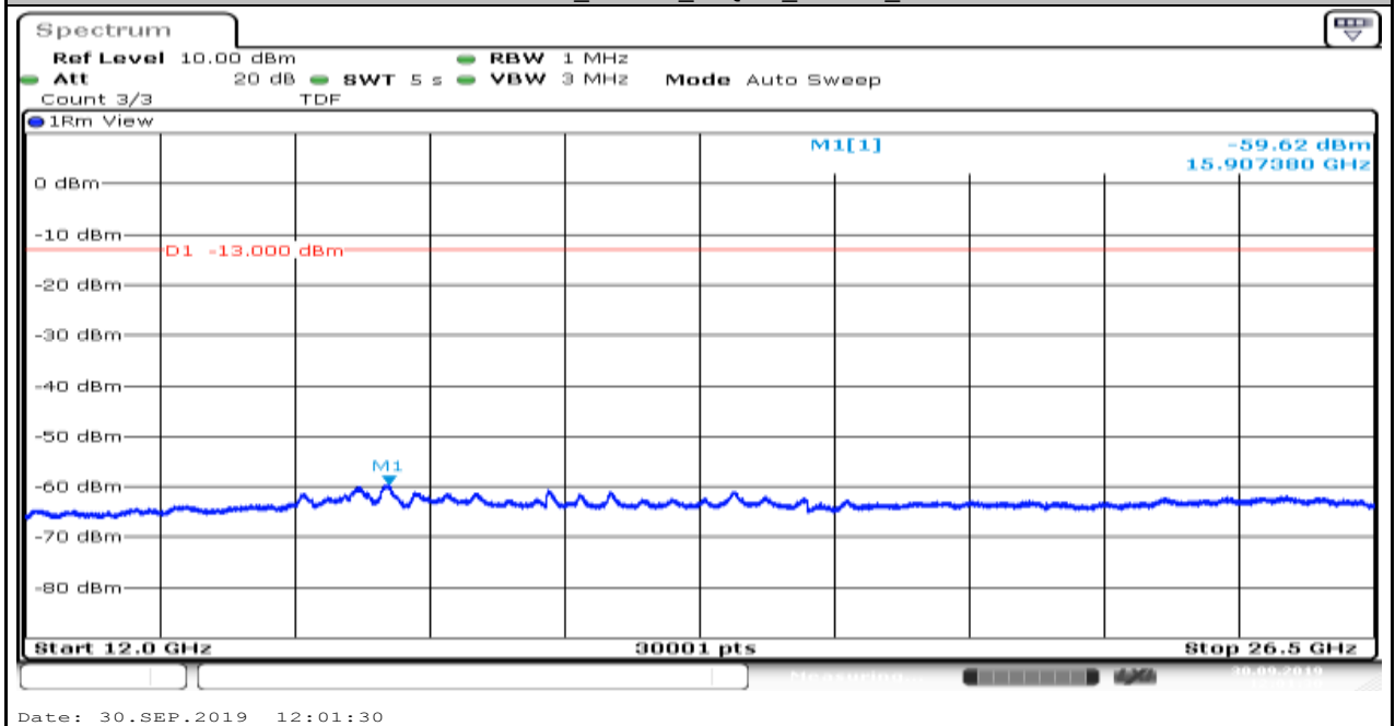
Band66_1.4MHz_16QAM_132665_1
