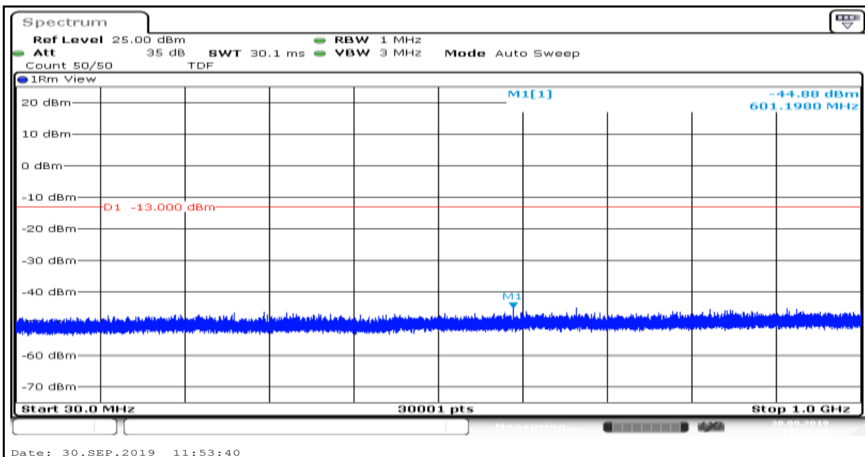
Band66_1.4MHz_16QAM_132322_1
