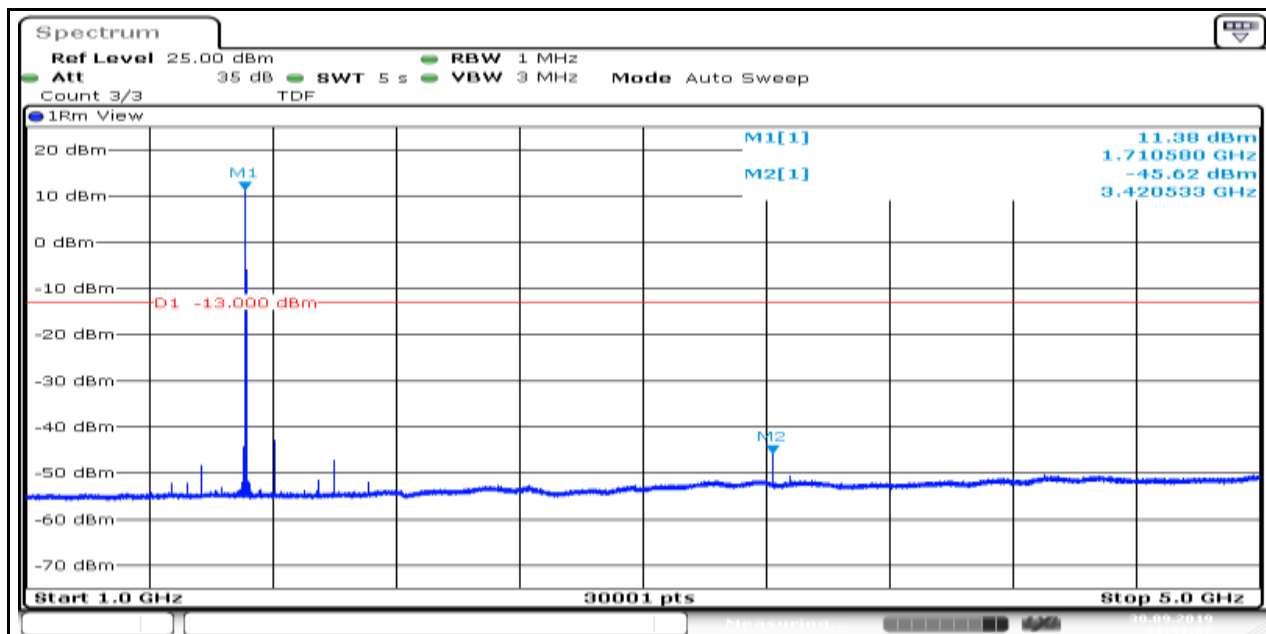
Band66_1.4MHz_QPSK_131979_1
