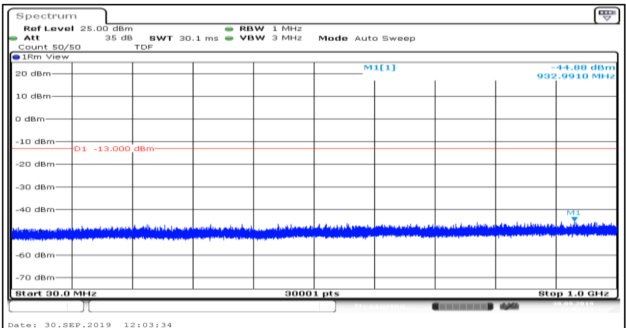
Band66_1.4MHz_16QAM_132665_1
