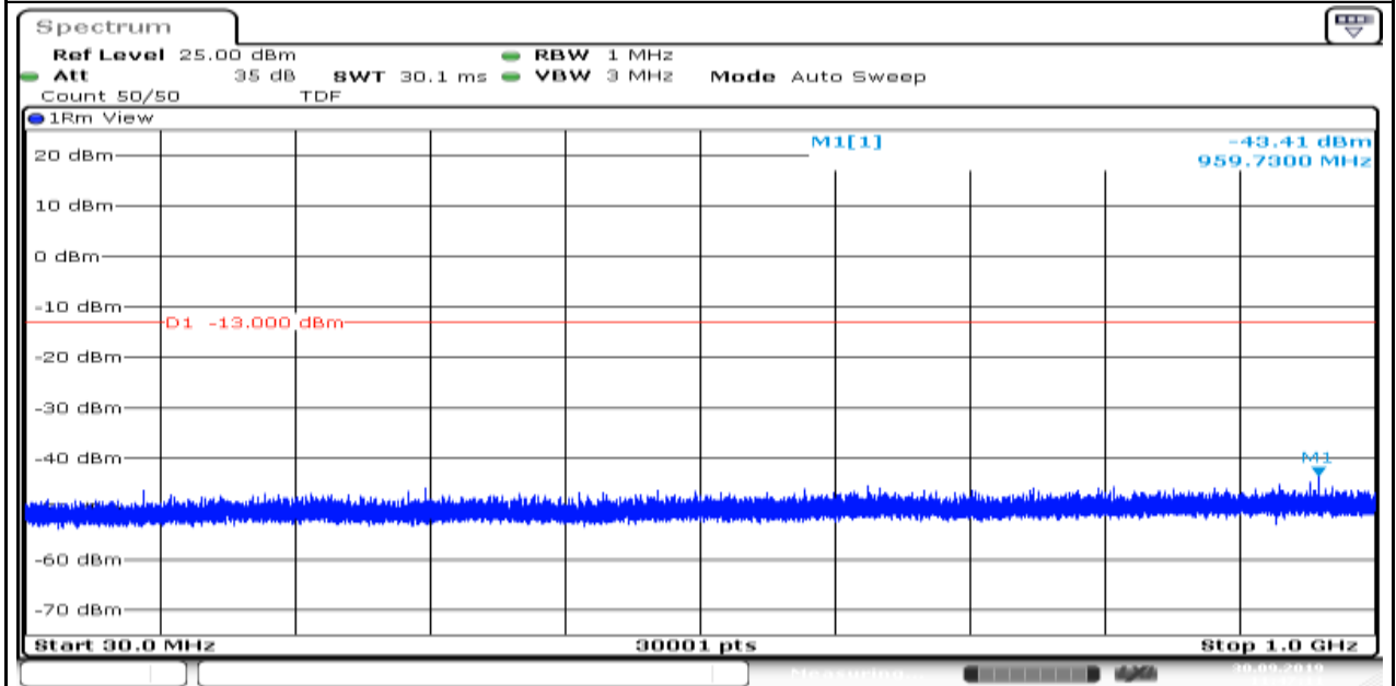
Band66_1.4MHz_QPSK_132322_1
