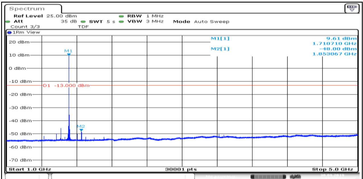
Band66_1.4MHz_QPSK_131979_1
