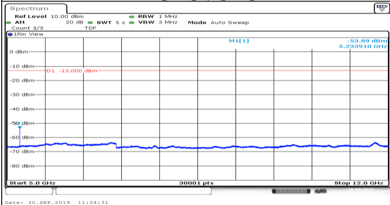
Band66_1.4MHz_16QAM_132665_6
