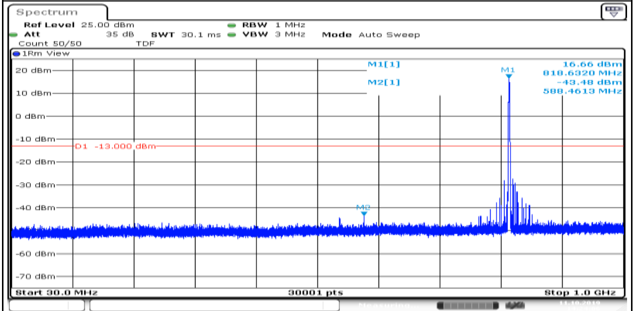
Band26_1.4MHz_16QAM_26740_1_0_Low_30_1000
