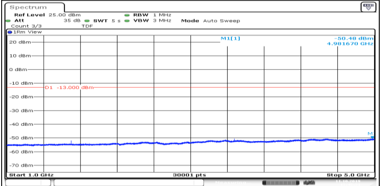
Band26_1.4MHz_16QAM_27033_1_5_Low_1000_5000
