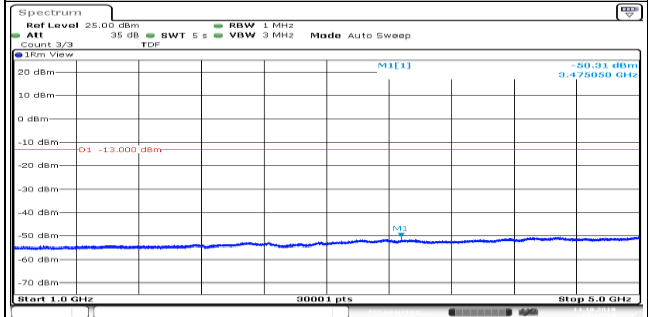
Band26_1.4MHz_QPSK_26740_1_0_Low_1000_5000
