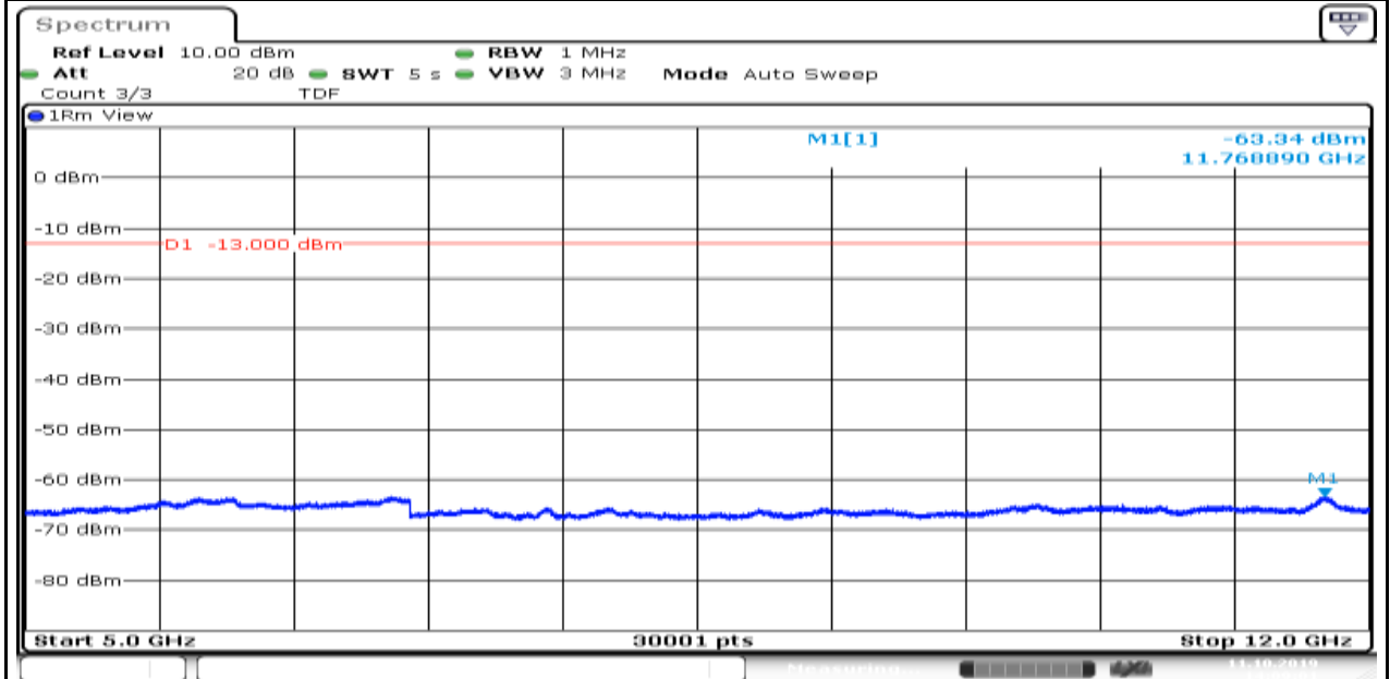
Band26_1.4MHz_QPSK_26697_1_0_Low_5000_12000
