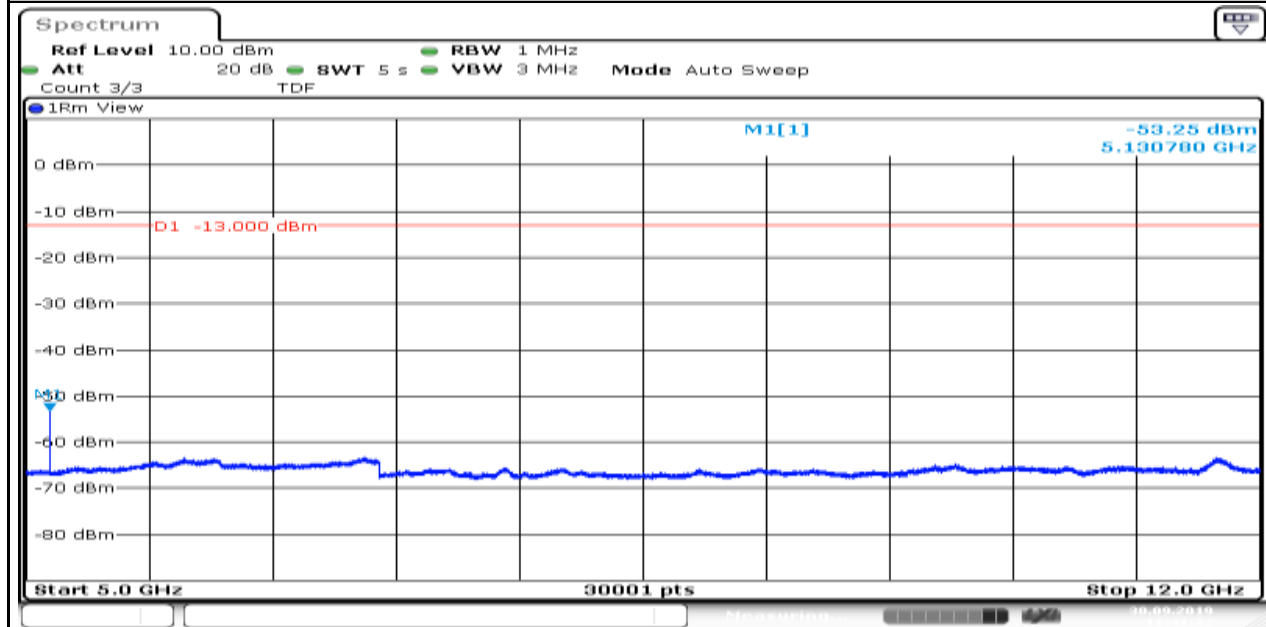
Band66_1.4MHz_QPSK_131979_1
