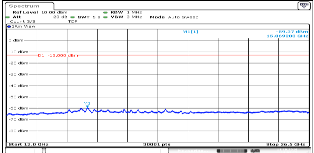
Band26_1.4MHz_QPSK_26697_1_0_Low_12000_26500
