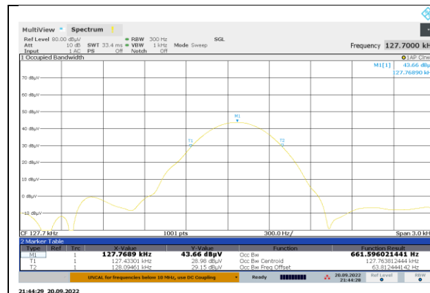
CONFIGURATION 1 (127.7kHz)
