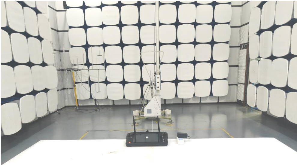
Radiated Emission
